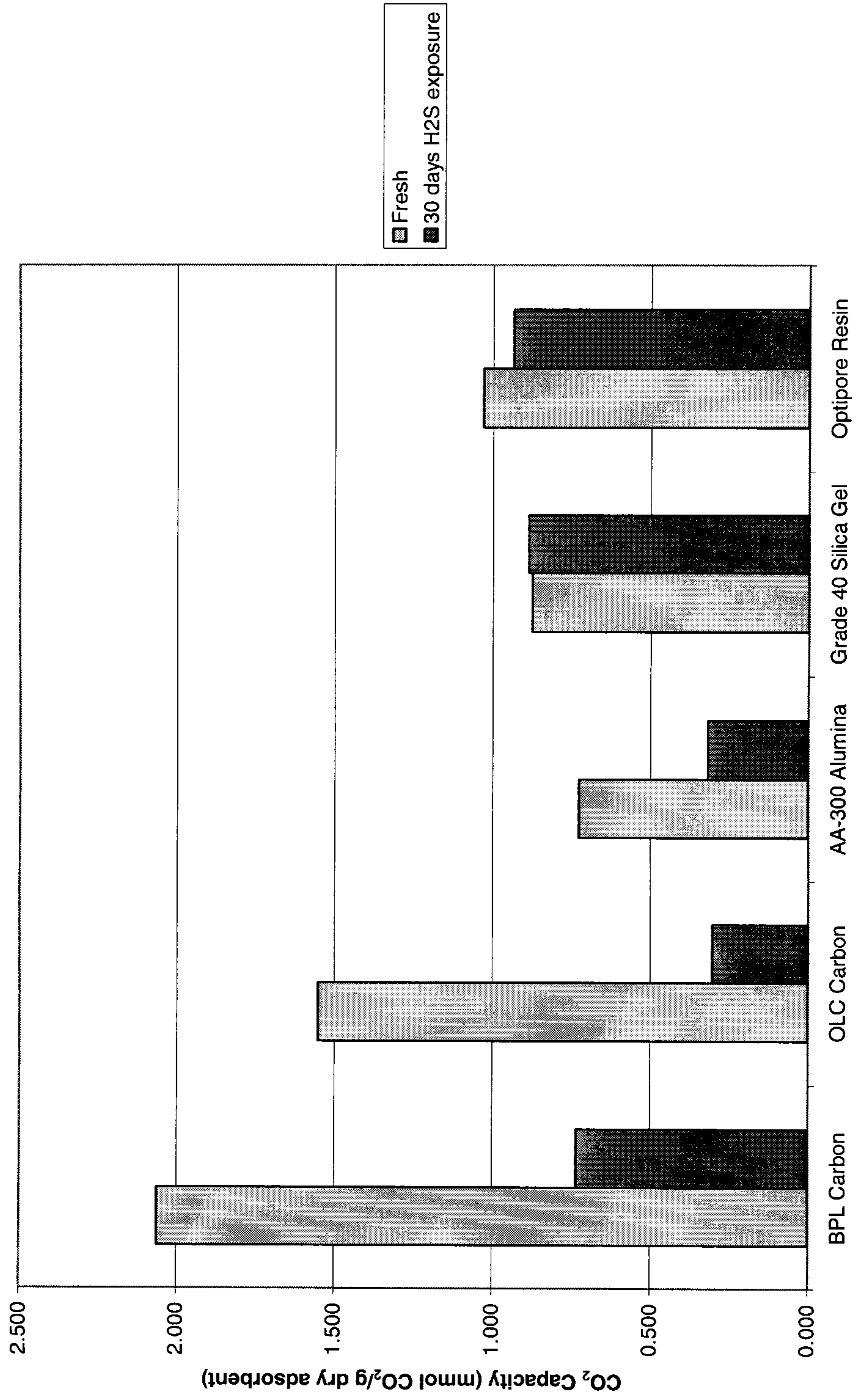
Figure 10. Effect of H 2 S exposure on CO 2 Capacity
