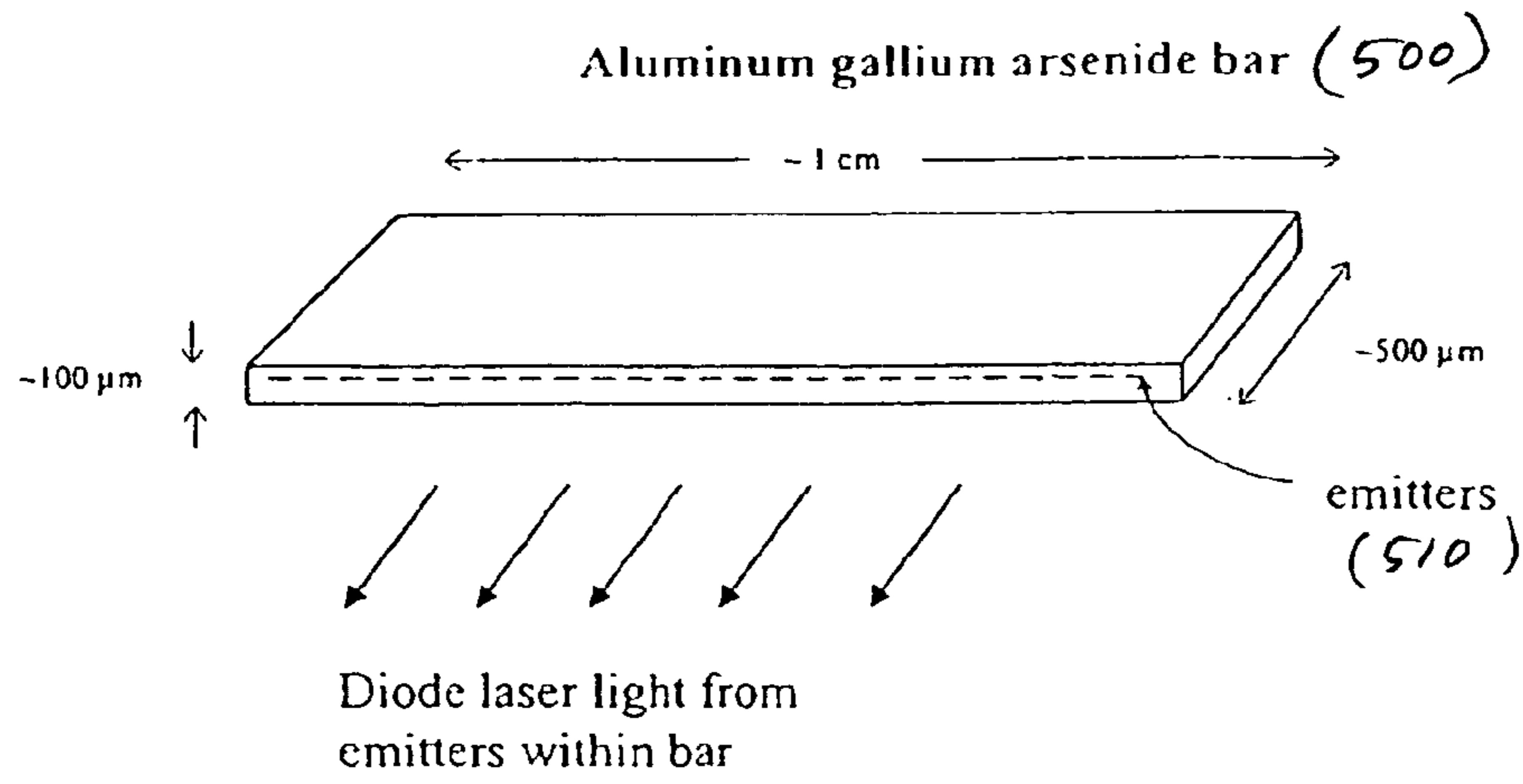
FIGURE 9 (PRIOR ART)
