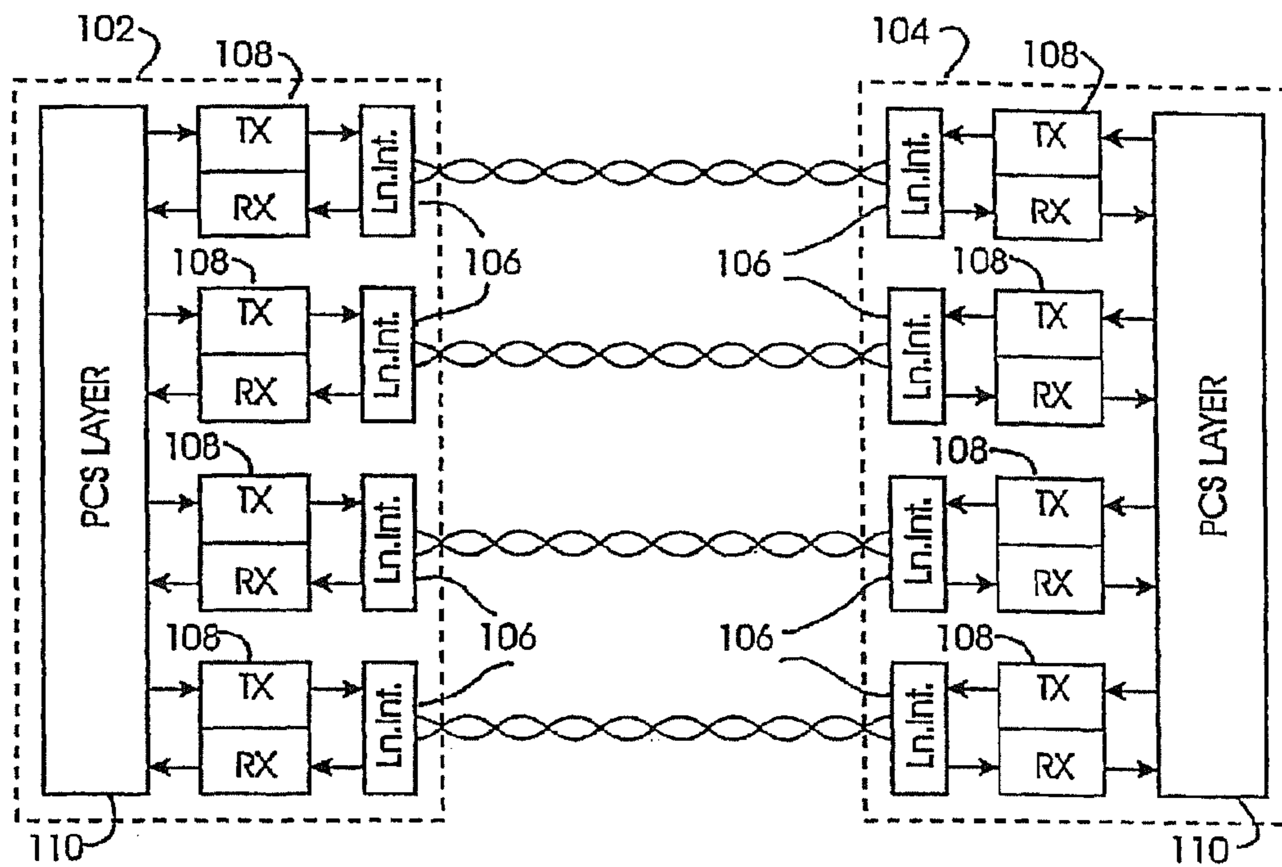
FIG. 1 (PRIOR ART)
