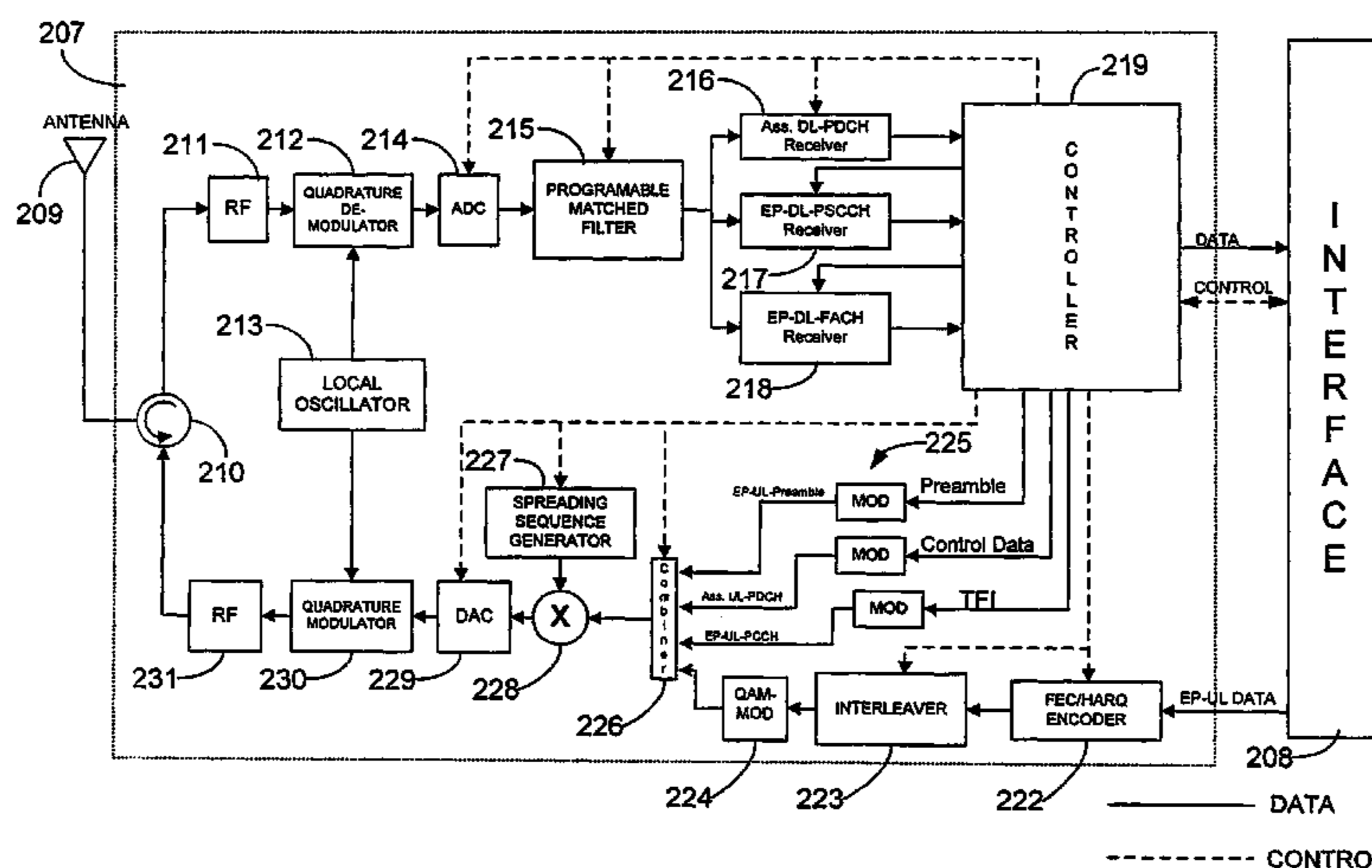
Remote Station Transceiver for Enhanced Uplink Packet Communications.
