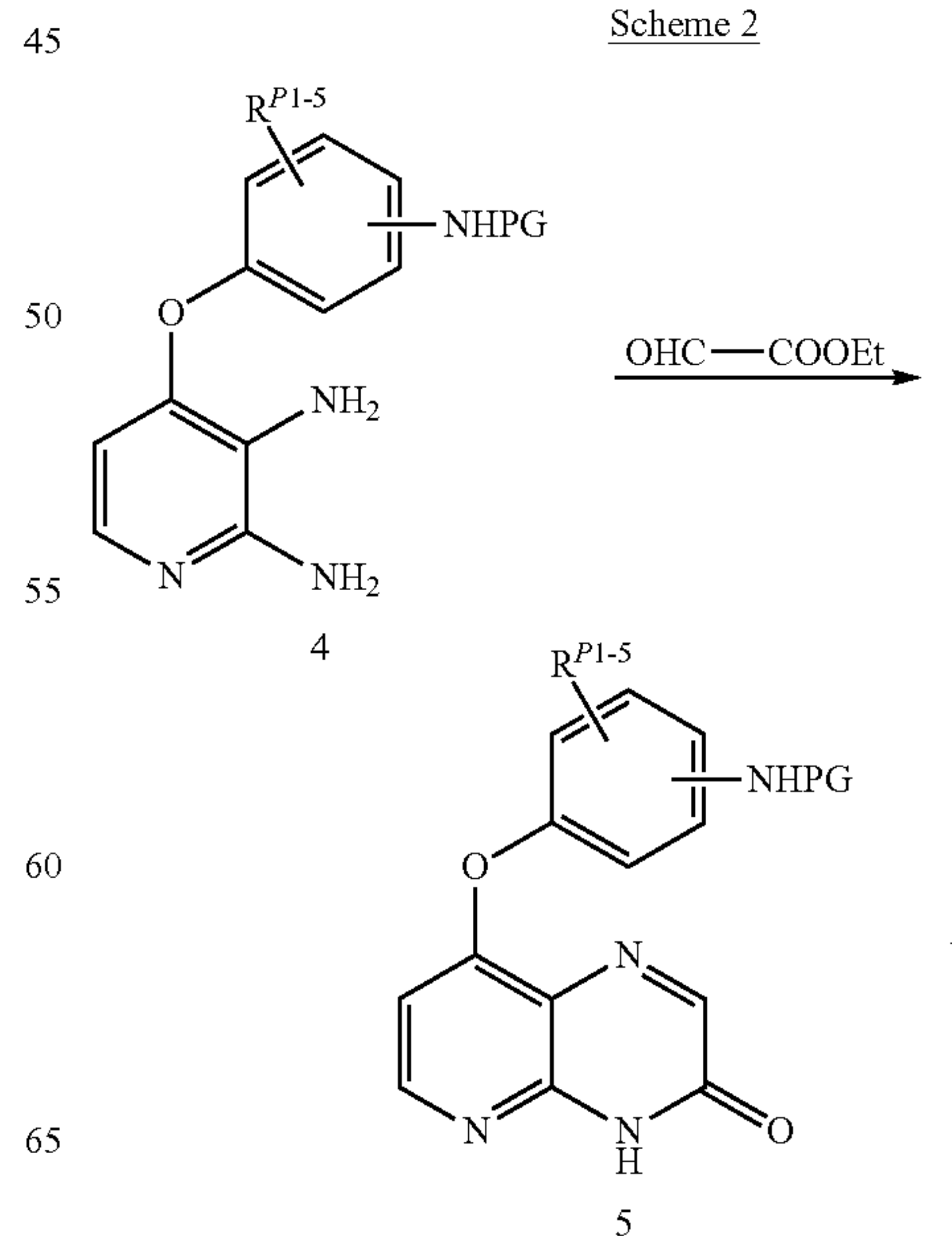
Scheme 2
