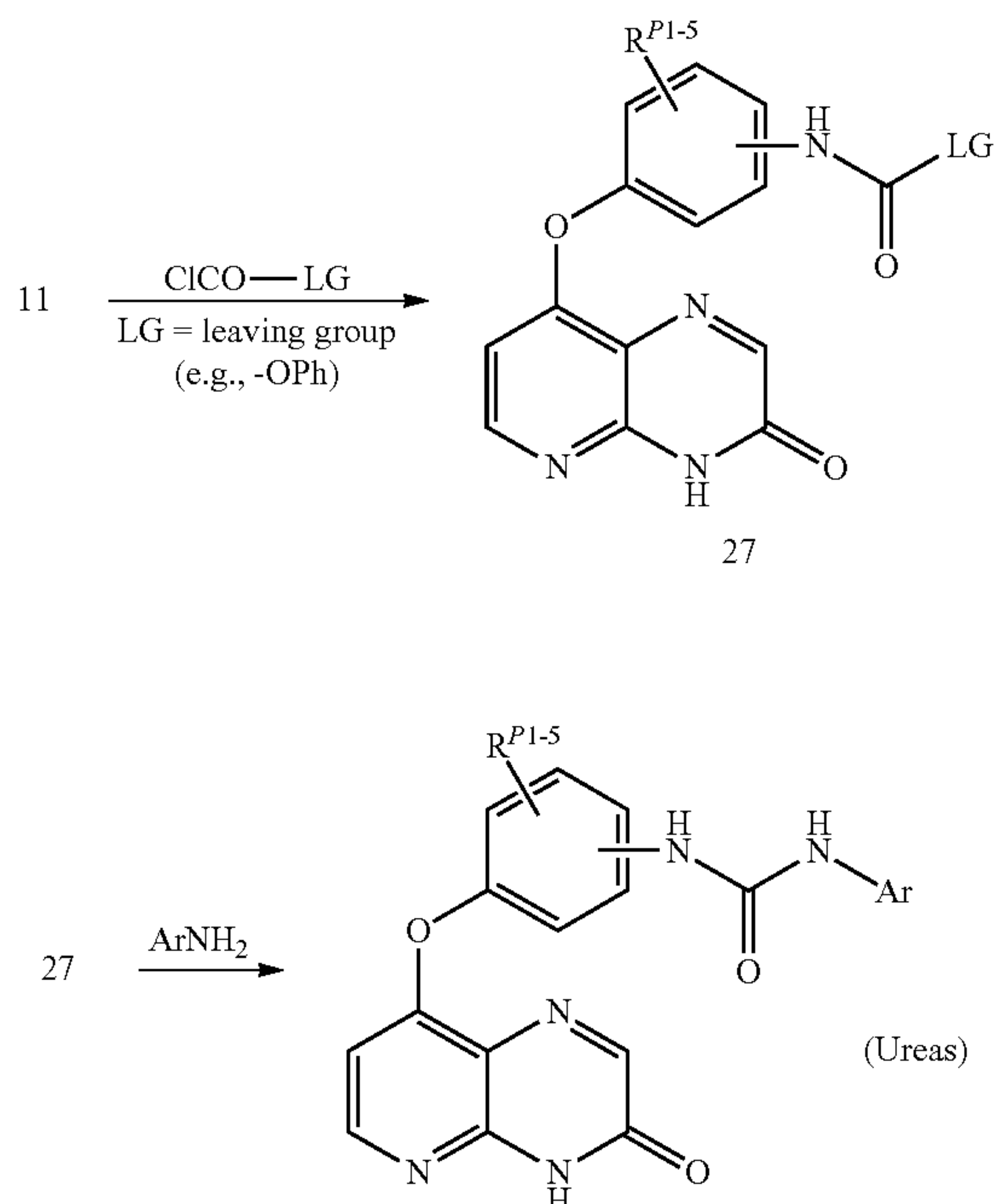
Scheme 8
