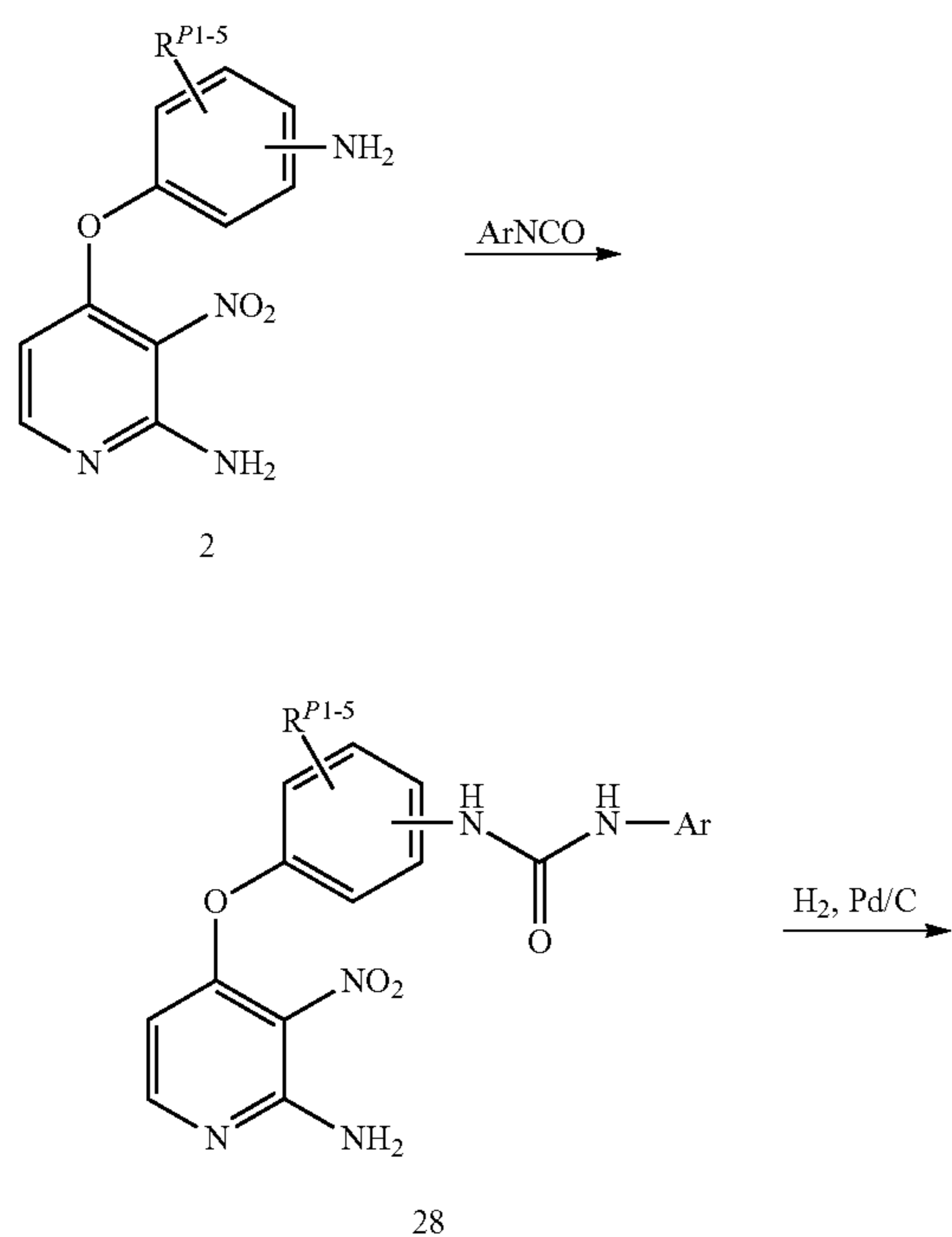
Scheme 9
