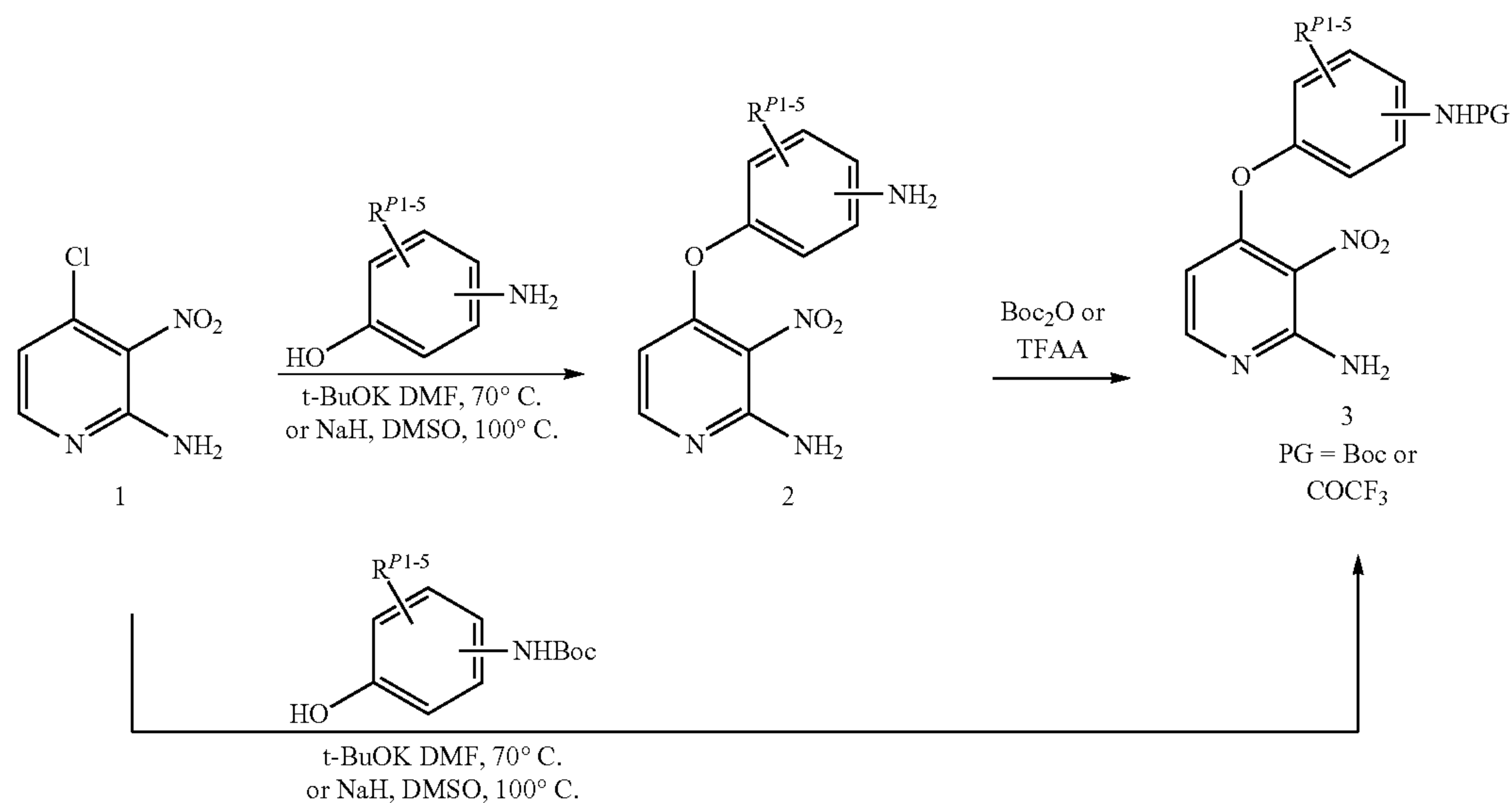
Scheme 1
