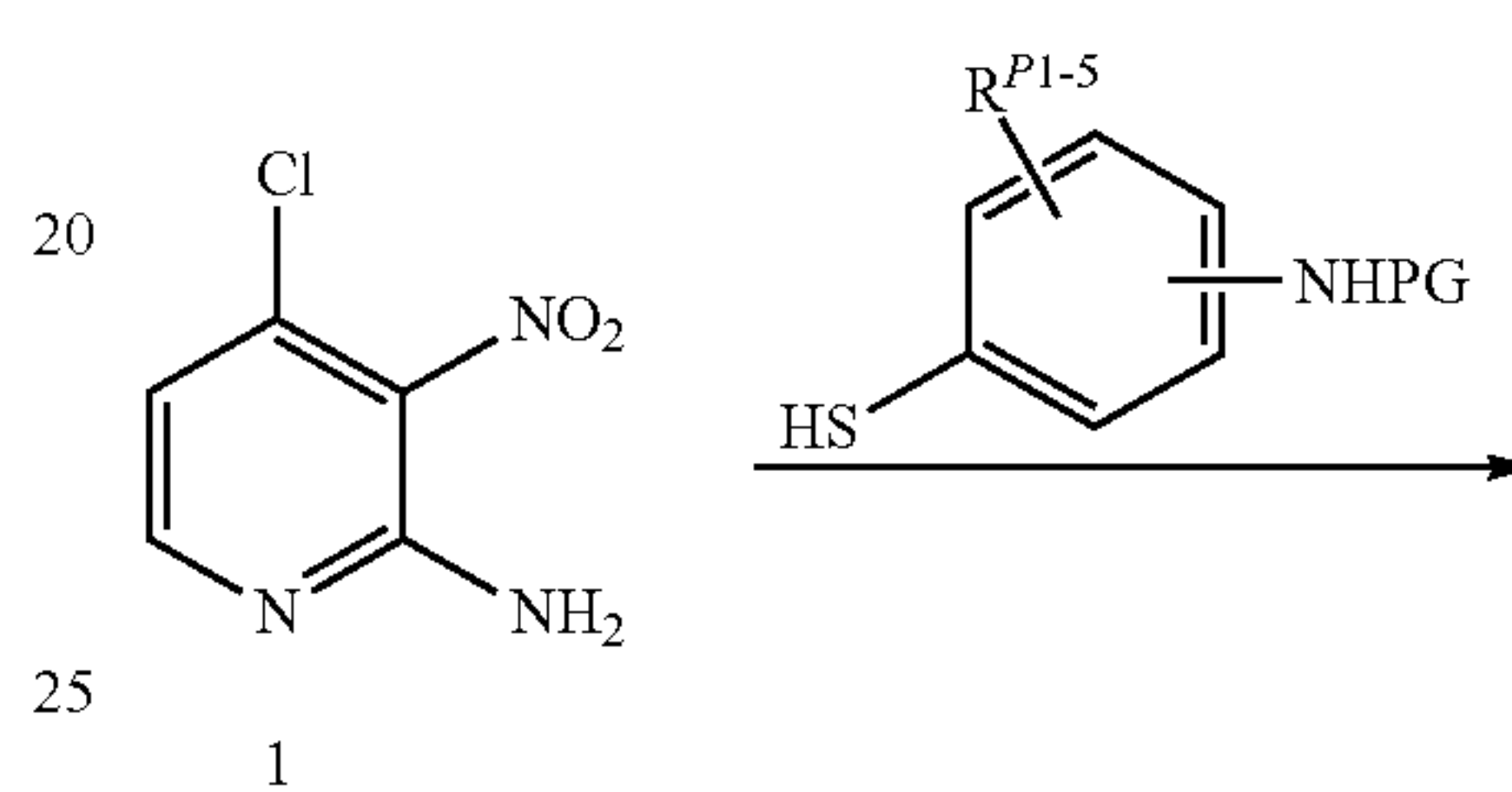
Scheme 11
