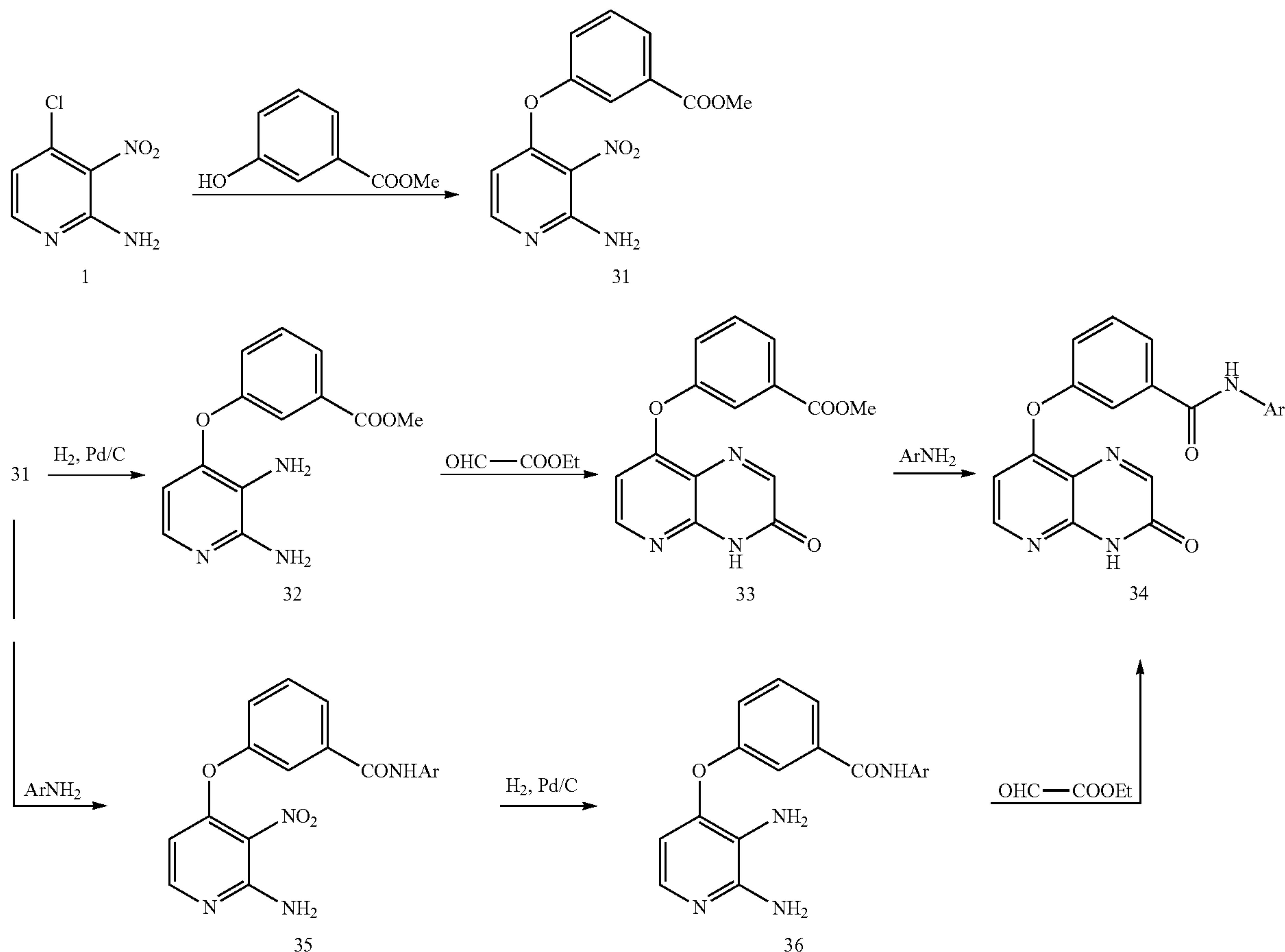
Scheme 10
