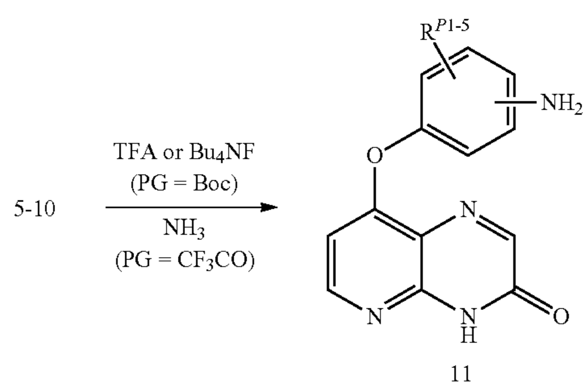
Scheme 3
