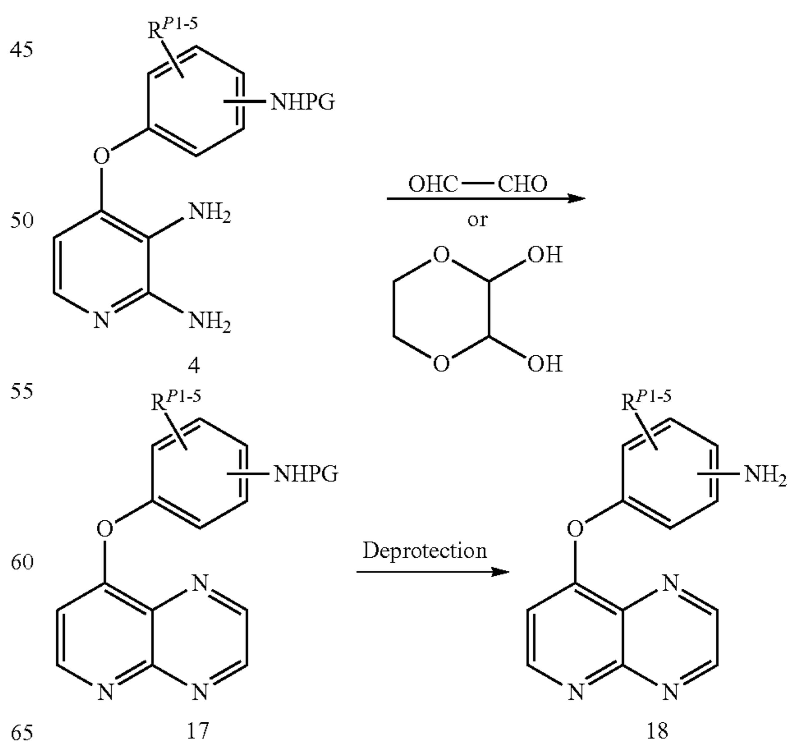
Scheme 4
