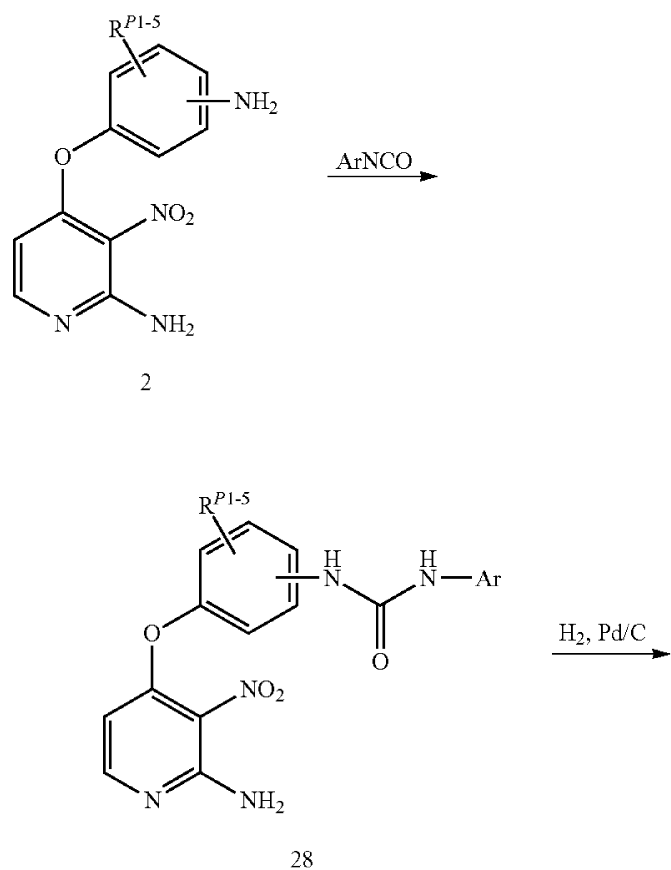
Scheme 9
