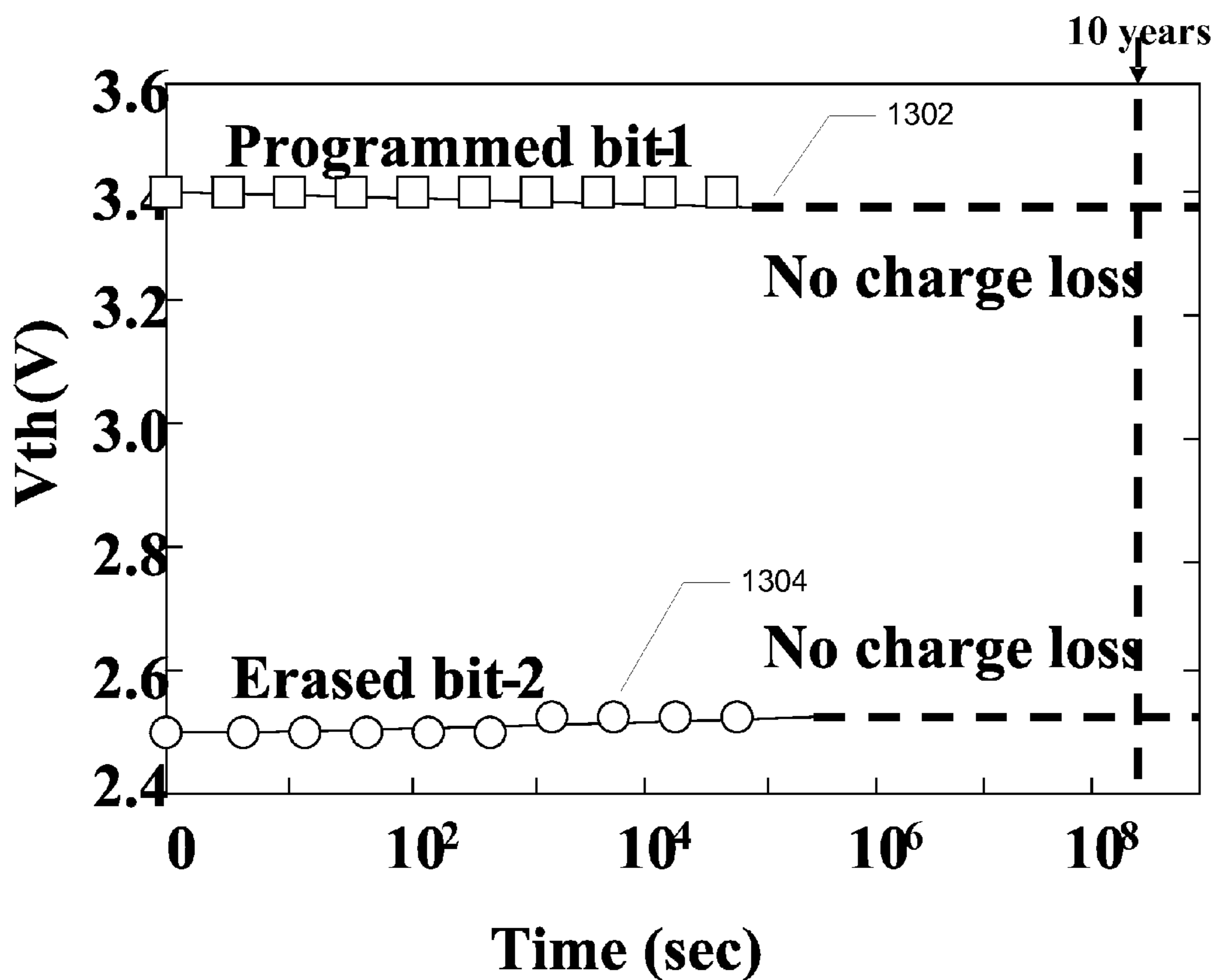
Retention characteristics of Al 2 O 3 storage layer V_g=V_d=V_s=V_b=0V
