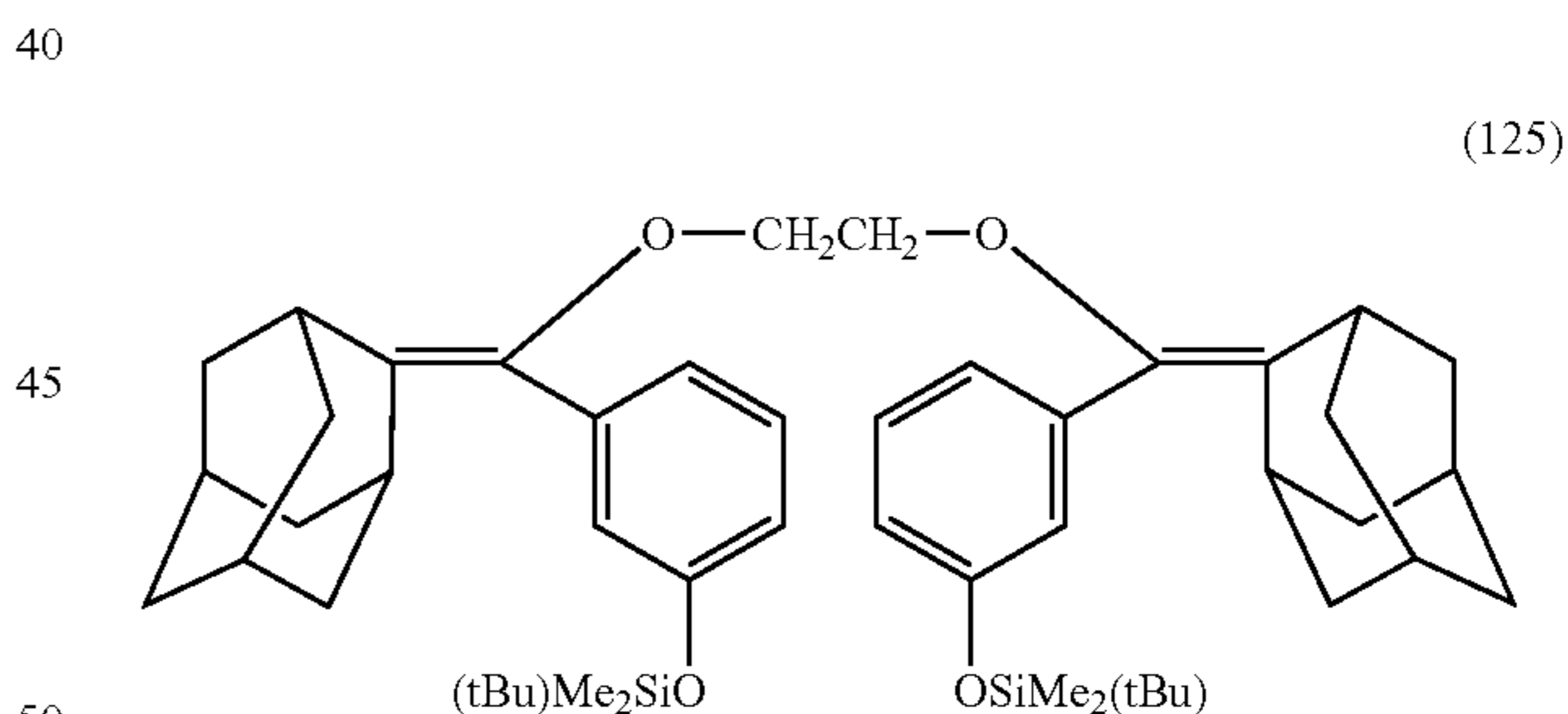
(f). Synthesis of bis[(3-hydroxyphenyl)methylenoxymethylene adamantane]
