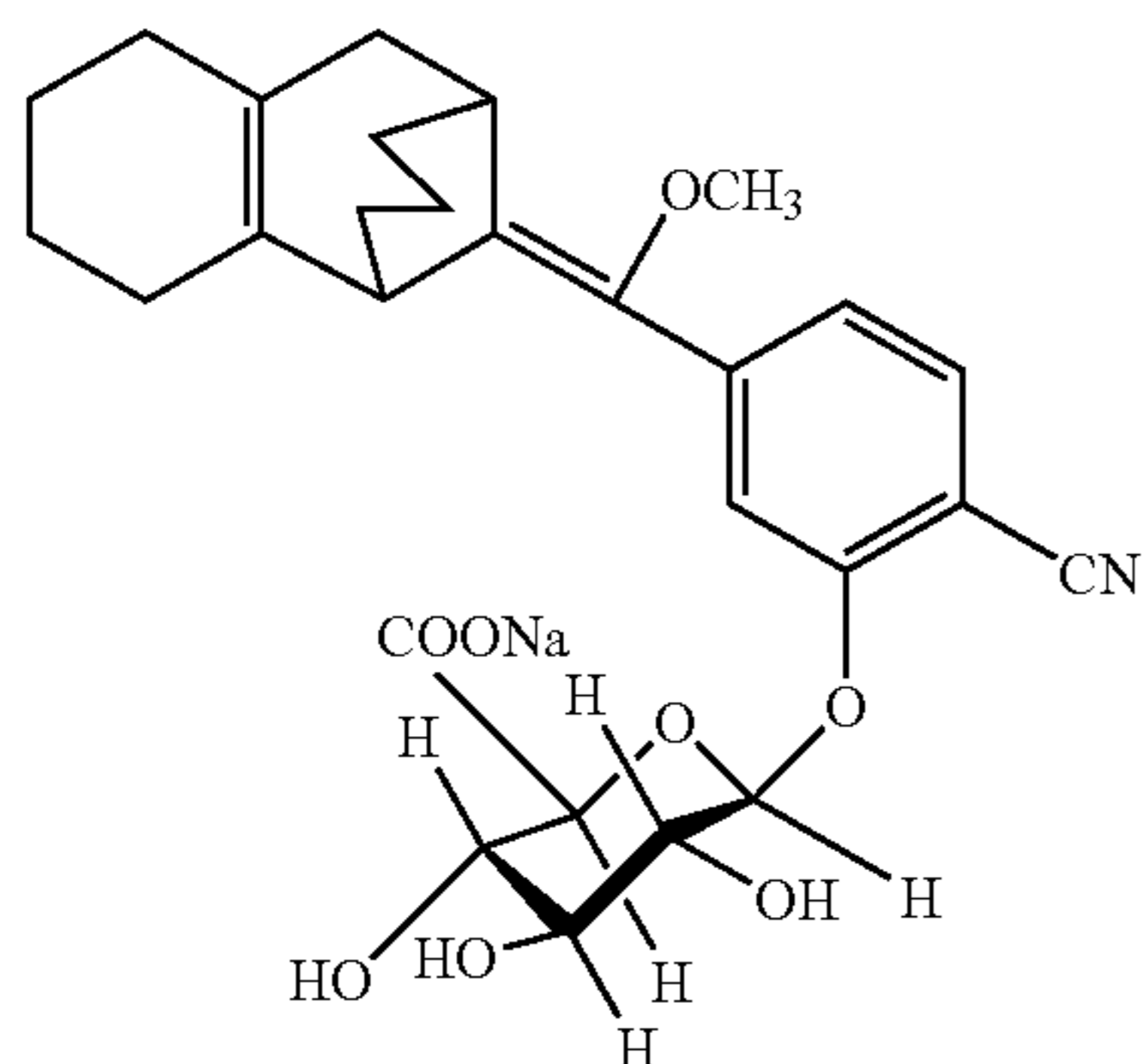
Synthesis of Sodium [(4-methoxy-4(3- \beta -D-glucoronic Acid-4-cyanophenyl)]spiro[1,2-dioxetane-3-1,3-tricyclo[7.3.1.0 2,7 ]tridec-2,7-ene
