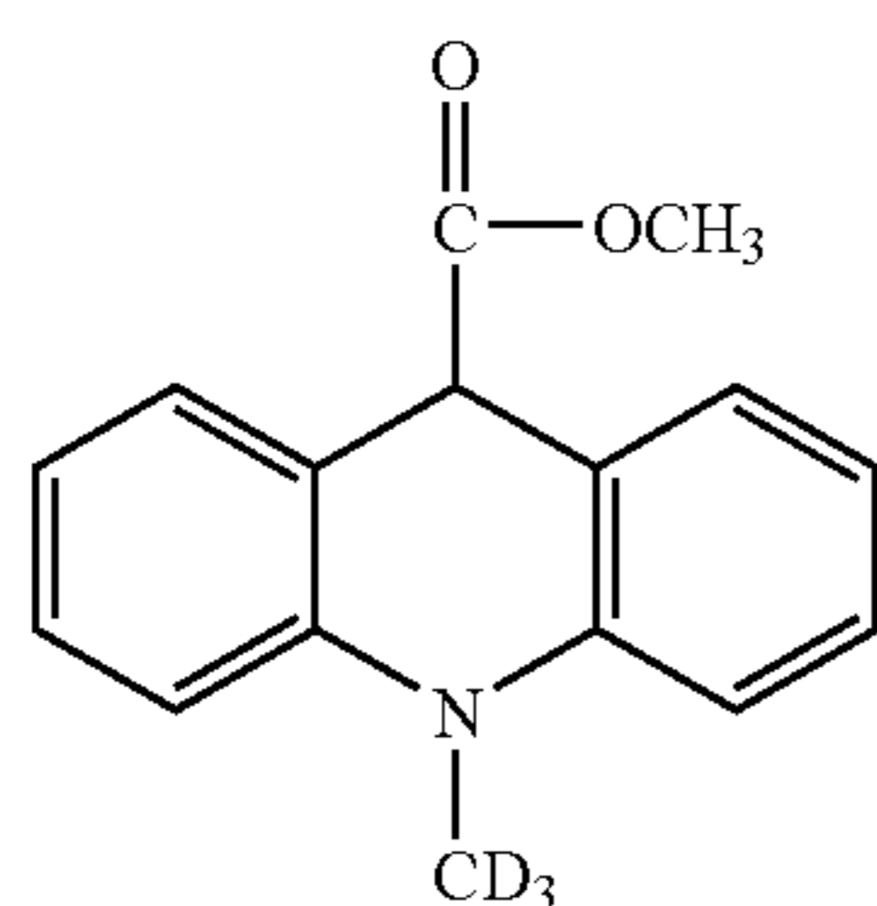
Synthesis of 10-methyl(D 3 )acridan-9-carboxylic Acid (70)
