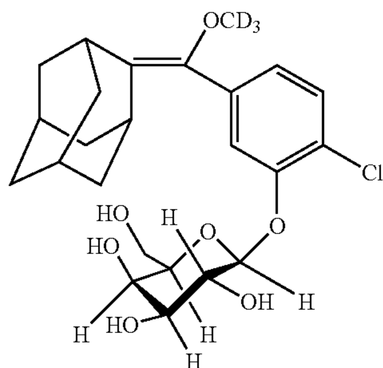
Synthesis of [4-methoxy( \text{D}_3 )-4-(3- \beta -D-galactose-4-chlorophenyl)]spiro[1,2-dioxetane-3,2'-adamantane
