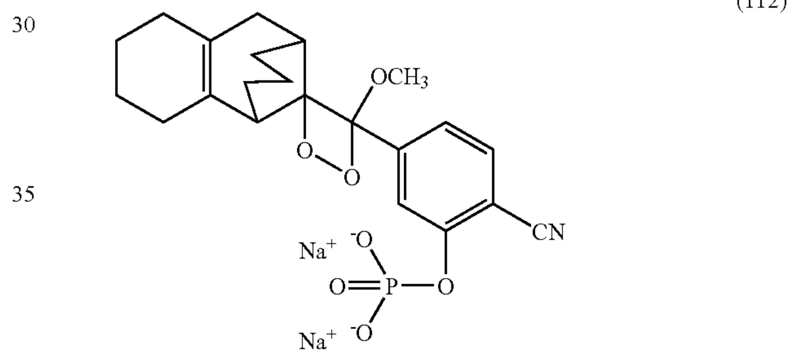
(e). Synthesis of (3-phosphoryloxy-4-cyanophenyl)methoxymethylene[7.3.1.0 2,7 ]tricyclo tridec-2,7-ene, disodium salt
