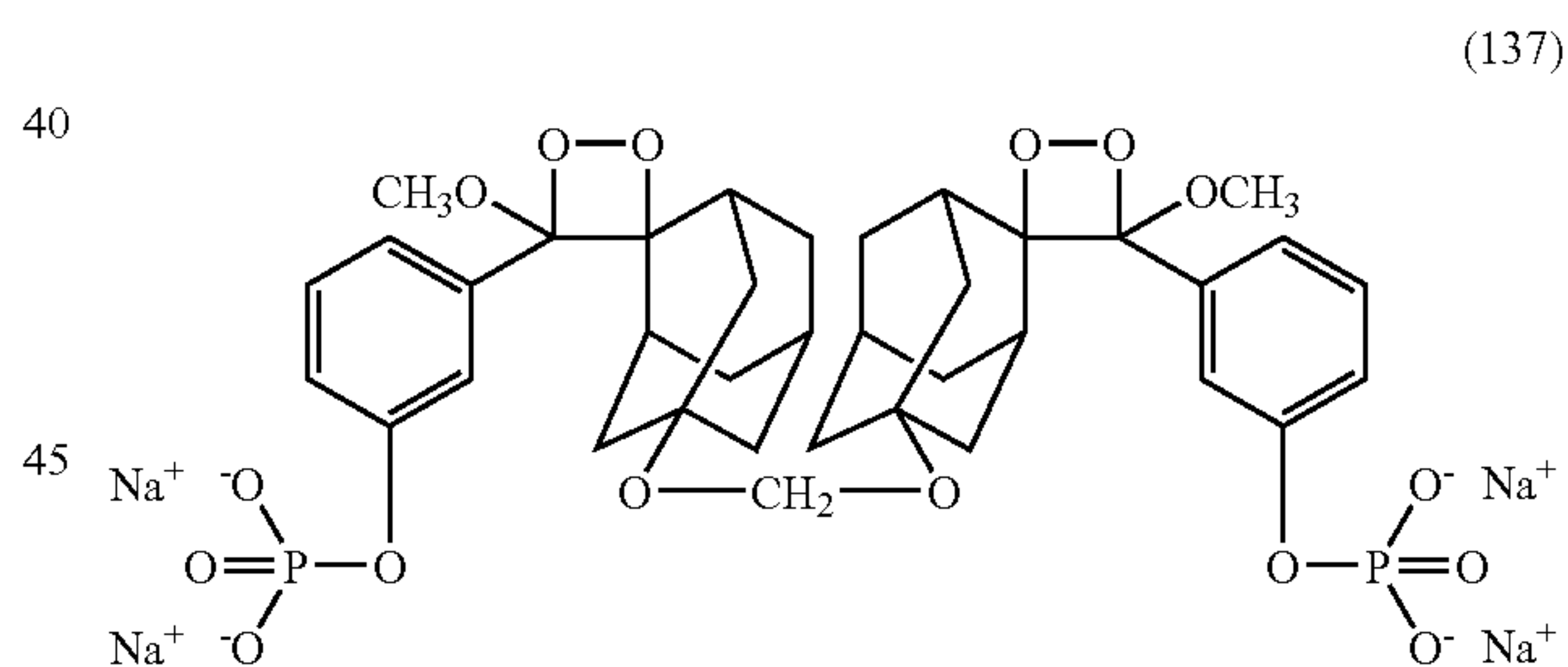
Photooxidation of bis[(3-phosphoryloxy-4-chlorophenyl)methoxy(D3)methylene5-oxy-adamantane, disodium salt]methane
