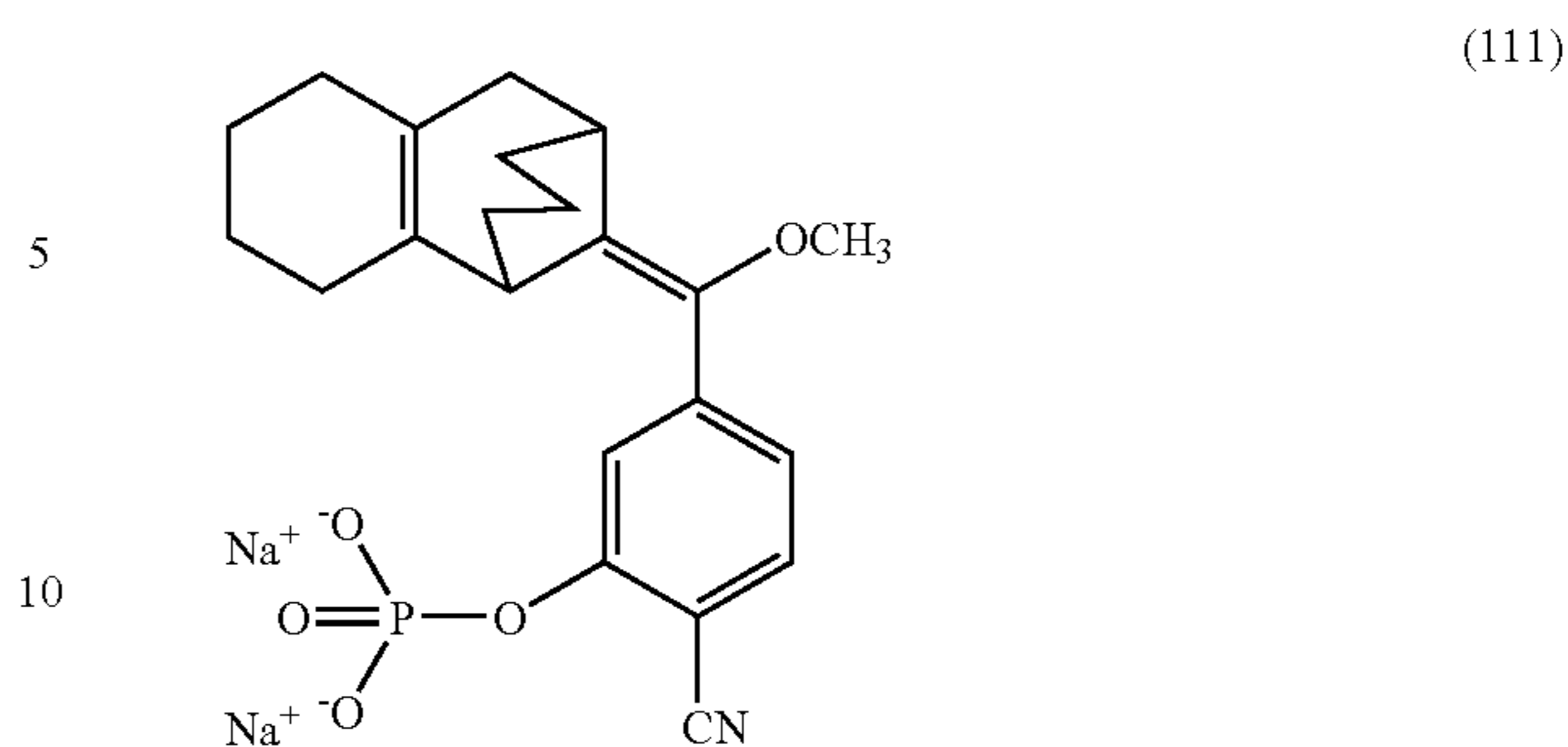
(f). Synthesis of [4-Methoxy-4-(3-phosphoryloxy-4-cyanophenyl)]spiro[1,2 dioxetane-3,13'-tricyclo [7.3.1.0 2,7 ]tridec-2,7-ene, disodium salt (123)
