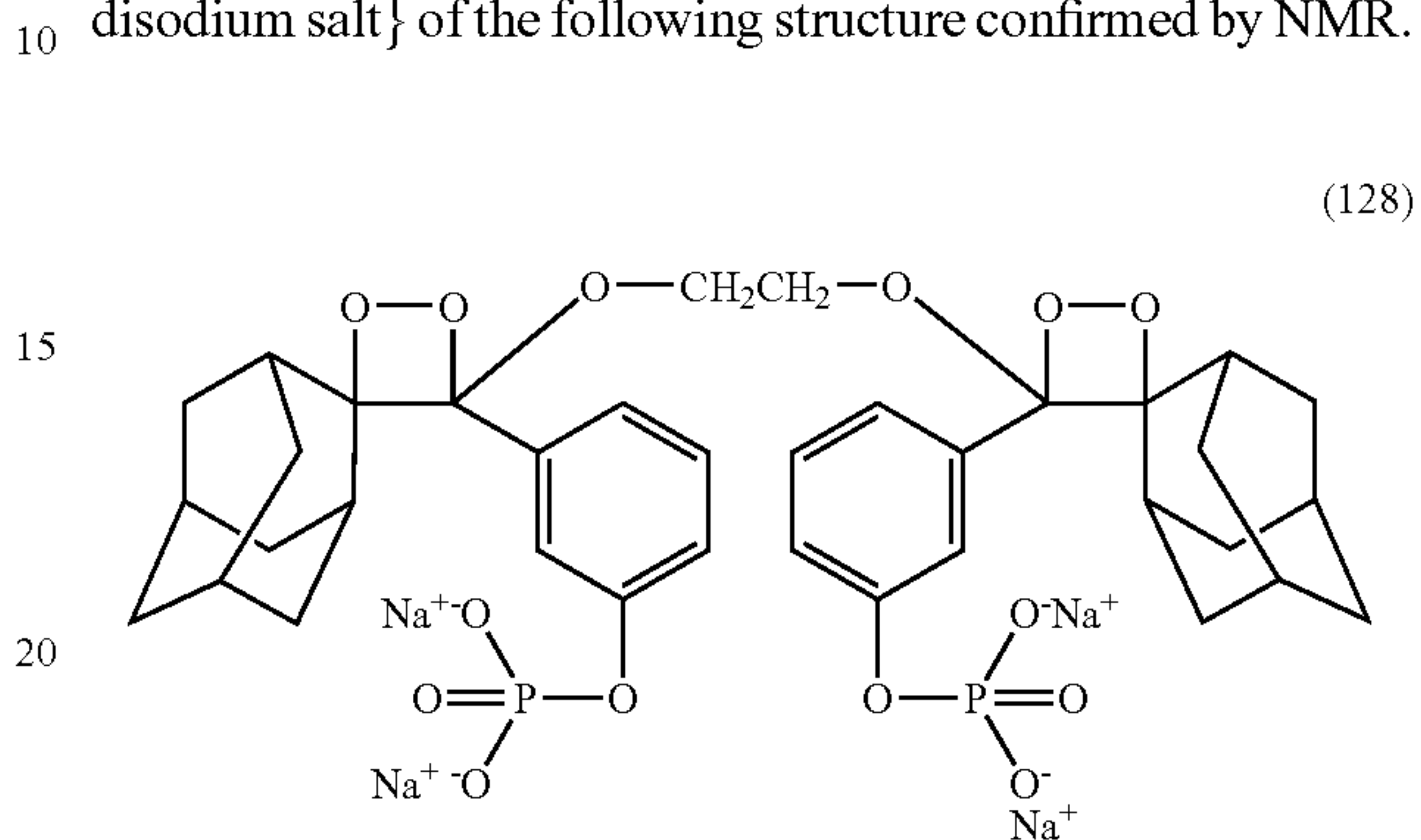
(g). Synthesis of bis[(3-phosphoryloxyphenyl)methylenoxymethylene adamantane, disodium salt]
