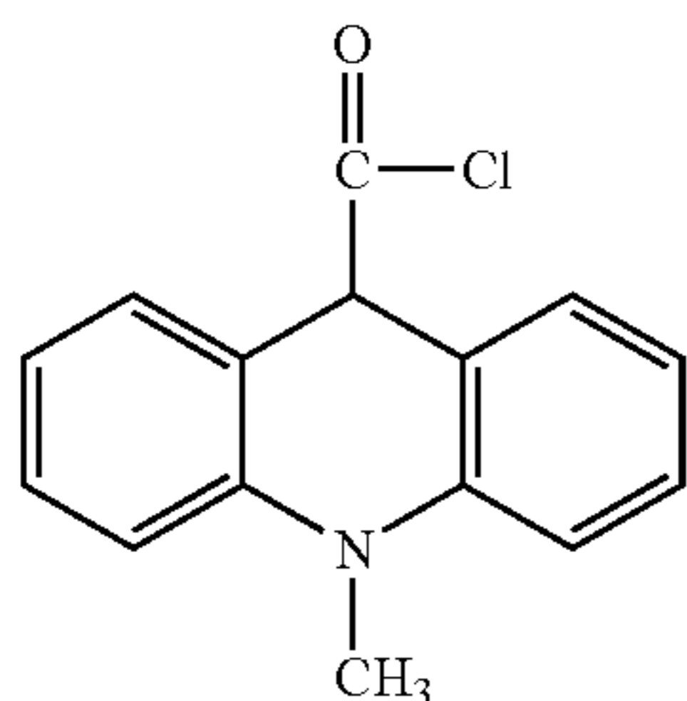
Synthesis of phenyl(D 5 )10-methylacridan-9-carboxylate (79)
