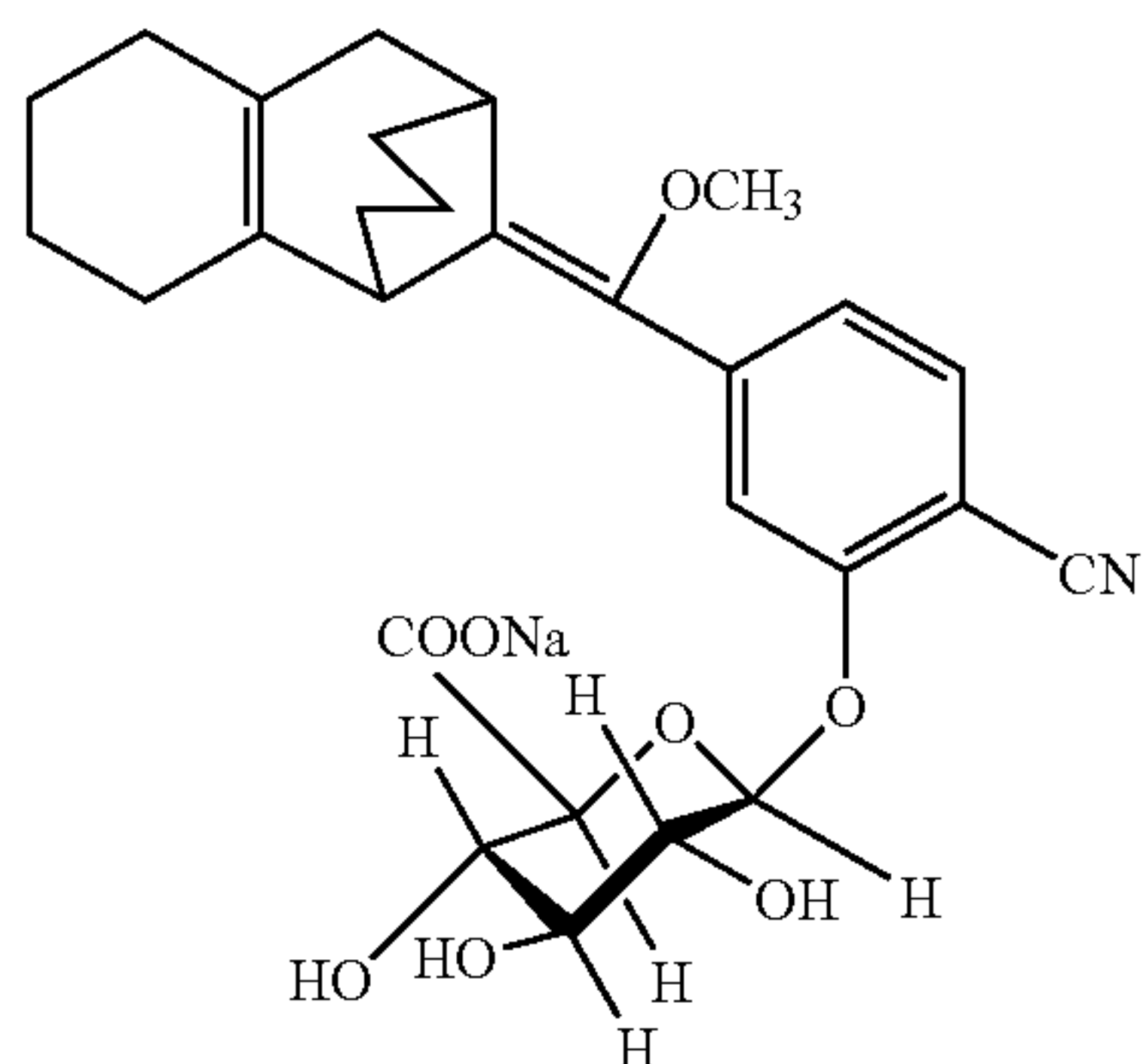
Synthesis of Sodium [(4-methoxy-4(3-β-D-glucoronic Acid-4-cyanophenyl)]spiro[1,2-dioxetane-3-1,3-tricyclo[7.3.1.0 2,7 ]tridec-2,7-ene
