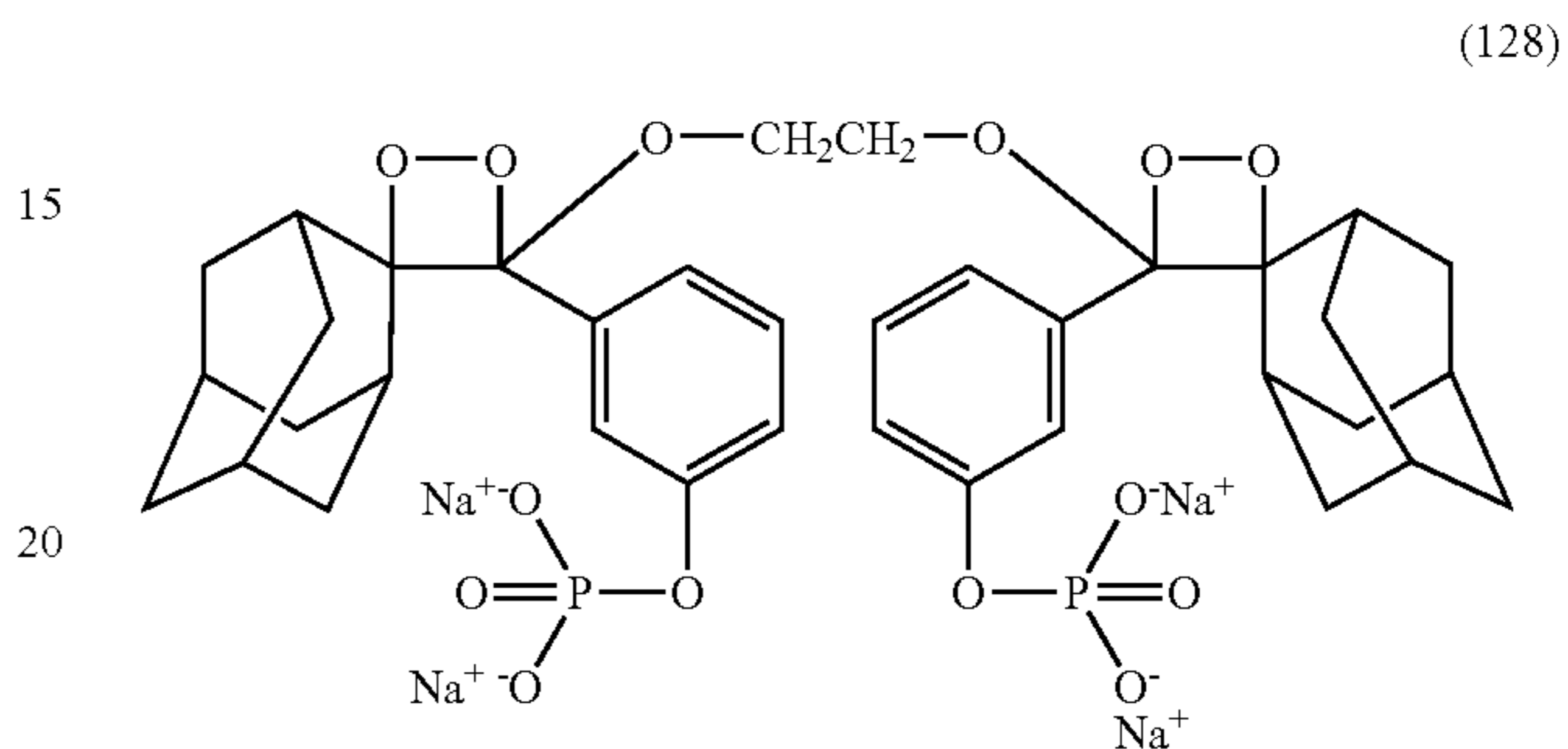
(g). Synthesis of bis[(3-phosphoryloxyphenyl)methylenoxymethylene adamantane, disodium salt]
