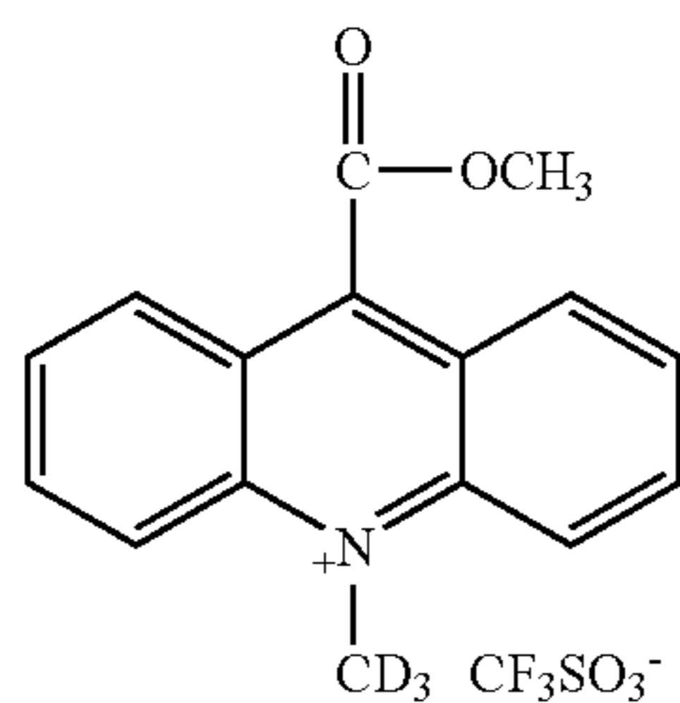
Synthesis of methyl 10-methyl(D 3 )acridan-9-carboxylate (69)
