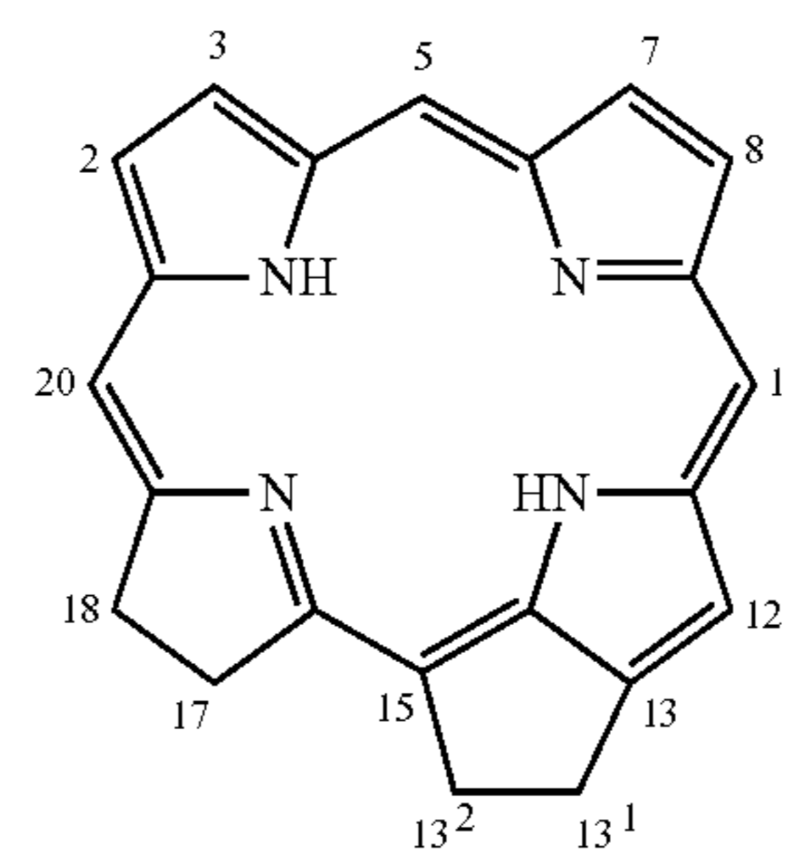
phorbine (with normal "chlorophyll" numbering)
