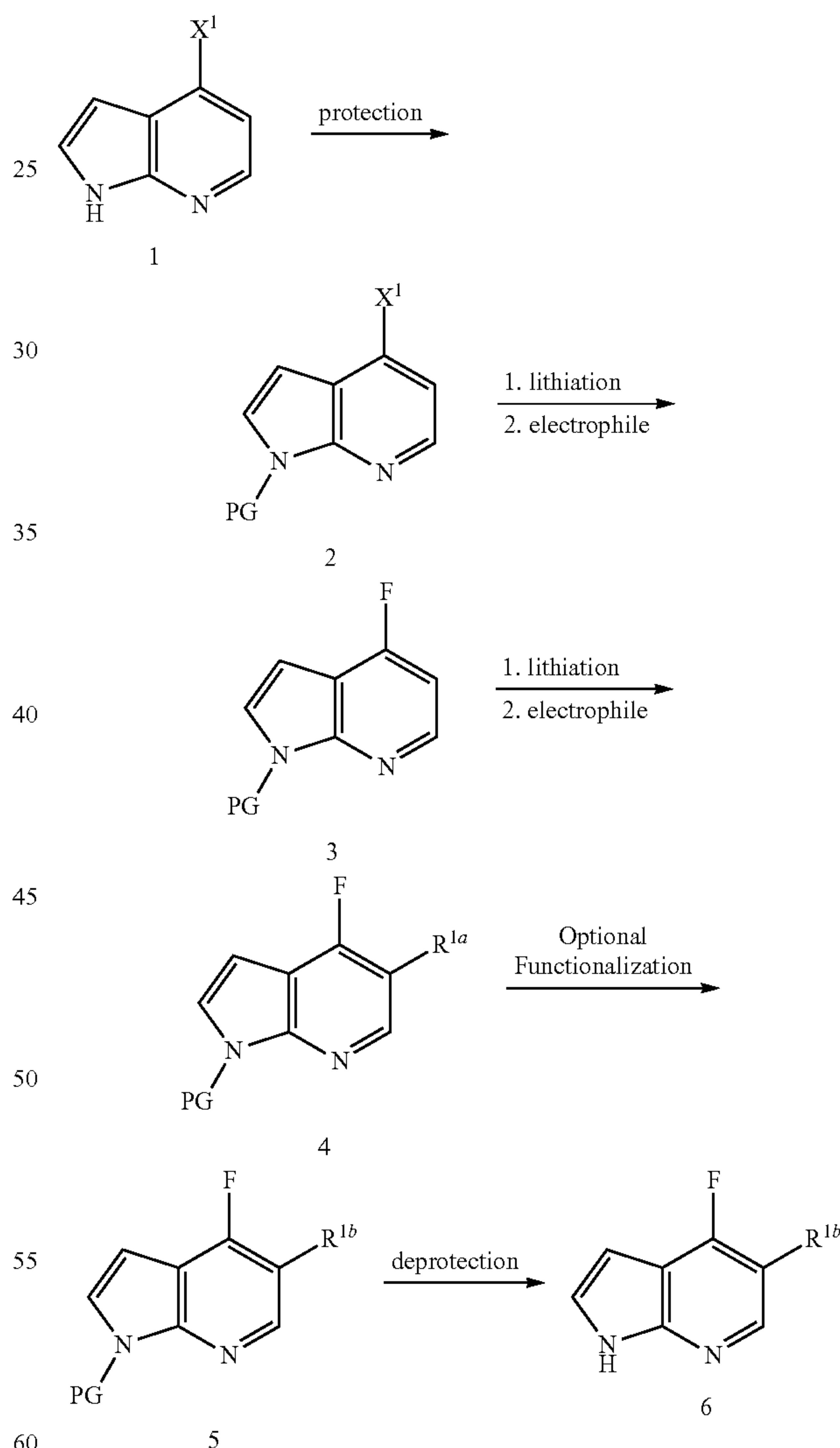
Scheme 1
