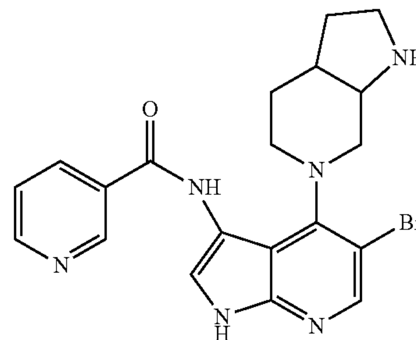
N-(5-Bromo-4-(tetrahydro-1H-pyrrolo[2,3-c]pyridin-6(2H, 7H, 7aH)-yl)-1H-pyrrolo[2,3-b]pyridin-3-yl)nicotinamide
