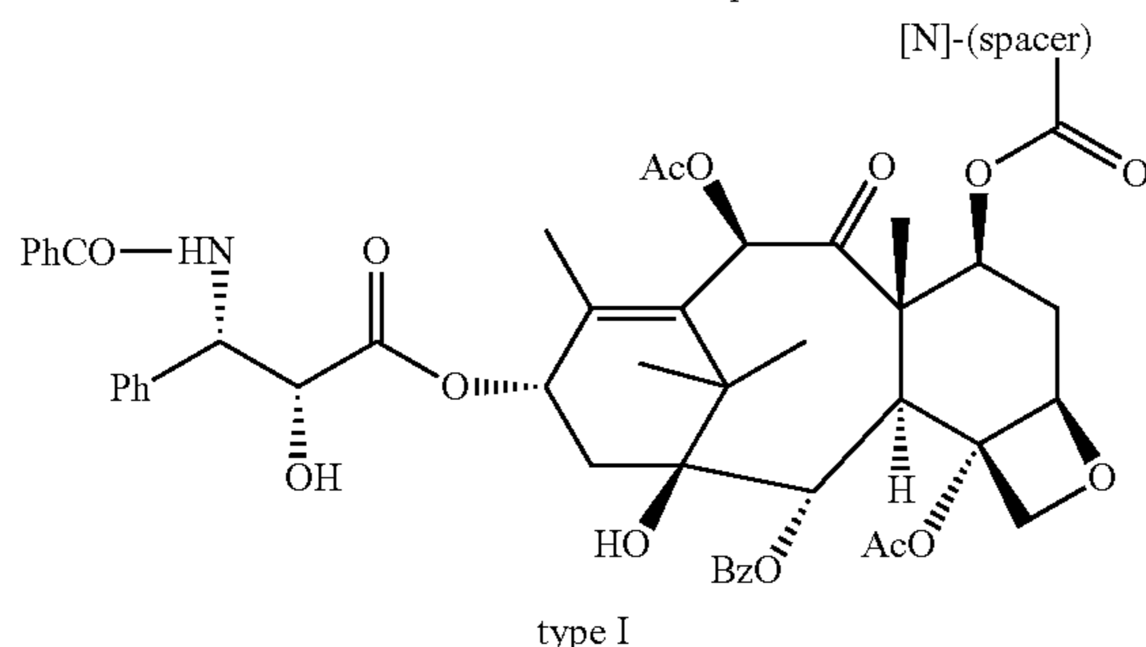
type H monoester derivatives of paclitaxel
