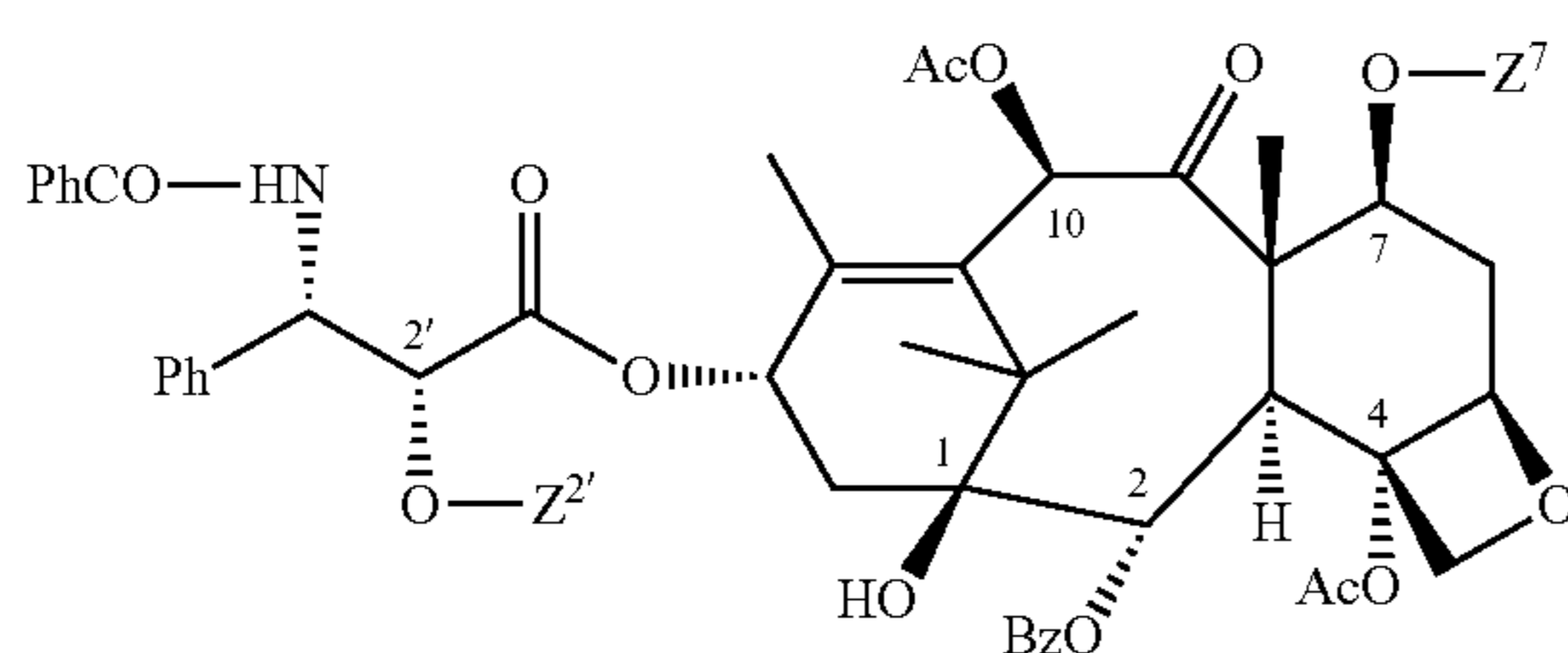
general structure of paclitaxel derivatives
