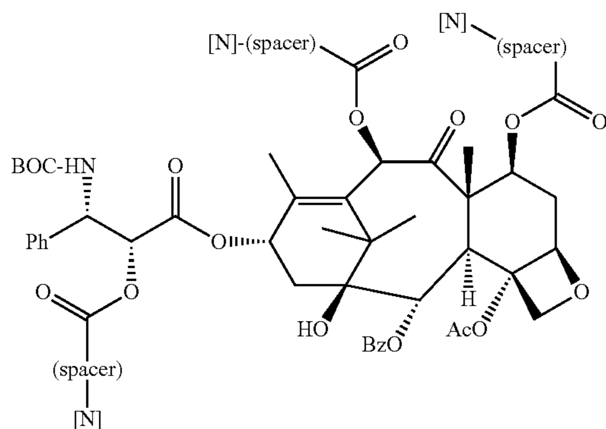
type G triester derivative of docetaxel
