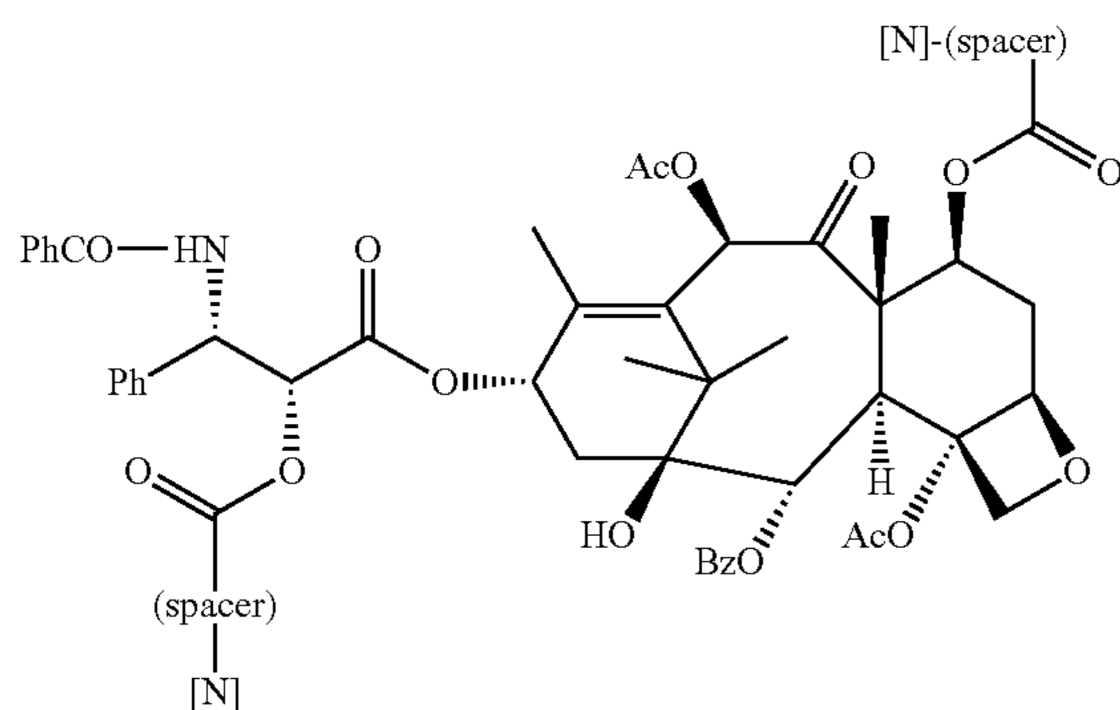
type J diester derivative of paclitaxel
