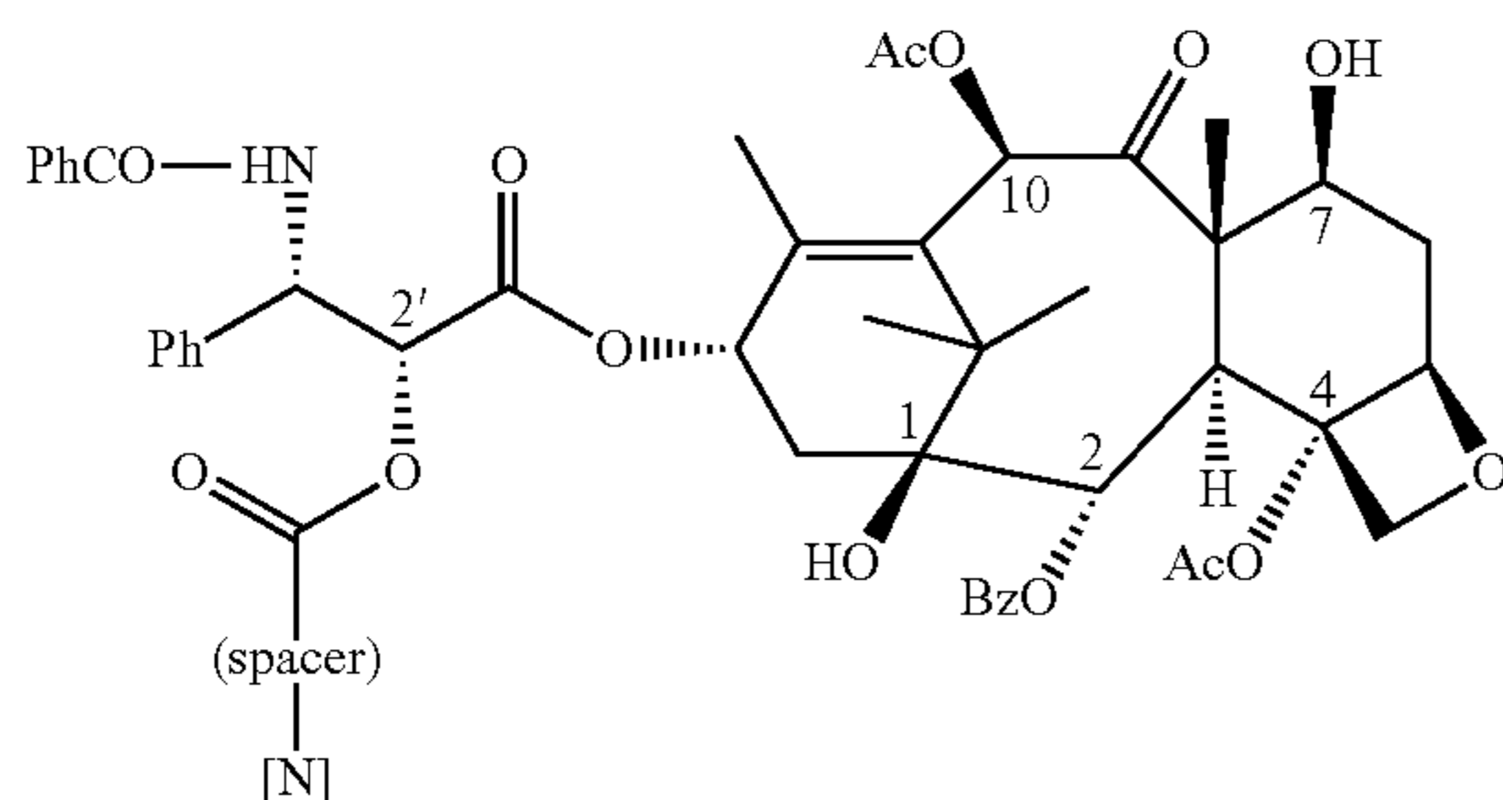
type H monoester derivatives of paclitaxel
