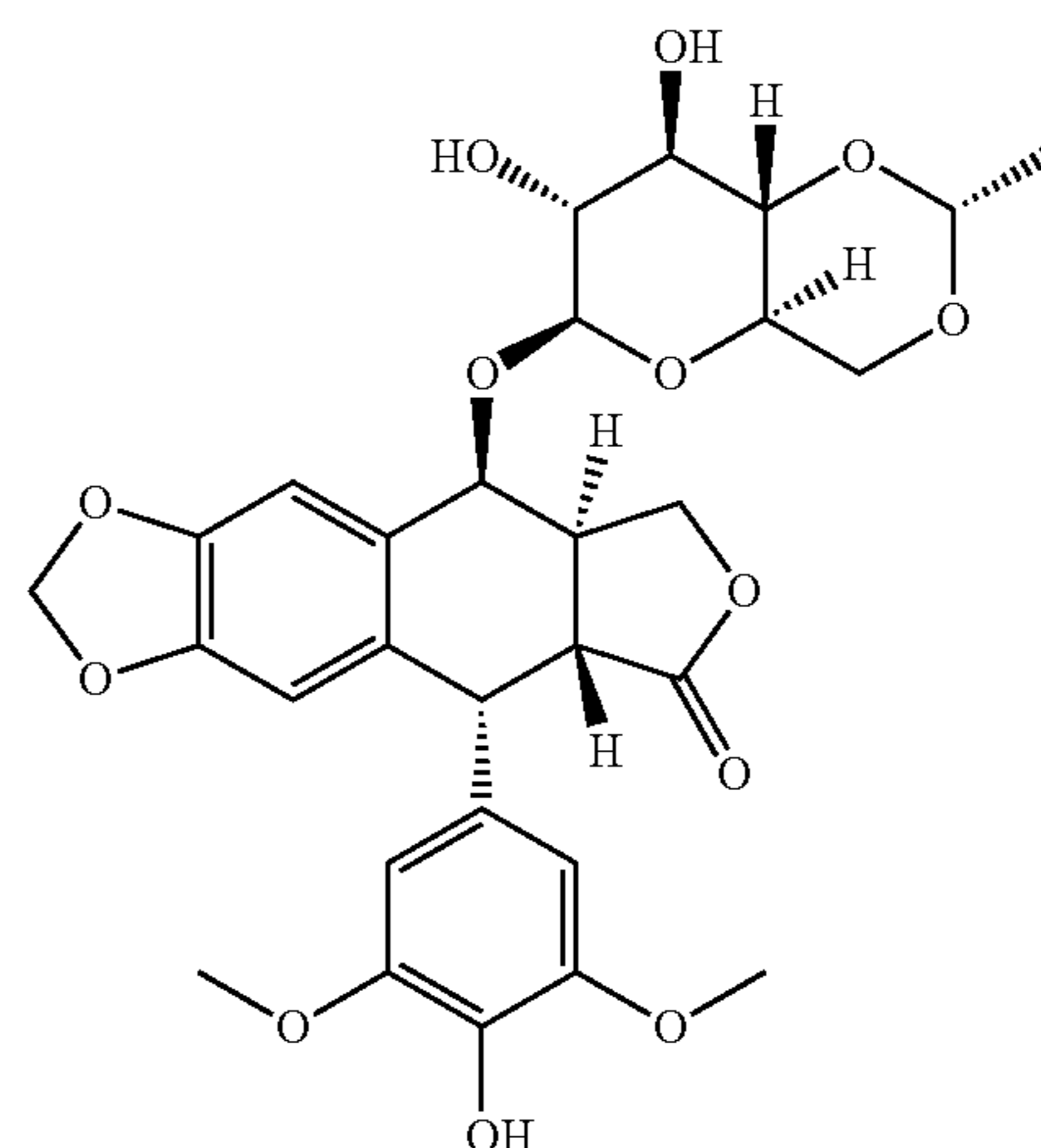
Etoposide 6
