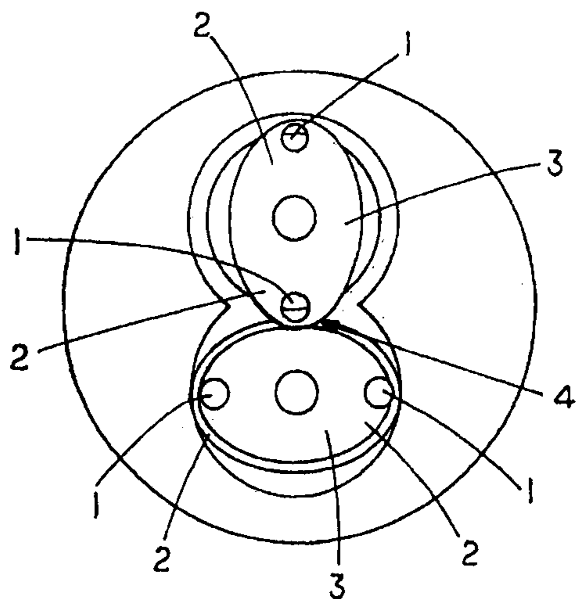
FIG. 1 (PRIOR ART)
