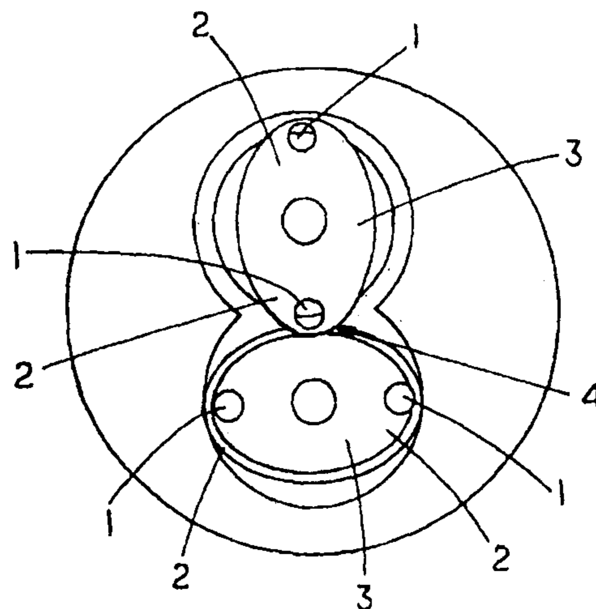
FIG. 1 (PRIOR ART)
