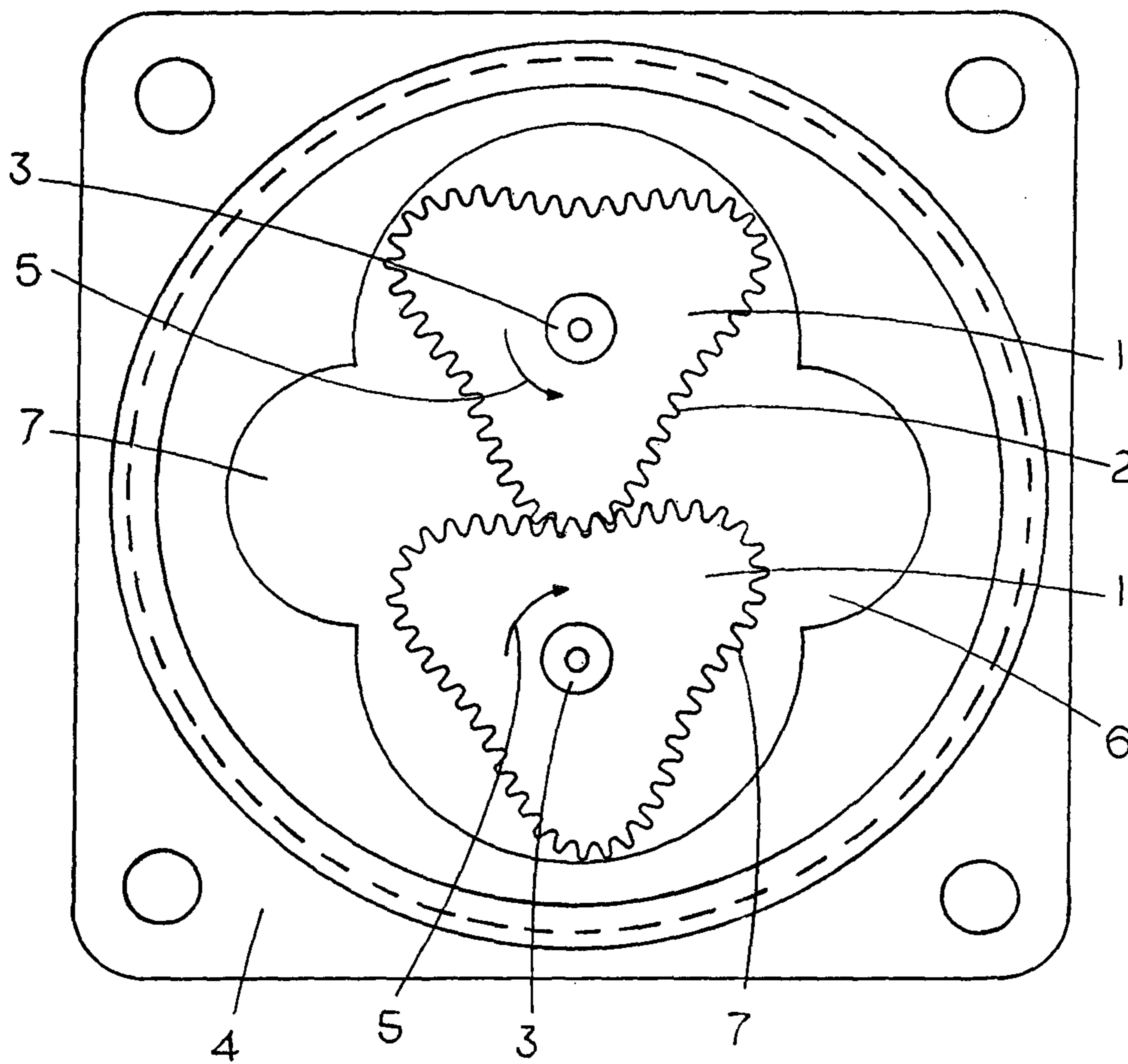
FIG. 1 (PRIOR ART)
