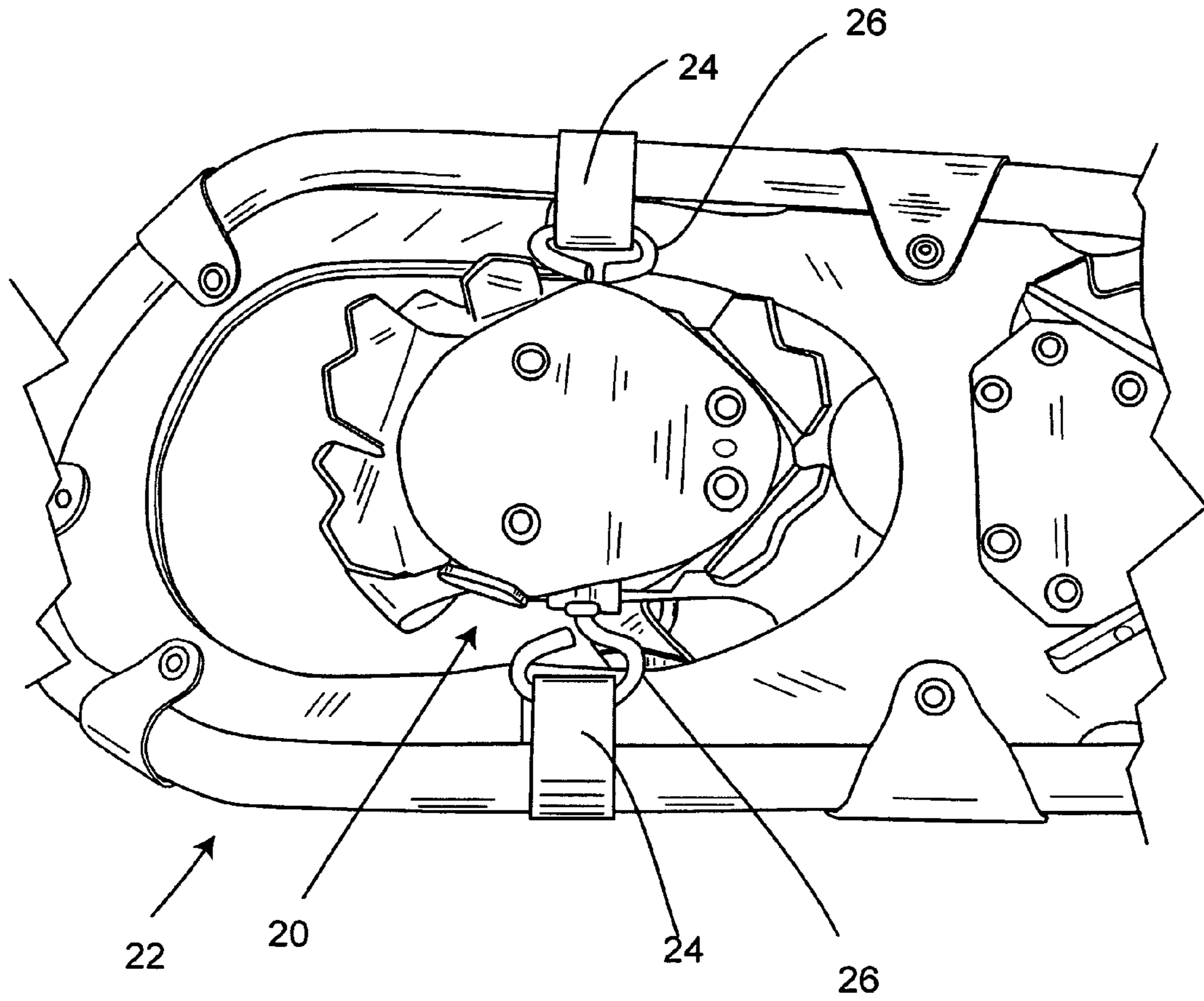
FIG. 2 PRIOR ART
