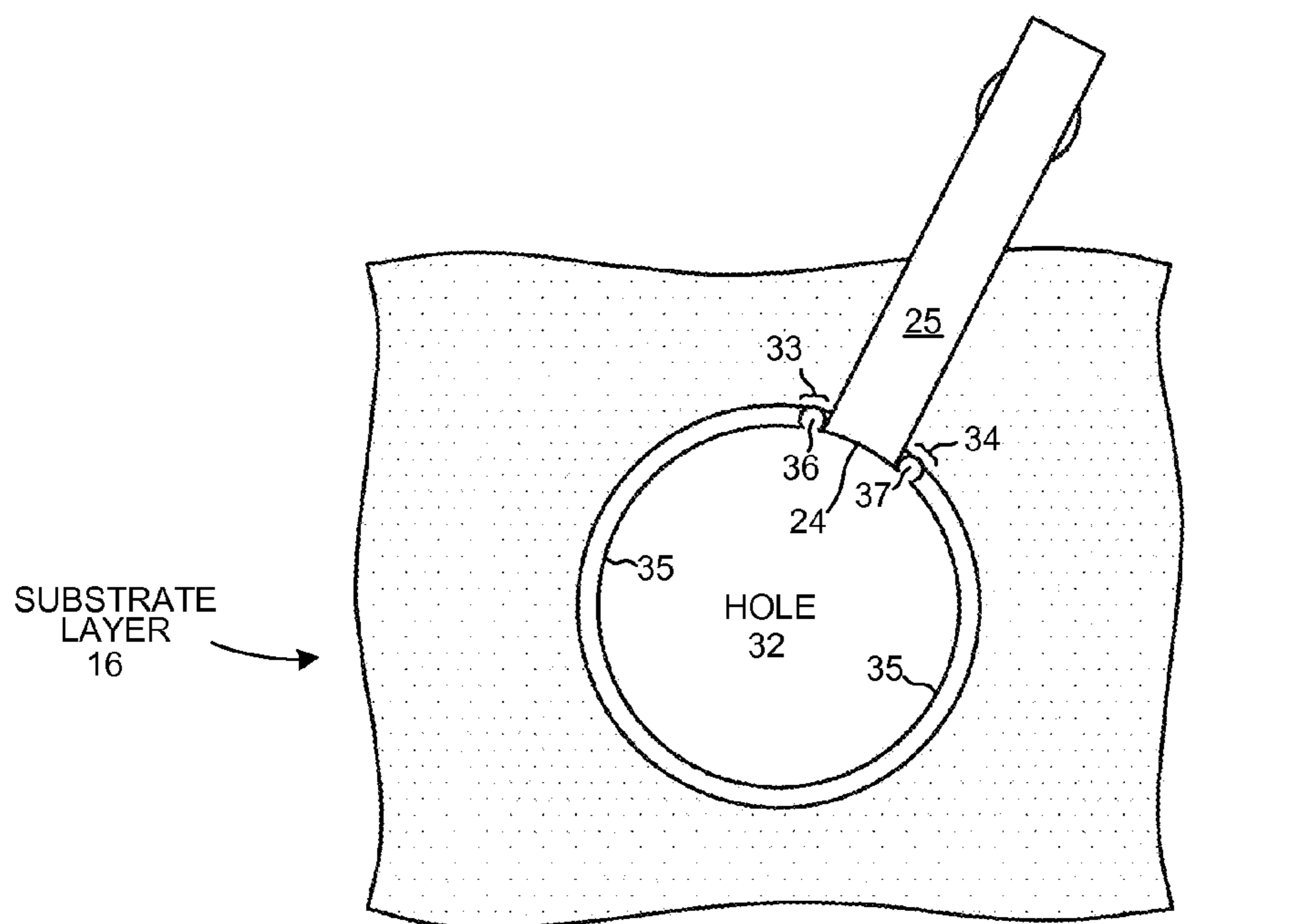
TSV HAVING A STRIP-SHAPED SIGNAL CONDUCTOR (TOP-DOWN VIEW)
