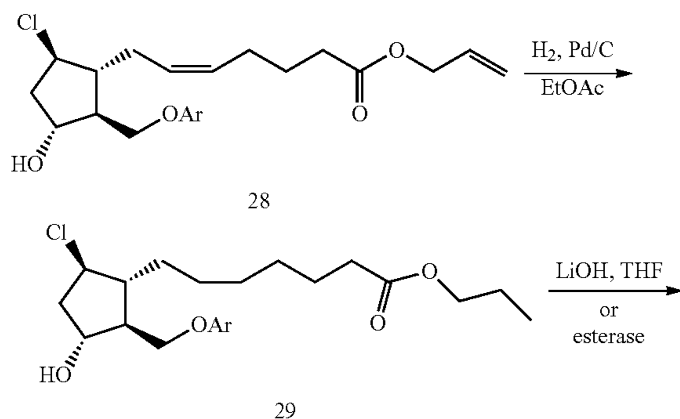
Scheme 6
