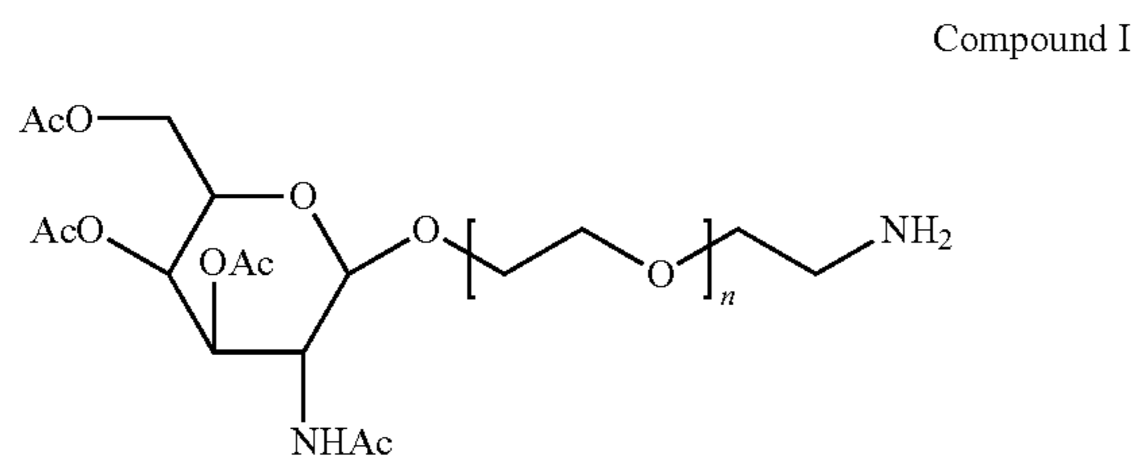
(Aminoethoxy)ethyl derivatives of 2-acetamido-3,4,6-tri-O-acetyl-2-deoxy- \beta -D-galactopyranoside
