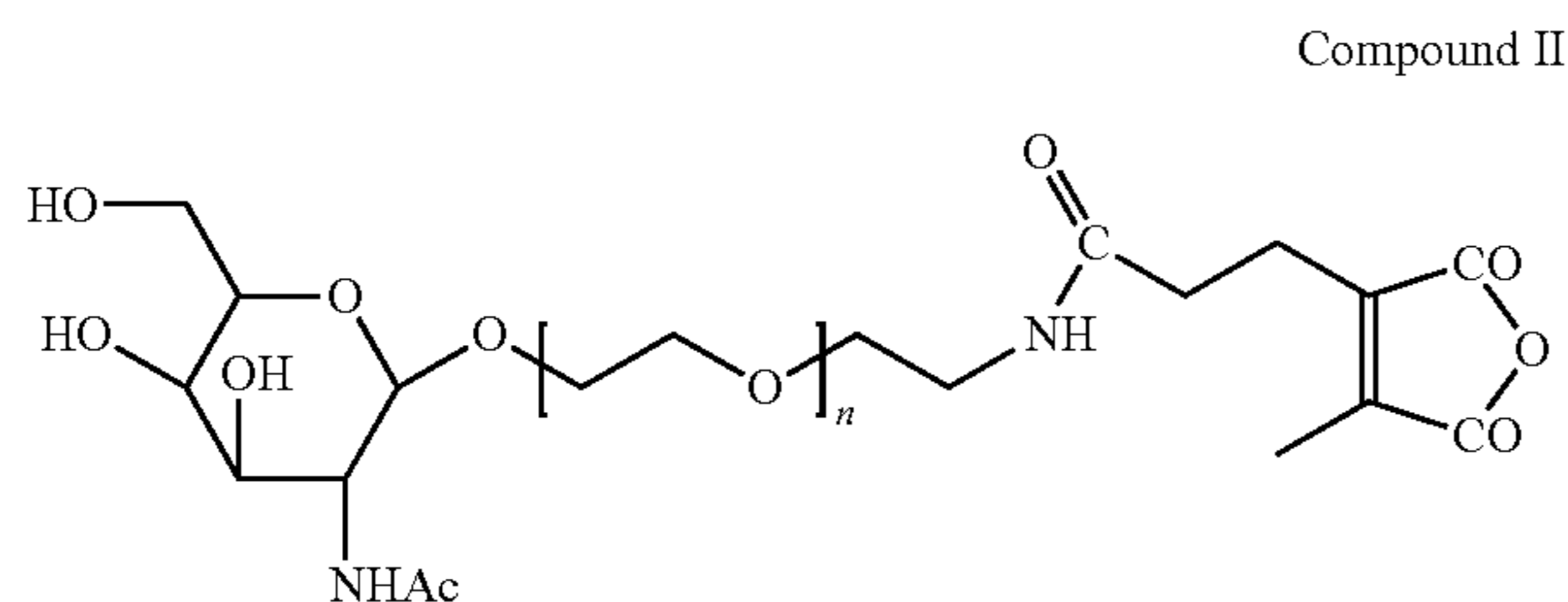
N-Acetyl-galactosamine-PEG-methyl maleic anhydride
