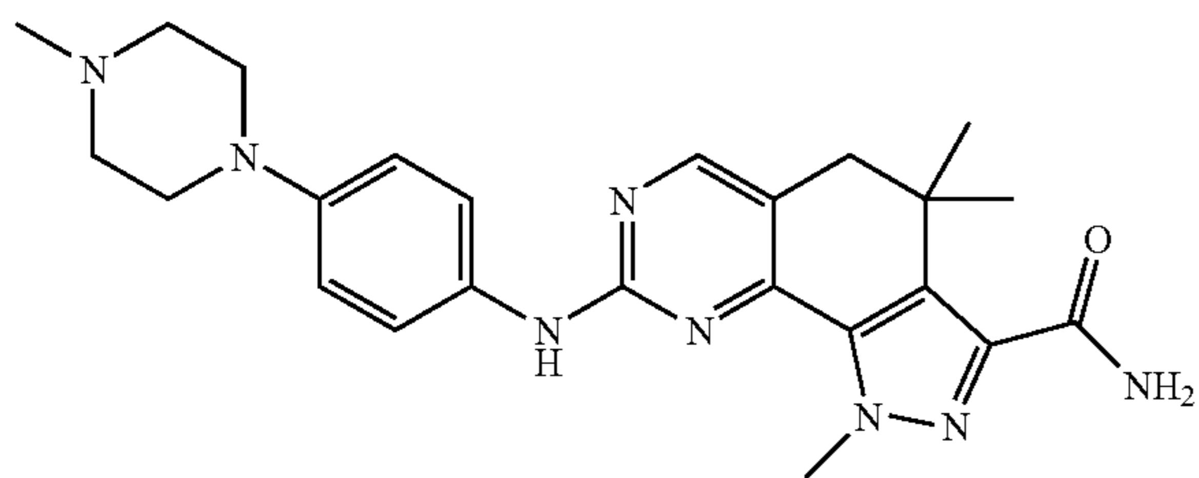
8-[4-(4-methyl-piperazin-1-yl)-phenylamino]-1,4,4-trimethyl-4,5-dihydro-1H-pyrazolo[4,3-h]quinazoline-3-carboxamide [B10-X00-M03(C01)-D03]
