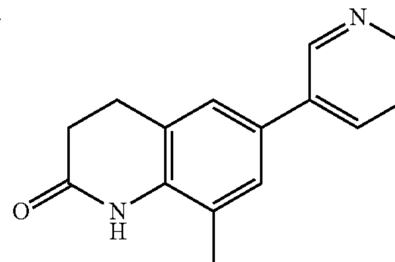
8-Methyl-6-pyridin-3-yl-3,4-dihydroquinolin-2(1H)-one
