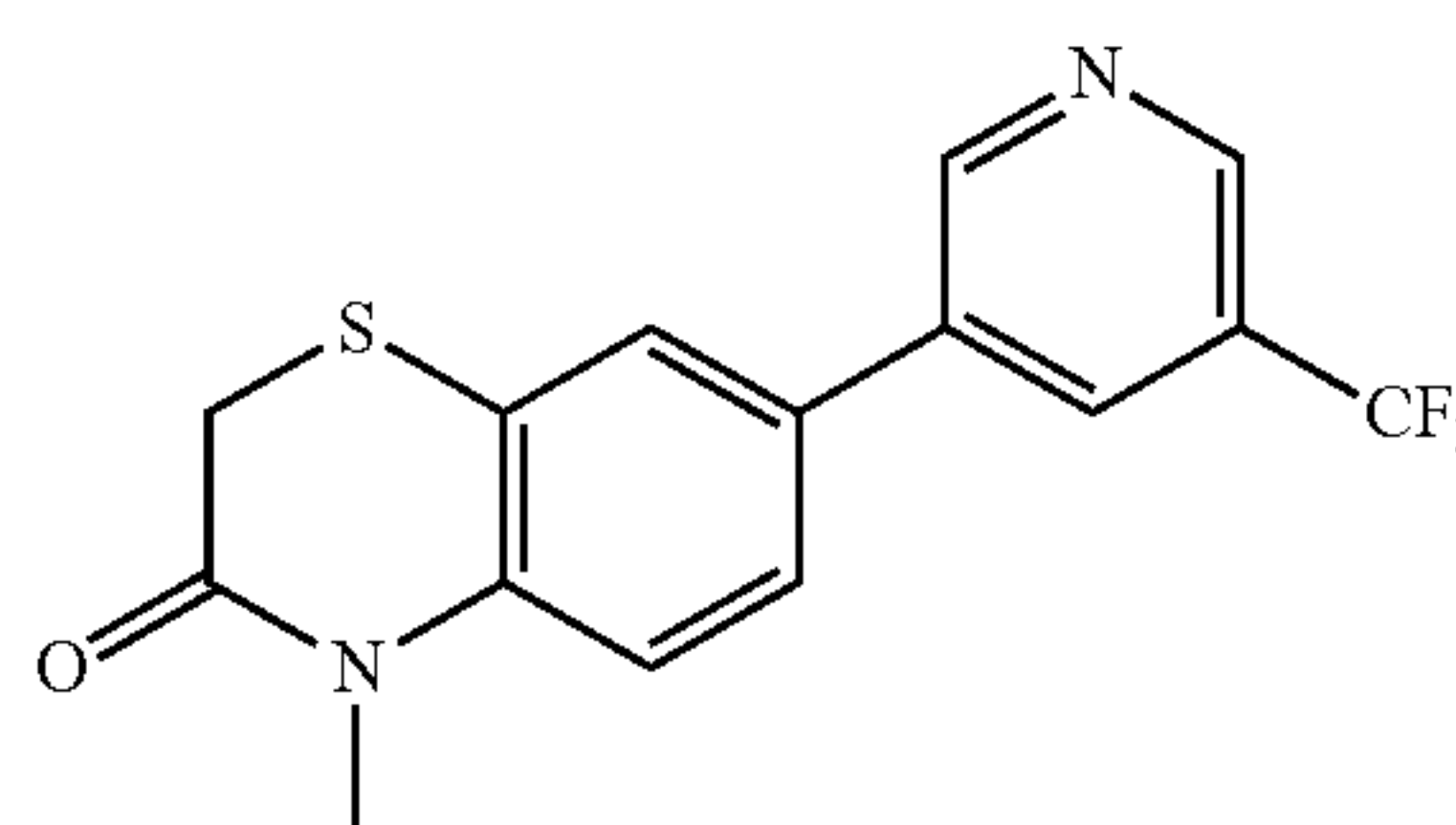
4-Methyl-7-(5-(trifluoromethyl)pyridin-3-yl)-2H-benzo[b][1,4]thiazin-3(4H)-one
