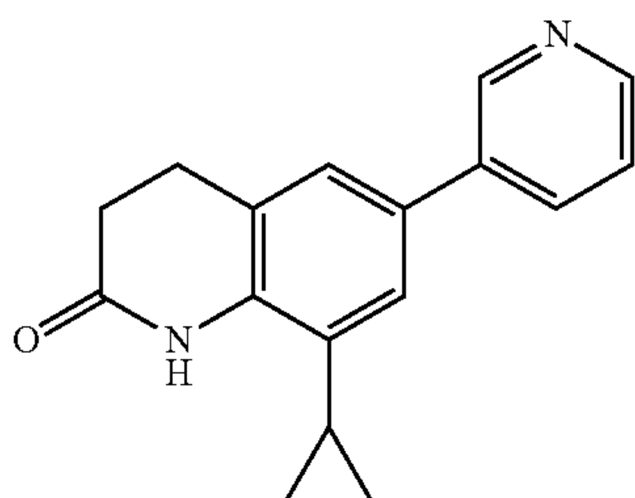
8-Cyclopropyl-6-(pyridin- 3-yl)-3,4-dihydroquinolin- 2(1H)-one
