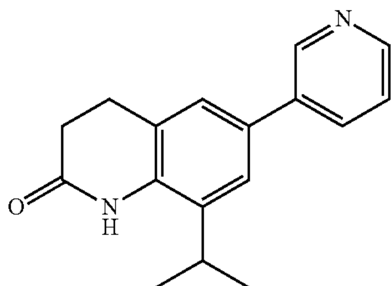
8-Isopropyl-6-(pyridin-3-yl)- 3,4-dihydroquinolin- 2(1H)-one
