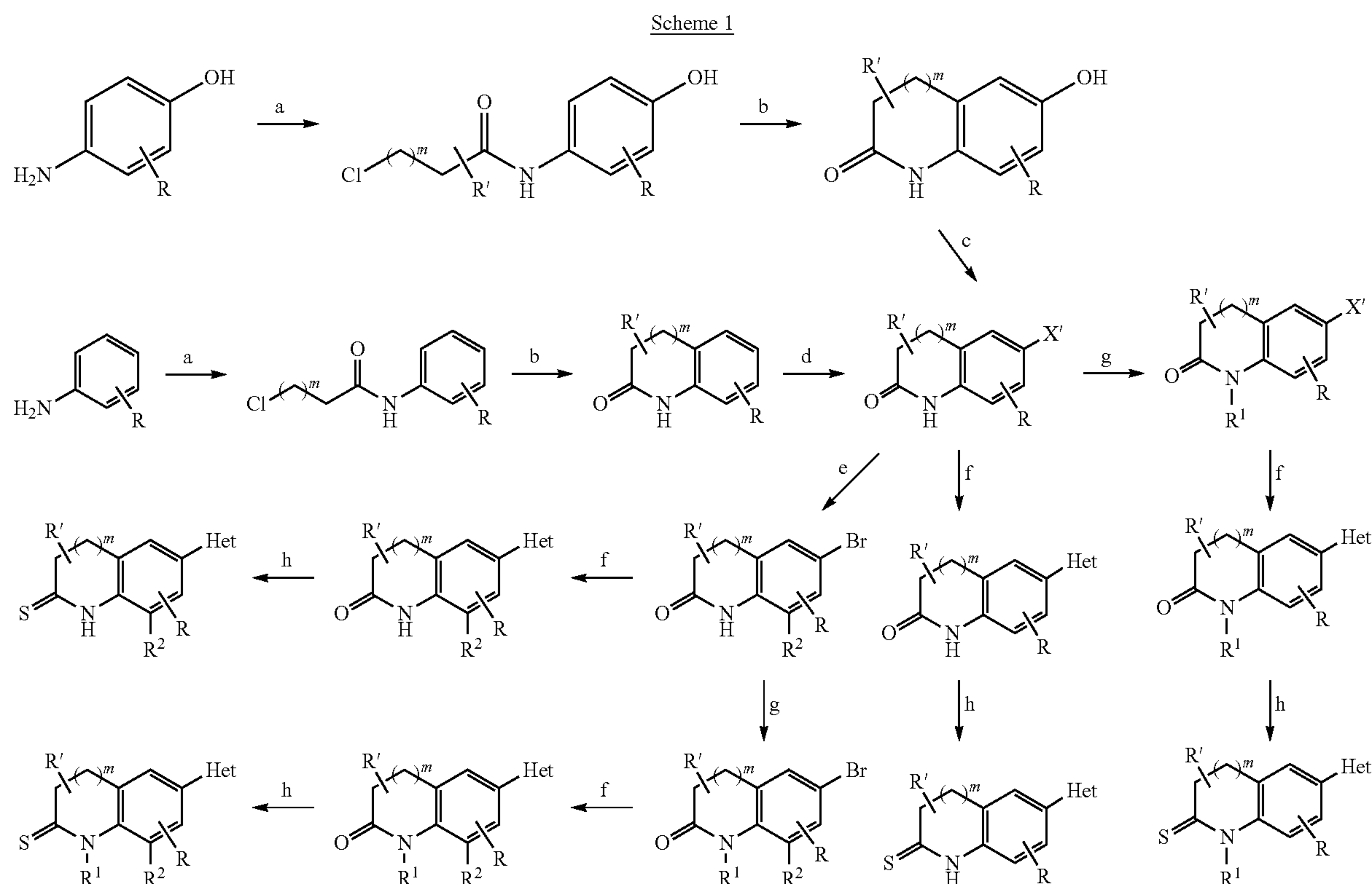
Scheme 1: a) \omega -Chlorocarboxylic acid chloride, acetone, 60° C.; b) \text{AlCl}_3 , NaCl, 150° C.; c) \text{Ti}_2\text{O} , \text{CH}_2\text{Cl}_2 , pyridine, 0° C., or: \text{Ti}_2\text{NPh} , \text{K}_2\text{CO}_3 , THF, \mu\text{w} , 120° C. (when \text{X}' is OTf); d) NBS, DMF, 0° C. (when \text{X}' is Br); e) \text{R}^2 insertable as electrophile, eg. N-chlorosuccinimide, DMF, 65° C. (when \text{R}^2 is Cl) or: \text{HNO}_3/\text{H}_2\text{SO}_4 (when \text{R}^2 is \text{NO}_2 ); f) Het-B(OR ^n ) _2 , Pd(PPh _3 ) _4 , Na _2 CO _3 , toluene/ethanol/water, 100° C., or: Pd(PPh _3 ) _4 , NaHCO _3 , DMF/water, \mu\text{w} , 150° C.; g) R ^1 -Br or R ^1 -I (wherein R ^1 is alkyl), DMF or THF, base (eg. K _2 CO _3 or NaH), RT to 65° C.; h) Lawesson's reagent, toluene, 120° C. (m is 0, 1, or 2).
