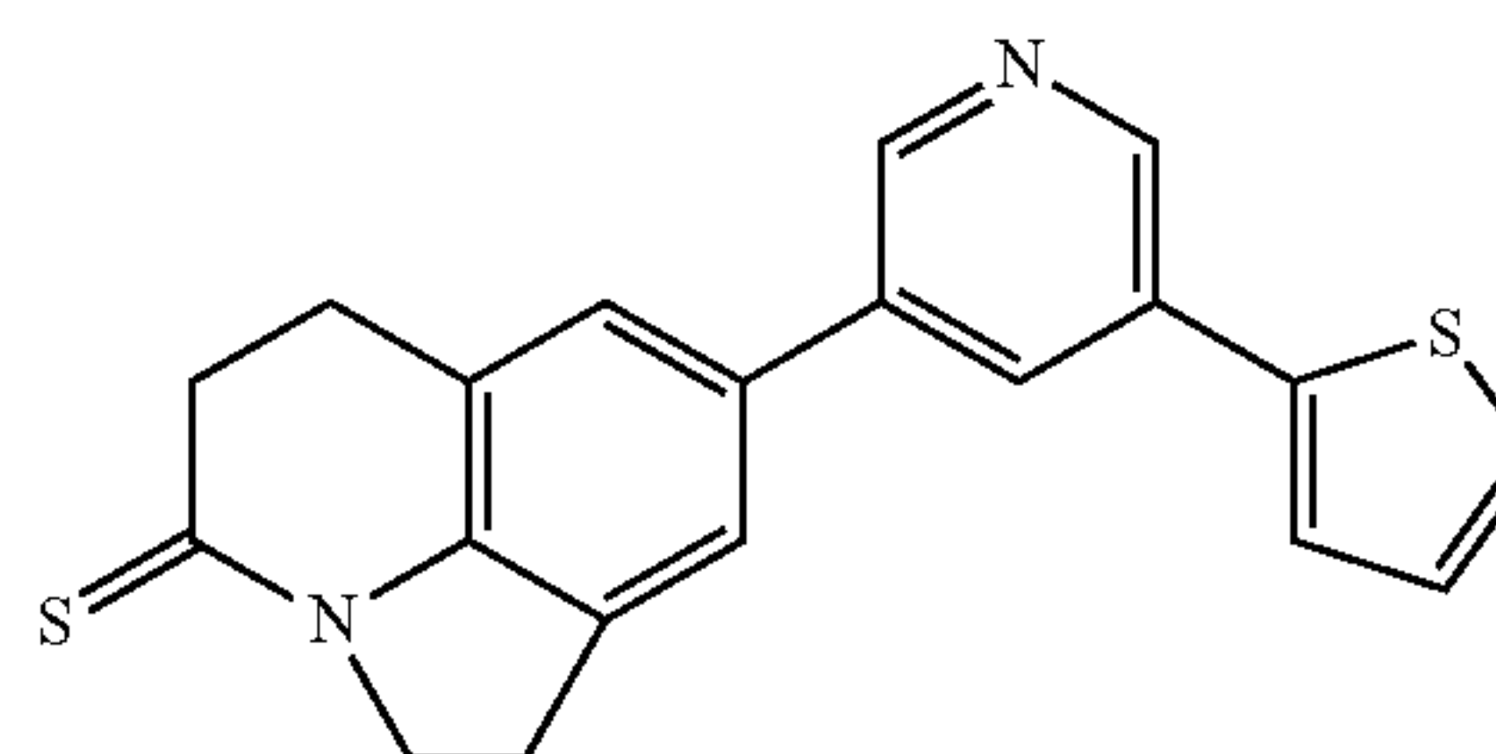
8-[5-(2-thiophen-2-yl)pyridin-3-yl]-1,2,5,6-tetrahydro-4H-pyrrolo[3,2,1-ij]quinolin-4-thione
