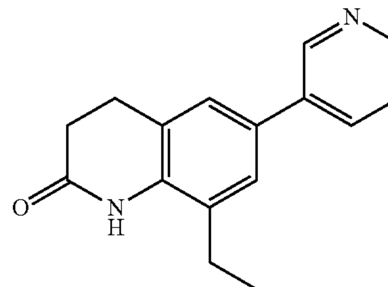
8-Ethyl-6-(pyridin-3-yl)-3,4-dihydroquinolin-2(1H)-one
