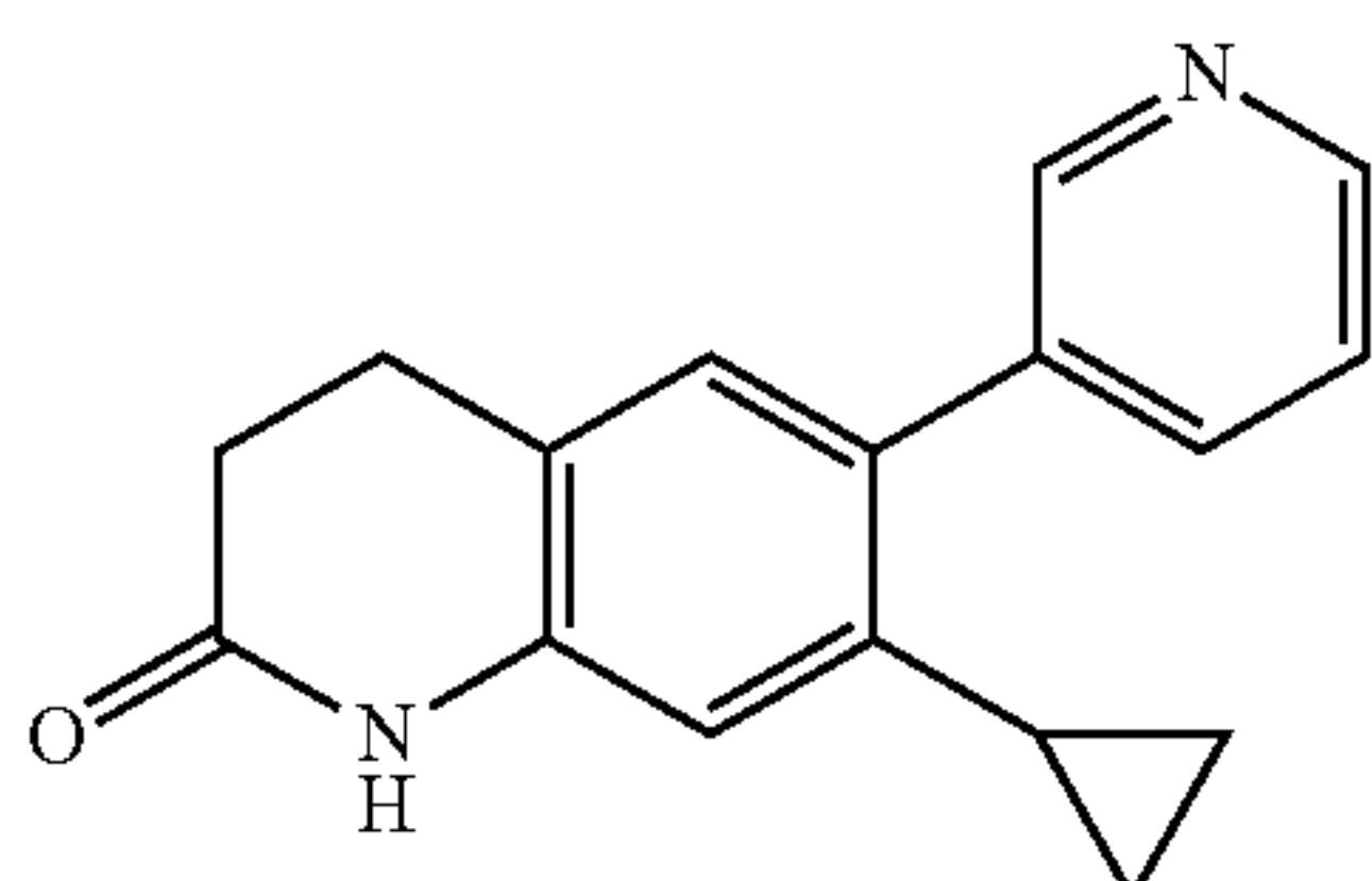
7-Cyclopropyl-6-(pyridin- 3-yl)-3,4-dihydroquinolin- 2(1H)-one
