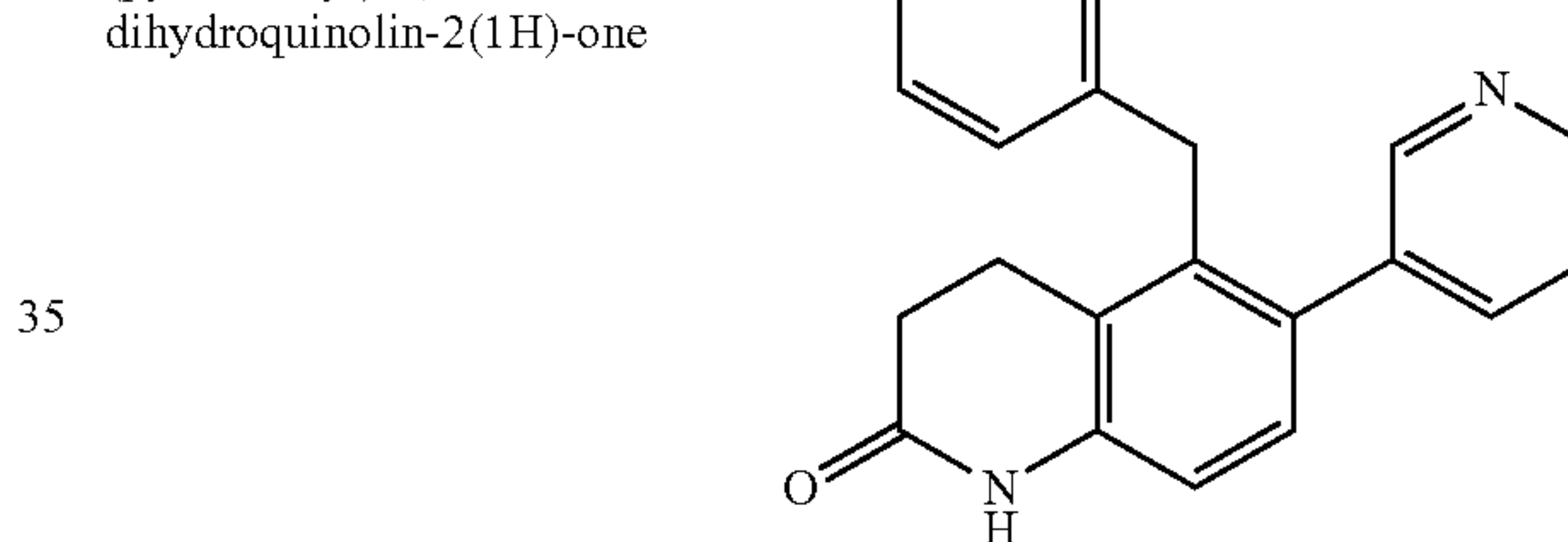
7-(4-Methoxybenzyl)-6- (pyridin-3-yl)-3,4- dihydroquinolin-2(1H)-one
