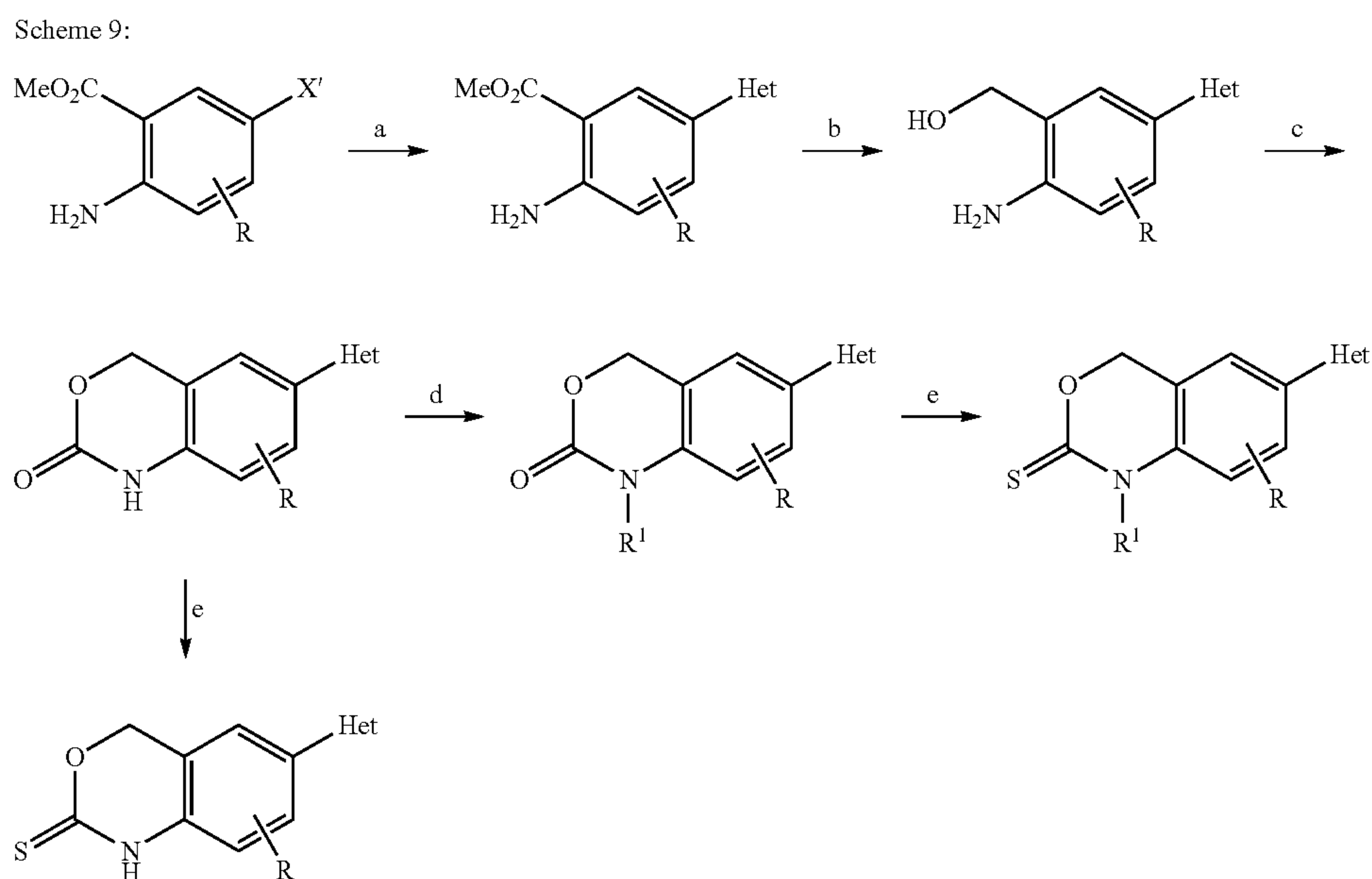
Scheme 9
