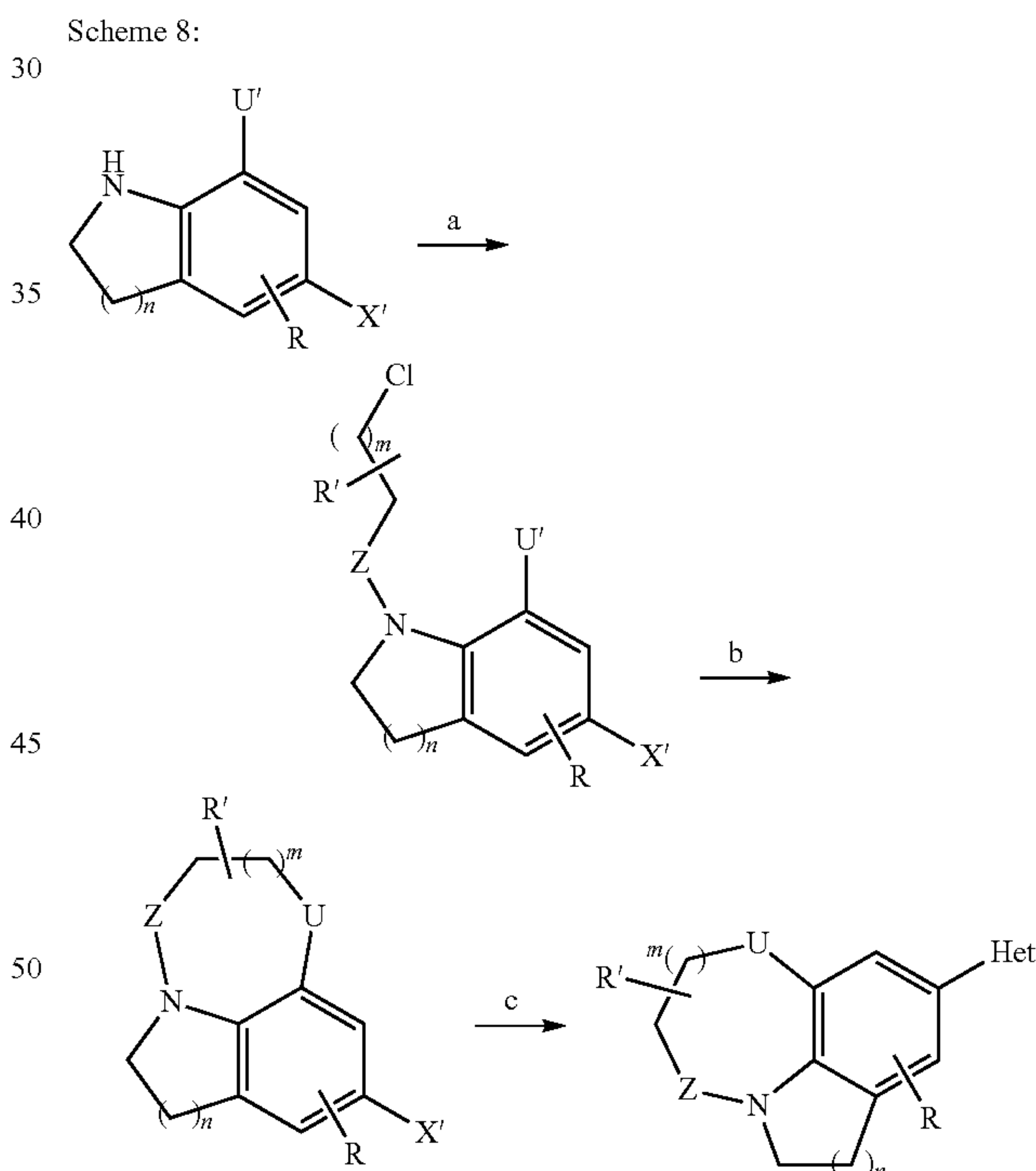
Scheme 8
