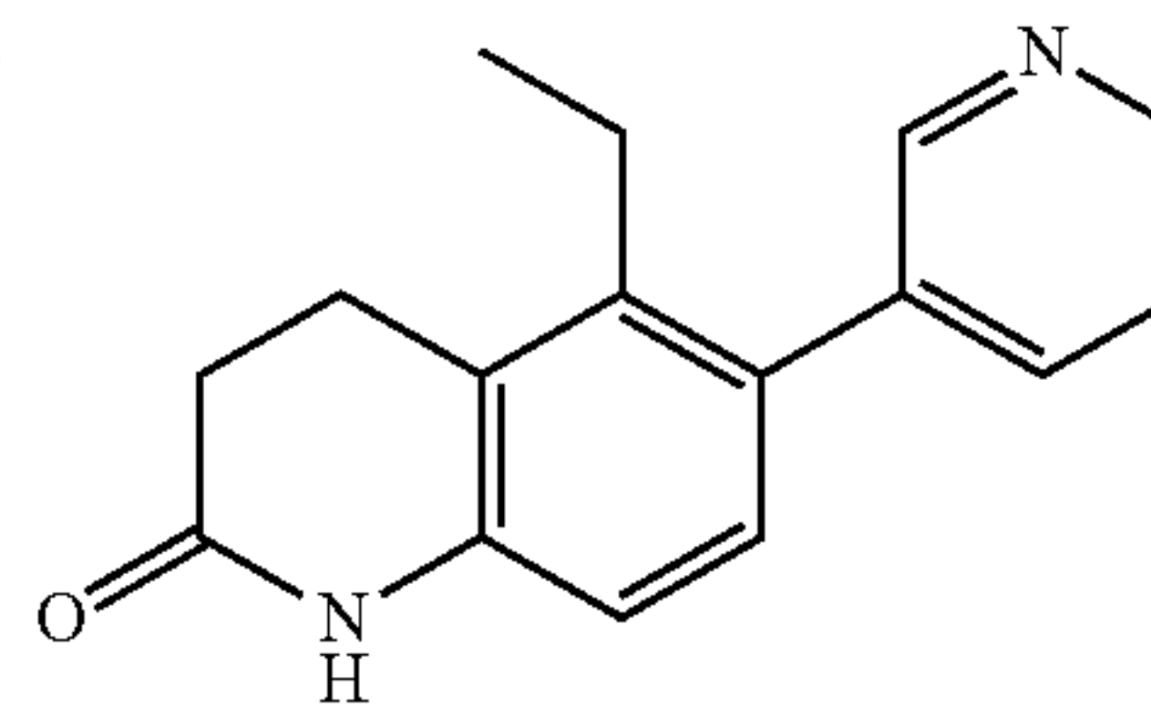
5-Ethyl-6-(pyridin-3-yl)-3,4-dihydroquinolin-2(1H)-one
