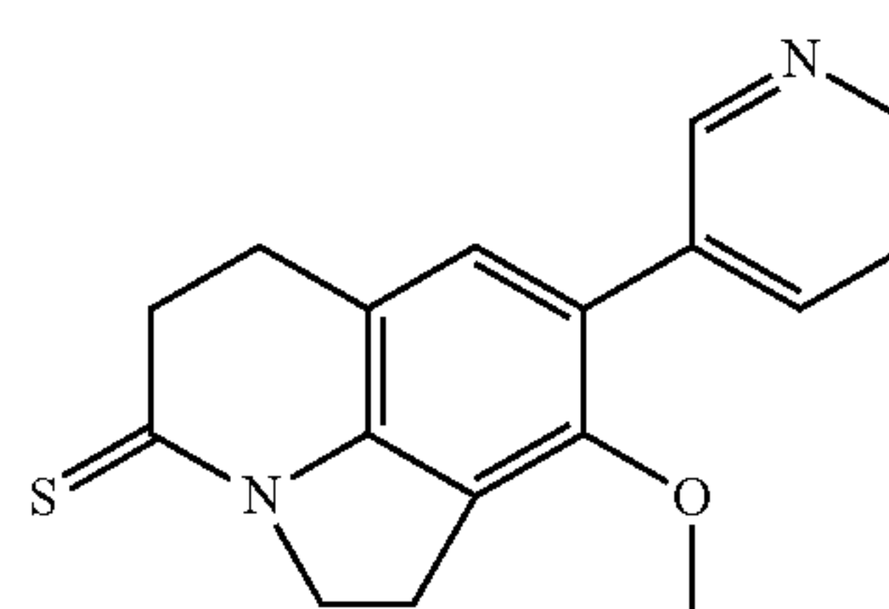
9-Methoxy-8-pyridin-3-yl-1,2,5,6-tetrahydro-4H-pyrrolo[3,2,1-ij]quinolin-4-thione
