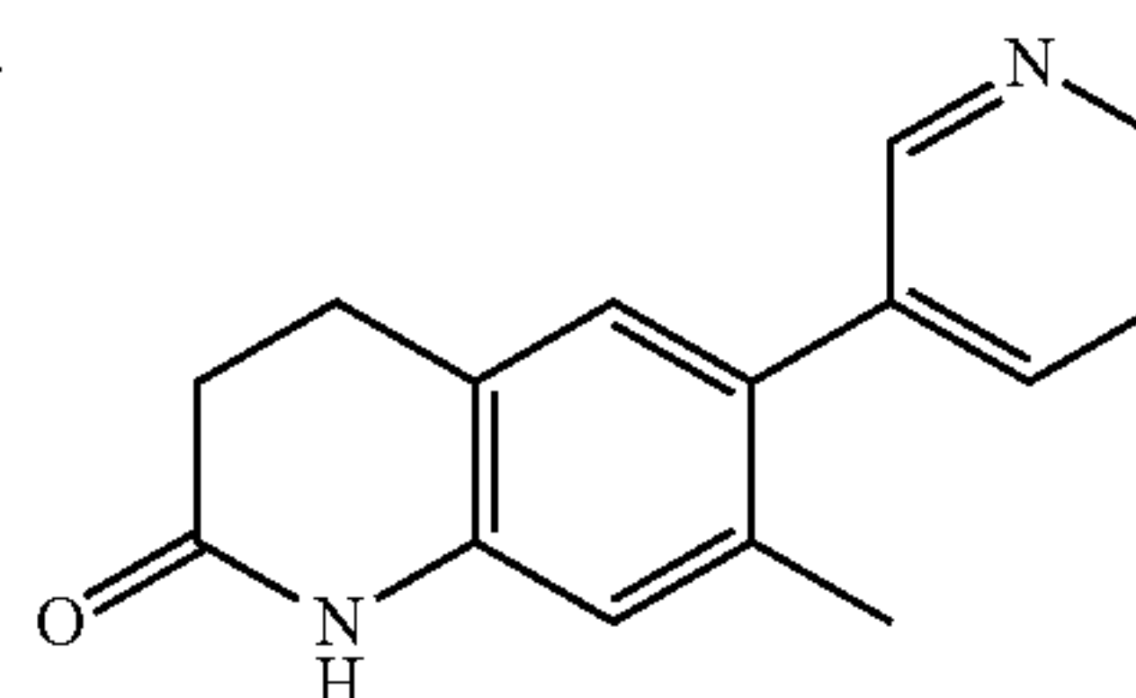
7-Methyl-6-pyridin-3-yl-3,4-dihydroquinolin-2(1H)-one
