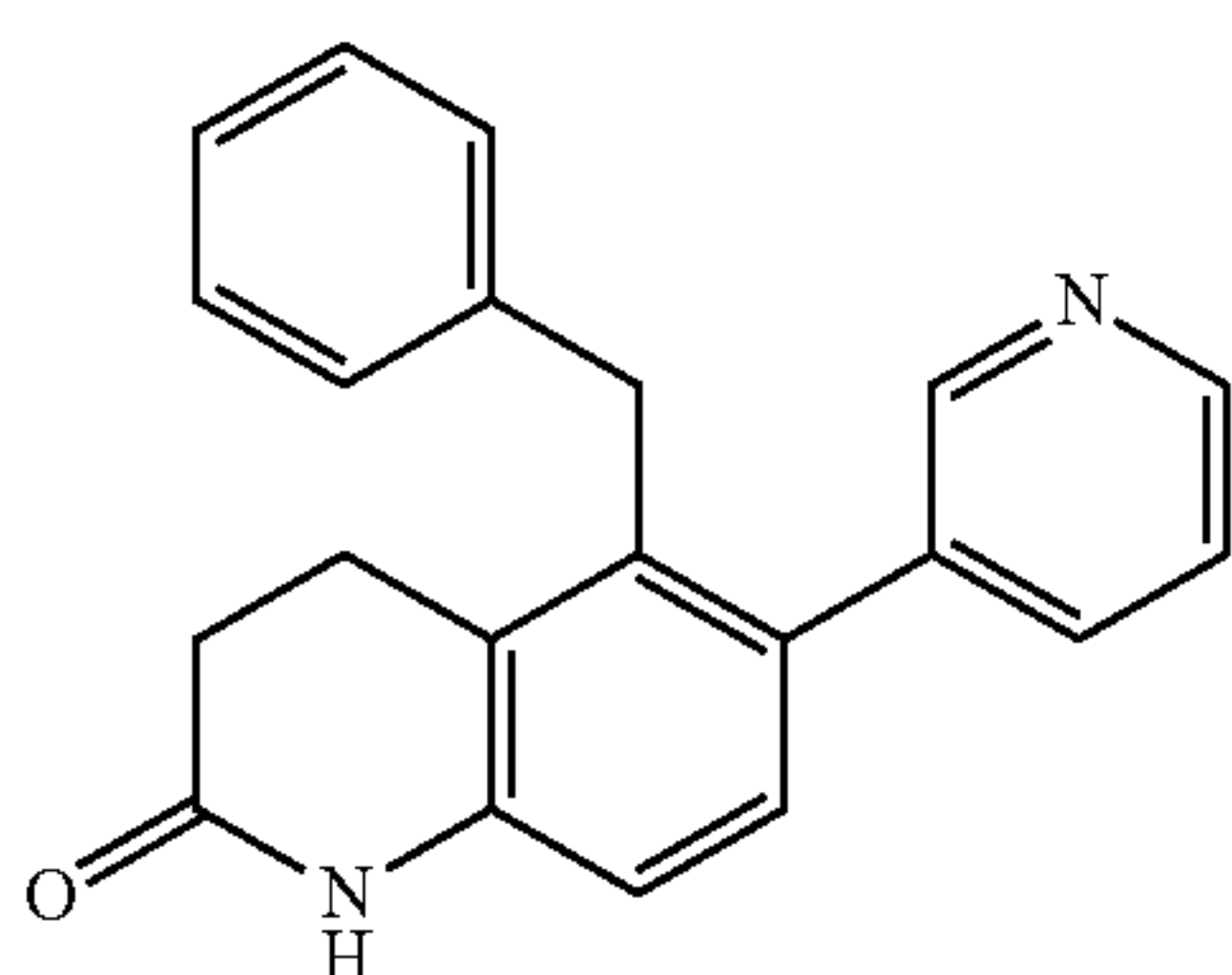
5-Benzyl-6-(pyridine-3-yl)- 3,4-dihydroquinolin- 2(1H)-one
