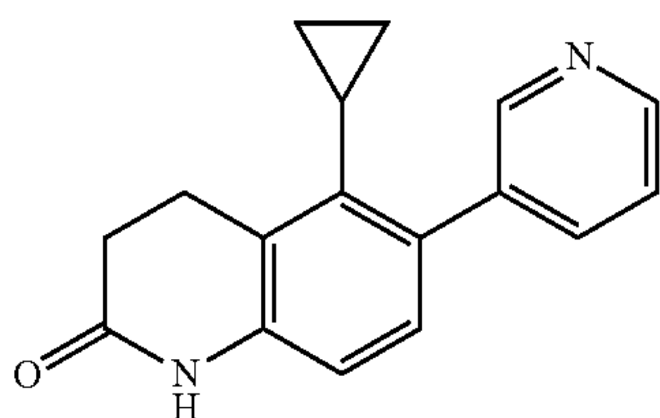
5-Cyclopropyl-6-(pyridin- 3-yl)-3,4-dihydroquinolin- 2(1H)-one
