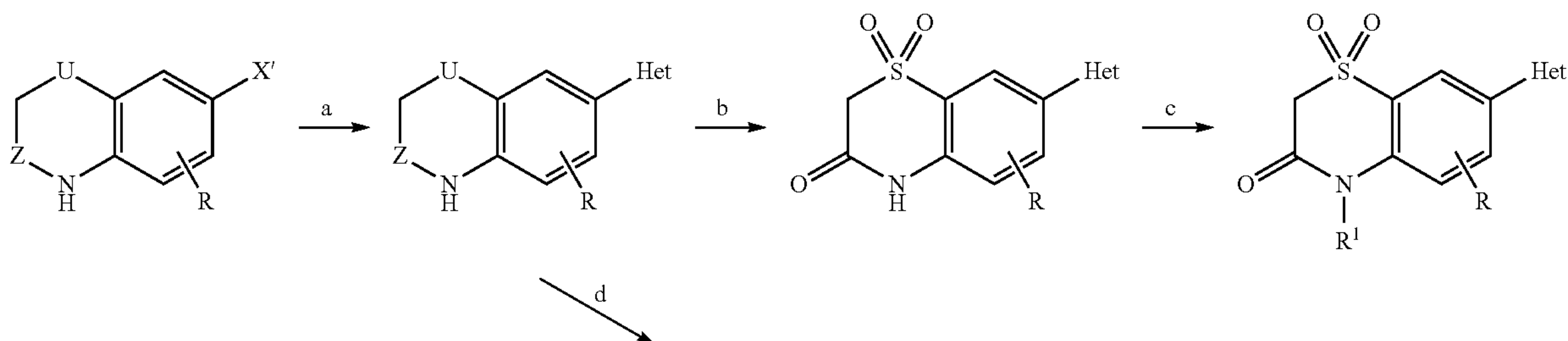
Scheme 14:
