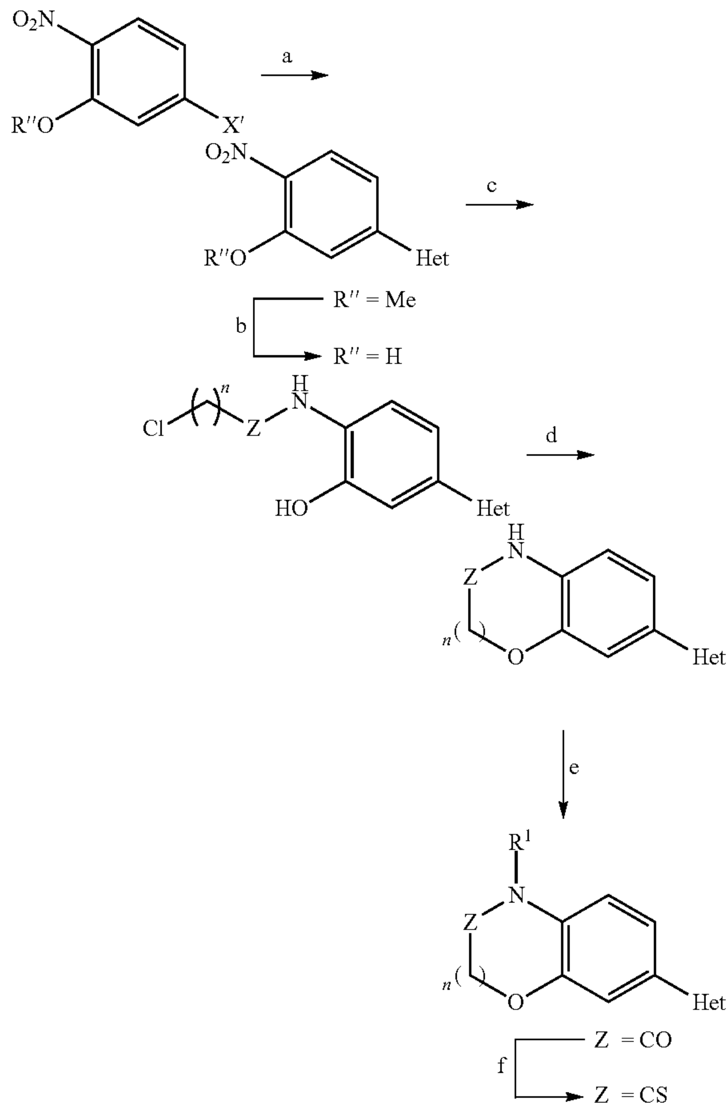
Scheme 13:
