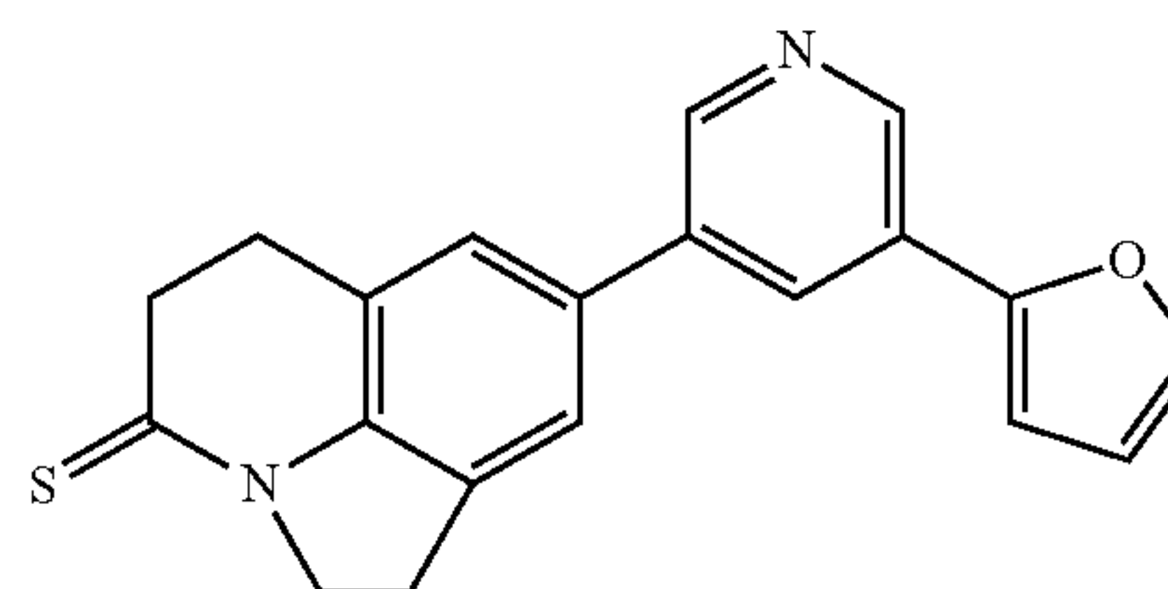
8-[5-(2-furan-2-yl)pyridin-3-yl]-1,2,5,6-tetrahydro-4H-pyrrolo[3,2,1-ij]quinolin-4-thione
