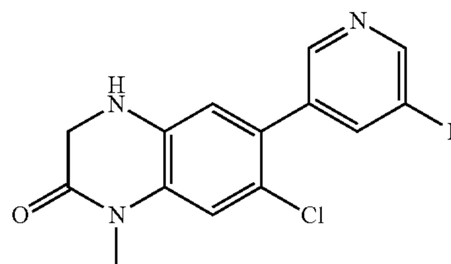
7-Chloro-6-(5-fluoropyridin-3-yl)-1-methyl-3,4-dihydroquinoxalin-2(1H)-one
