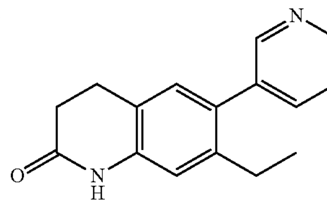
7-Ethyl-6-(pyridin-3-yl)-3,4-dihydroquinolin-2(1H)-one
