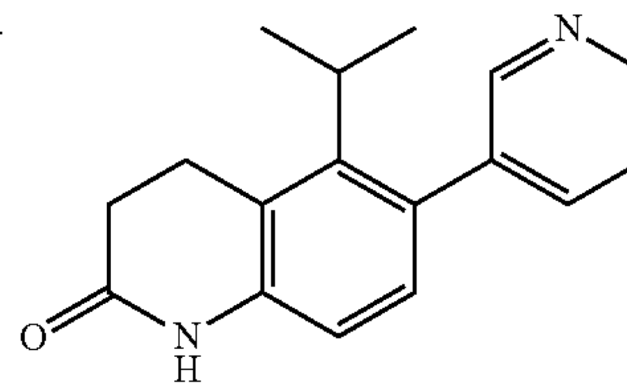
5-Isopropyl-6-(pyridin-3-yl)-3,4-dihydroquinolin-2(1H)-one
