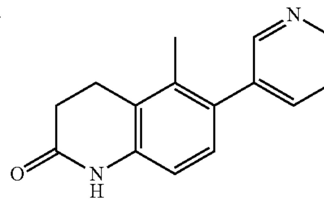
5-Methyl-6-pyridin-3-yl-3,4-dihydroquinolin-2(1H)-one
