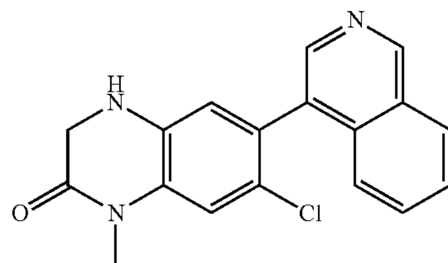
7-Chloro-6-(isoquinolin-4-yl)-1-methyl-3,4-dihydroquinoxalin-2(1H)-one
