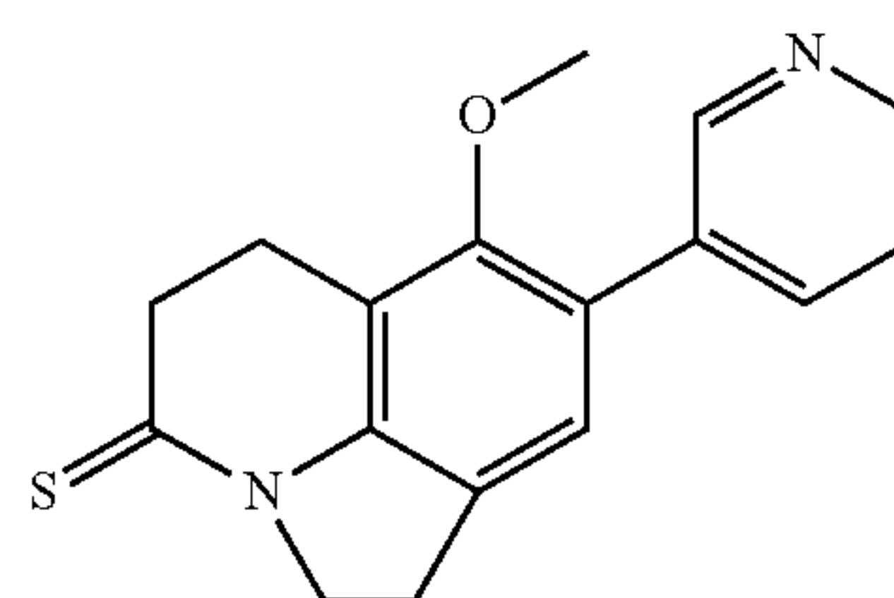
7-Methoxy-8-pyridin-3-yl-1,2,5,6-tetrahydro-4H-pyrrolo[3,2,1-ij]quinolin-4-thione
