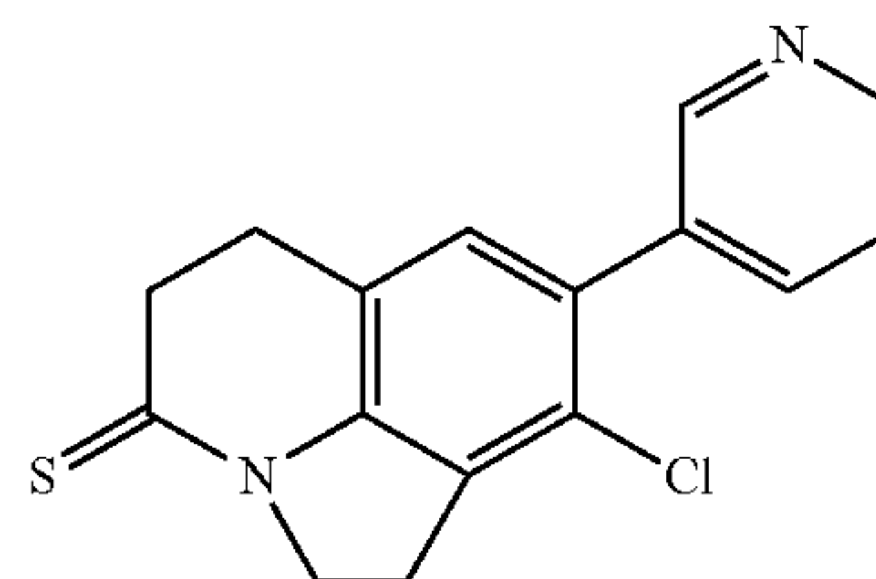
9-Chloro-8-pyridin-3-yl-1,2,5,6-tetrahydro-4H-pyrrolo[3,2,1-ij]quinolin-4-thione
