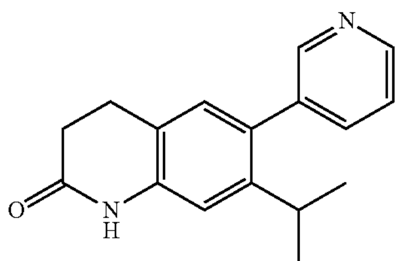
7-Isopropyl-6-(pyridin-3-yl)- 3,4-dihydroquinolin- 2(1H)-one
