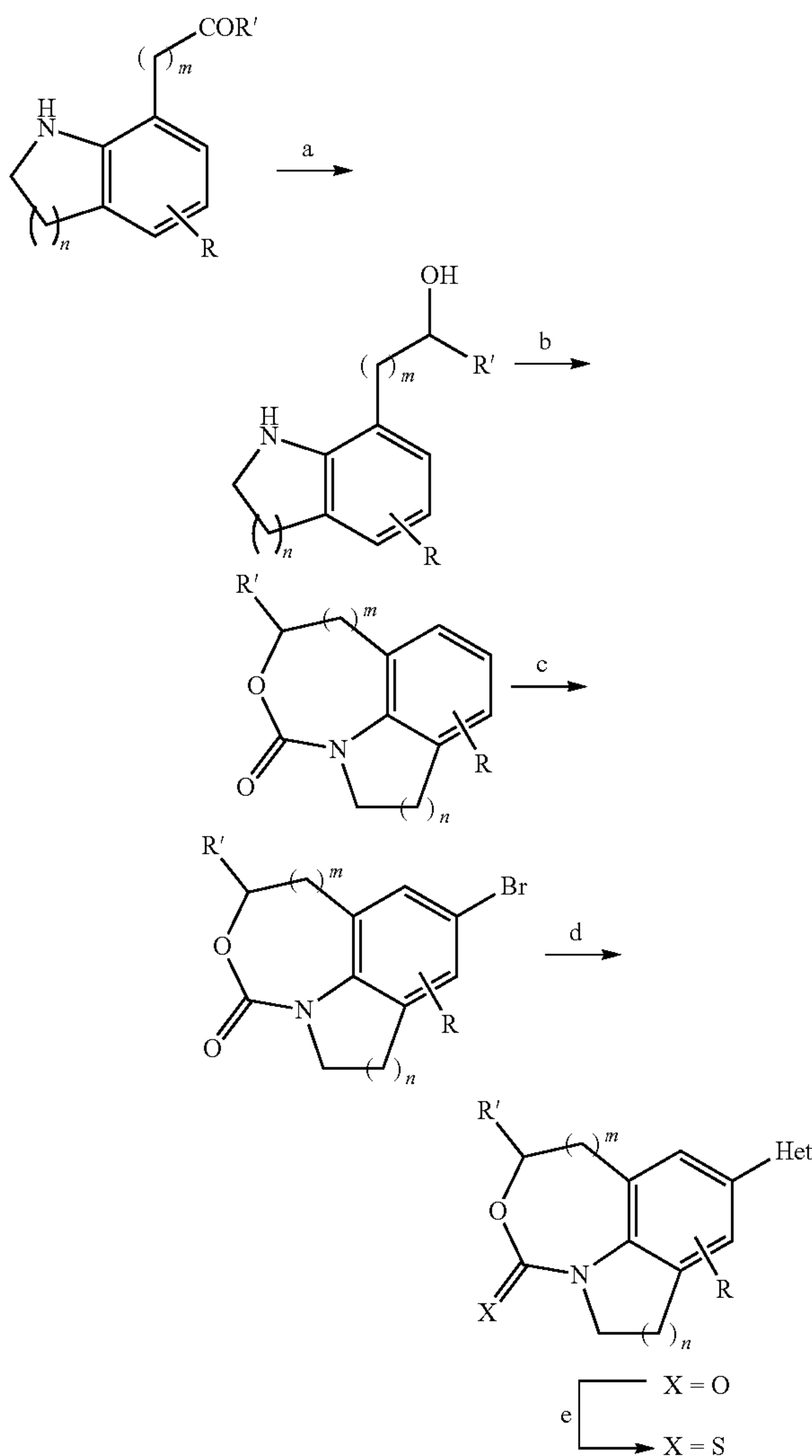
Scheme 7:
