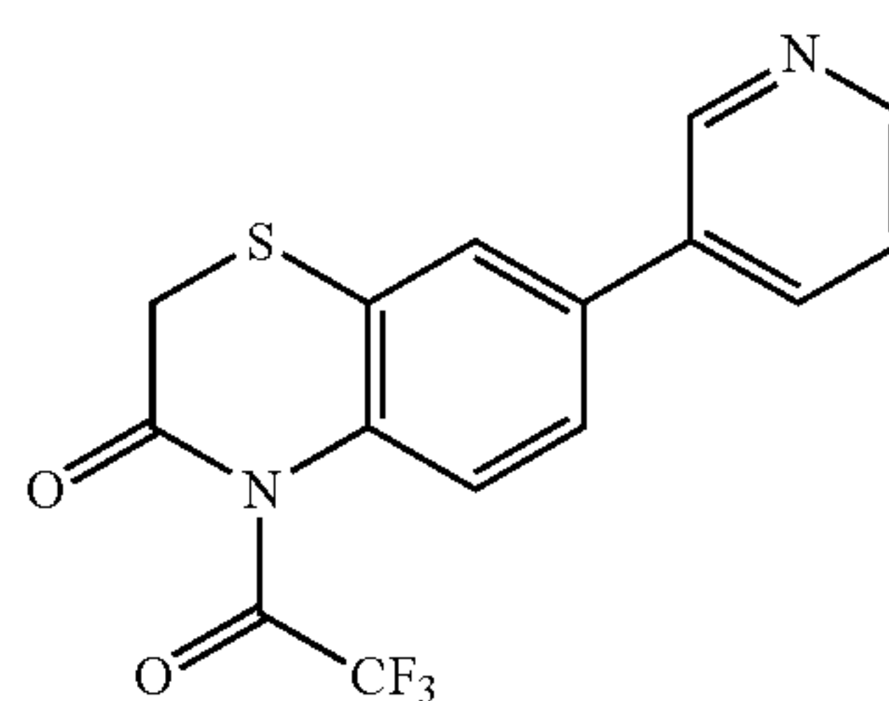
7-(Pyridin-3-yl)-4-(2,2,2-trifluoroacetyl)-2H-benzo[b][1,4]thiazin-3(4H)-one
