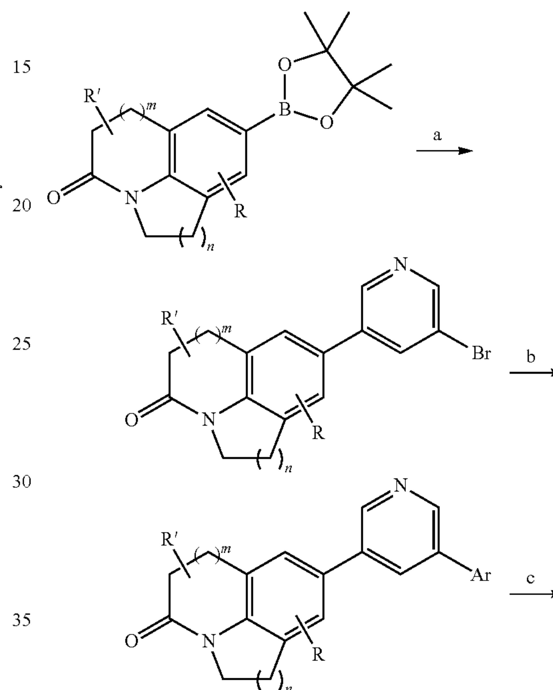
Scheme 3
