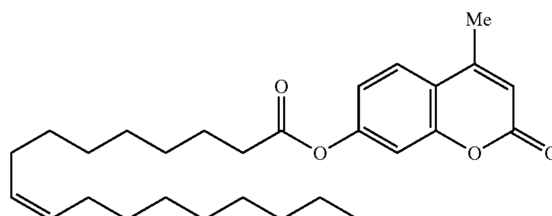
4-methylumbelliferyl oleate
