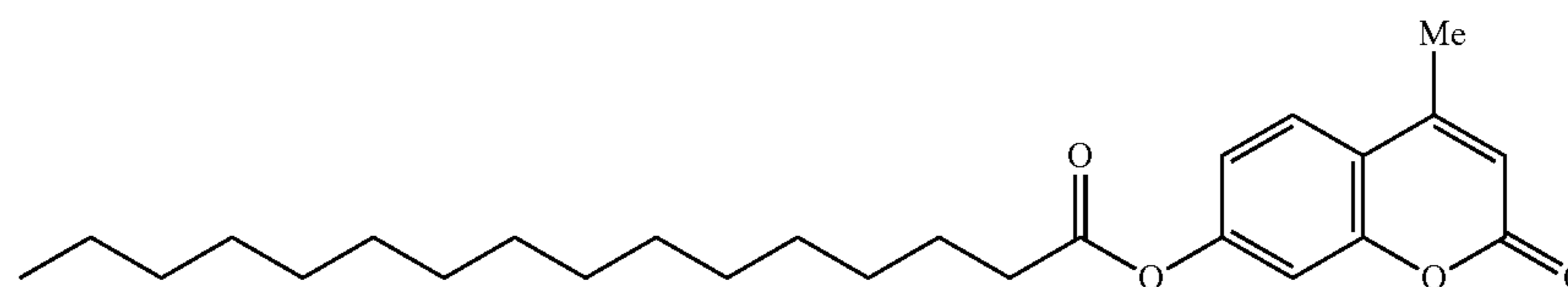
4-methylumbelliferyl palmitate
