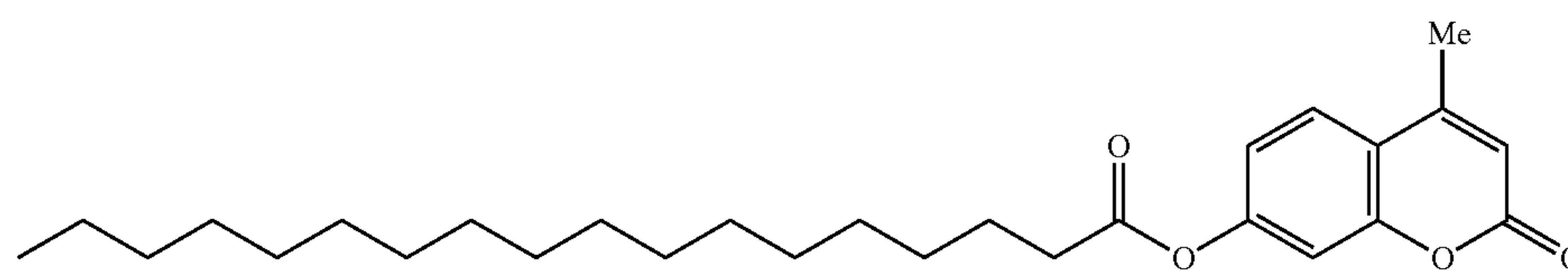
4-methylumbelliferyl stearate
