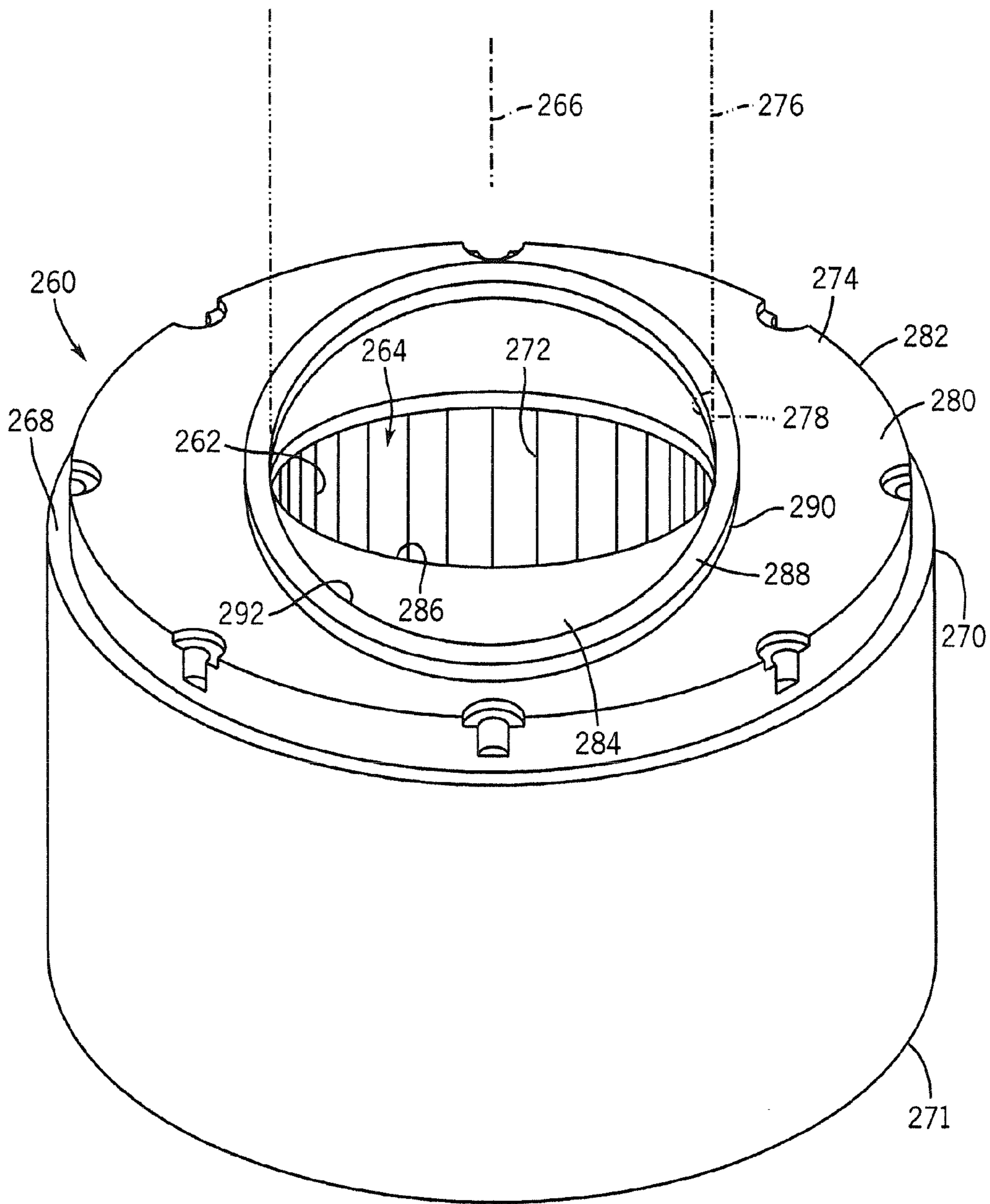
FIG. 14 PRIOR ART
