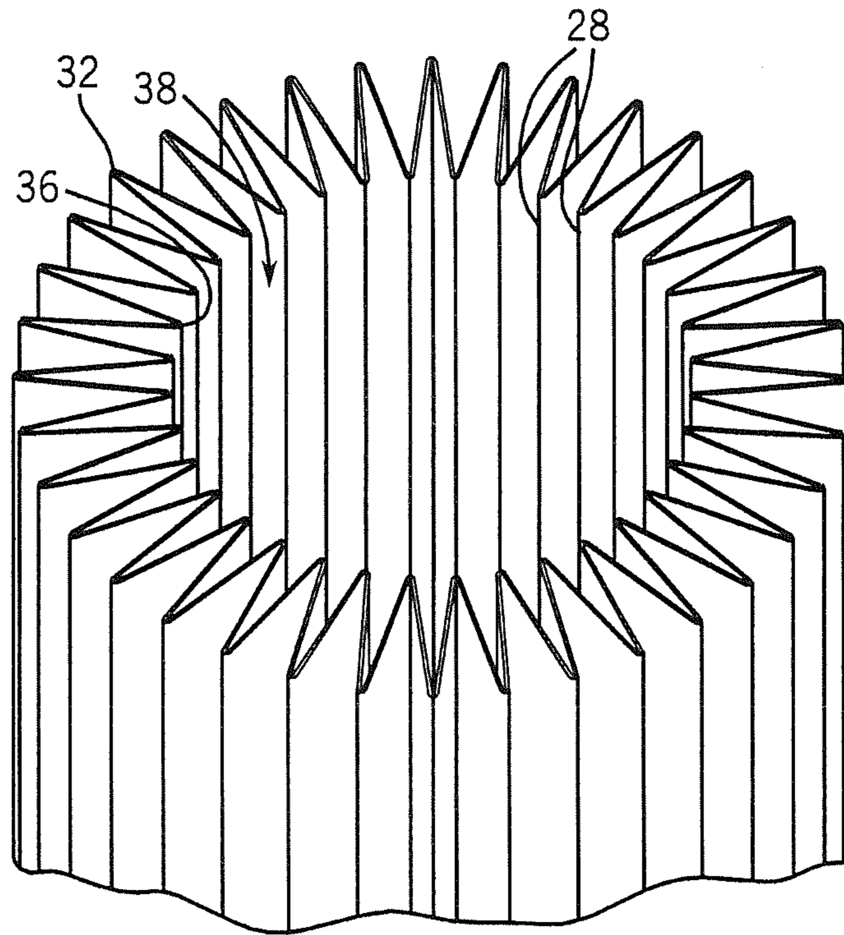
FIG. 8 PRIOR ART
