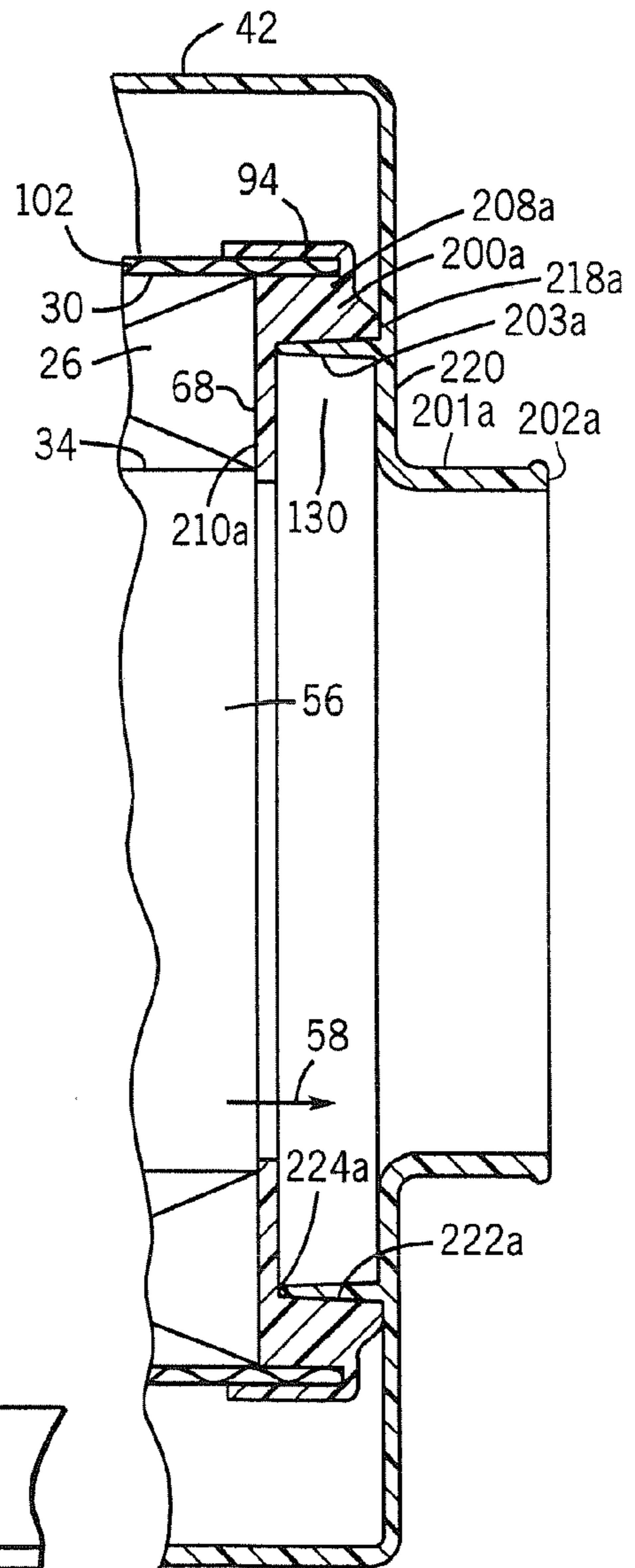
FIG. 11 PRIOR ART
