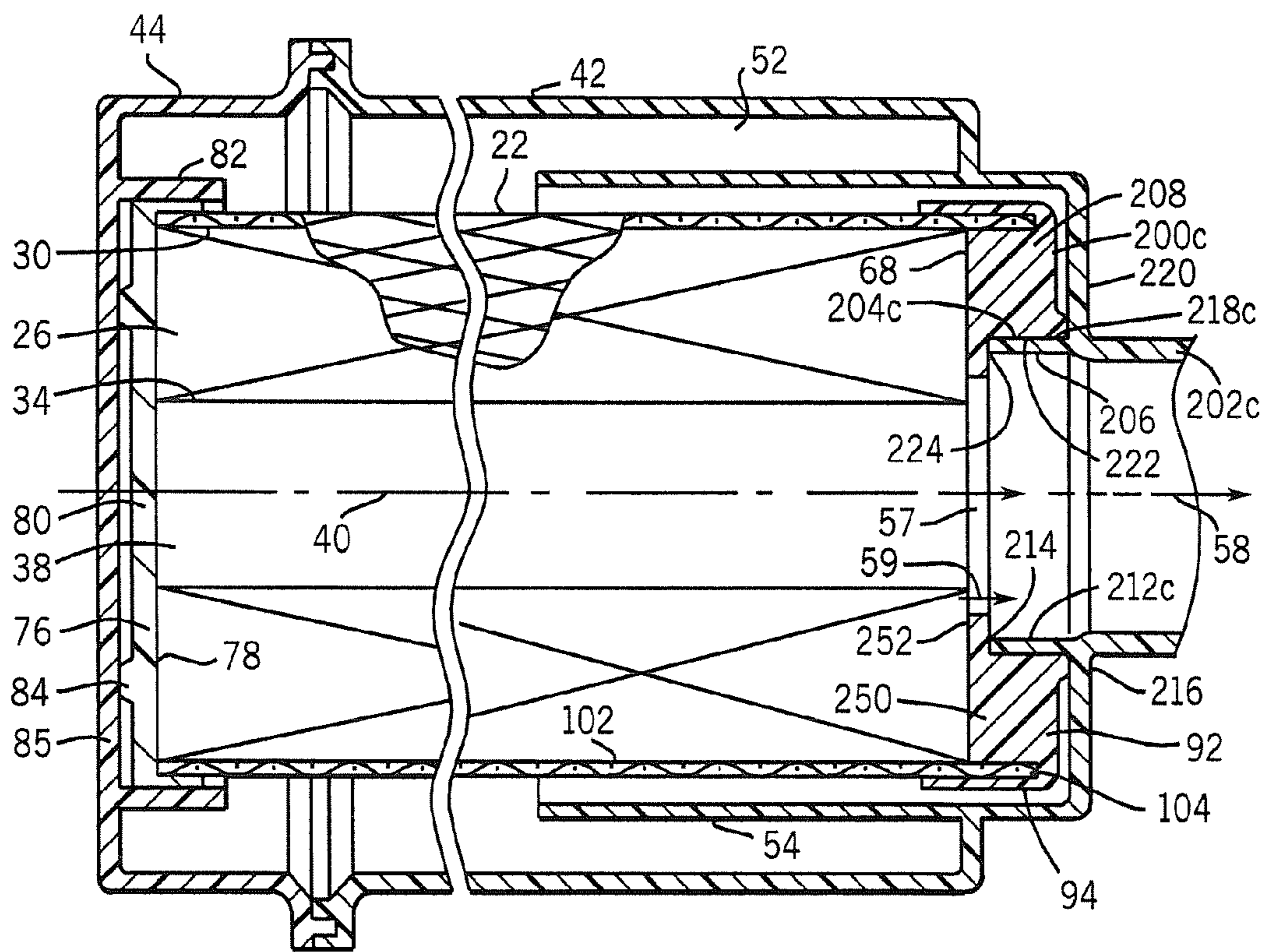
FIG. 13 PRIOR ART
