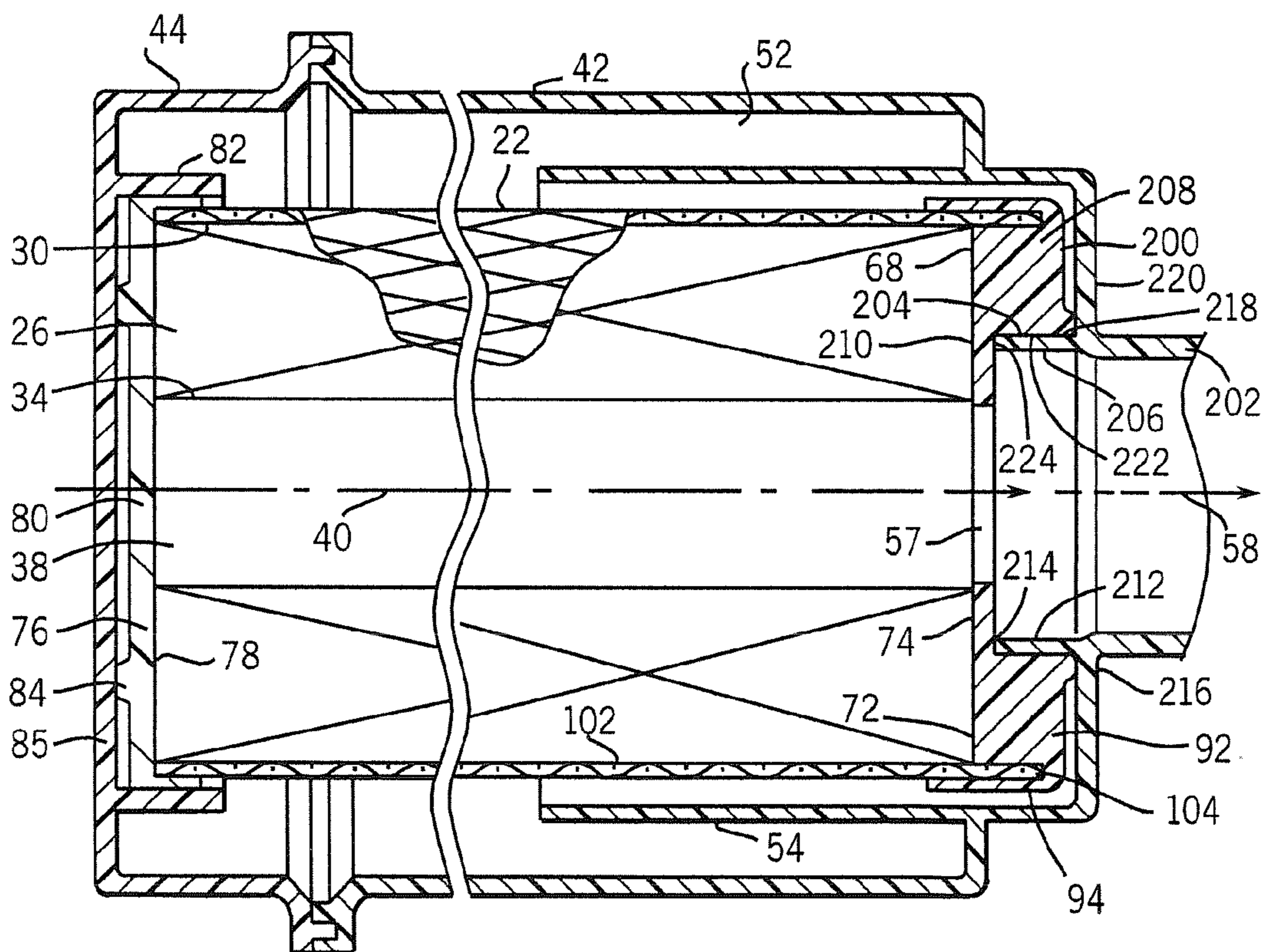
FIG. 7 PRIOR ART
