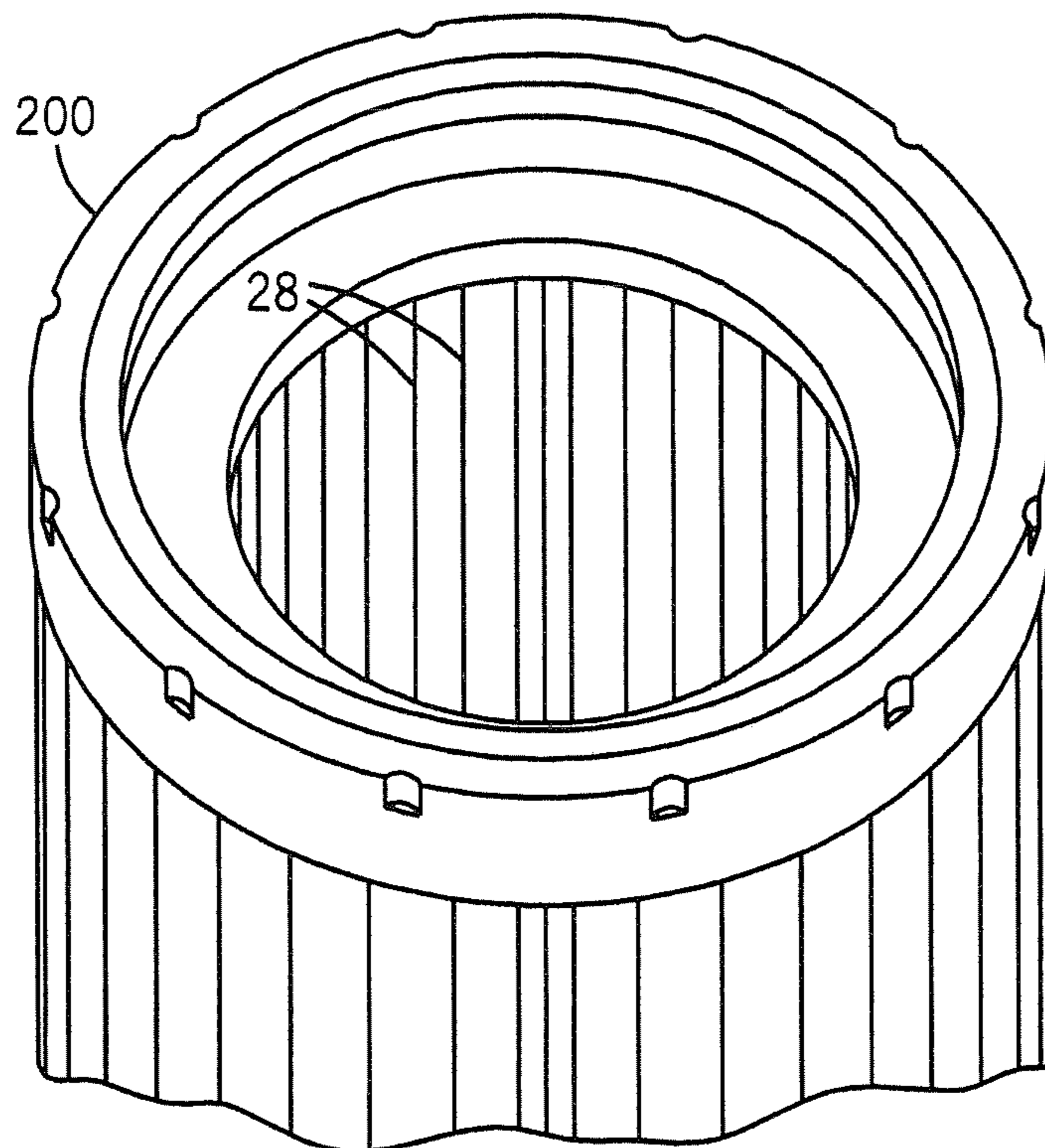
FIG. 9 PRIOR ART
