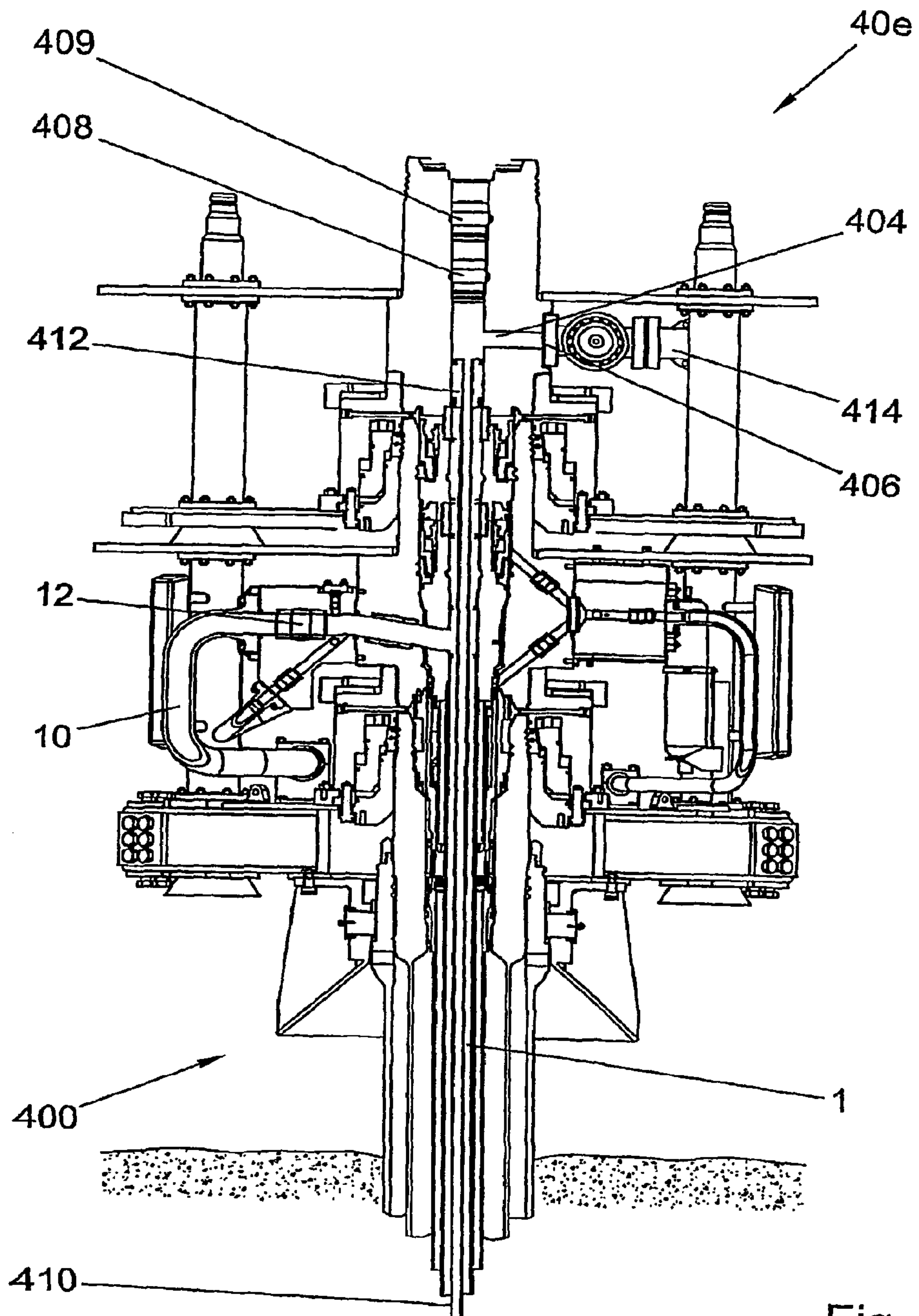
TYPICAL SECTION
