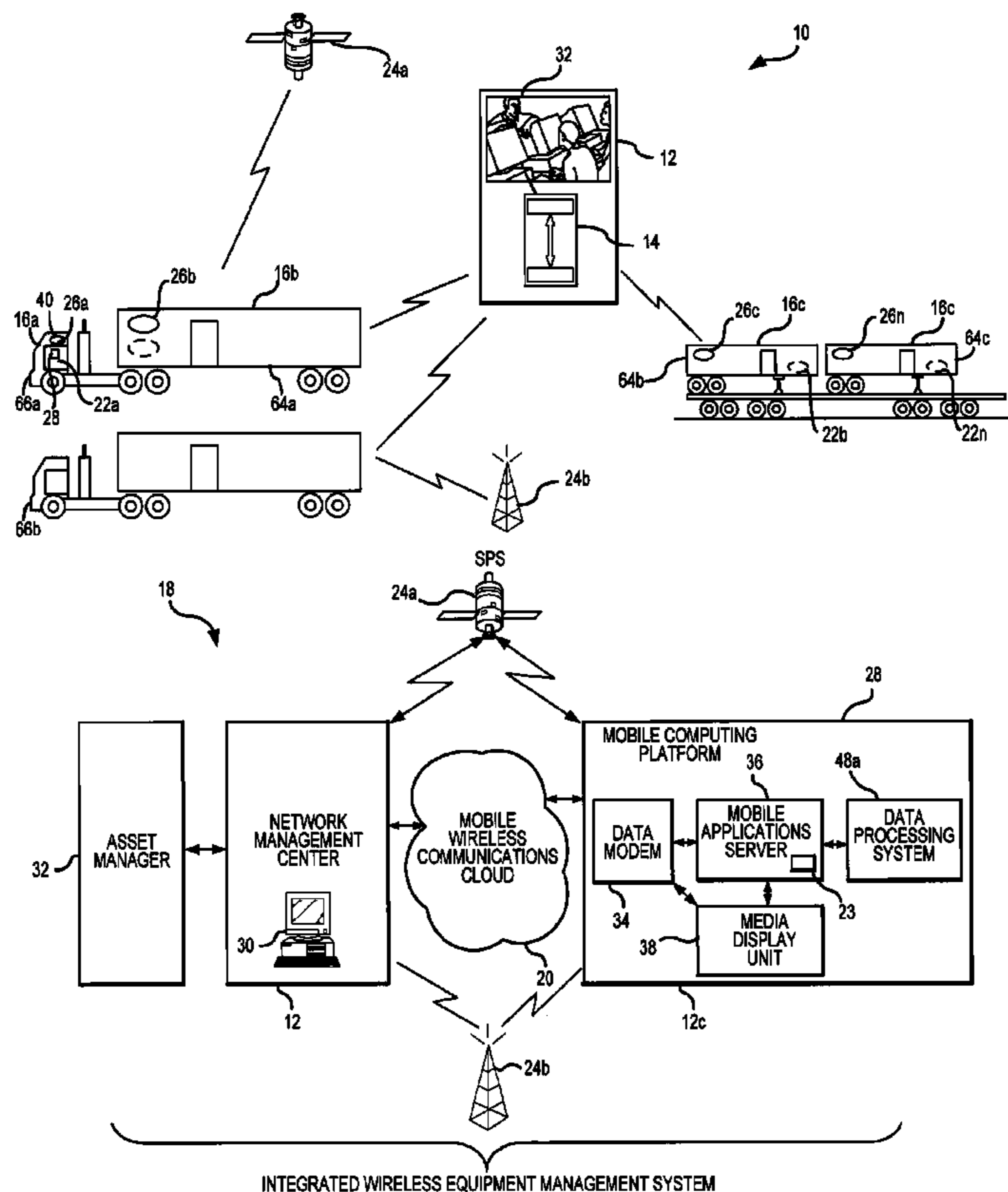
INTEGRATED WIRELESS EQUIPMENT MANAGEMENT SYSTEM
