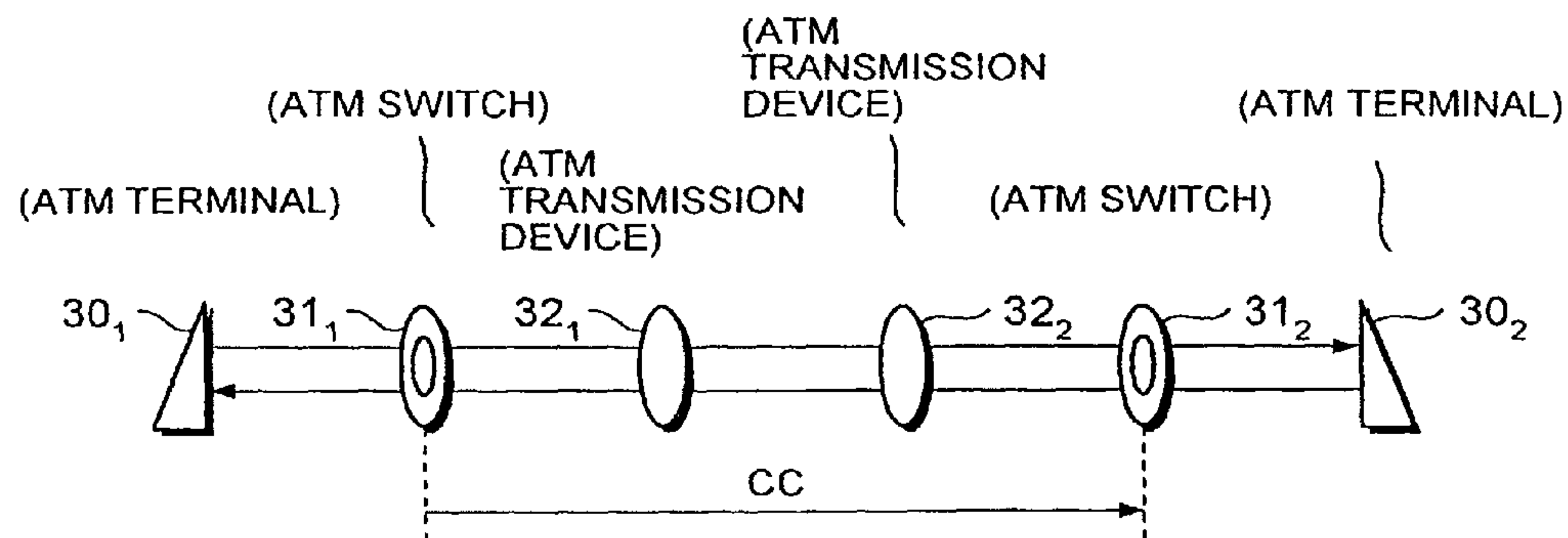
FIG. 24 (PRIOR ART)
