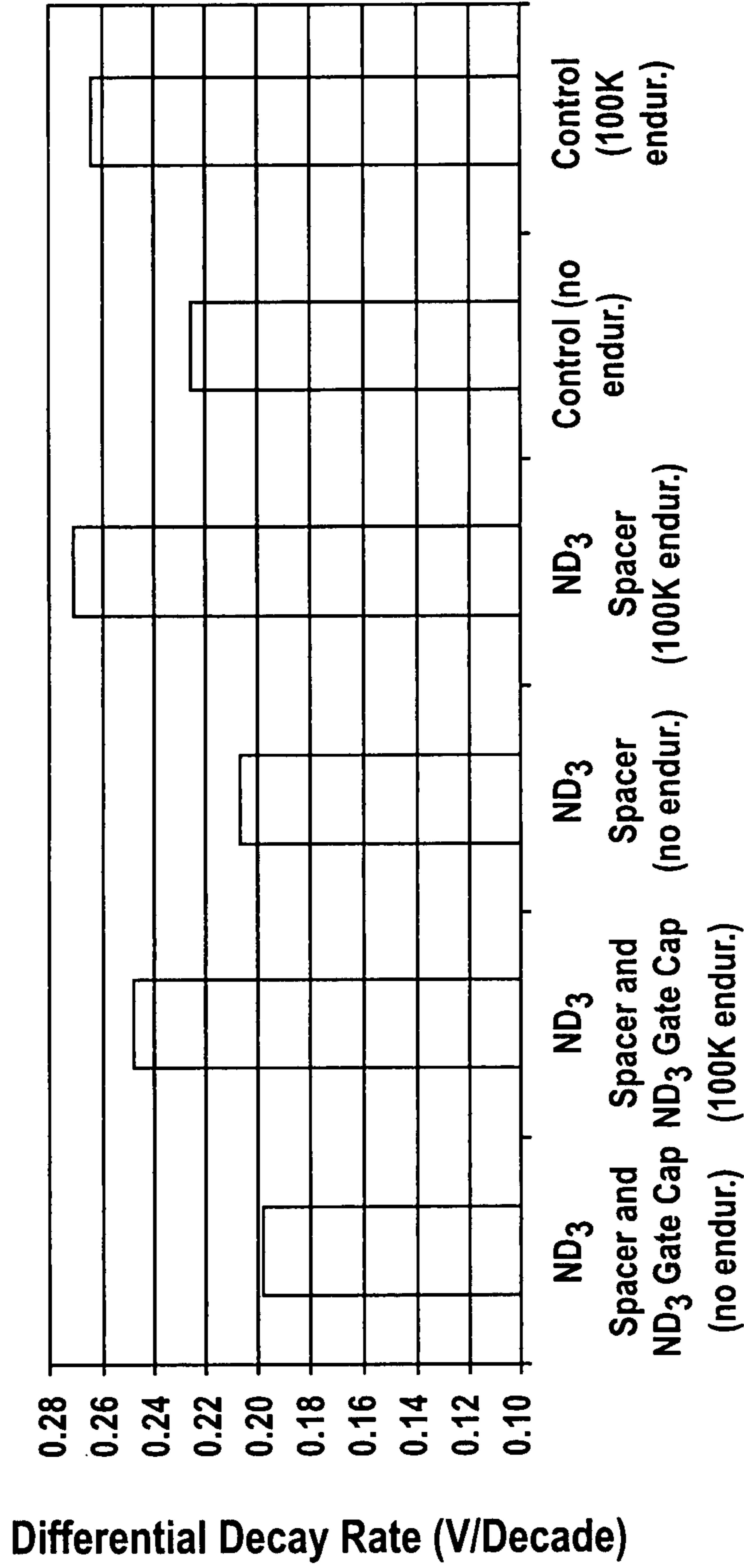
Decay Rate Comparison (100°C)
