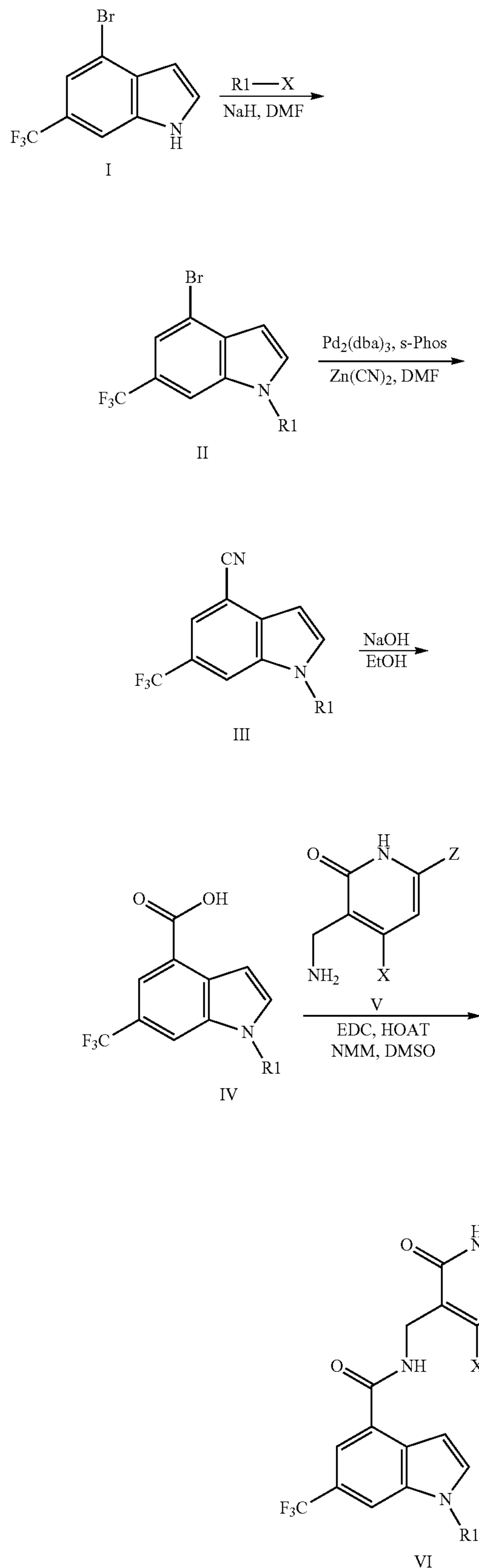
Scheme 2
