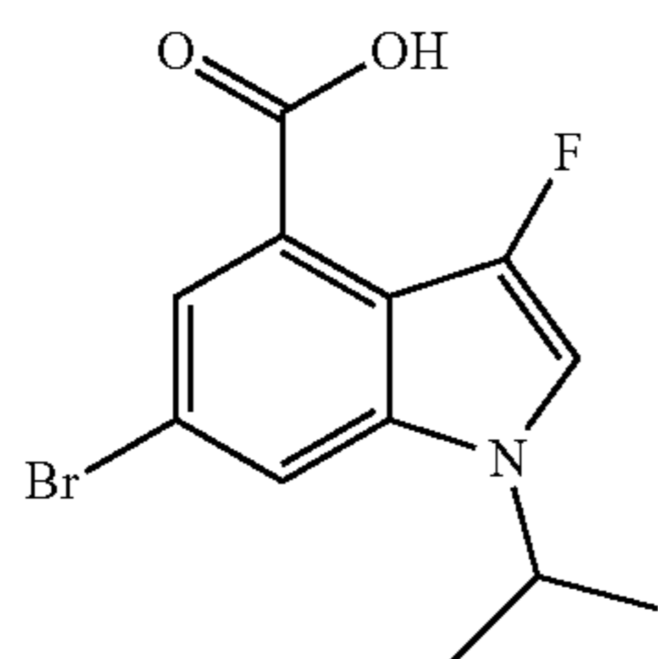
a) Methyl 6-bromo-3-fluoro-1-isopropyl-1H-indole-4-carboxylate
