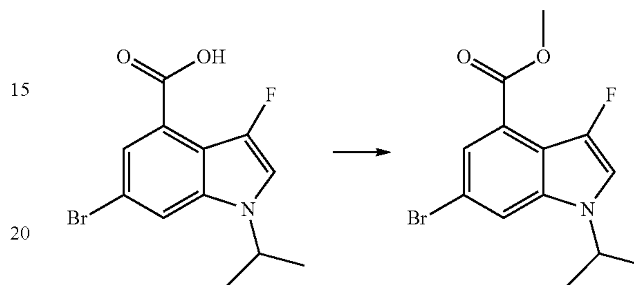
6-Bromo-3-fluoro-1-isopropyl-1H-indole-4-carboxylic acid
