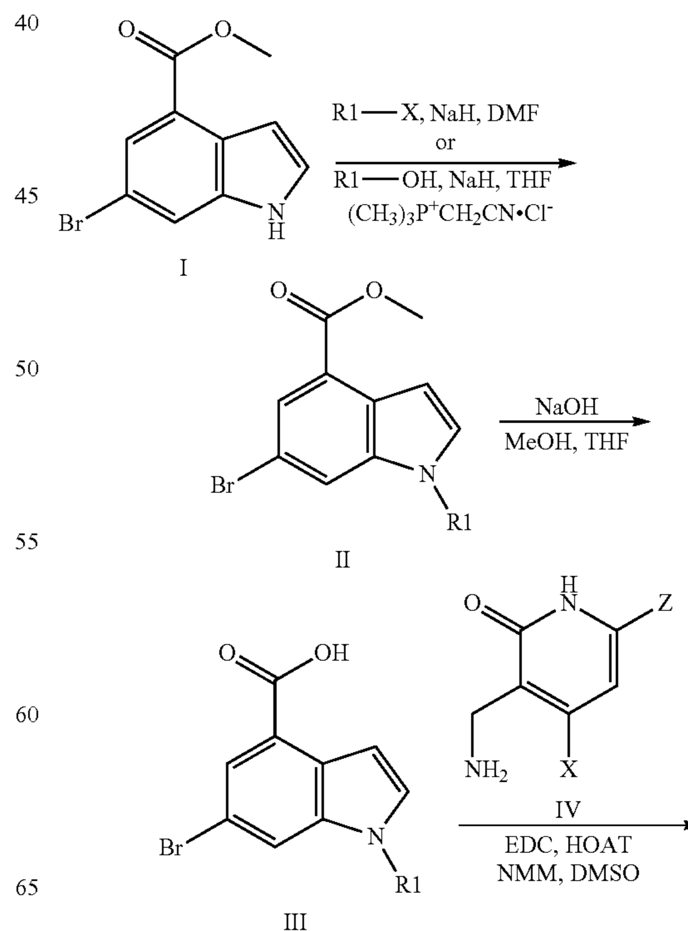
Scheme 1
