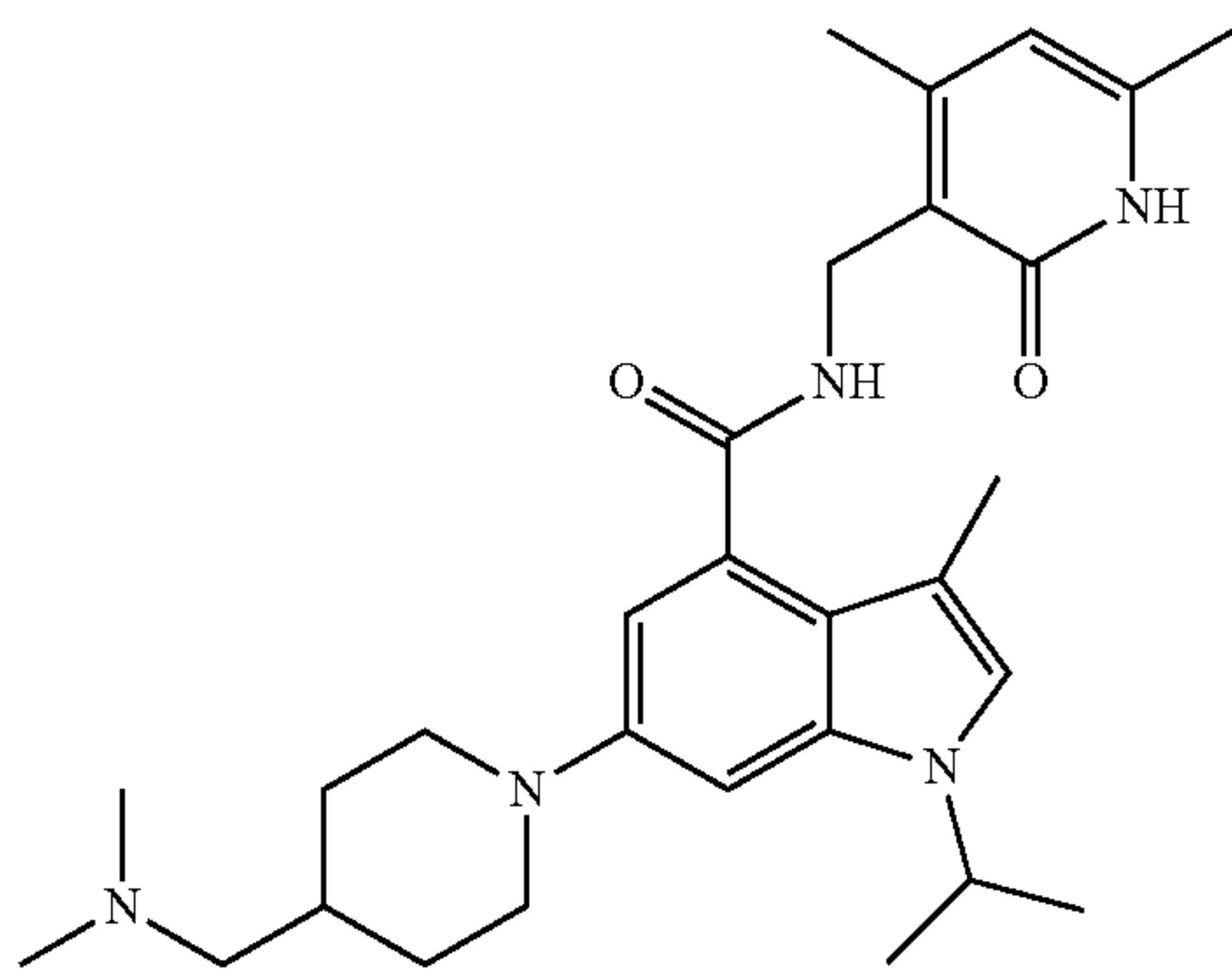
a) 6-(4-((Dimethylamino)methyl)piperidin-1-yl)-1-isopropyl-3-methyl-1H-indole-4-
