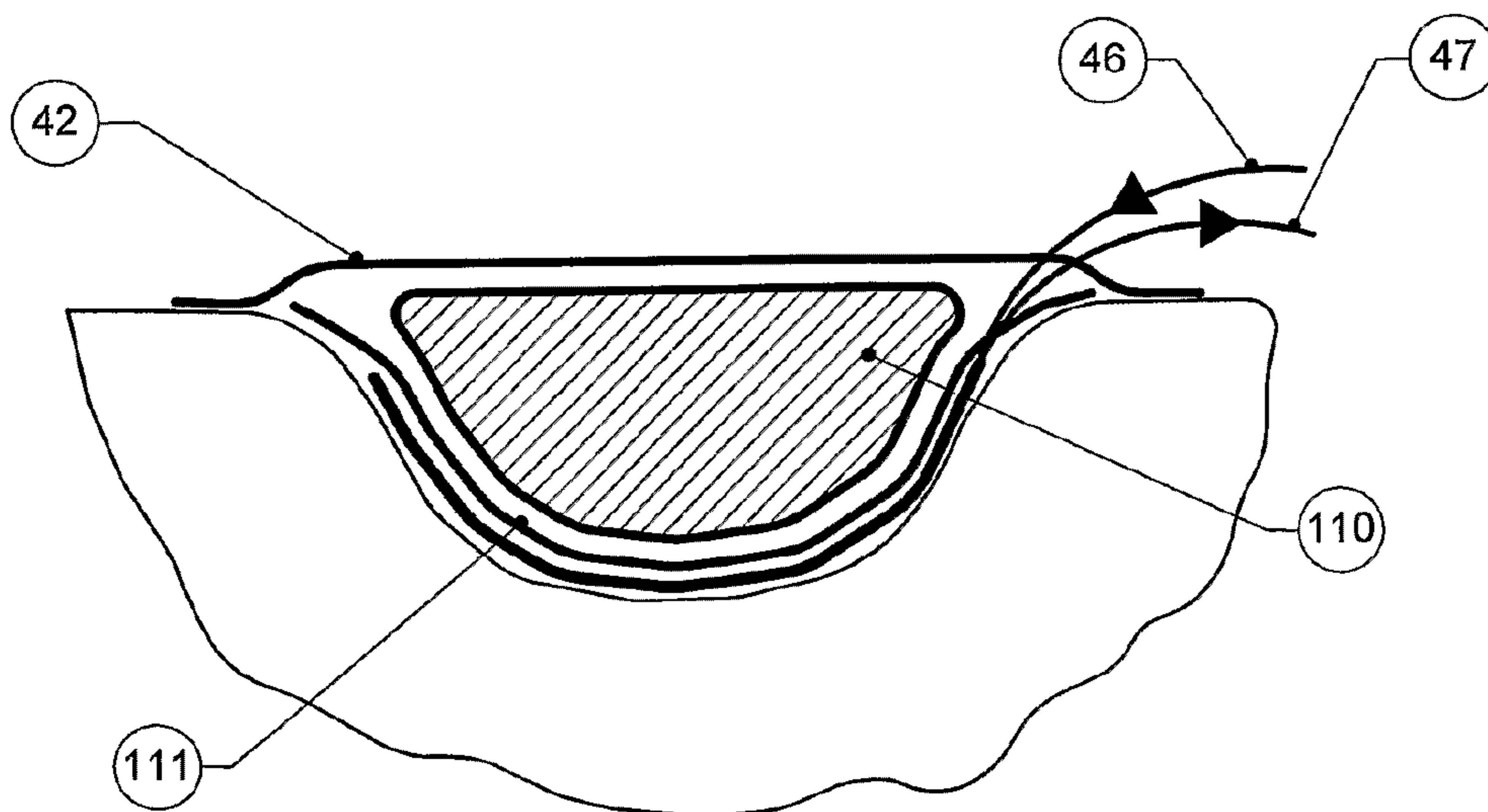
Section Through X -X
