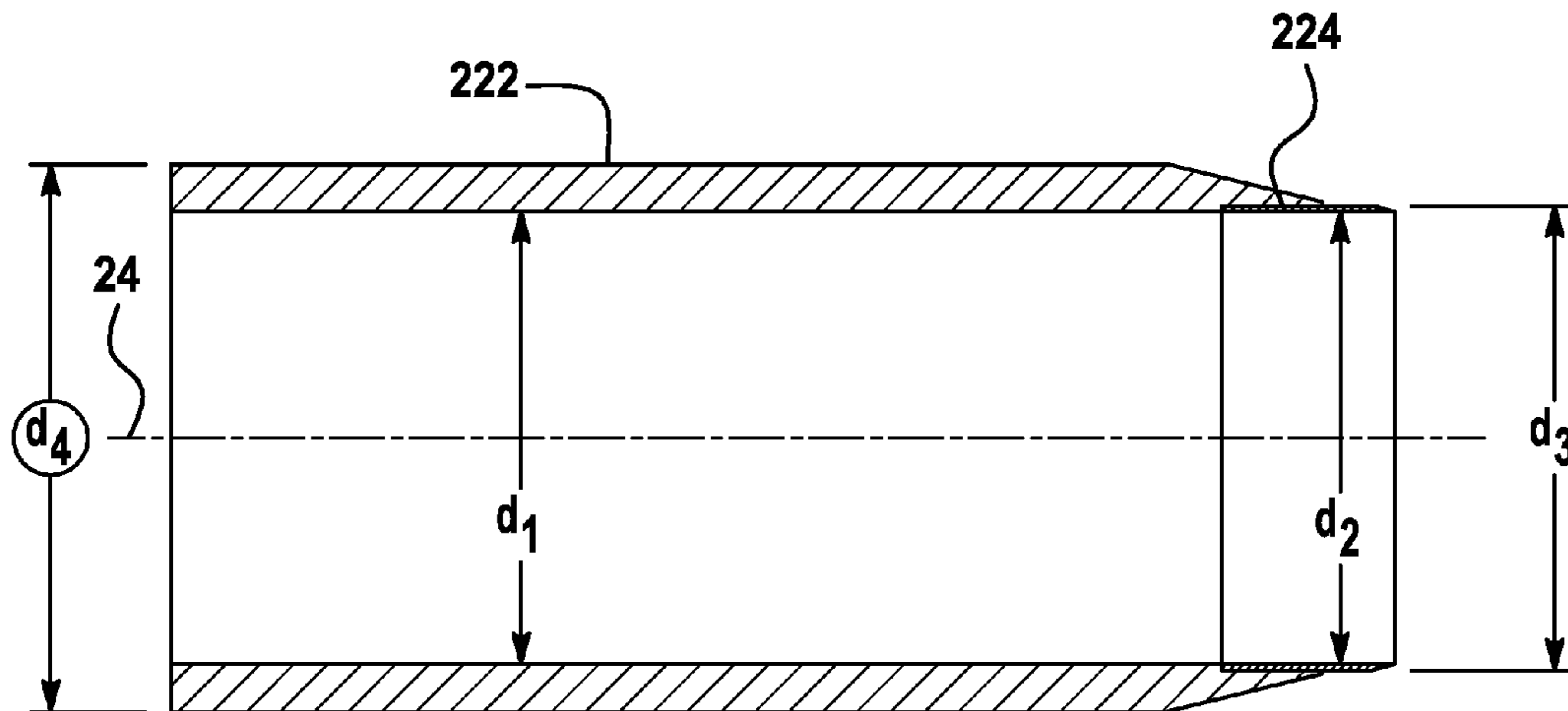
Figure 40 Prior Art
