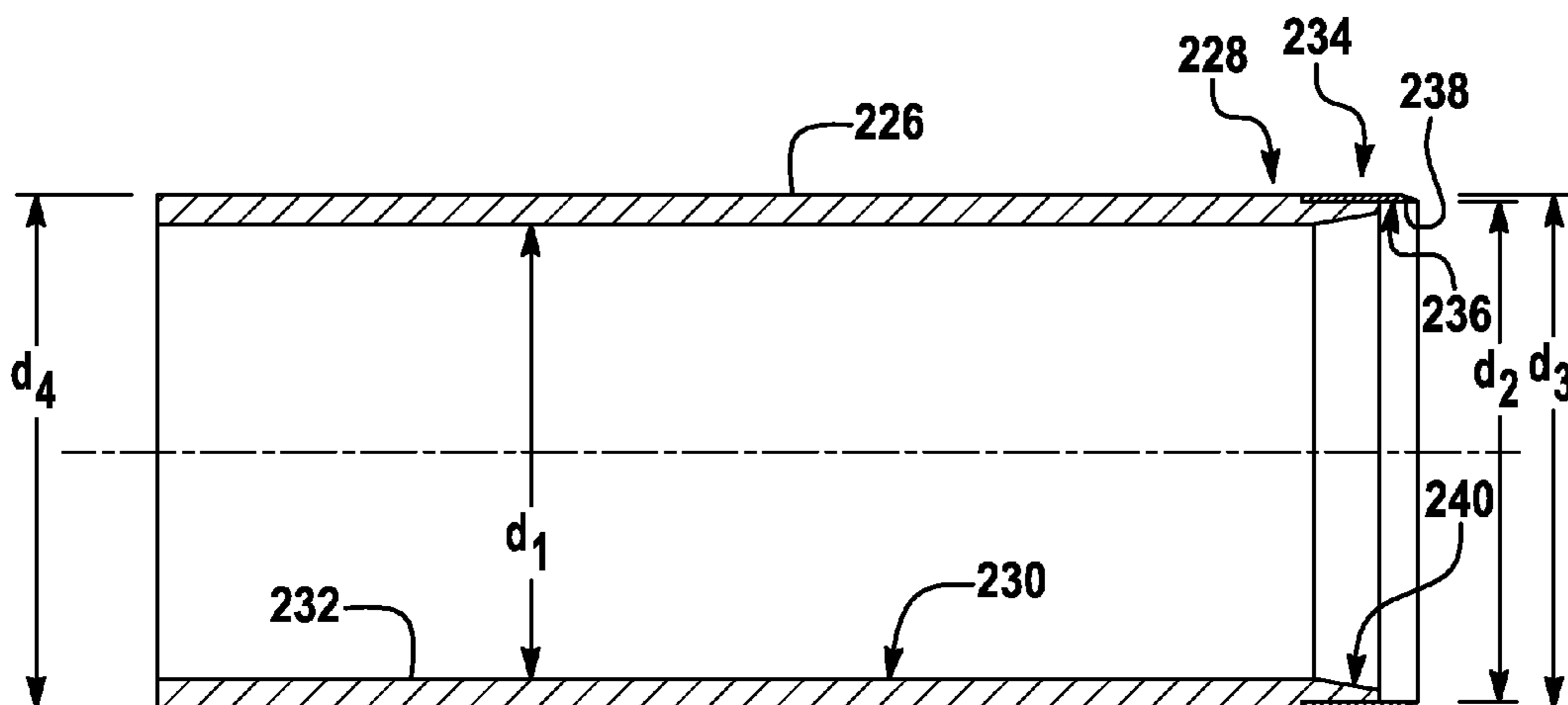
Figure 40 Prior Art
