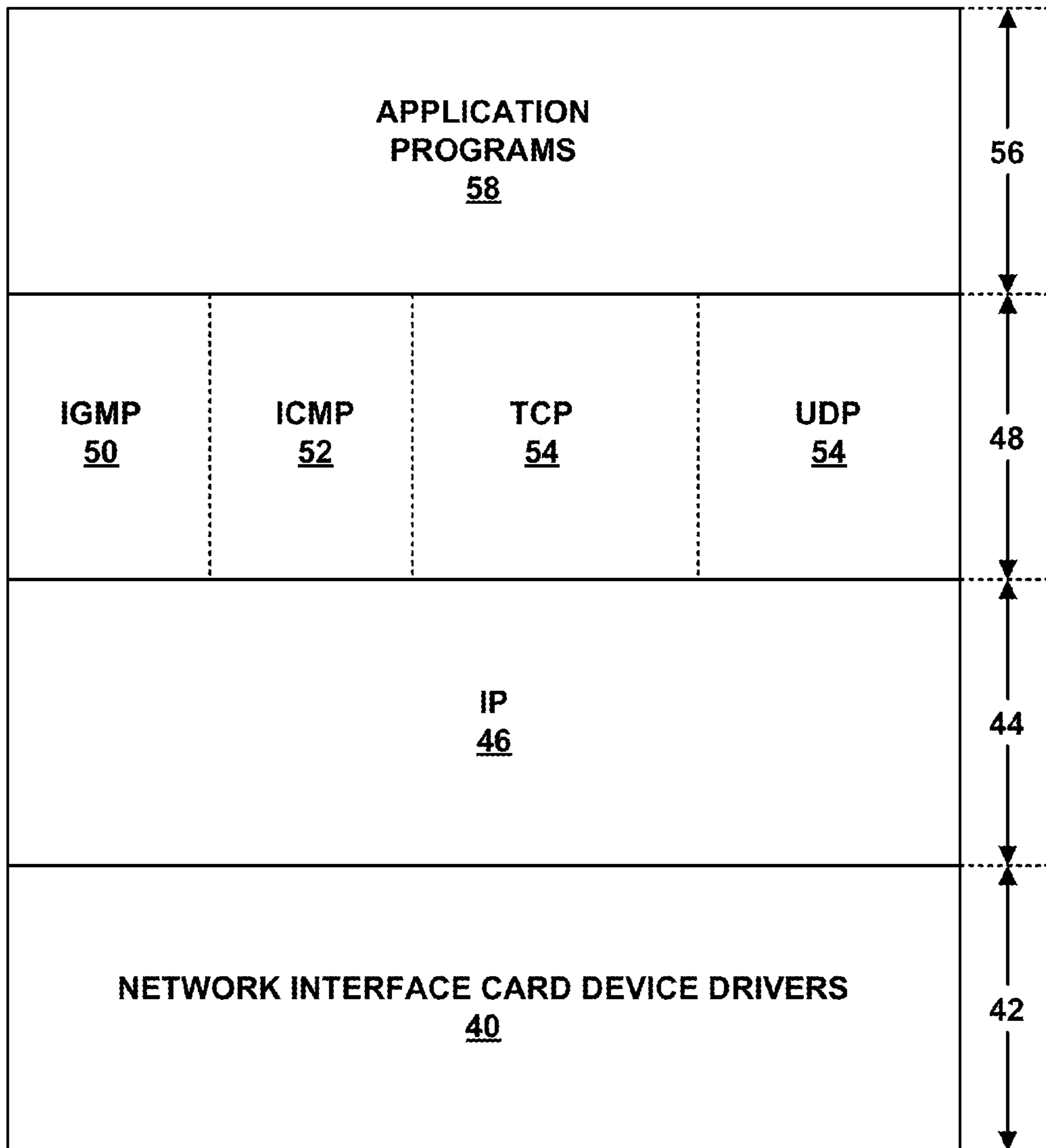
FIG. 3 PROTOCOL STACK
