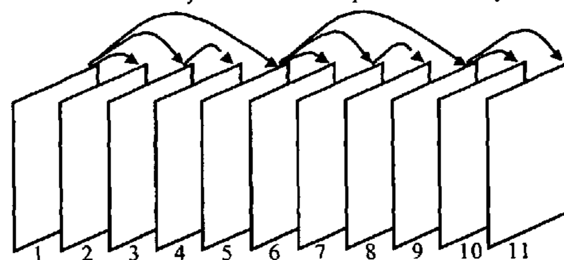
Three-layer recursive temporal scalability
