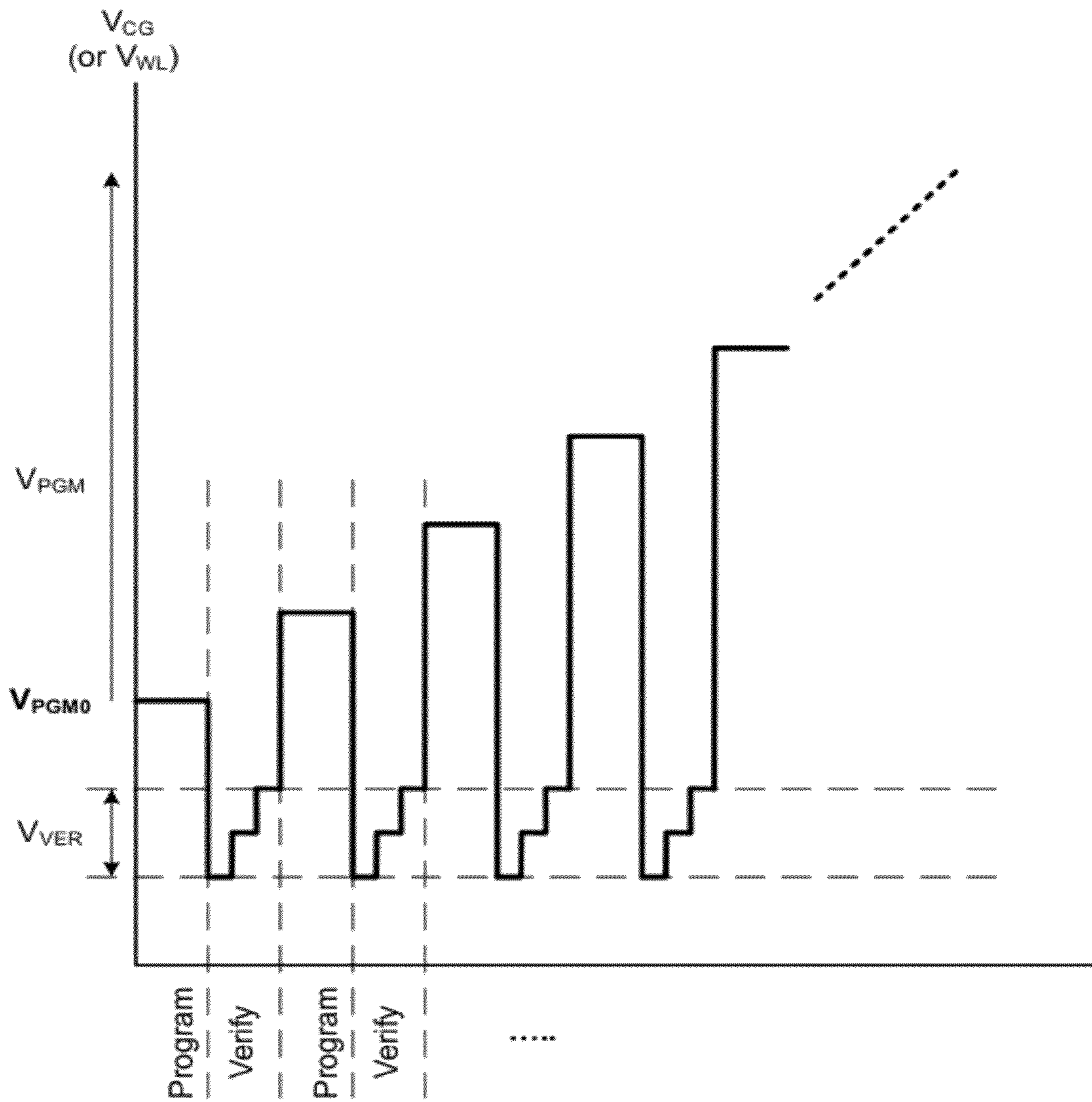
Convention Programming with alternate Program/Verify sequence
