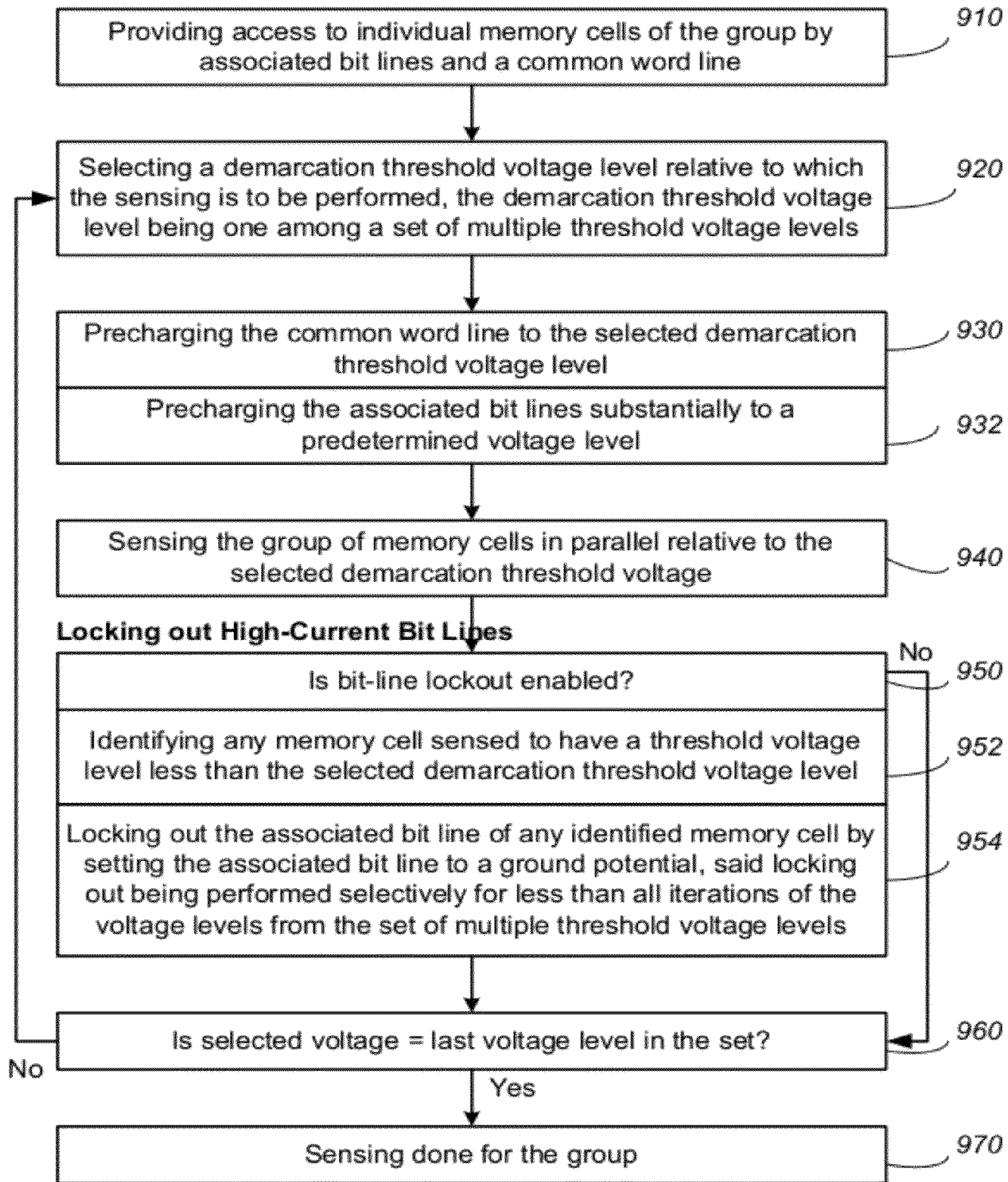
Sensing with Bit-line Lockout Control
