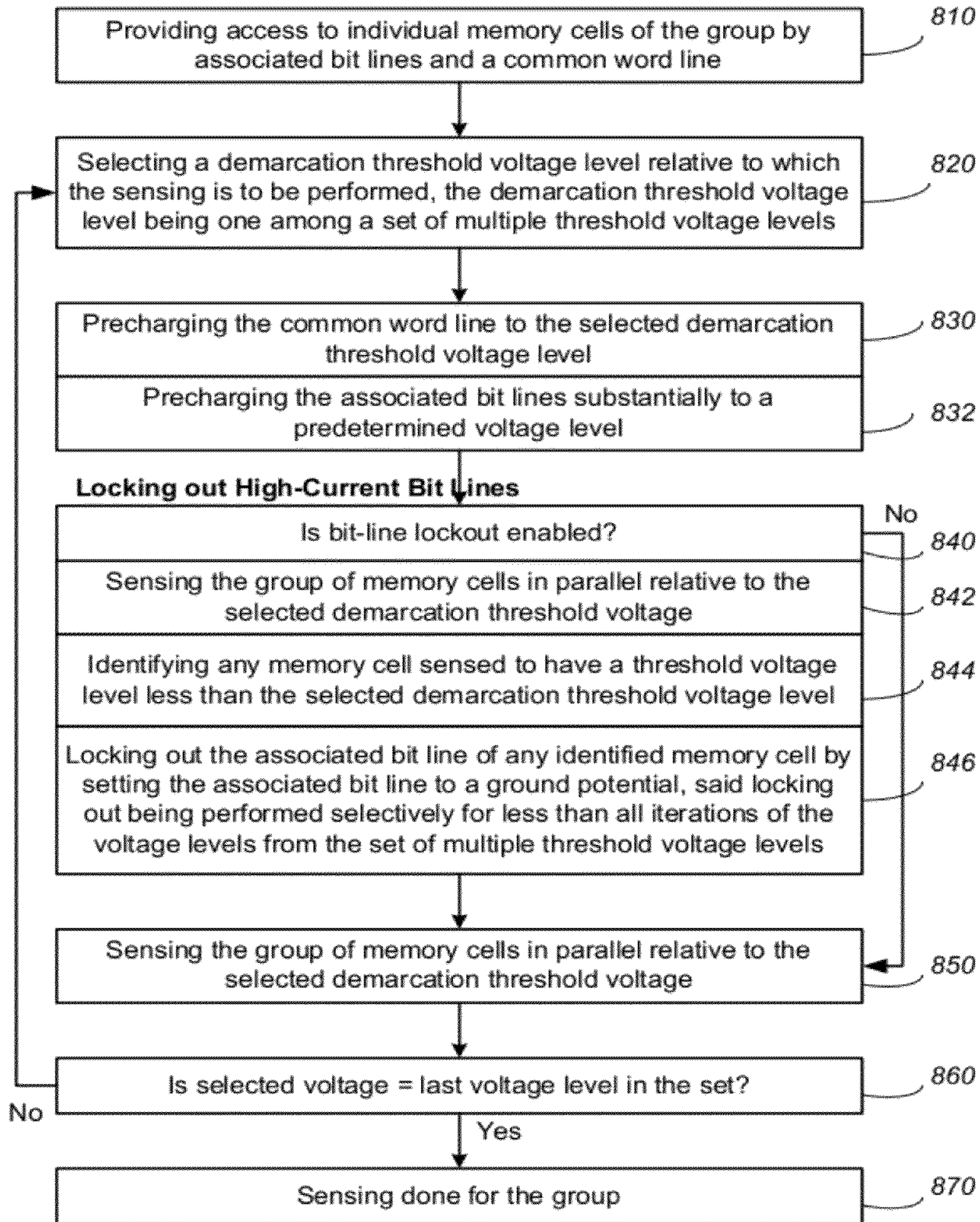
Sensing with Bit-line Lockout Control
