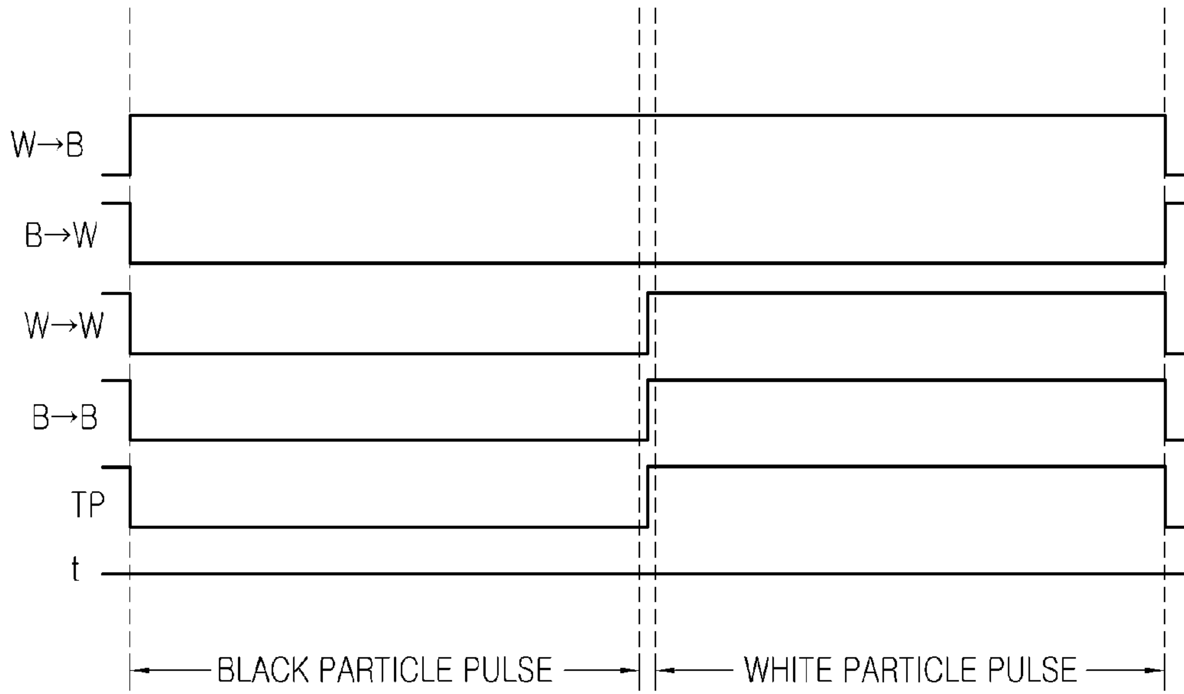
FIG.5 (PRIOR ART)
