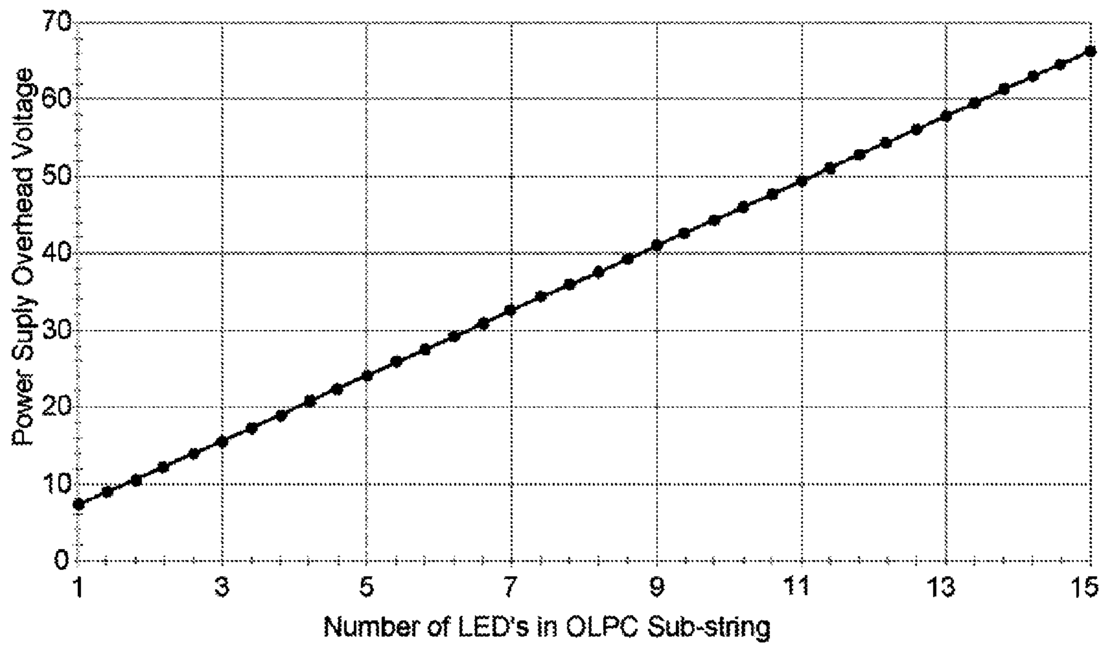
Power Supply Overhead Voltage required for number of LED's in Sub-String with q = 1 .
