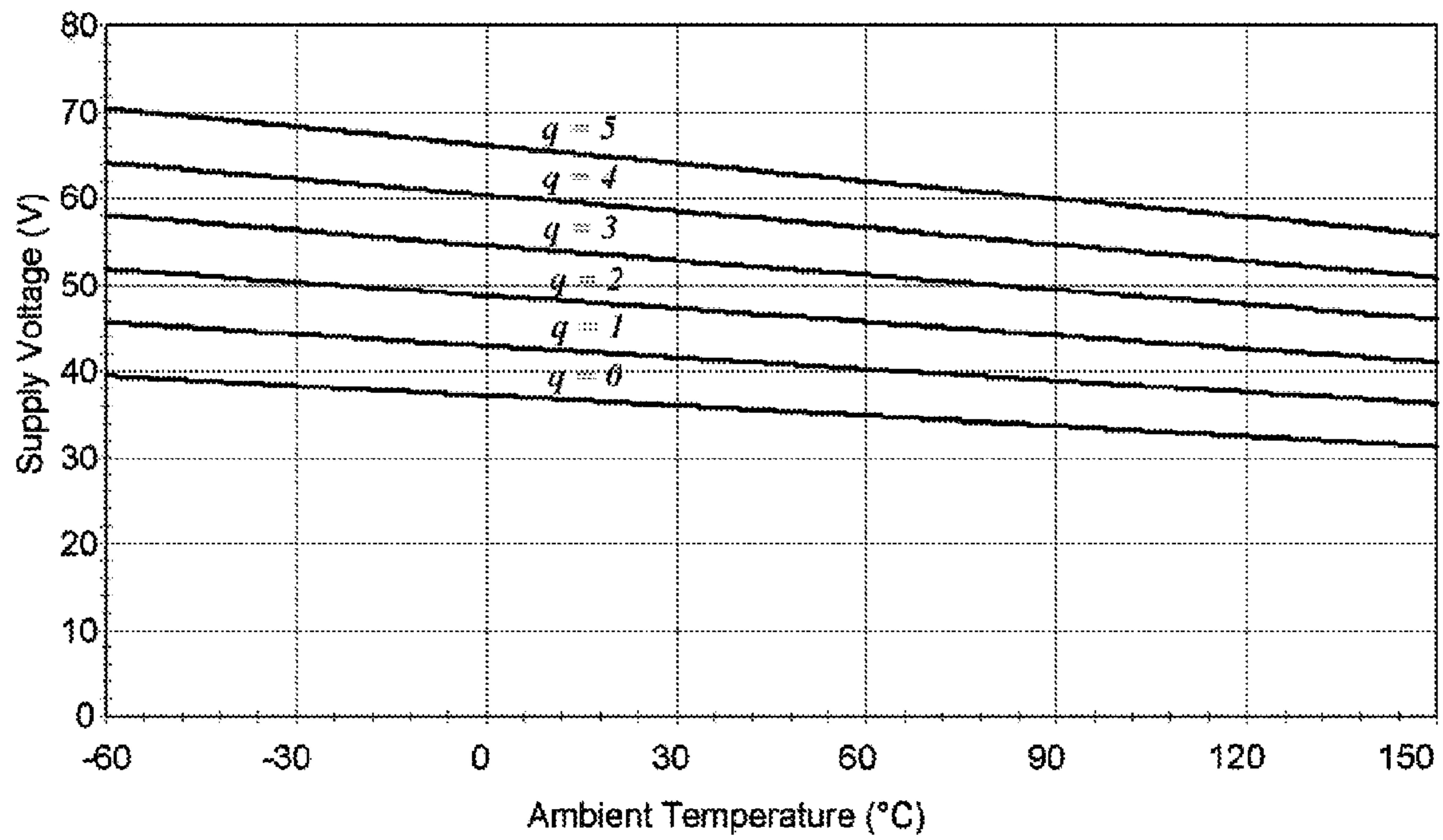
LED Required Supply Voltage ( V_{supply} ) when m = 10 , p = 1 , and 0 \leq q \leq 5 .
