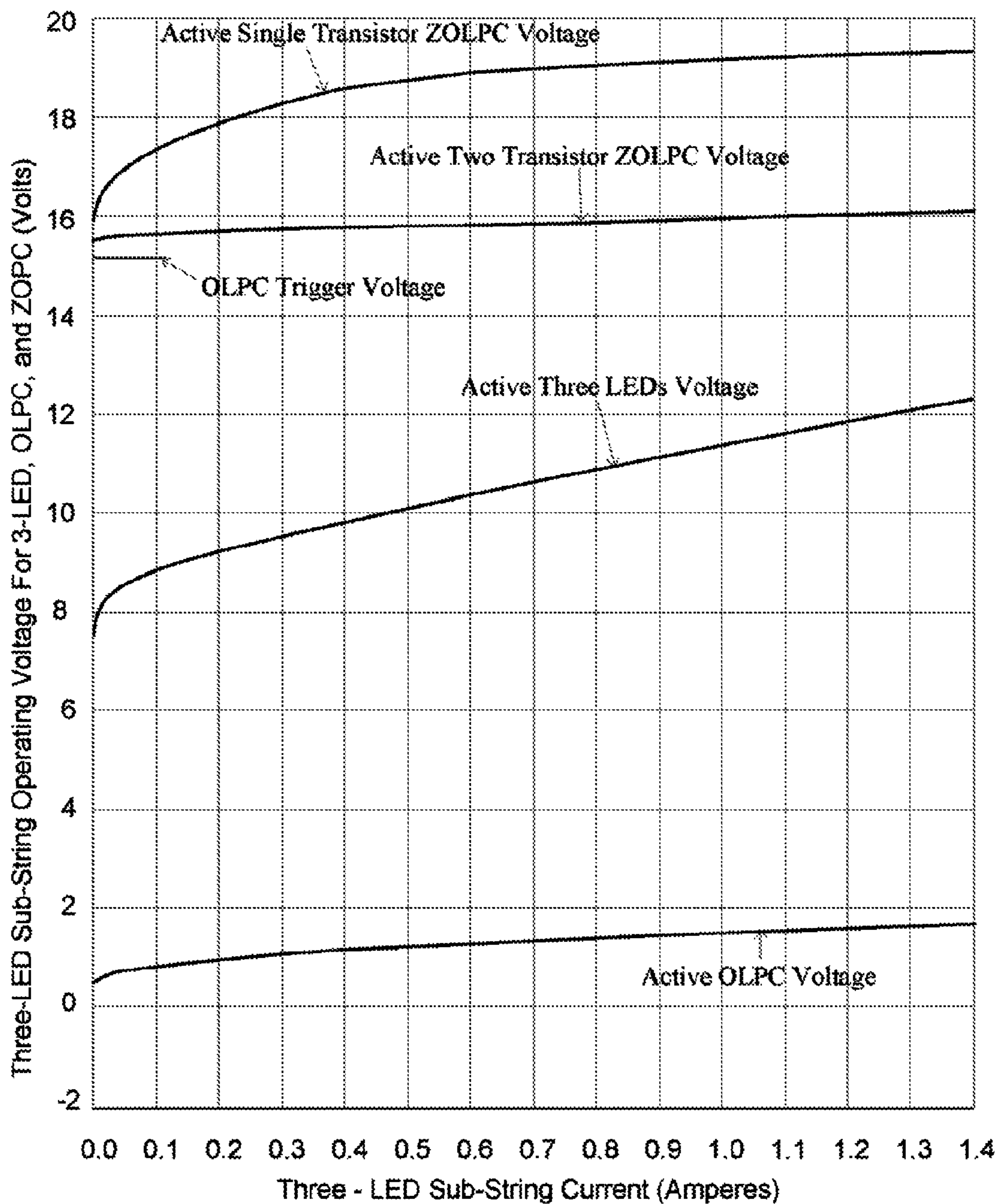
Three - LED Sub-String For Active 3-LED's, OLPC, and ZOLPC Voltages versus Current
