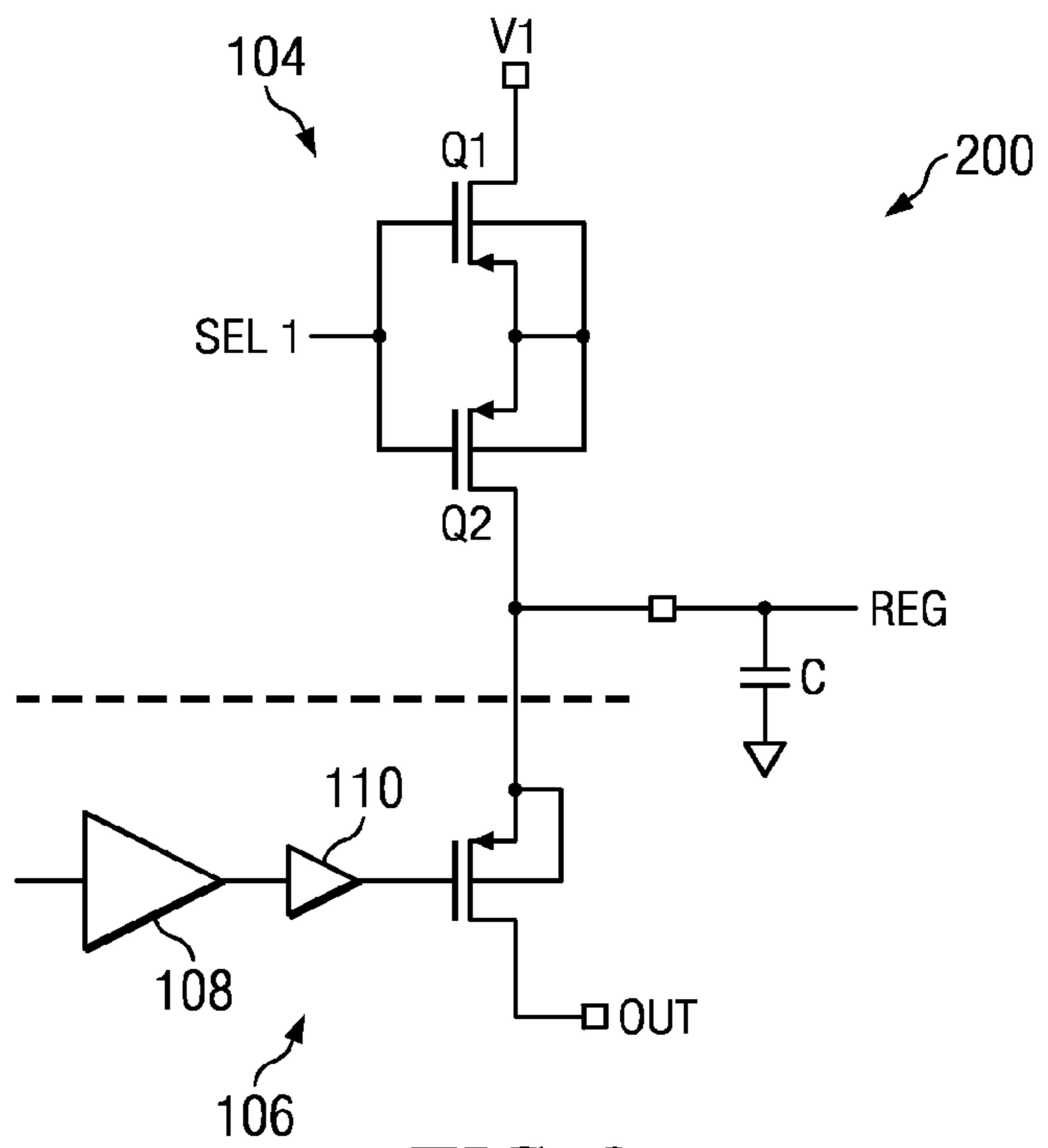
FIG. 2 (PRIOR ART)
