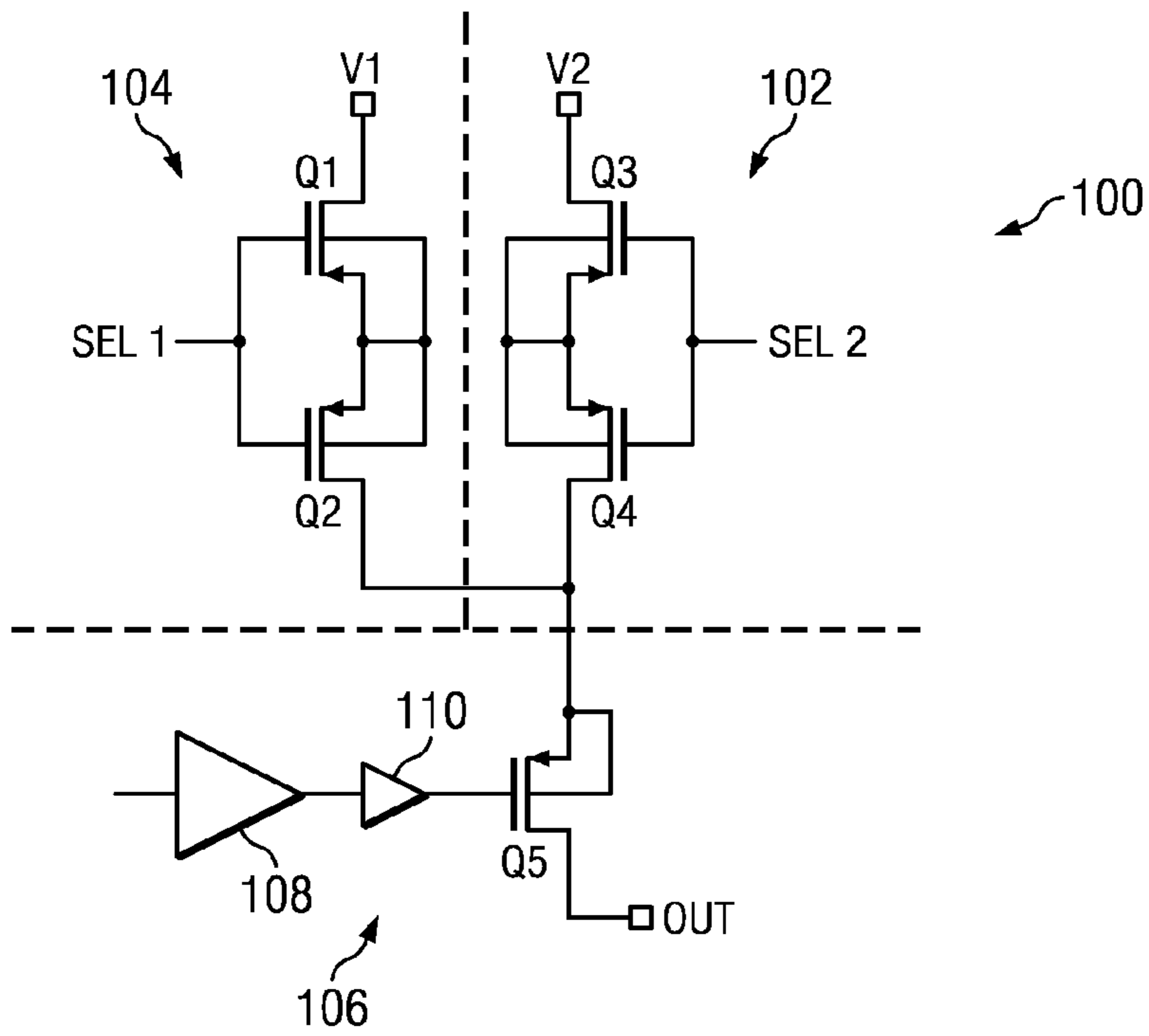
FIG. 1 (PRIOR ART)
