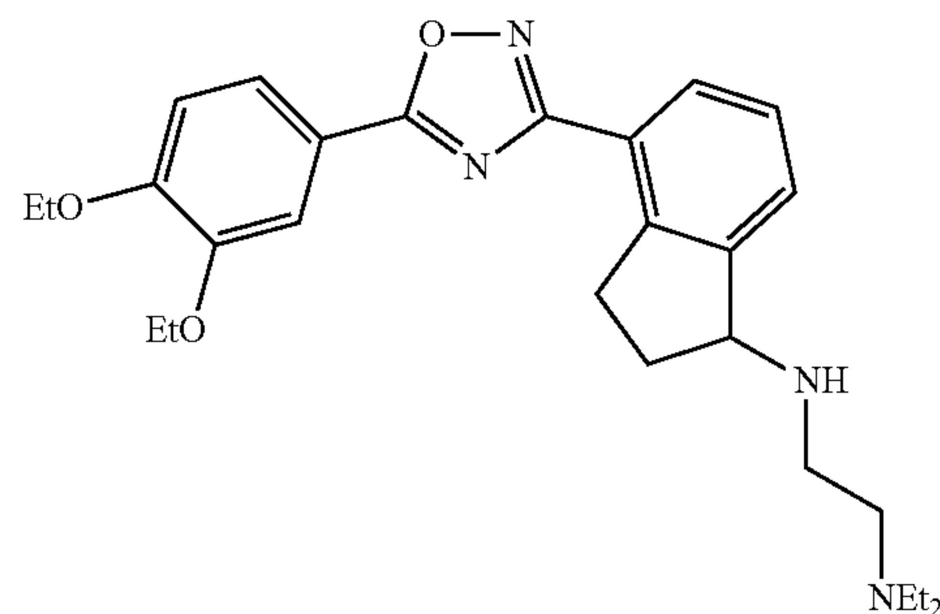
N1-(4-(5-(3,4-diethoxyphenyl)-1,2,4-oxadiazol-3-yl)-2,3-dihydro-1H-inden-1-yl)-N2,N2-diethylethane-1,2-diamine
