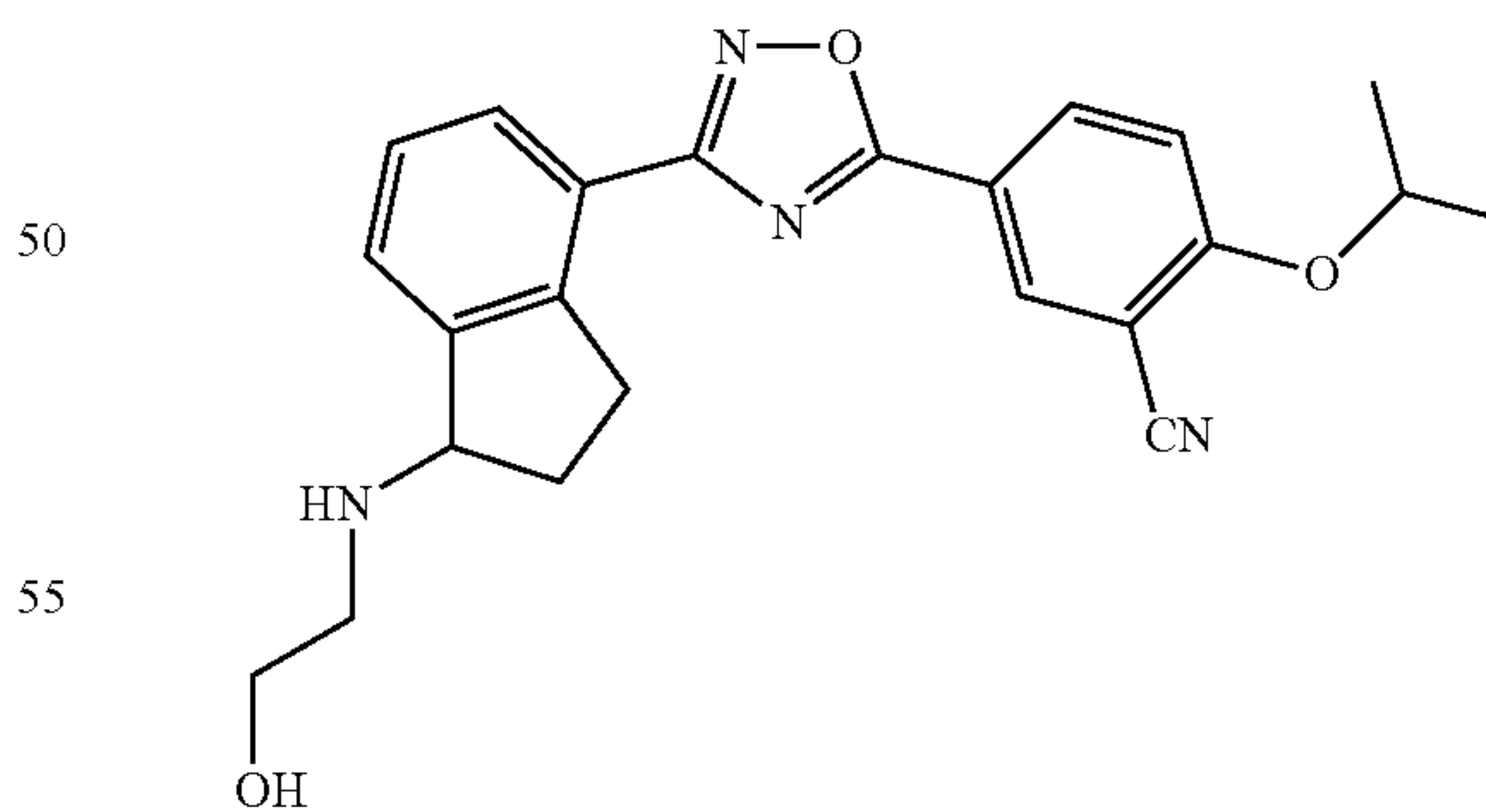
5-(3-(1-(2-hydroxyethylamino)-2,3-dihydro-1H-inden-4-yl)-1,2,4-oxadiazol-5-yl)-2-isopropoxybenzonitrile
