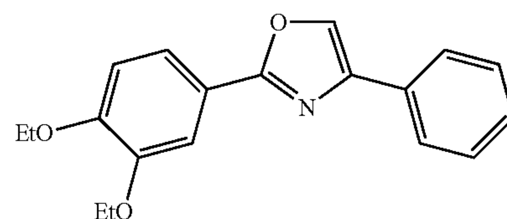
2-(3,4-diethoxyphenyl)-4-phenyloxazole
