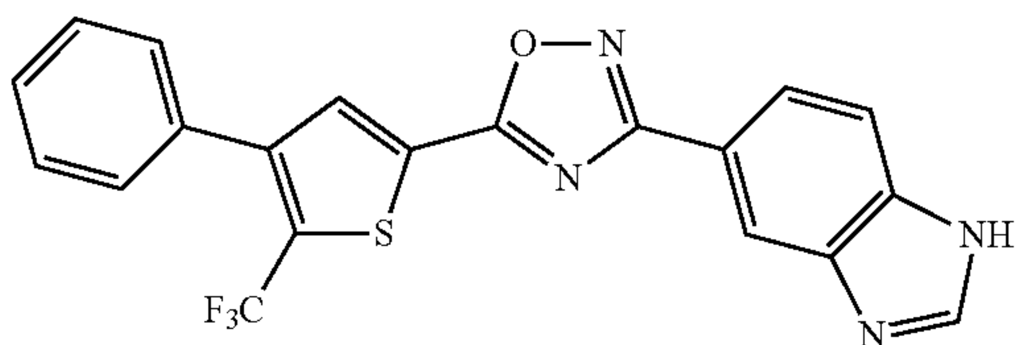
3-(1H-benzo[d]imidazol-5-yl)-5-(4-phenyl-5-(trifluoromethyl)thiophen-2-yl)-1,2,4-oxadiazole
