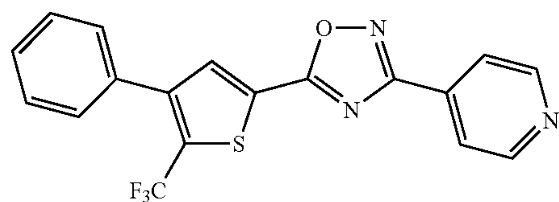
4-[5-(4-Phenyl-5-trifluoromethyl-thiophen-2-yl)-[1,2,4]oxadiazol-3-yl]-pyridine
