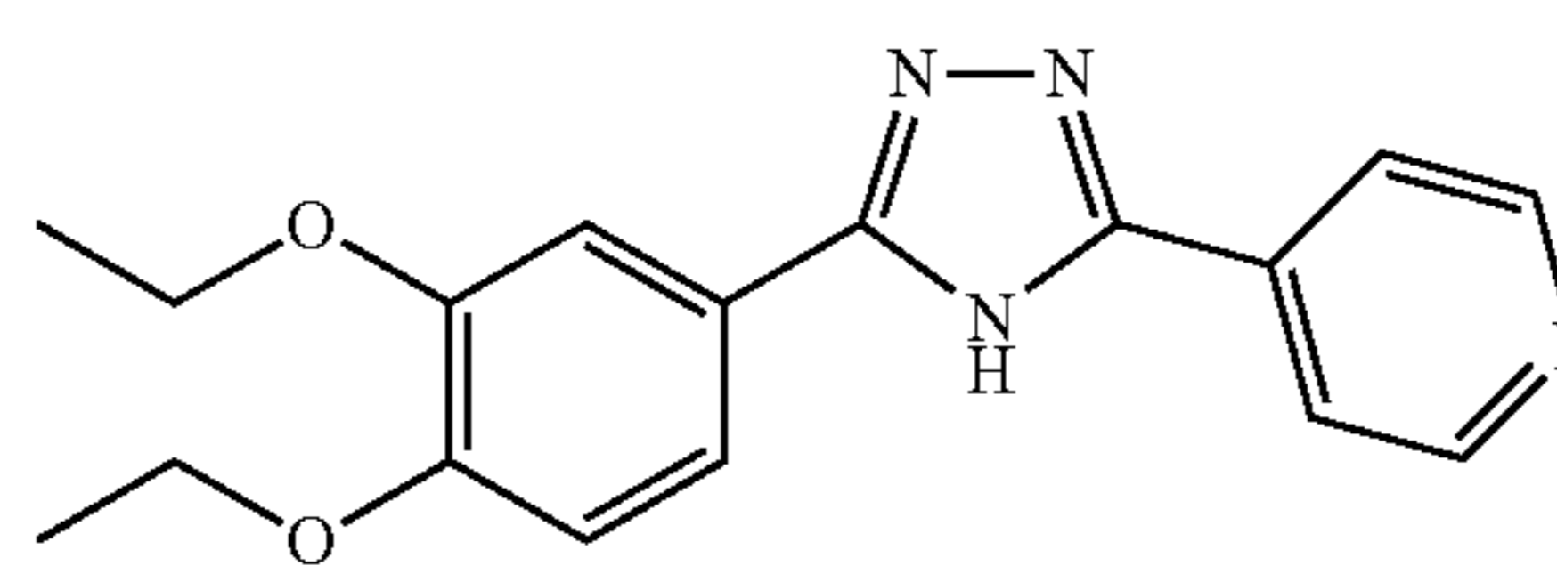
4-(5-(3,4-diethoxyphenyl)-4H-1,2,4-triazol-3-yl)pyridine
