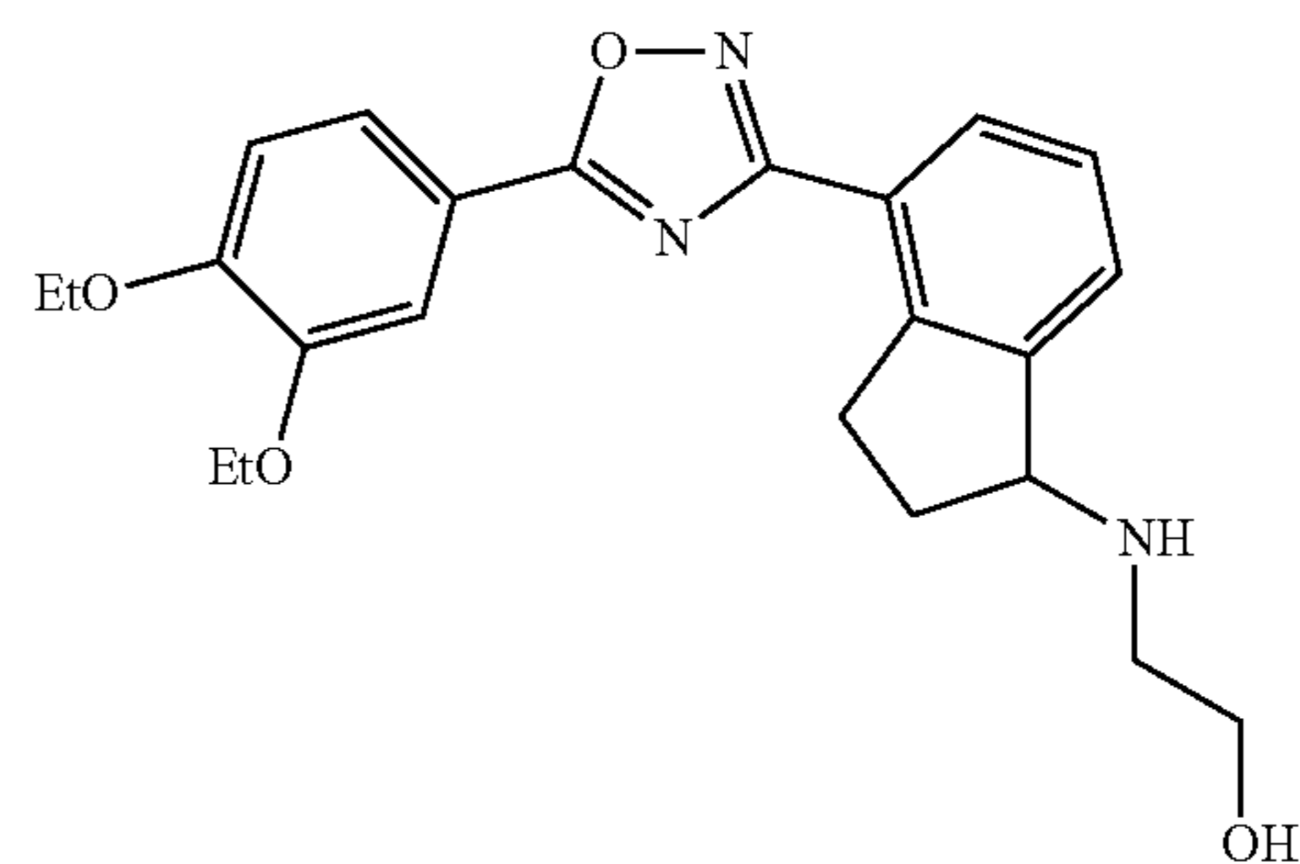
2-(4-(5-(3,4-diethoxyphenyl)-1,2,4-oxadiazol-3-yl)-2,3-dihydro-1H-inden-1-ylamino)ethanol
