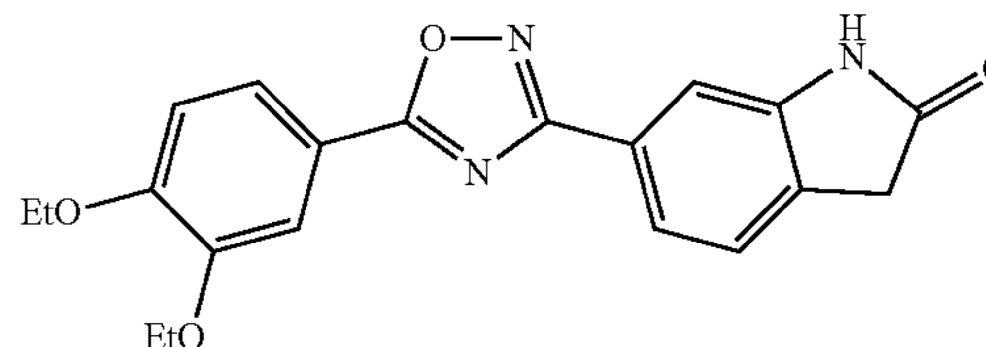
6-(5-(3,4-diethoxyphenyl)-1,2,4-oxadiazol-3-yl)indolin-2-one
