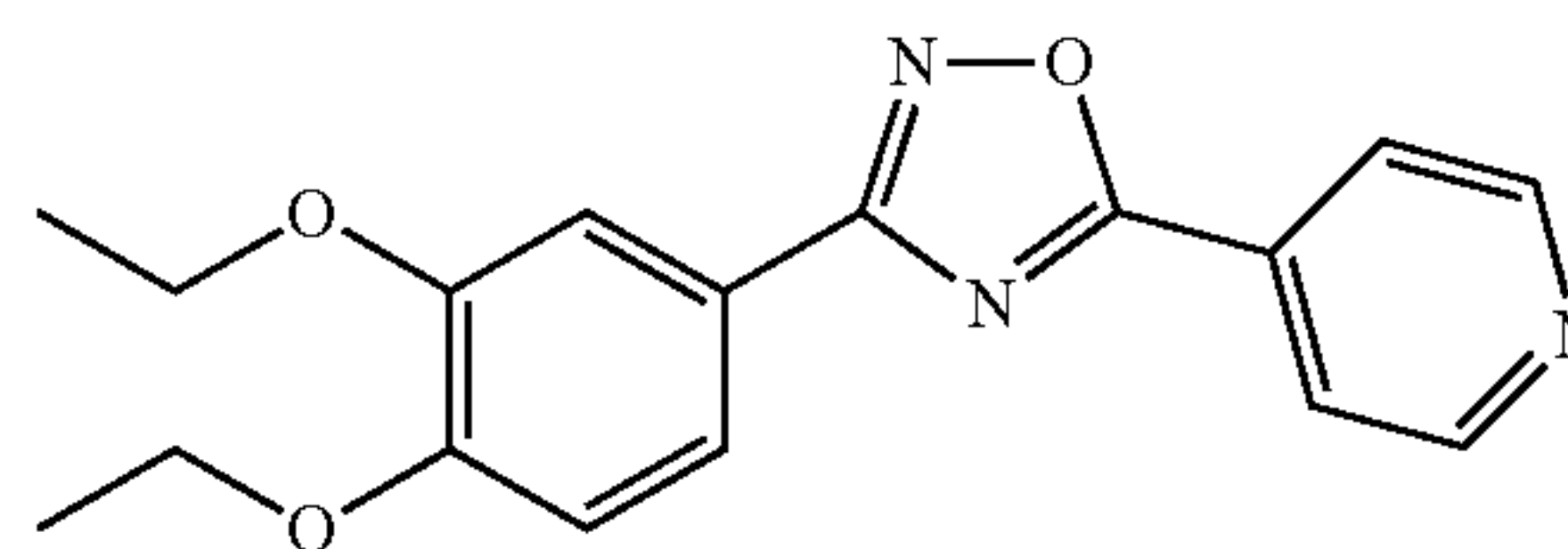
3-(3,4-diethoxyphenyl)-5-(pyridin-4-yl)-1,2,4-oxadiazole
