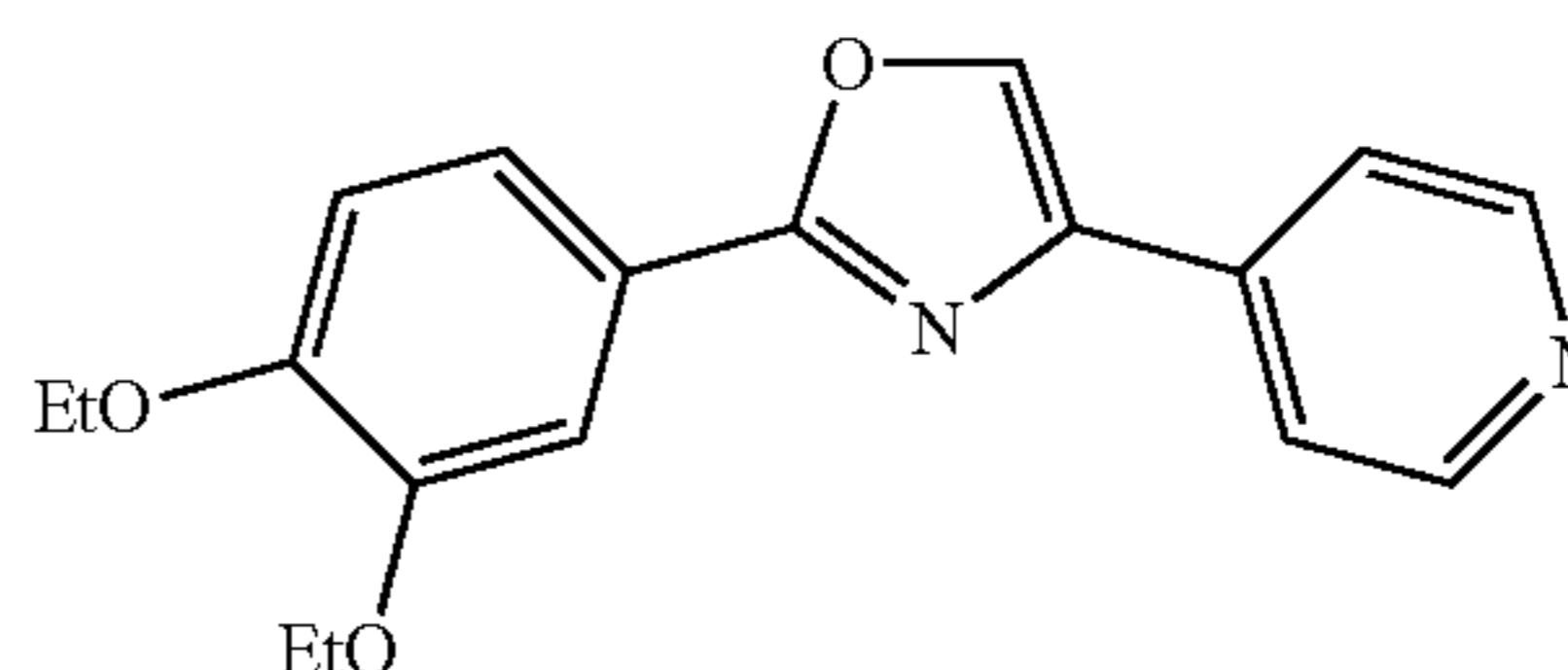
2-(3,4-diethoxyphenyl)-4-(pyridin-4-yl)oxazole
