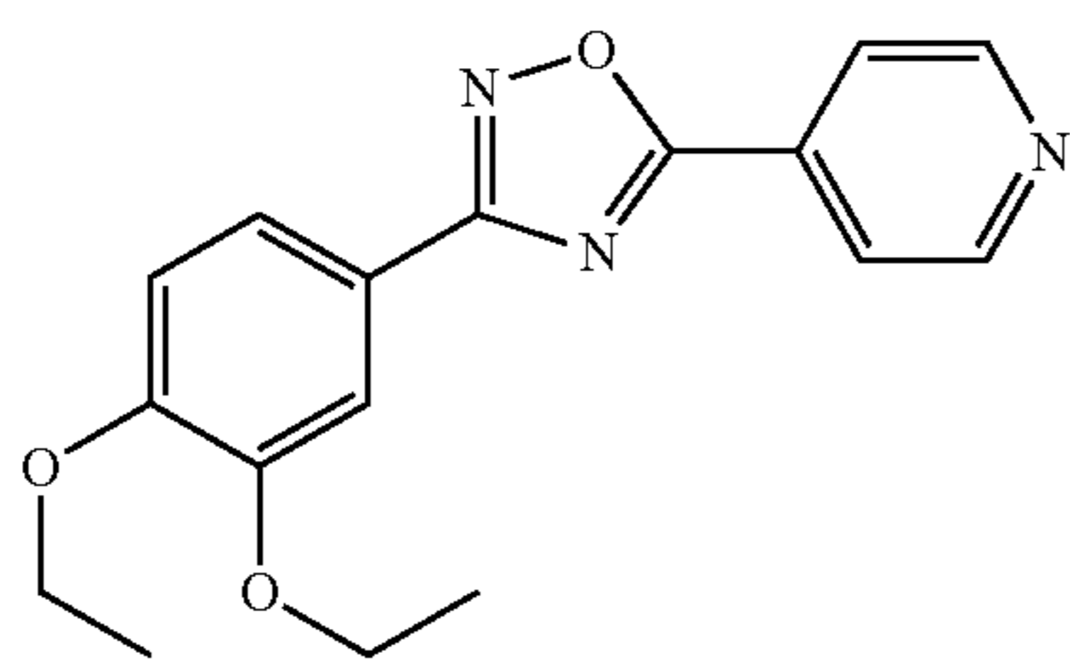
3-(3,4-diethoxyphenyl)-5-(pyridin-4-yl)-1,2,4-oxadiazole
