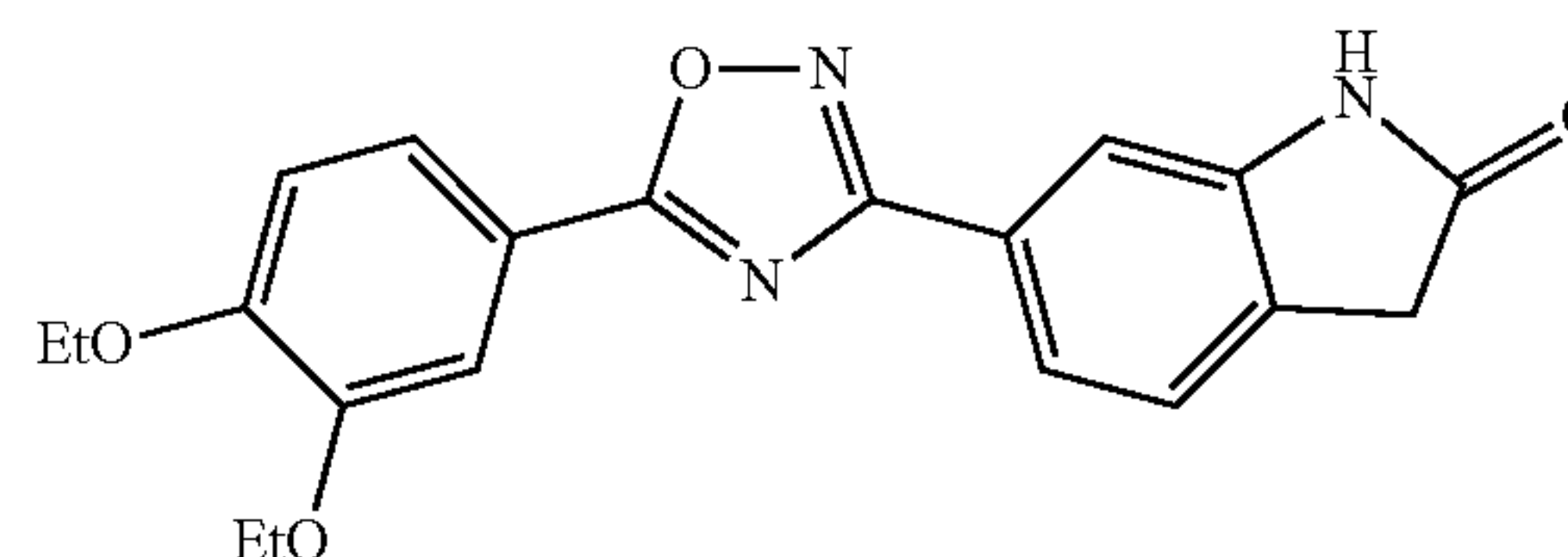
6-(5-(3,4-diethoxyphenyl)-1,2,4-oxadiazol-3-yl)indolin-2-one
