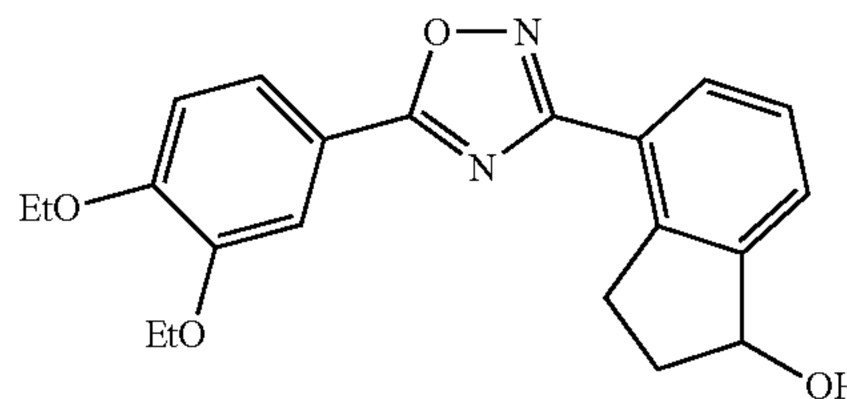
4-(5-(3,4-diethoxyphenyl)-1,2,4-oxadiazol-3-yl)-2,3-dihydro-1H-inden-1-ol
