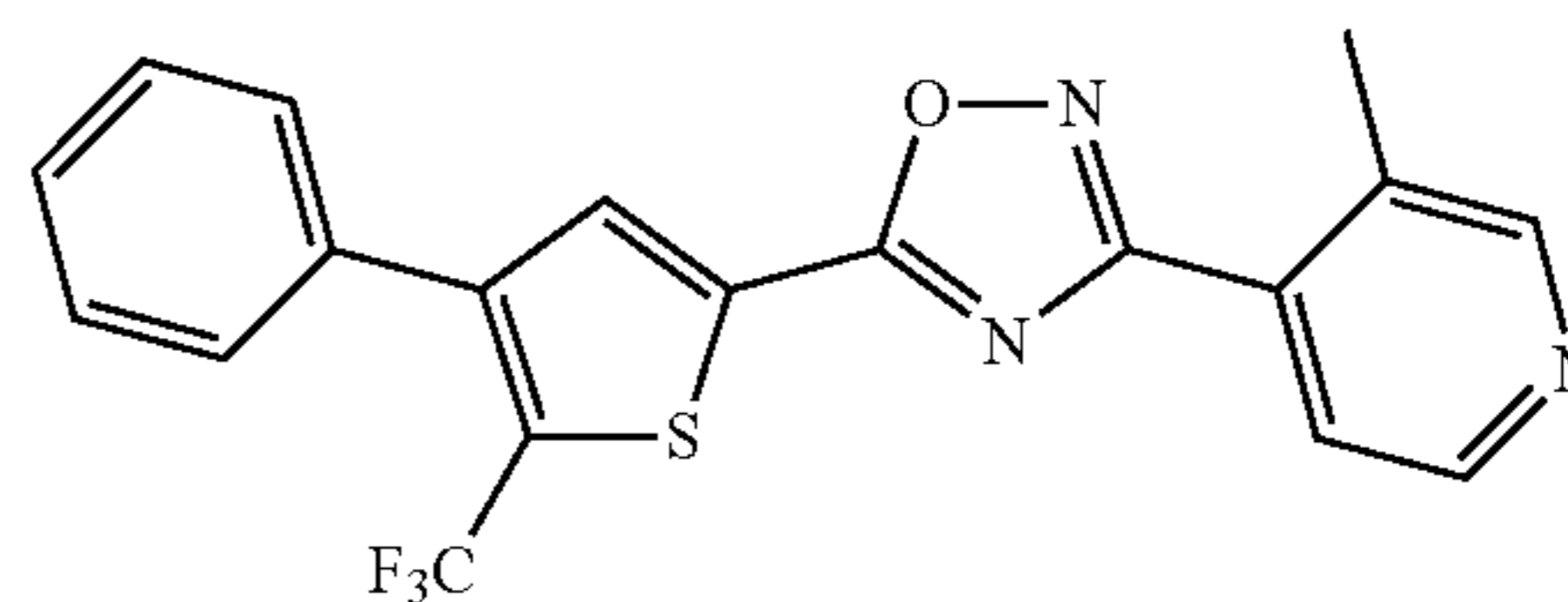
3-(3-methylpyridin-4-yl)-5-(4-phenyl-5-(trifluoromethyl)thiophen-2-yl)-1,2,4-oxadiazole
