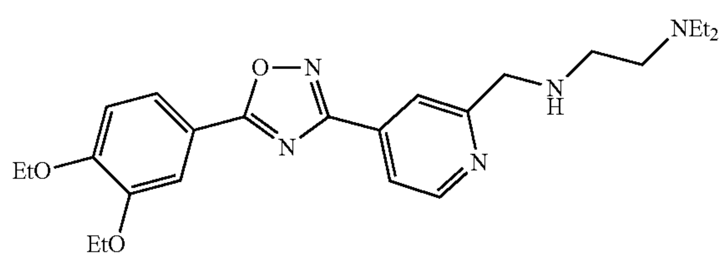
N1-((4-(5-(3,4-diethoxyphenyl)-1,2,4-oxadiazol-3-yl)pyridin-2-yl)methyl)-N2,N2-diethylethane-1,2-diamine
