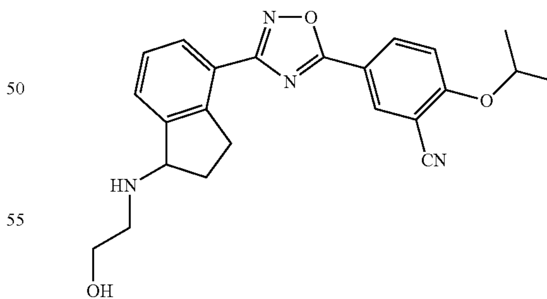
5-(3-(1-(2-hydroxyethylamino)-2,3-dihydro-1H-inden-4-yl)-1,2,4-oxadiazol-5-yl)-2-isopropoxybenzonitrile
