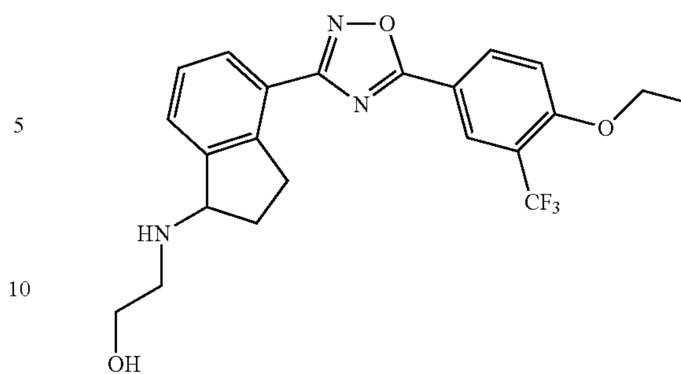
2-(4-(5-(4-ethoxy-3-(trifluoromethyl)phenyl)-1,2,4-oxadiazol-3-yl)-2,3-dihydro-1H-inden-1-ylamino)ethanol
