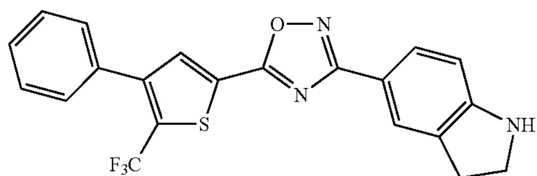
3-(indolin-5-yl)-5-(4-phenyl-5-(trifluoromethyl)thiophen-2-yl)-1,2,4-oxadiazole
