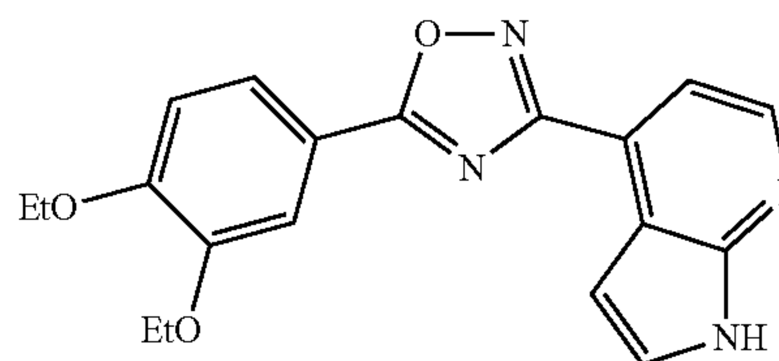
5-(3,4-diethoxyphenyl)-3-(1H-pyrrolo[2,3-b]pyridin-4-yl)-1,2,4-oxadiazole
