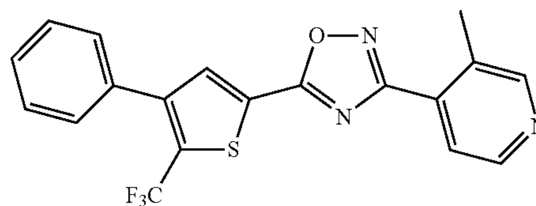
3-(3-methylpyridin-4-yl)-5-(4-phenyl-5-(trifluoromethyl)thiophen-2-yl)-1,2,4-oxadiazole
