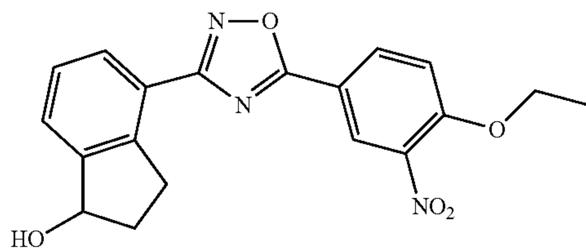
4-(5-(4-ethoxy-3-nitrophenyl)-1,2,4-oxadiazol-3-yl)- 2,3-dihydro-1H-inden-1-ol
