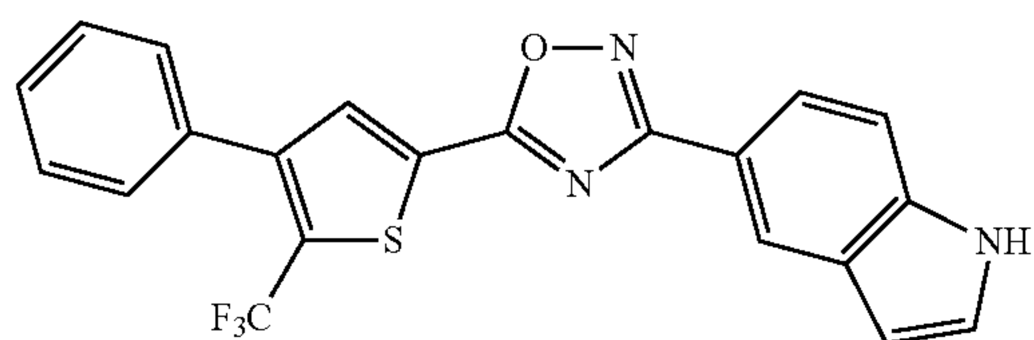
3-(1H-indol-5-yl)-5-(4-phenyl-5-(trifluoromethyl)thiophen-2-yl)-1,2,4-oxadiazole
