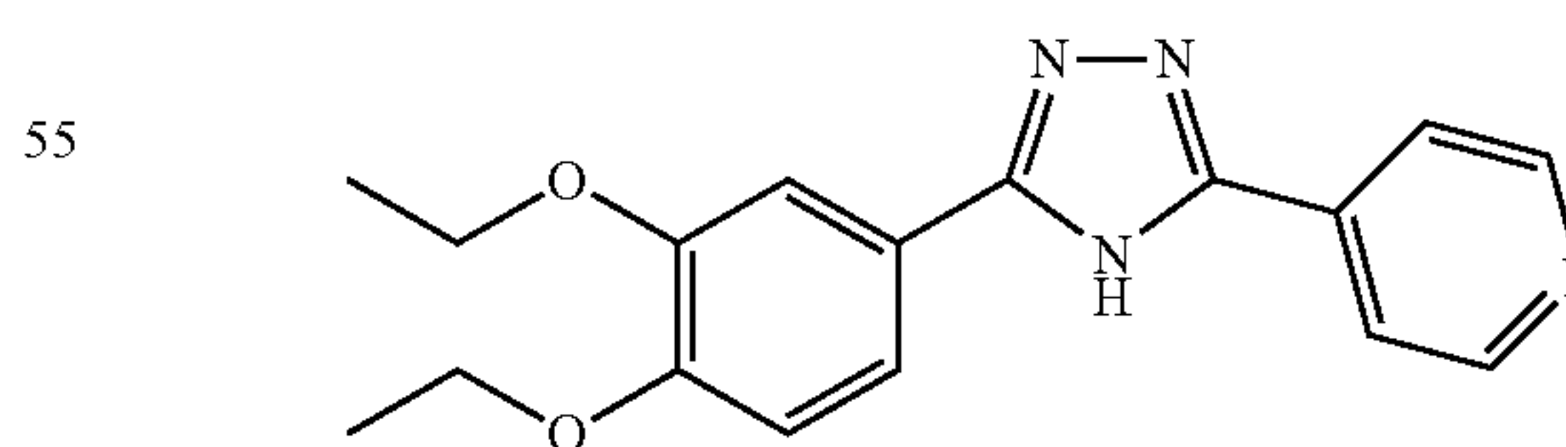
4-(5-(3,4-diethoxyphenyl)-4H-1,2,4-triazol-3-yl)pyridine
