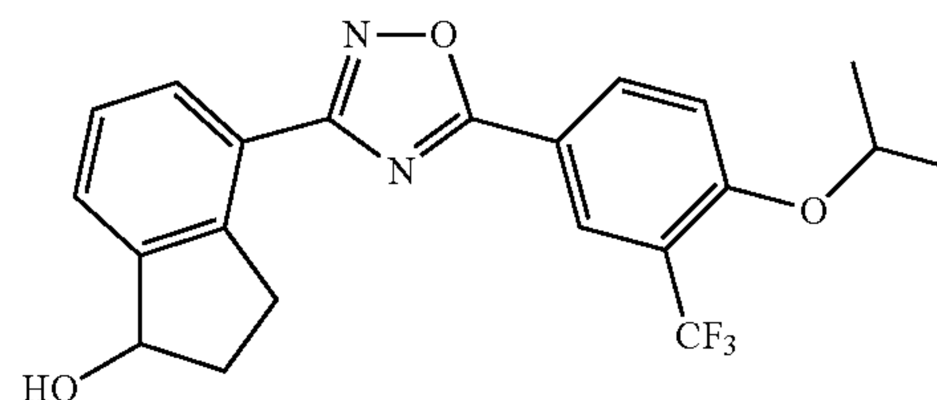
4-(5-(4-isopropoxy-3-(trifluoromethyl)phenyl)-1,2,4-oxadiazol-3-yl)-2,3-dihydro-1H-inden-1-ol
