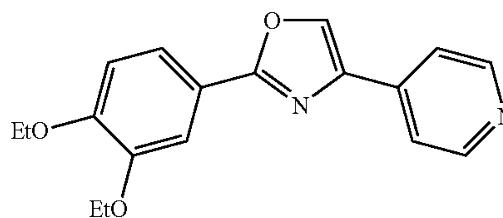
2-(3,4-diethoxyphenyl)-4-(pyridin-4-yl)oxazole
