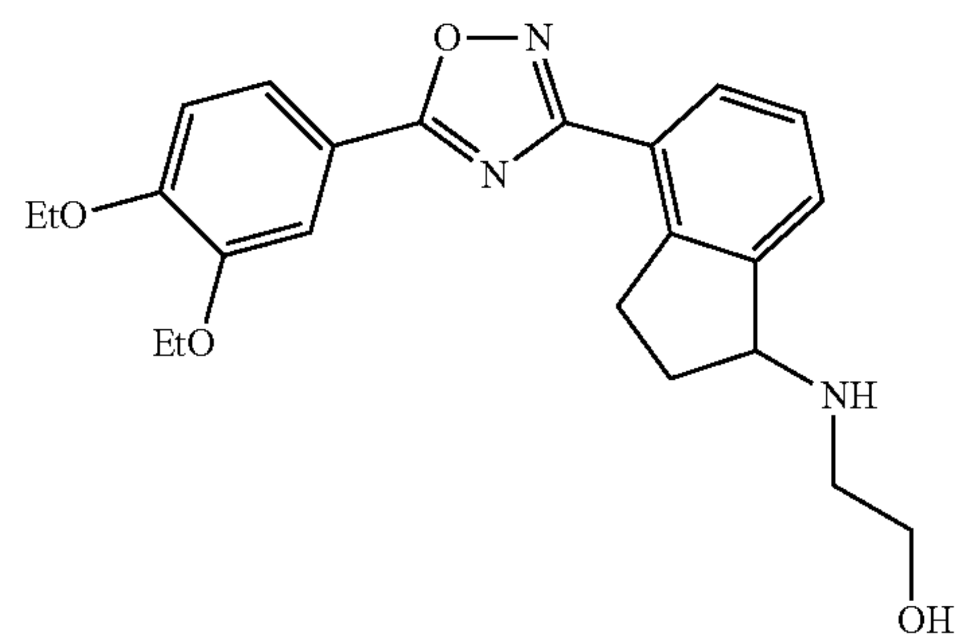
2-(4-(5-(3,4-diethoxyphenyl)-1,2,4-oxadiazol-3-yl)-2,3-dihydro-1H-inden-1-ylamino)ethanol
