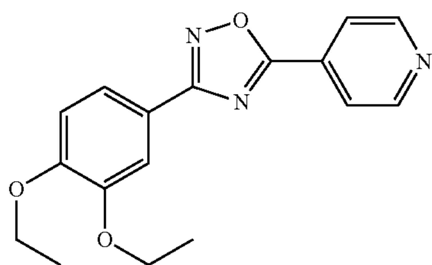
3-(3,4-diethoxyphenyl)-5-(pyridin-4-yl)-1,2,4-oxadiazole
