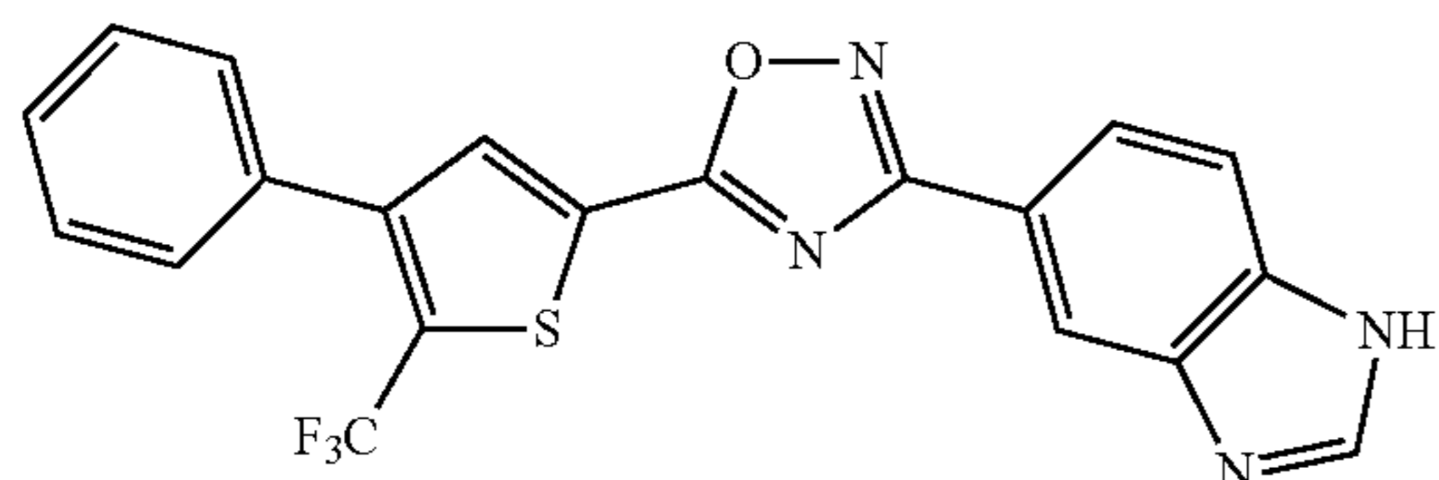
3-(1H-benzo[d]imidazol-5-yl)-5-(4-phenyl-5-(trifluoromethyl)thiophen-2-yl)-1,2,4-oxadiazole
