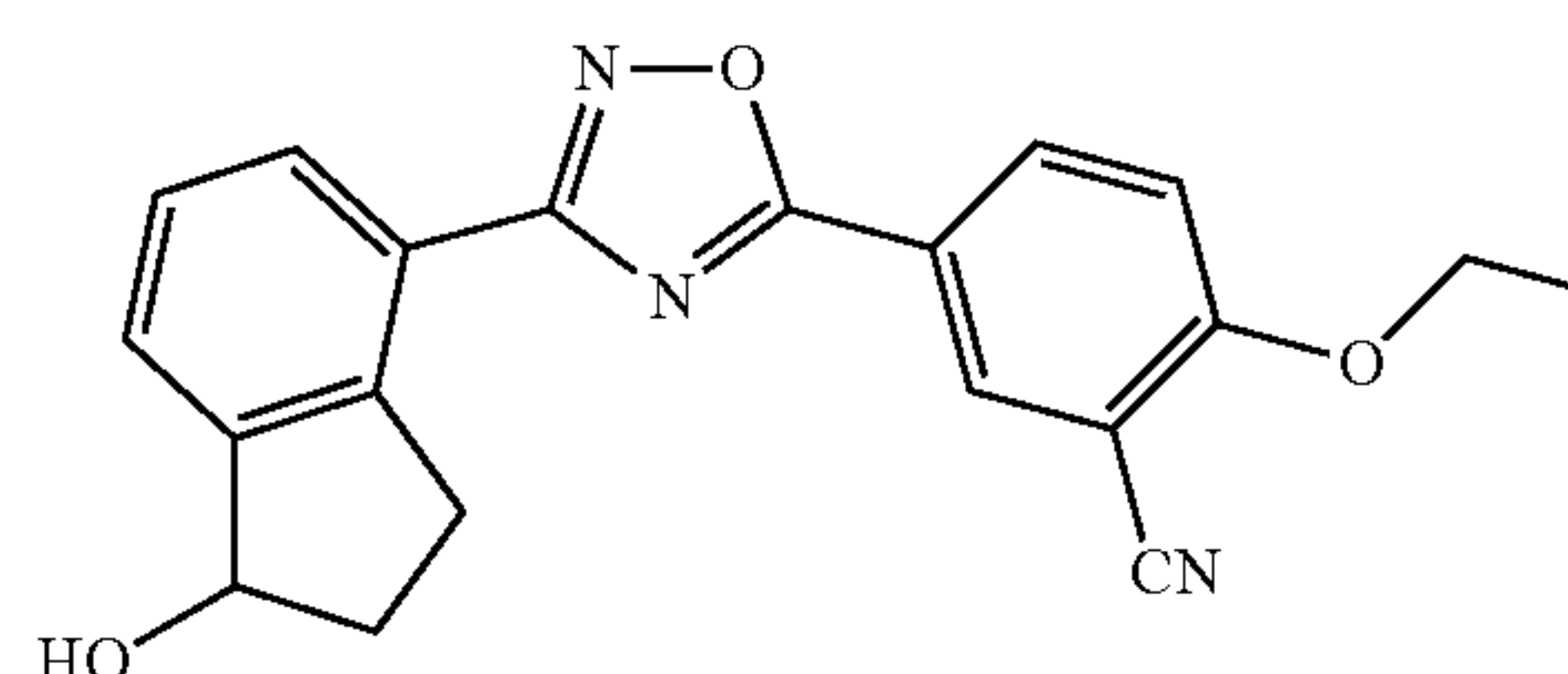
2-ethoxy-5-(3-(1-hydroxy-2,3-dihydro-1H-inden-4-yl)-1,2,4-oxadiazol-5-yl)benzonitrile
