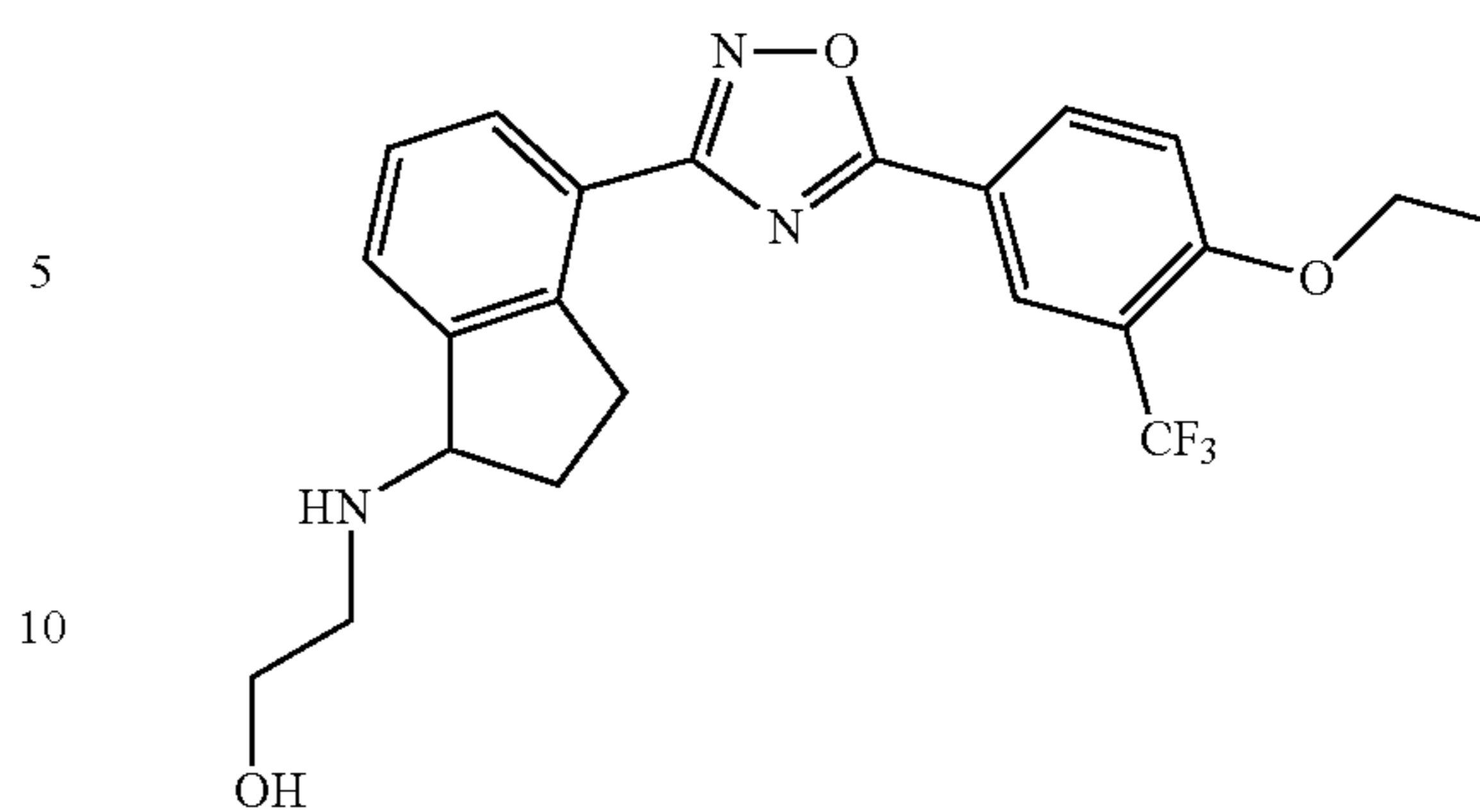
2-(4-(5-(4-ethoxy-3-(trifluoromethyl)phenyl)-1,2,4-oxadiazol-3-yl)-2,3-dihydro-1H-inden-1-ylamino)ethanol
