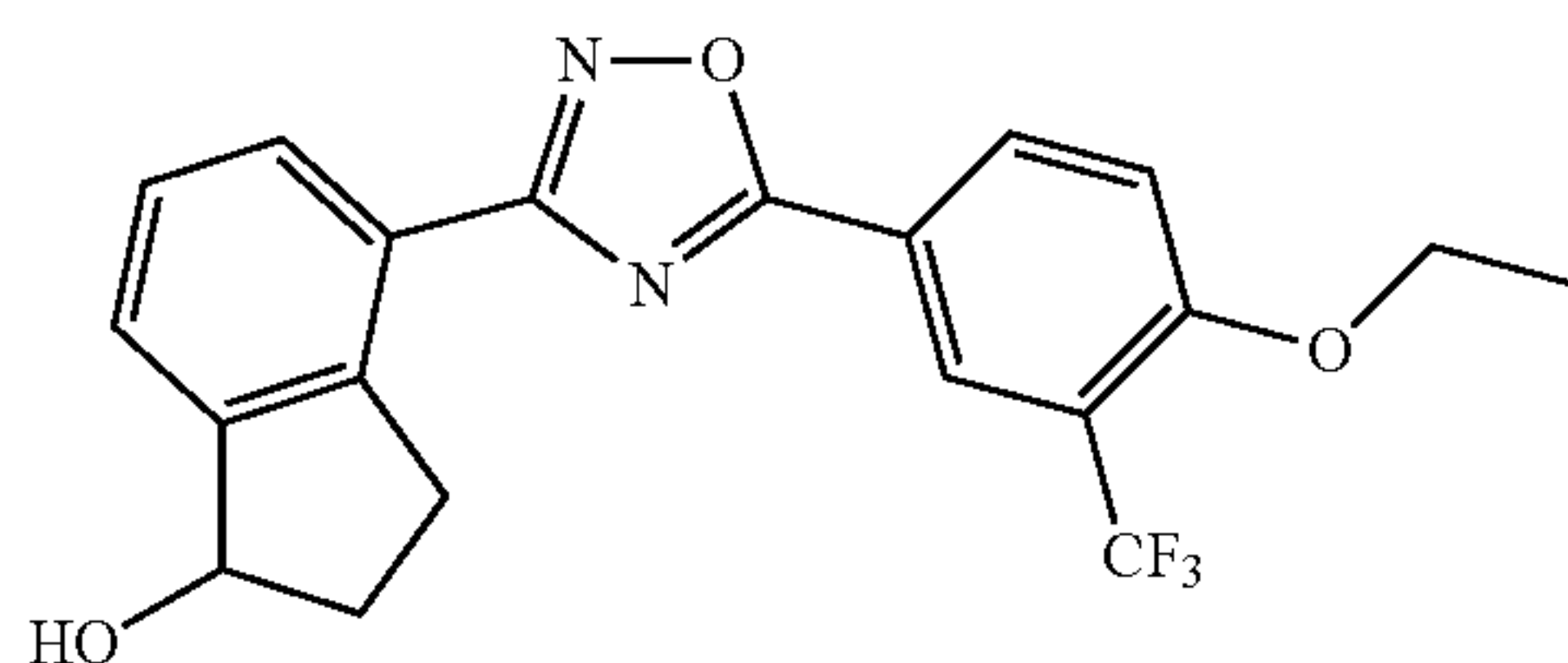
4-(5-(4-ethoxy-3-(trifluoromethyl)phenyl)-1,2,4-oxadiazol-3-yl)-2,3-dihydro-1H-inden-1-ol
