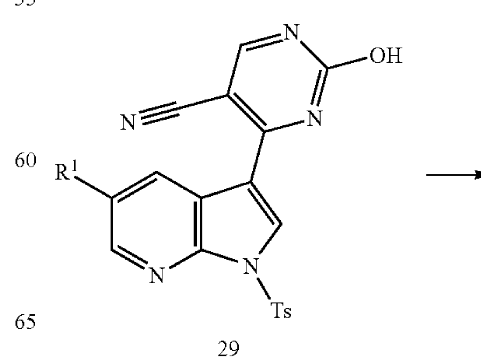
Scheme 12
