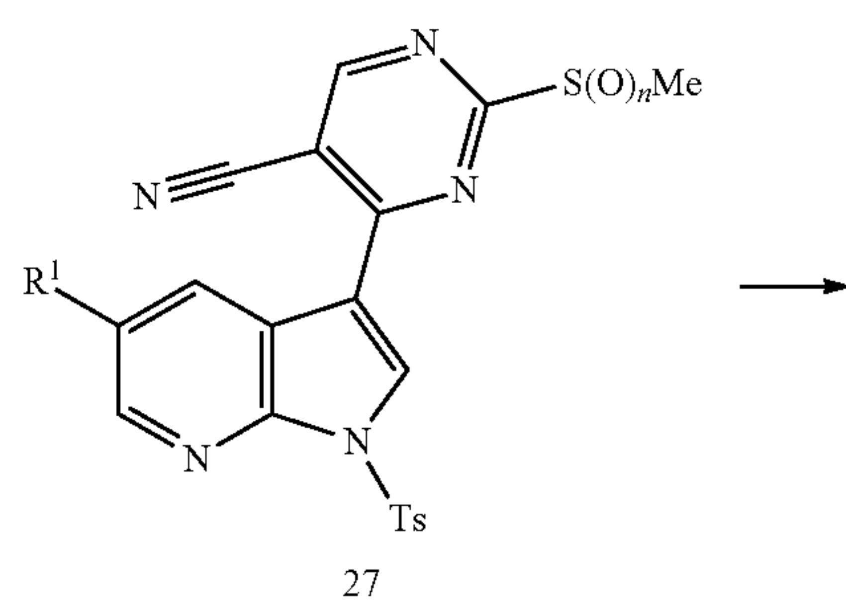
Scheme 11
