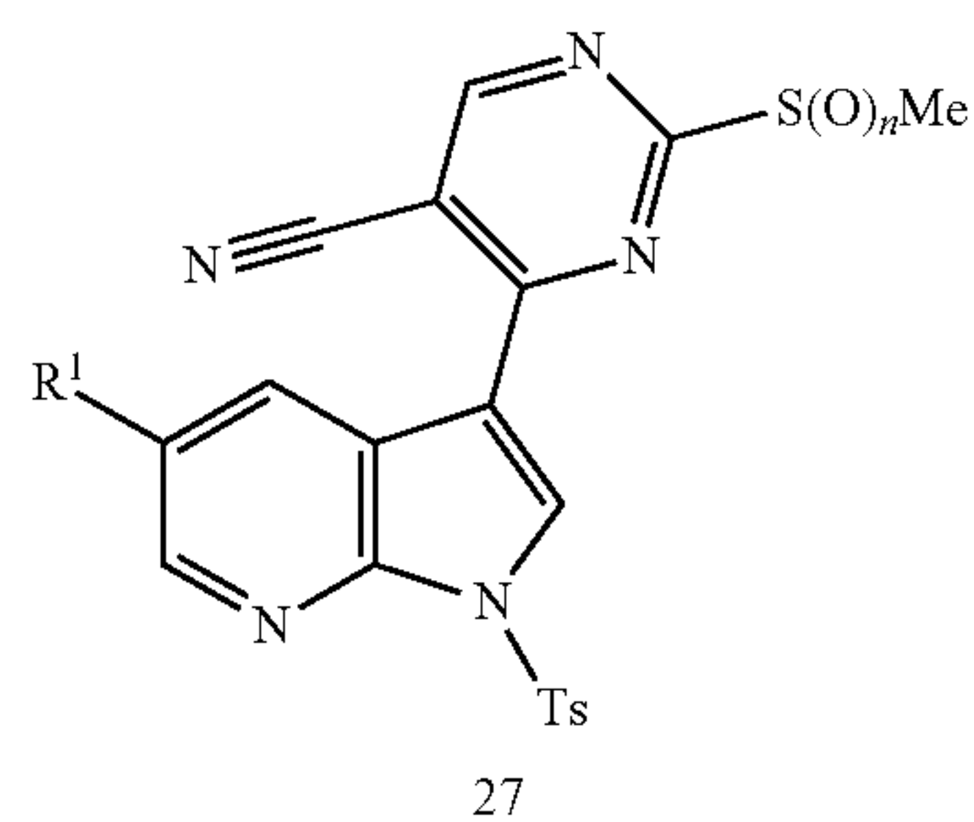
Scheme 7
