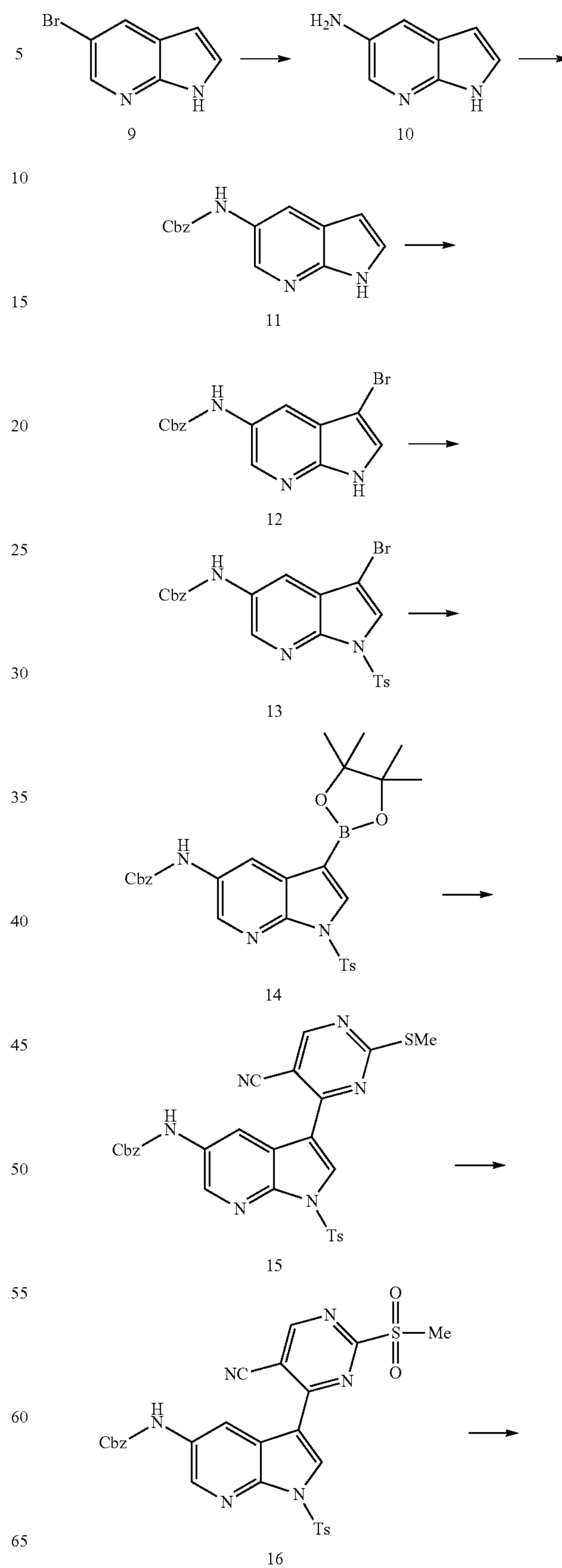
Scheme 4
