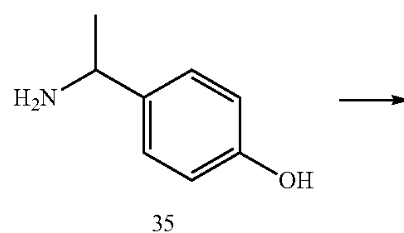
Scheme 9
