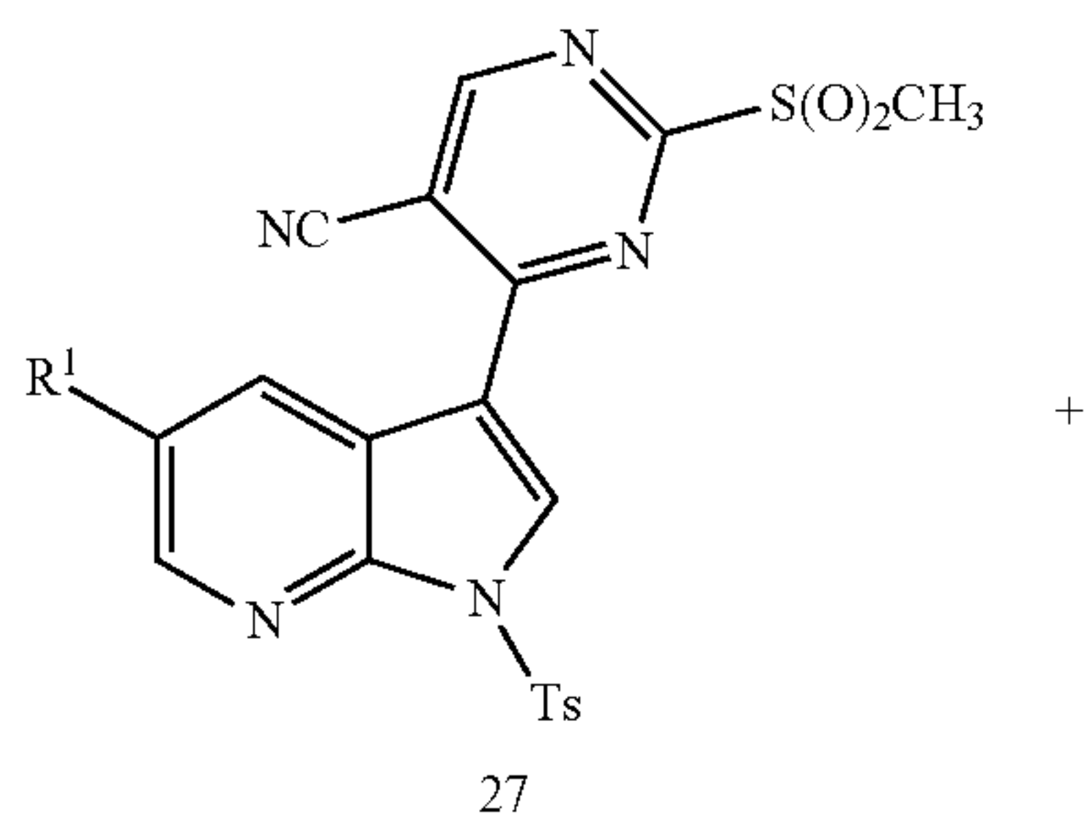
Scheme 8
