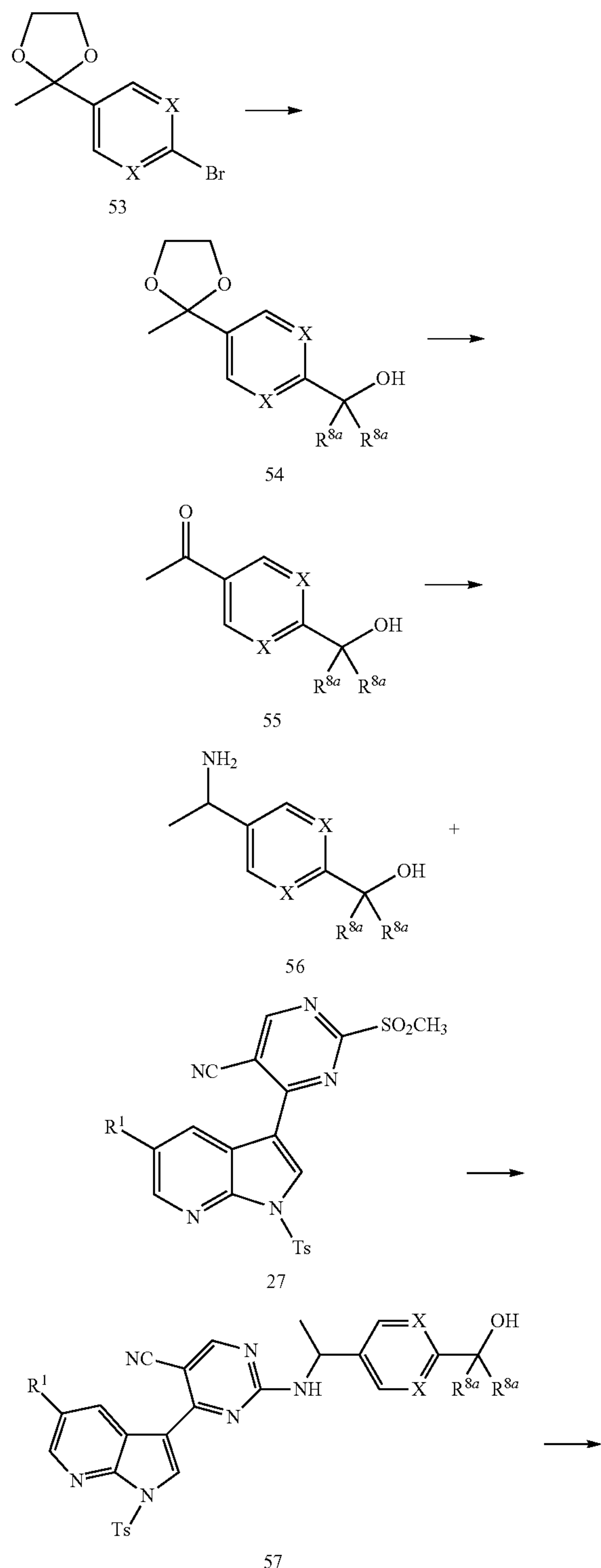
Scheme 14
