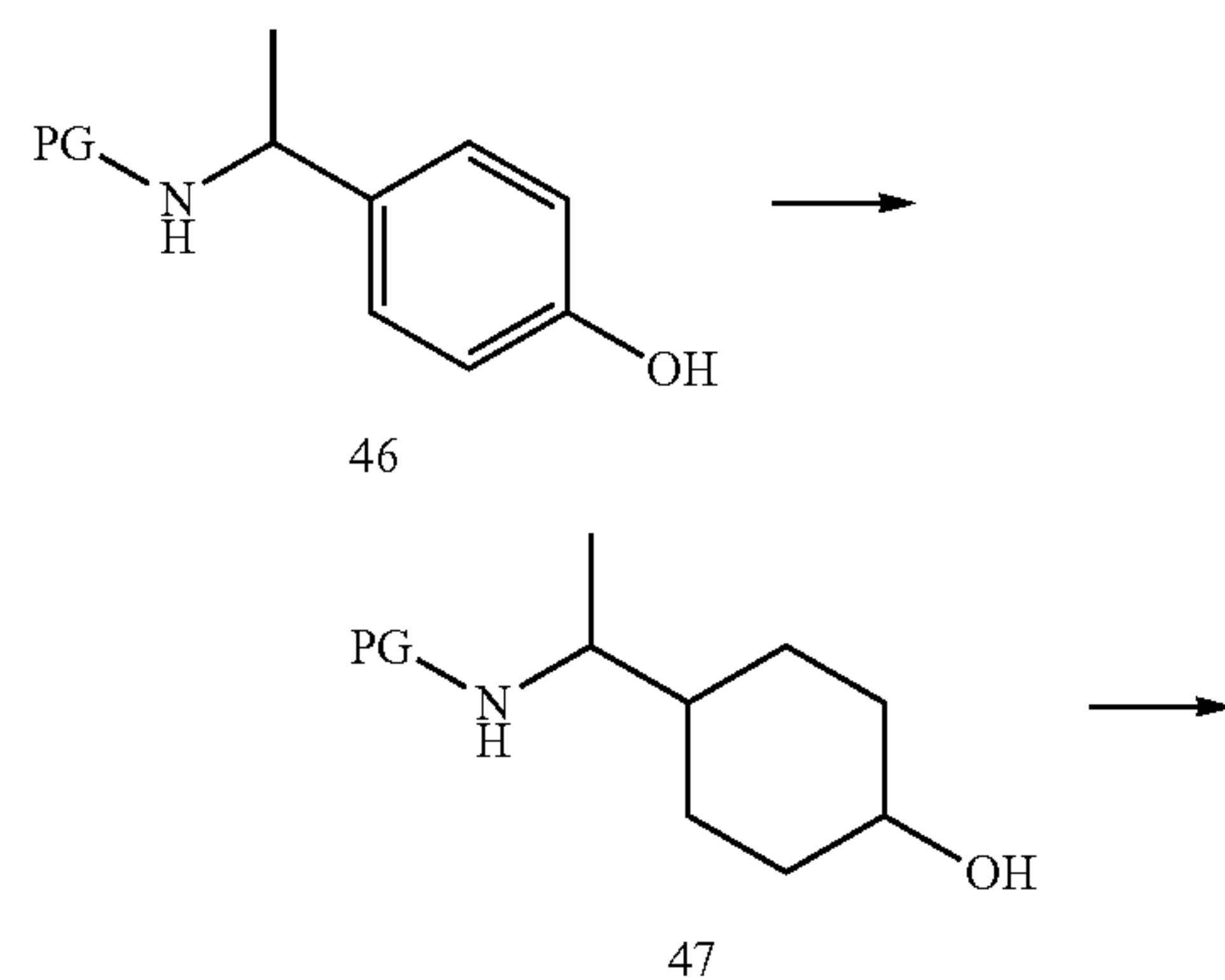
Scheme 13
