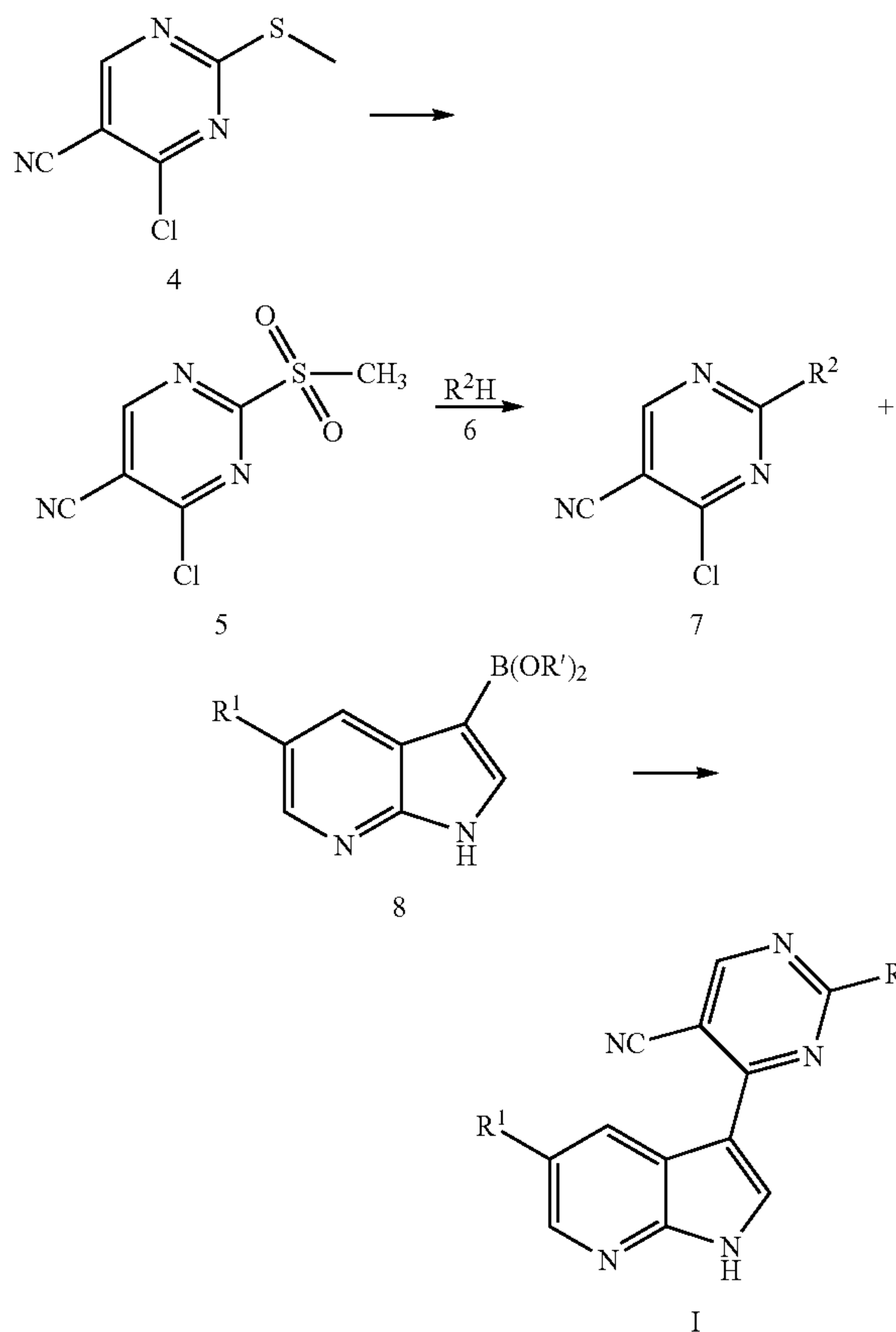
Scheme 3
