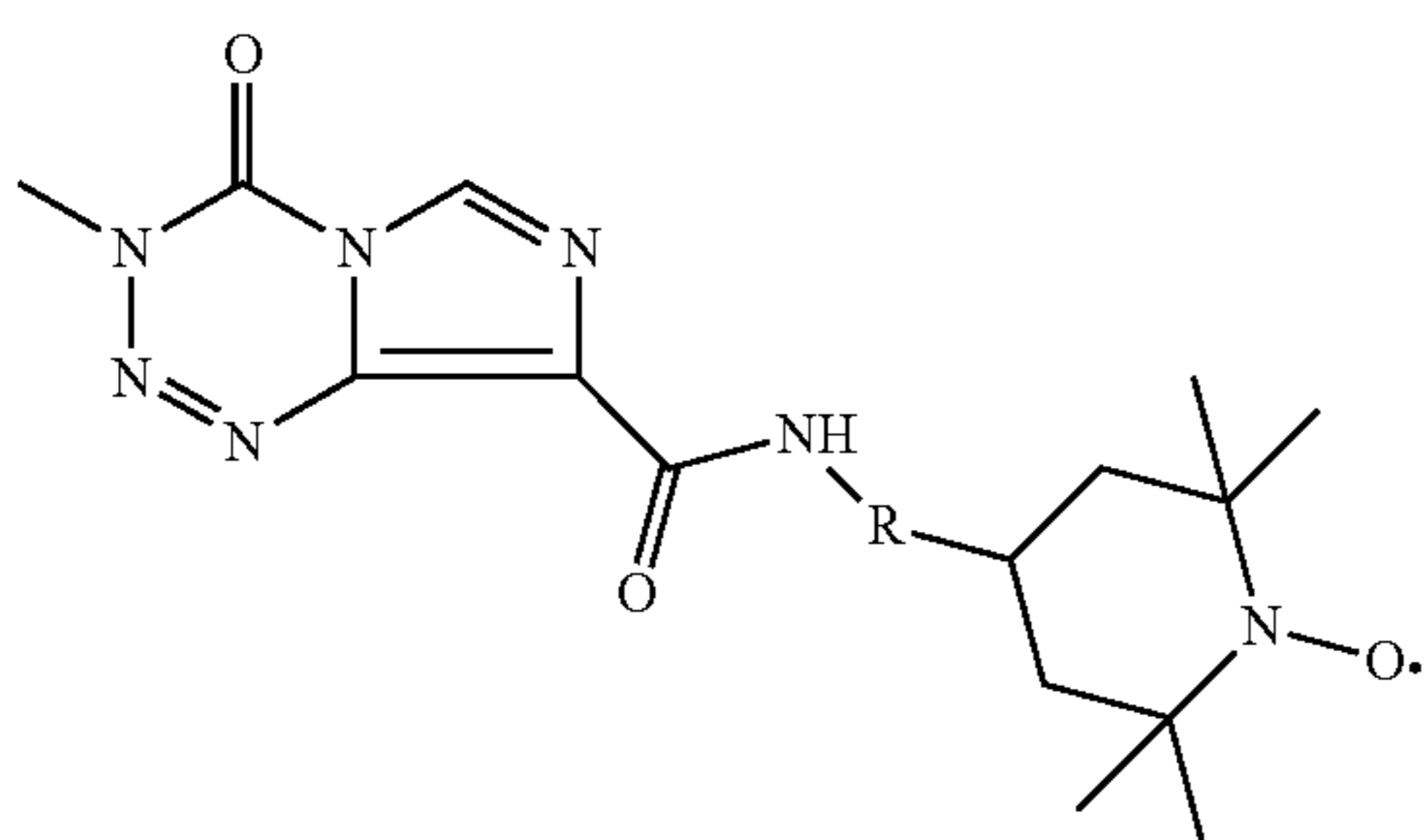
Temozolomide Adduct
