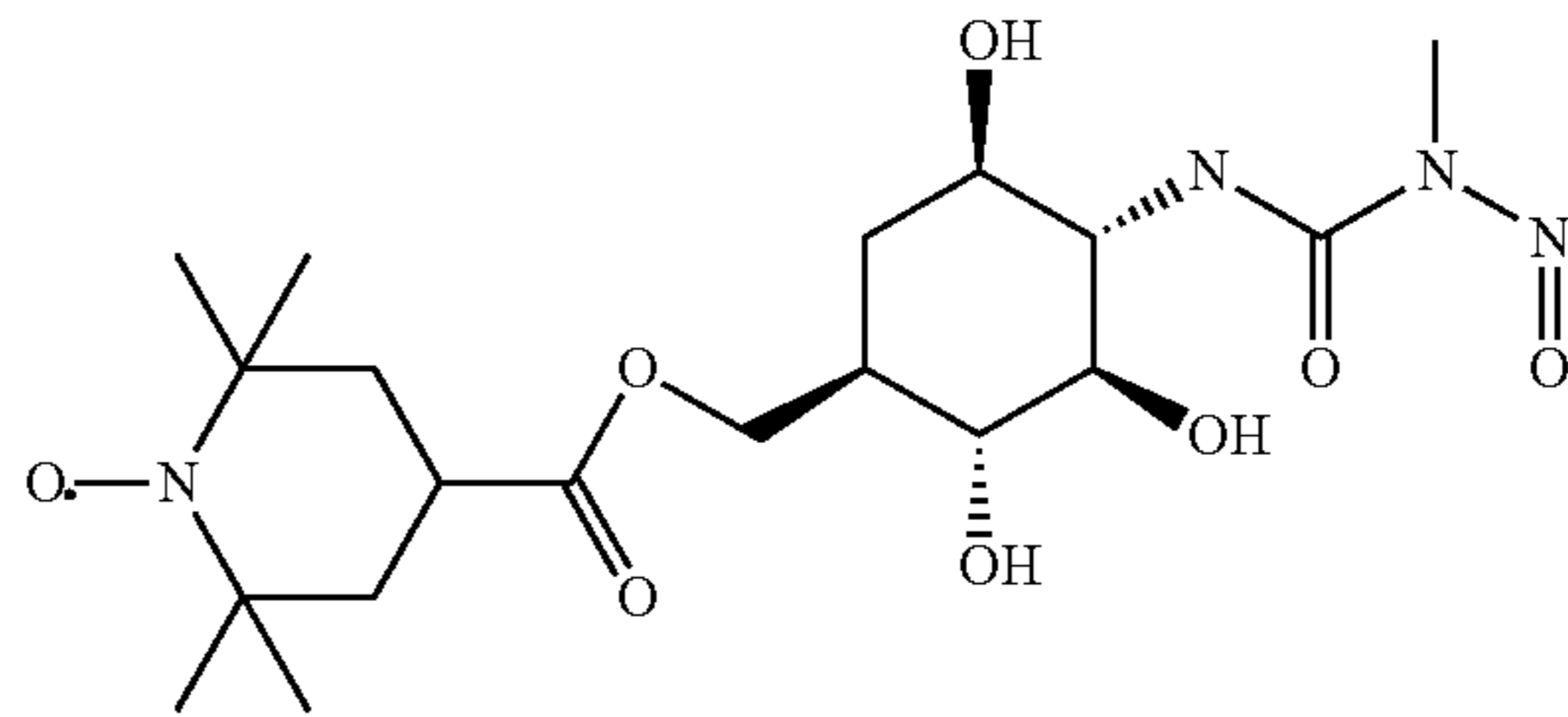
Streptozocin Adduct
