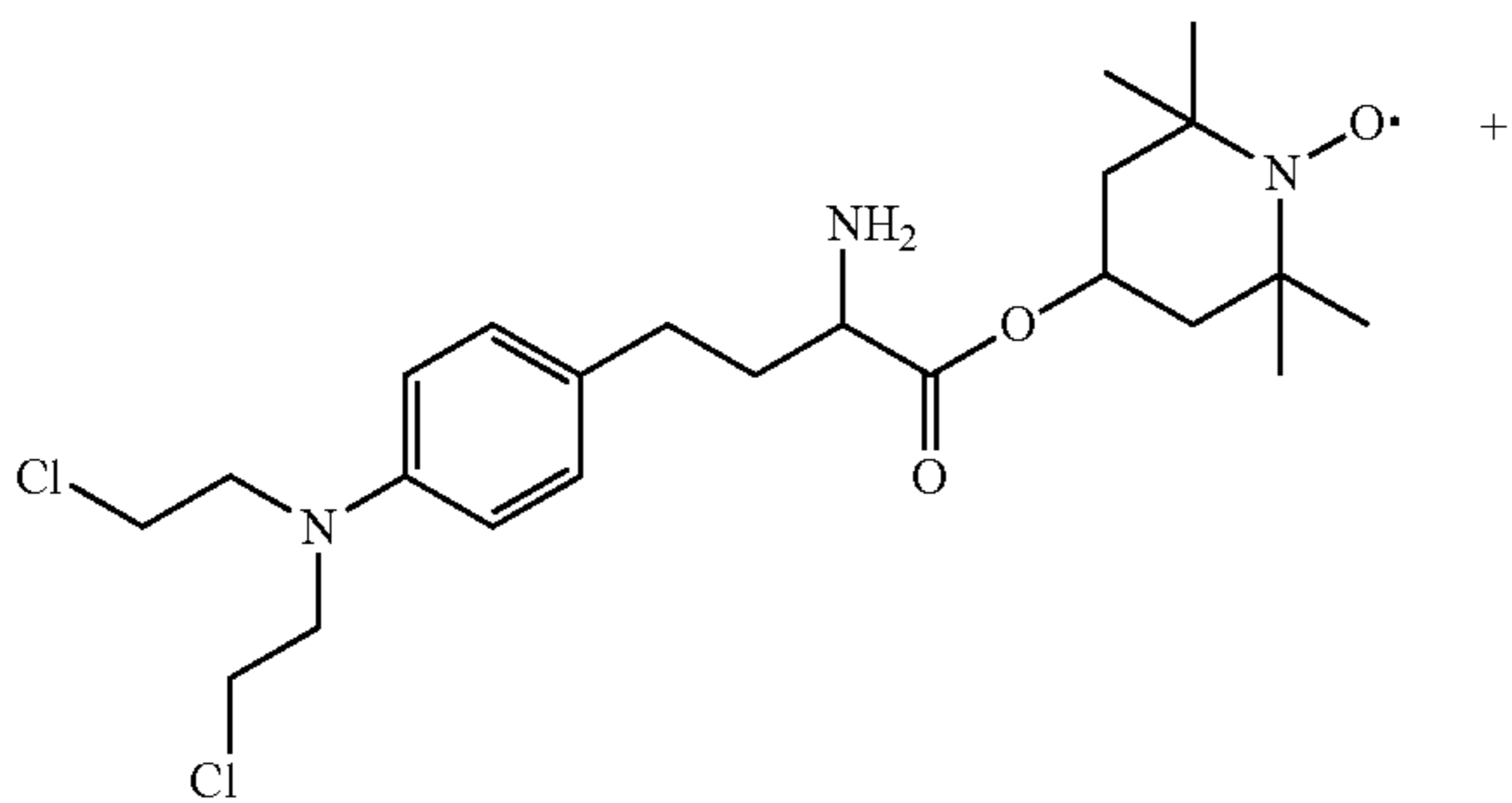
Melphalan Adducts
