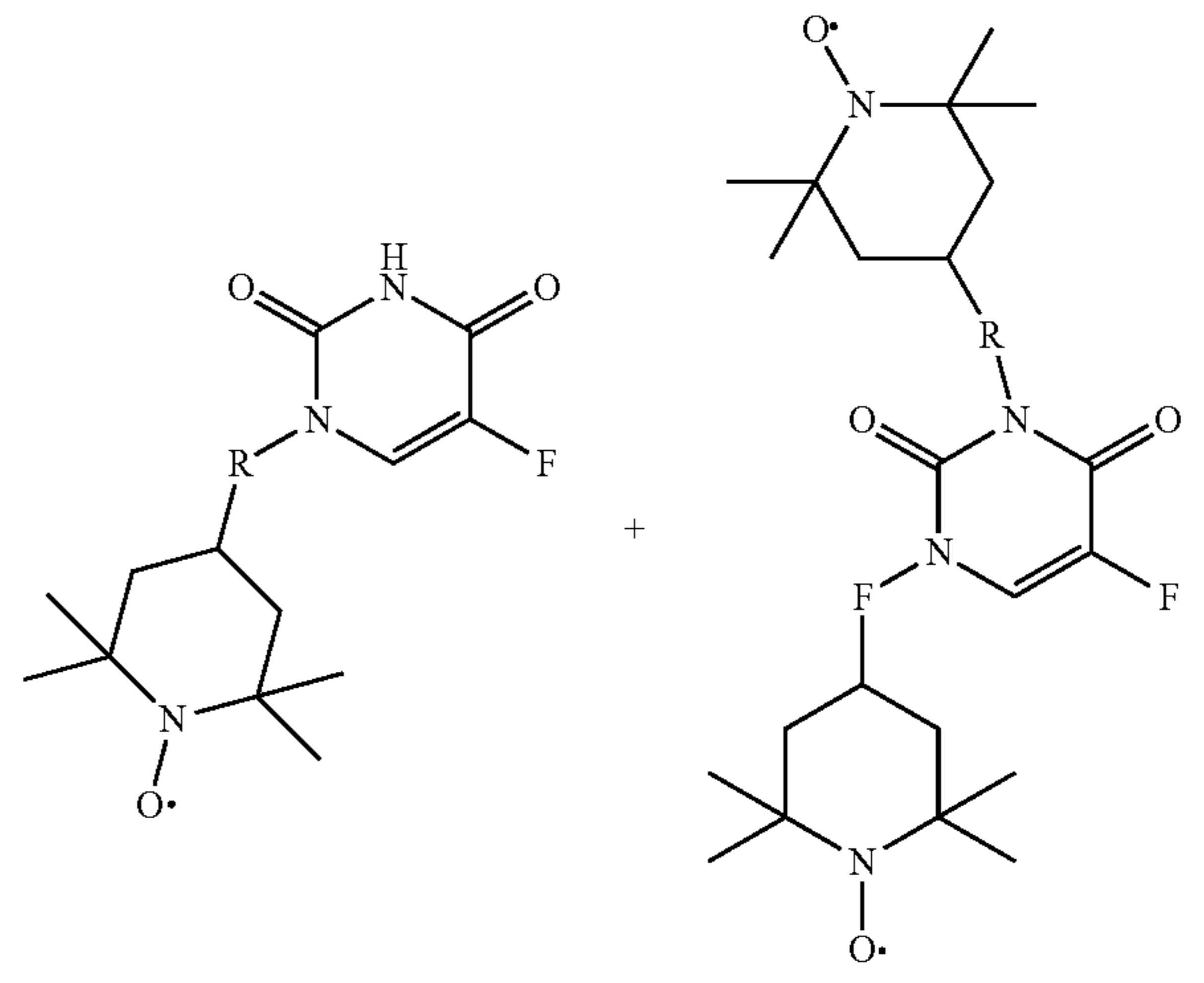
5-fluorouracil Adducts
