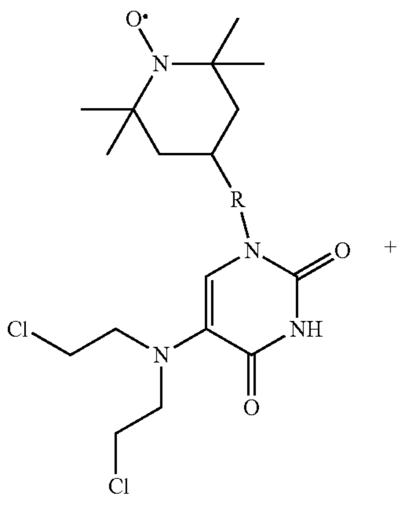
Cyclophosphamide Adduct
