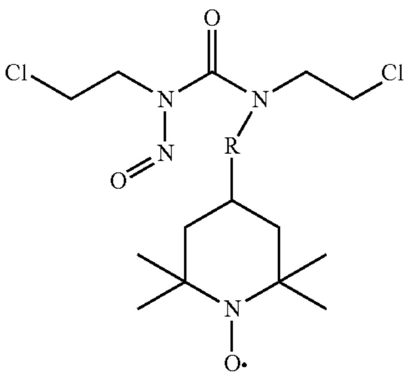
Carmustine Adduct
