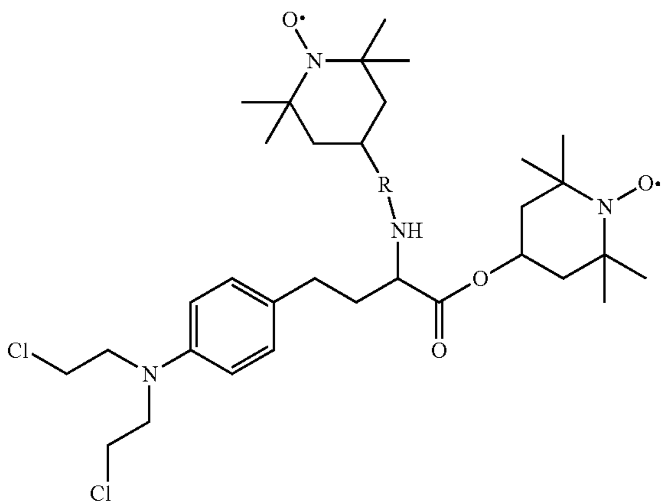
Melphalan Adducts
