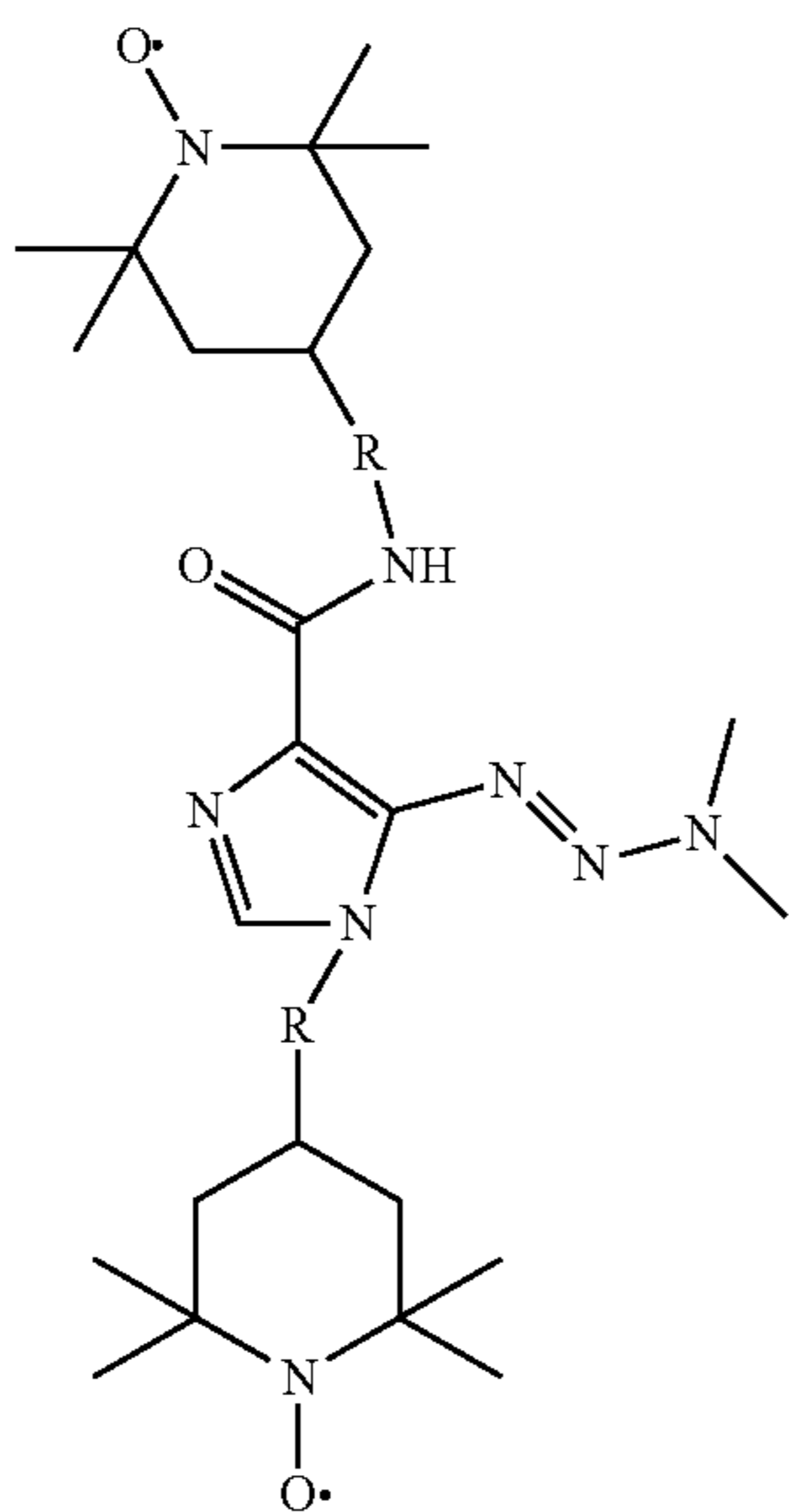
Dacarbazine Adducts
