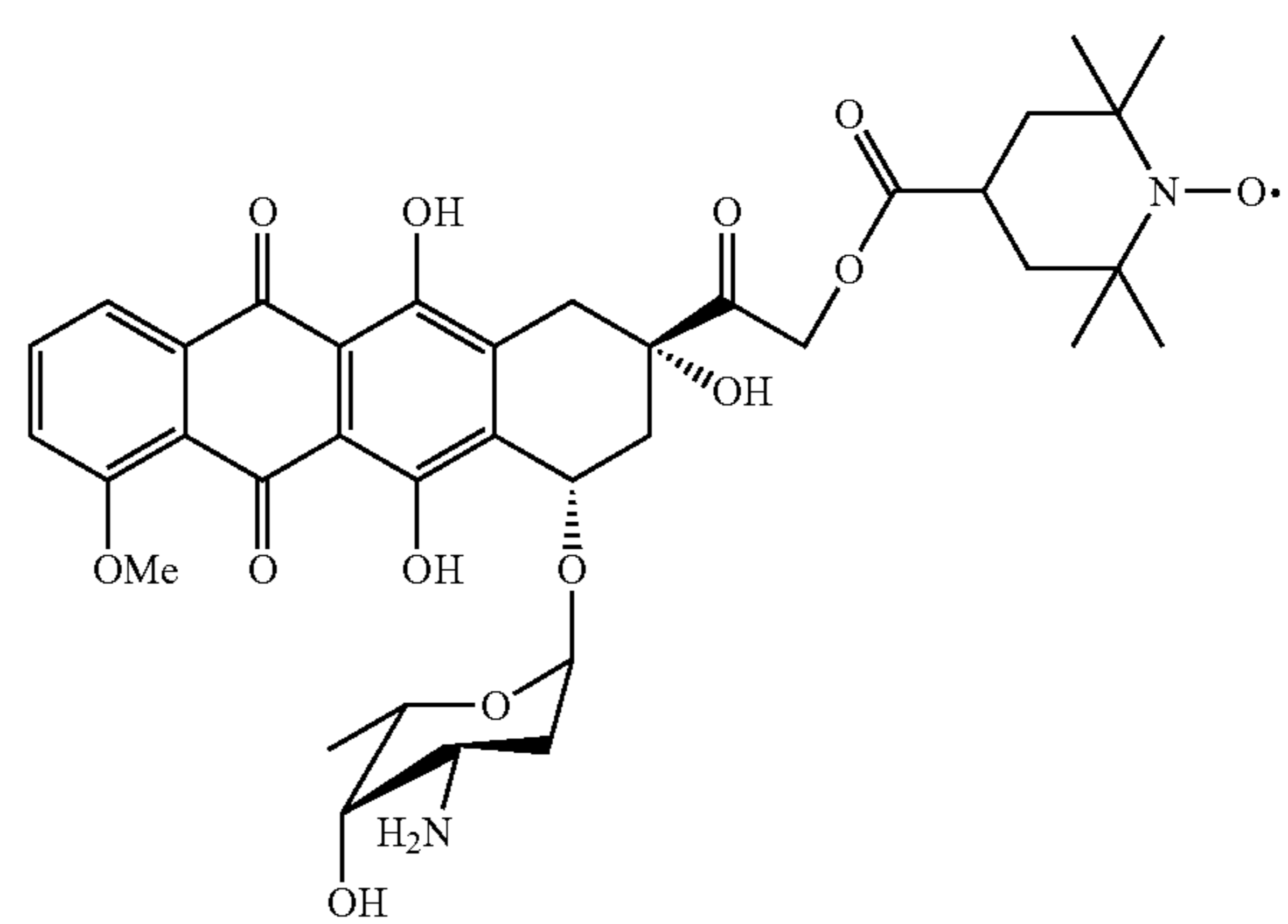
Doxorubicin Adduct
