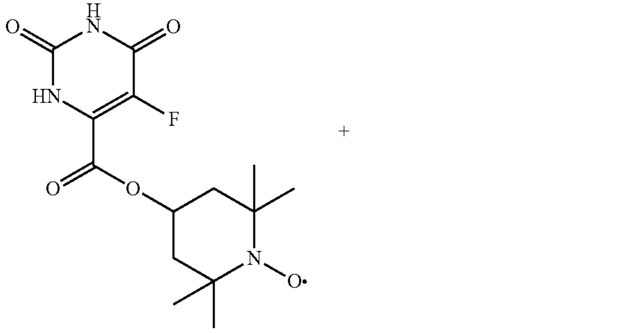
5-fluorouracil Adducts
