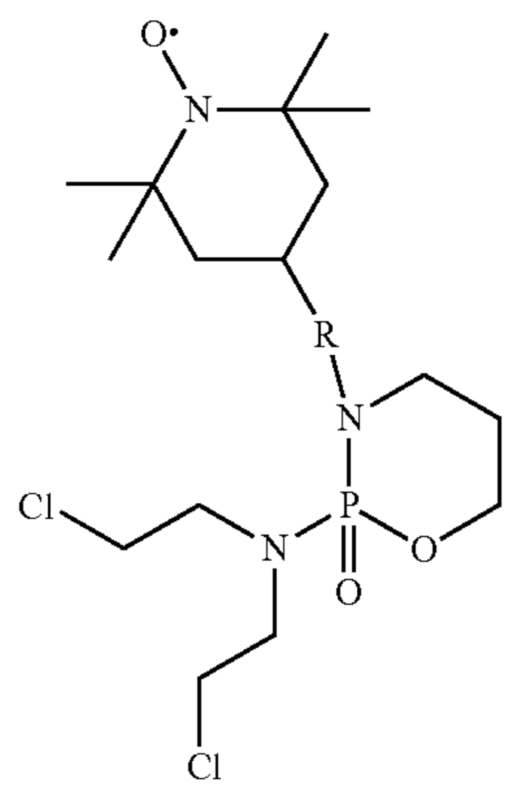
Cyclophosphamide Adduct
