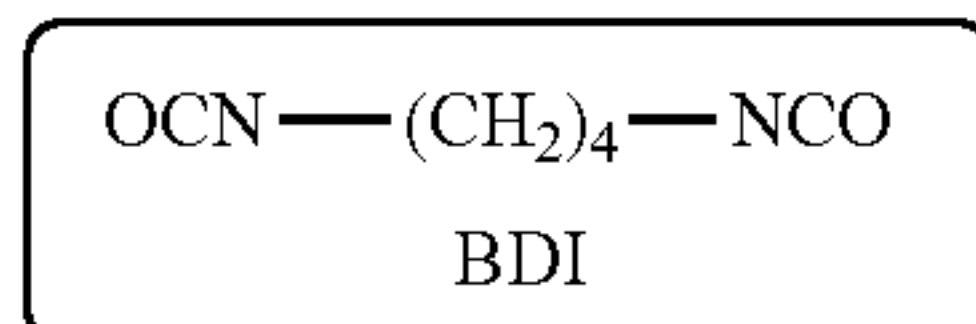
BDI 1,4-butane diisocyanate
