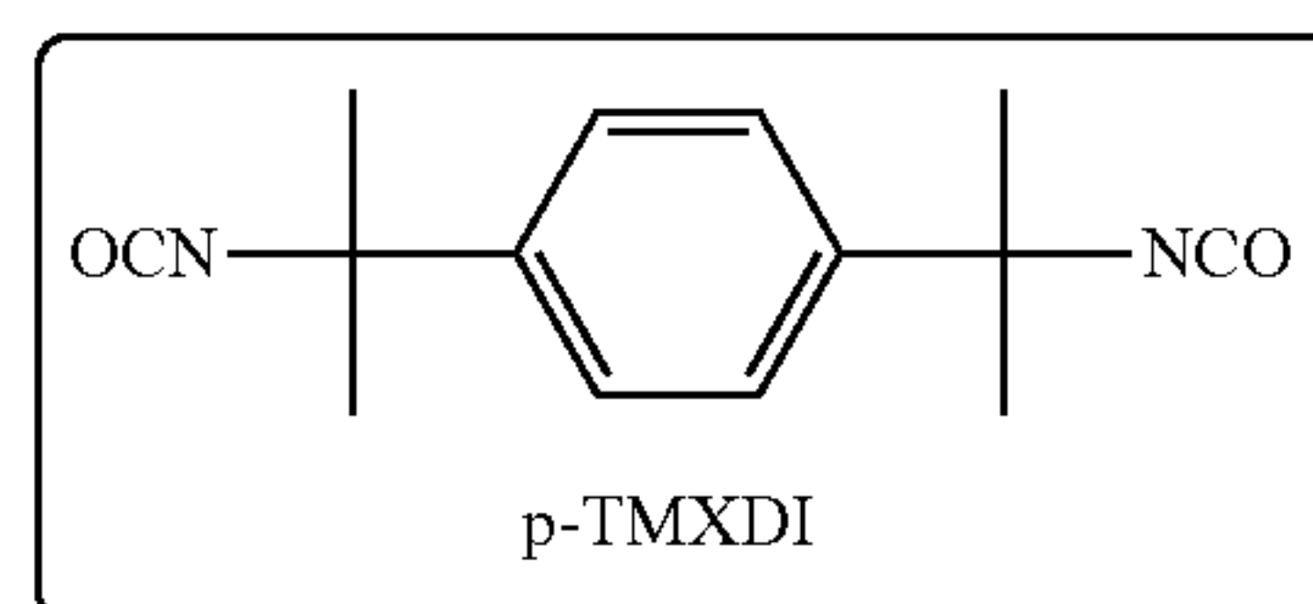
p-TMXDI p-tetramethyl xylene diisocyanate
