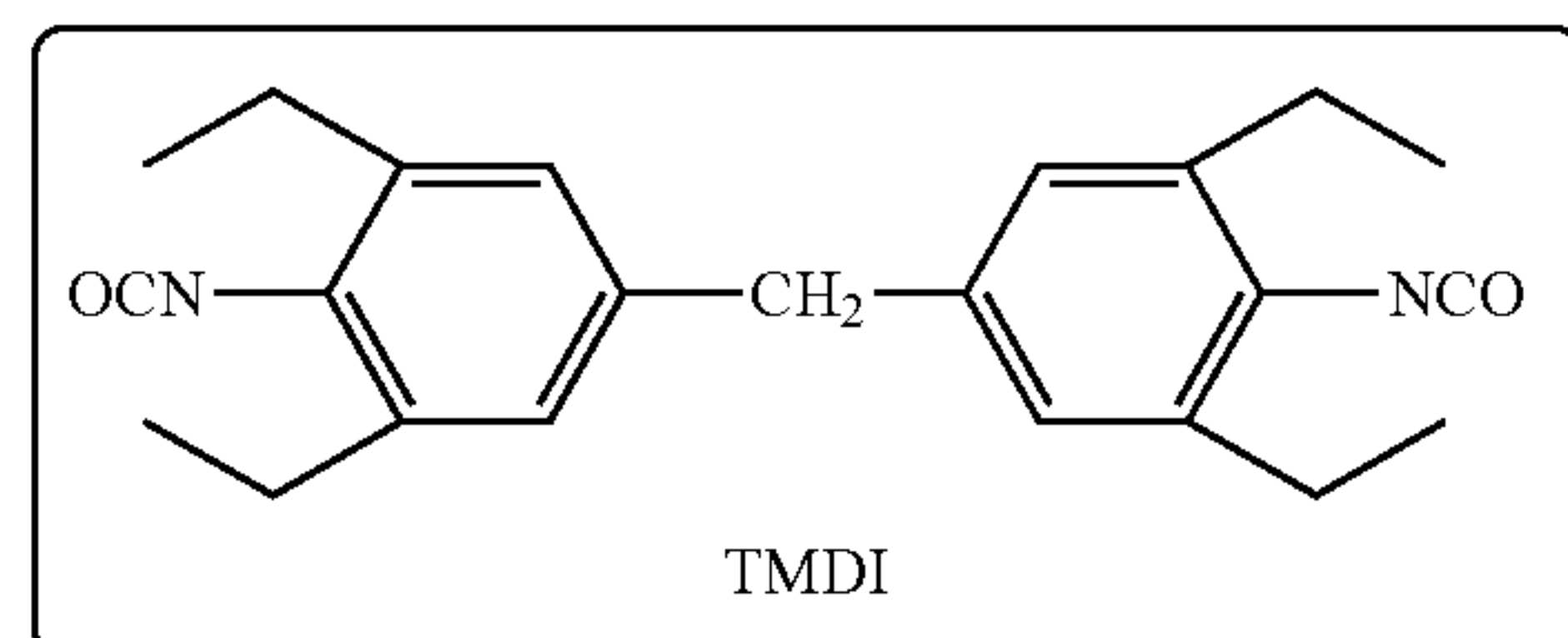
TMDI Tetraethyl methylene diphenyl diisocyanate
