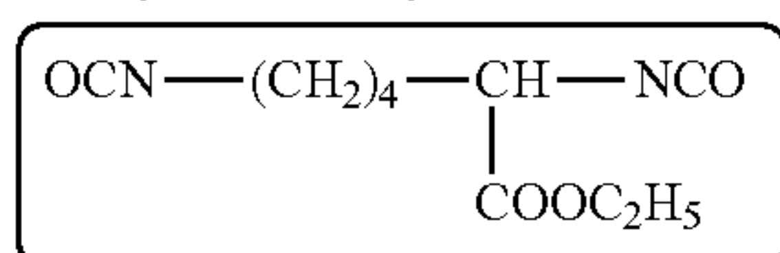
ELDI ethyl 2,6-diisocyanato hexanoate
