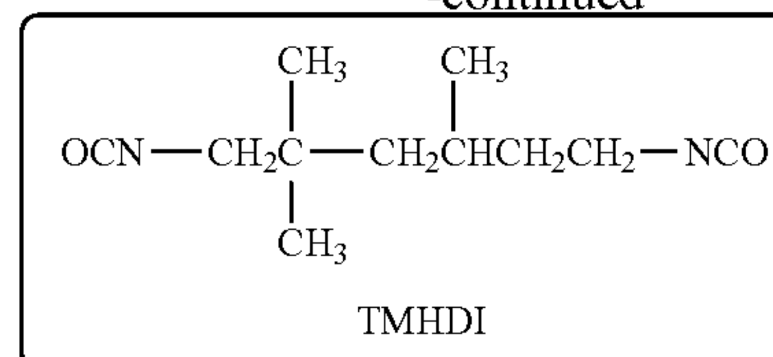
TMHDI 2,2,4-Trimethyl hexamethylene diisocyanate
