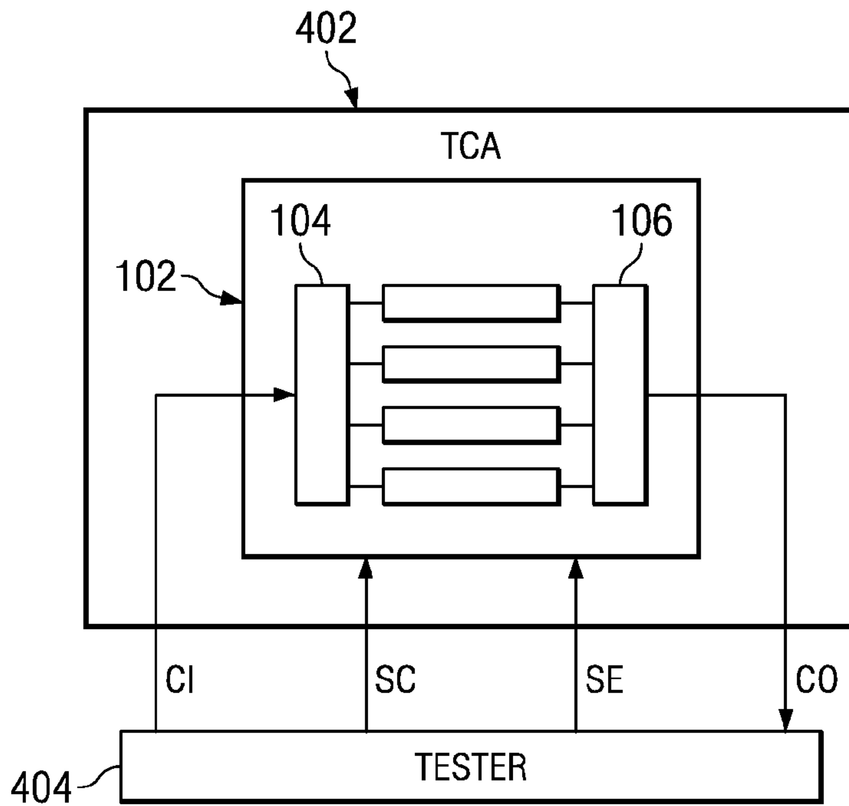
FIG. 4 (PRIOR ART)
