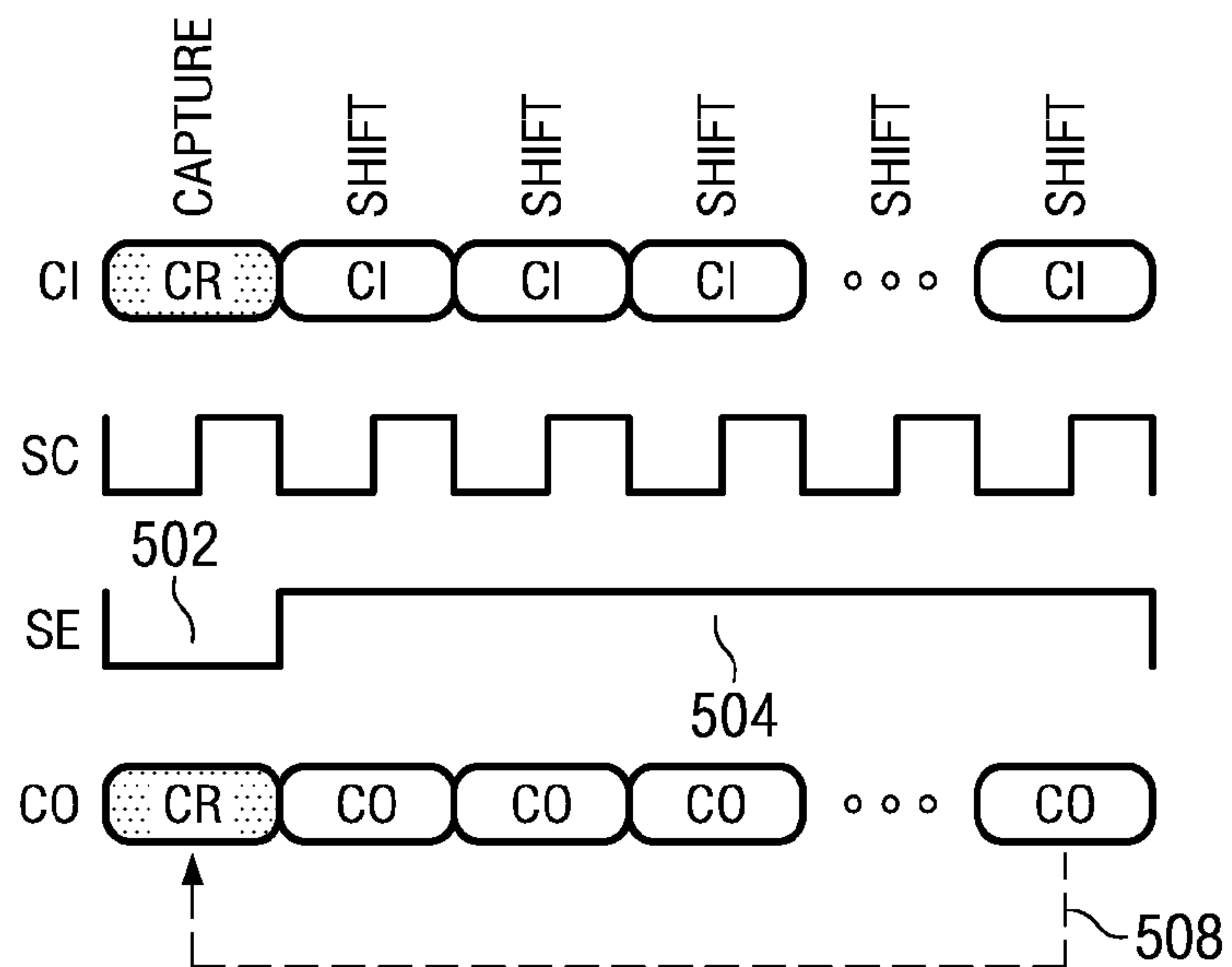
FIG. 5 (PRIOR ART)
