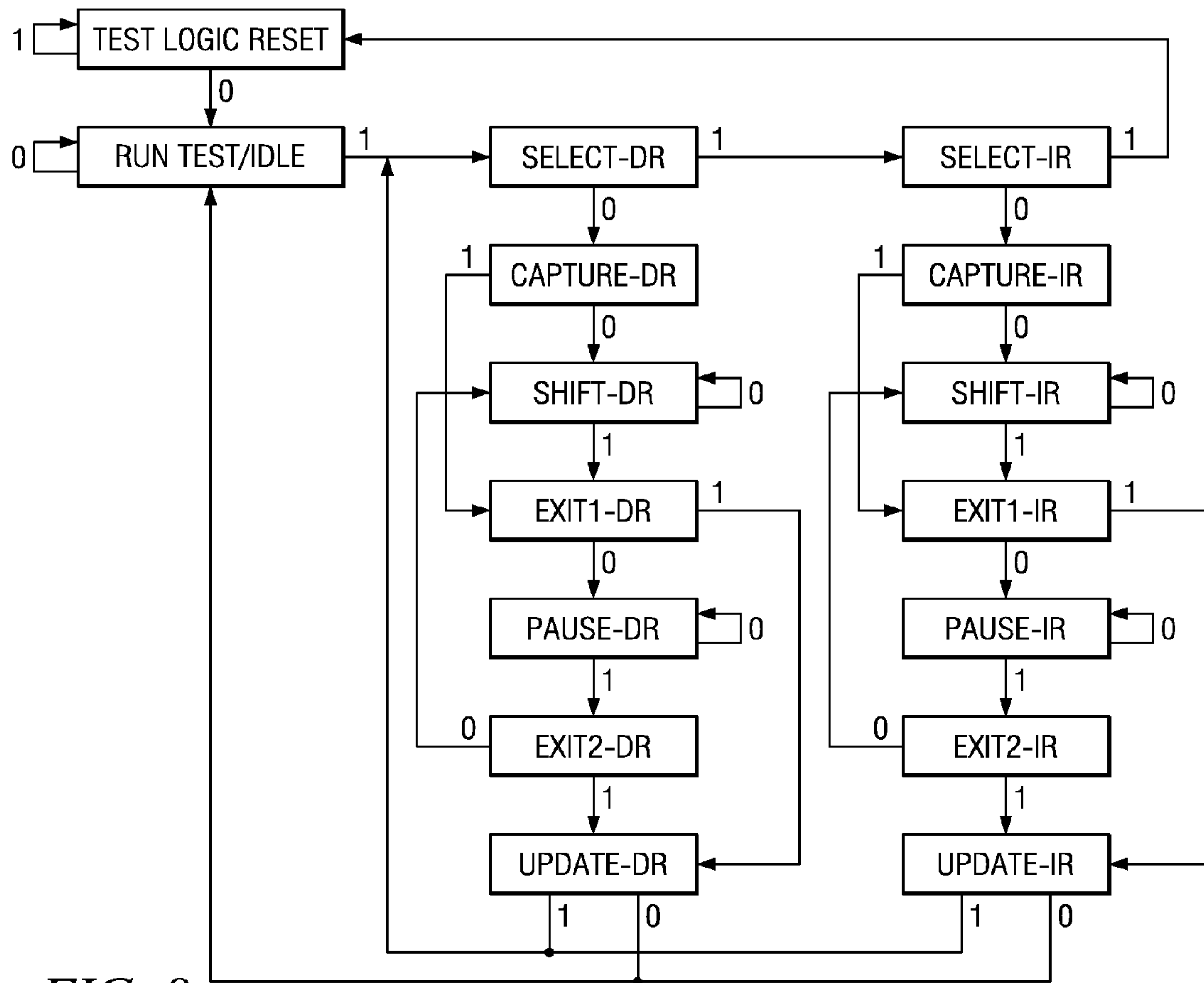
FIG. 8 (PRIOR ART)
