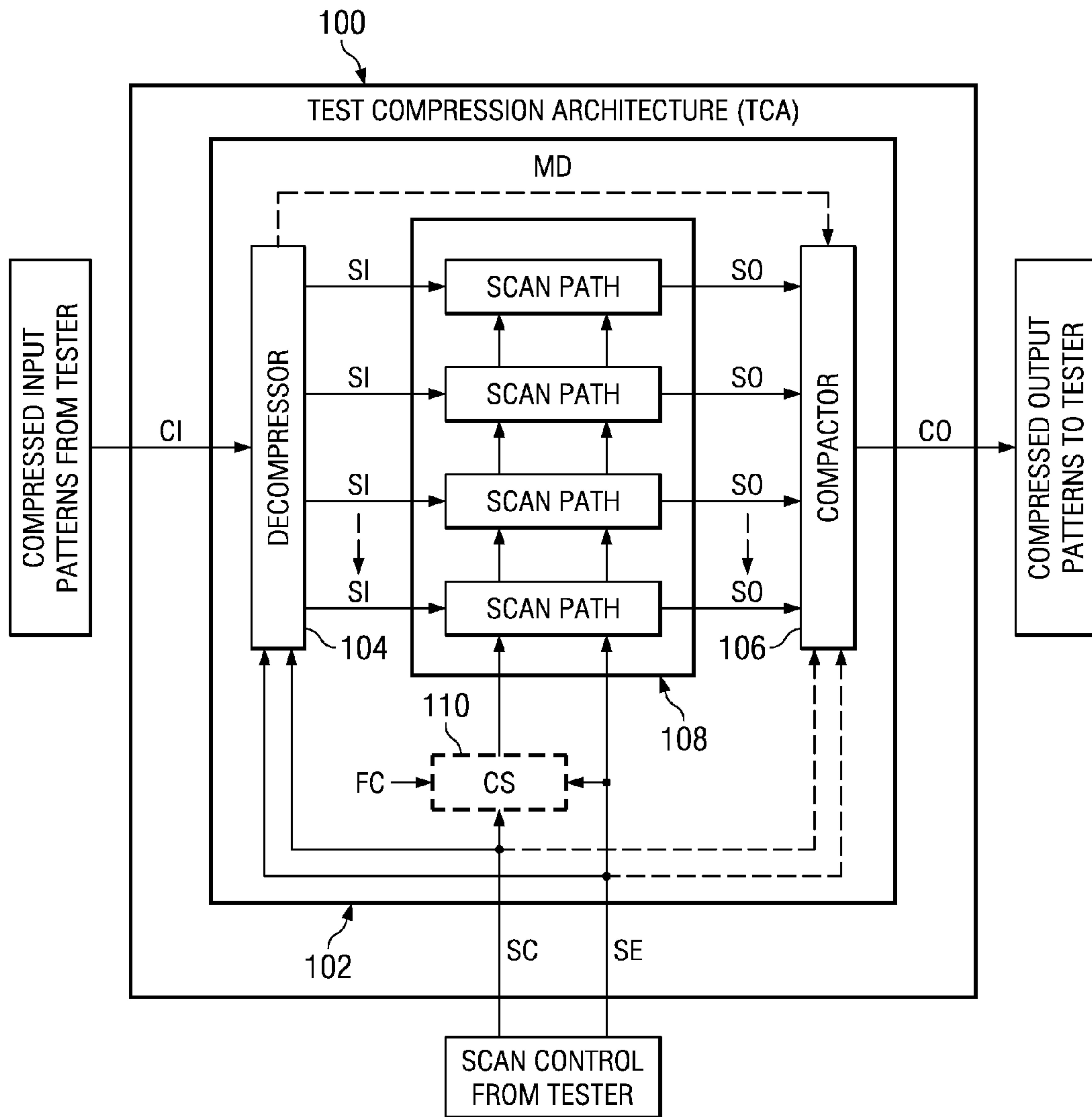
FIG. 1 (PRIOR ART)
