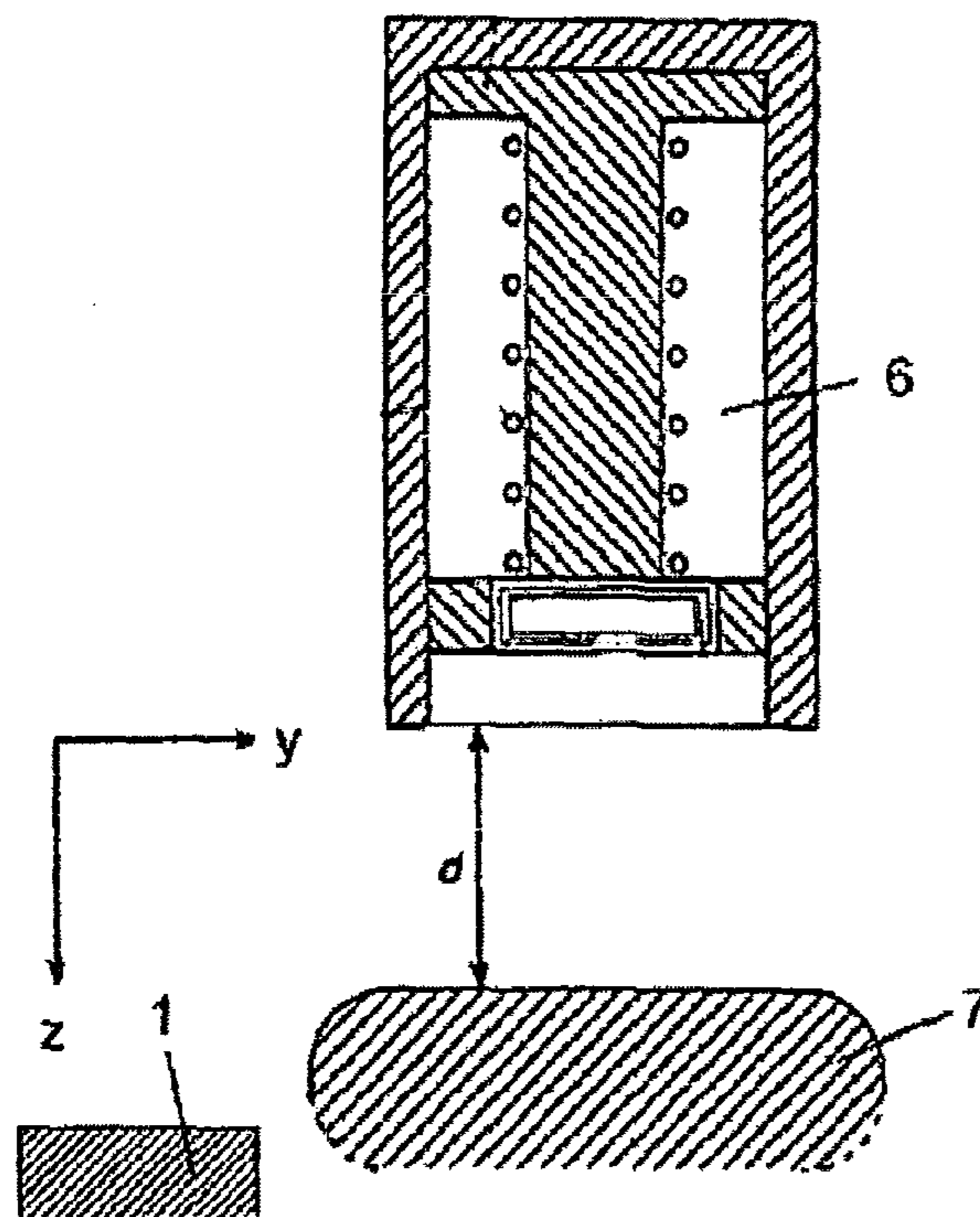
Figure 5: Cross-section of the Odometer, Railhead and Coded Tag Prior Art
