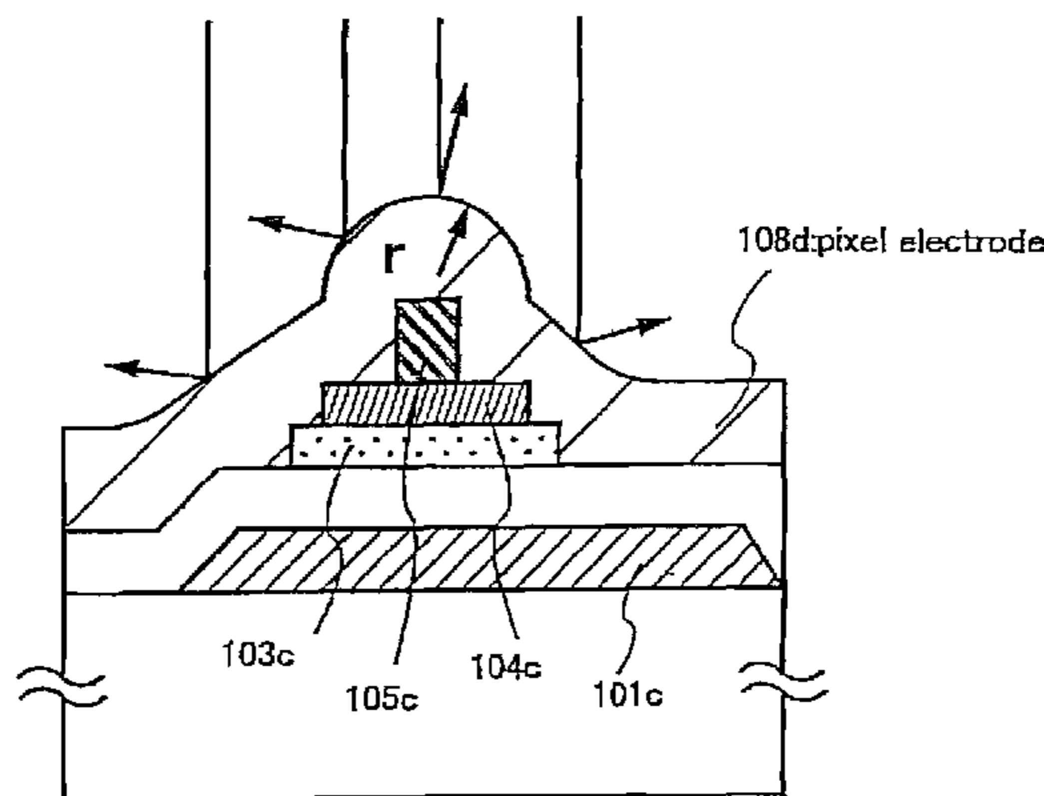
A drawing showing the radius of curvature r of a convex portion in a pixel electrode
