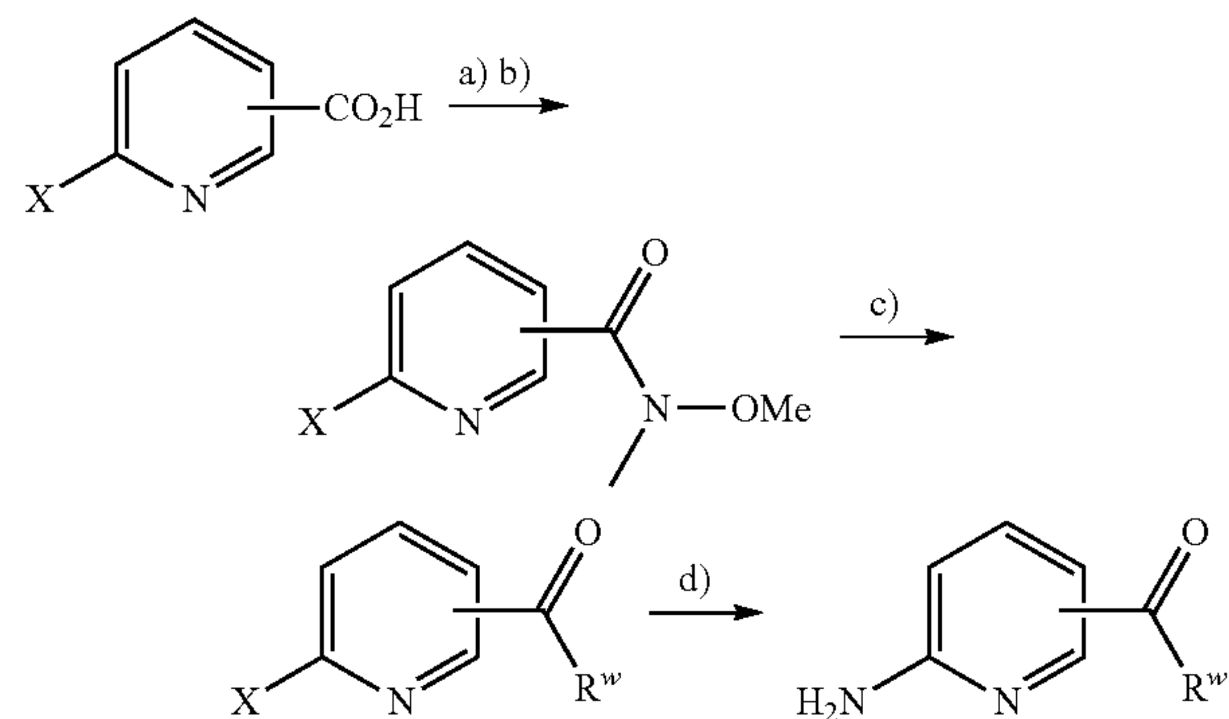
Scheme II. Preparation of amino pyridyl building blocks
