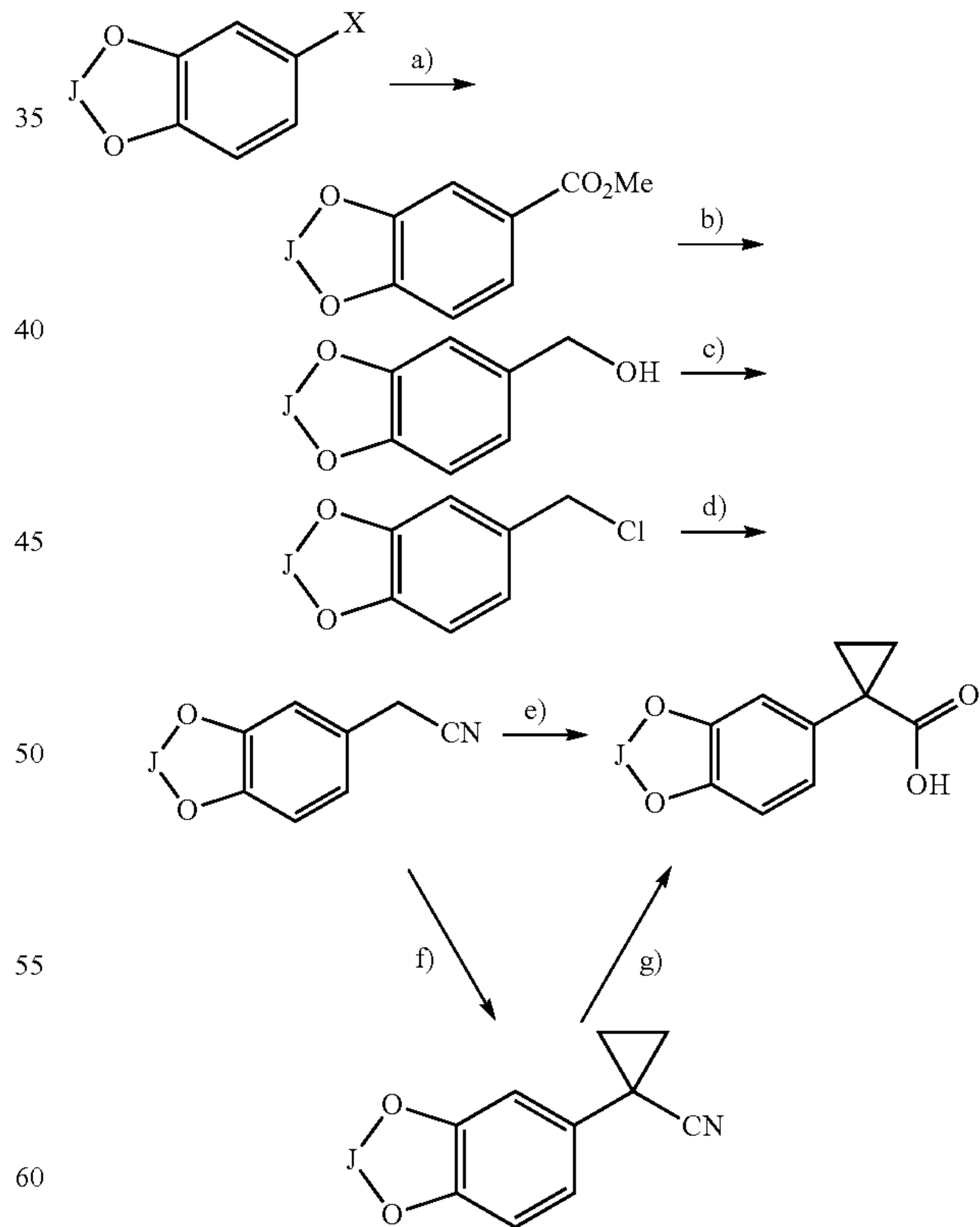
Scheme I. Preparation of cyclopropyl acids
