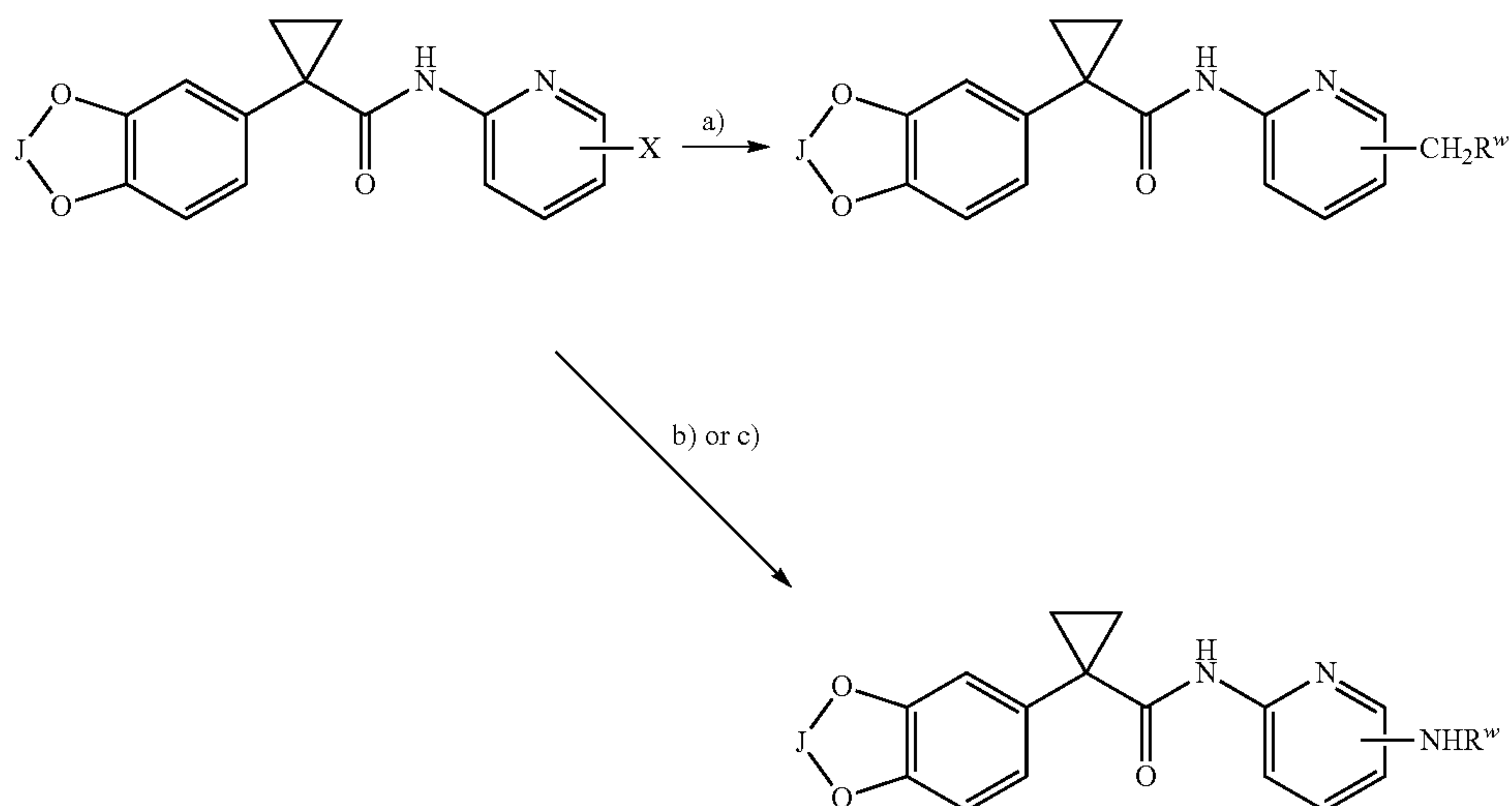
Scheme IV. Derivatization of Amides Scheme IVa
