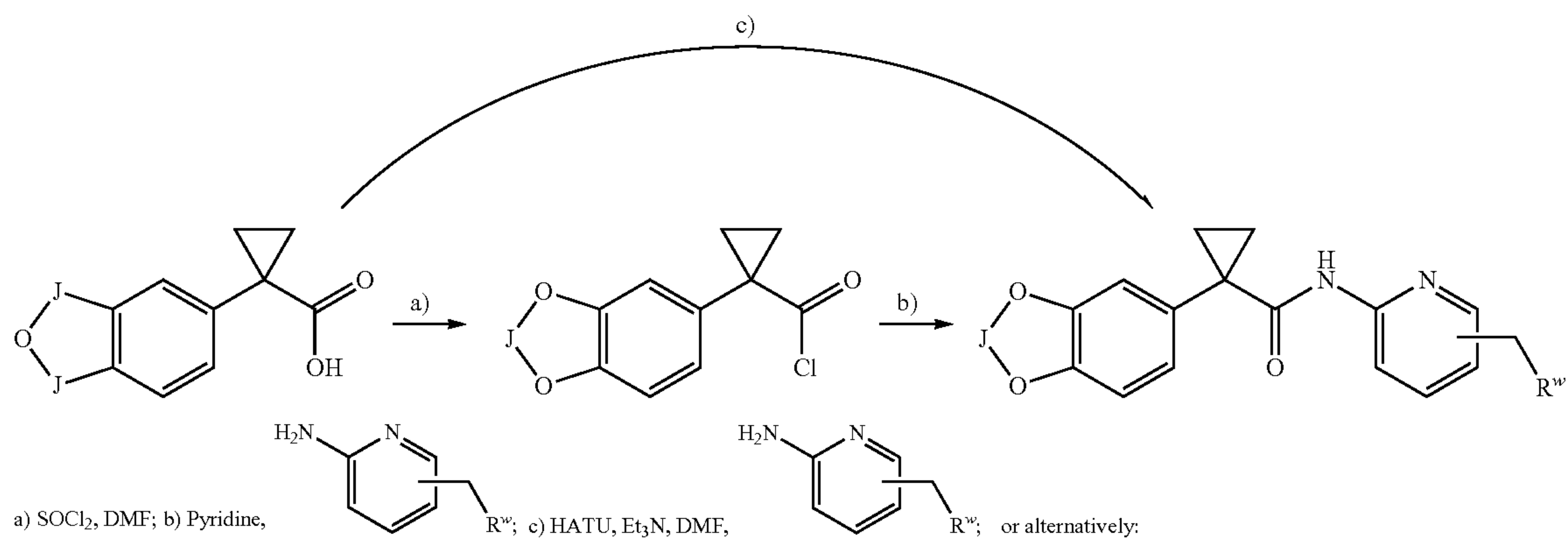
Scheme III. Amide coupling
