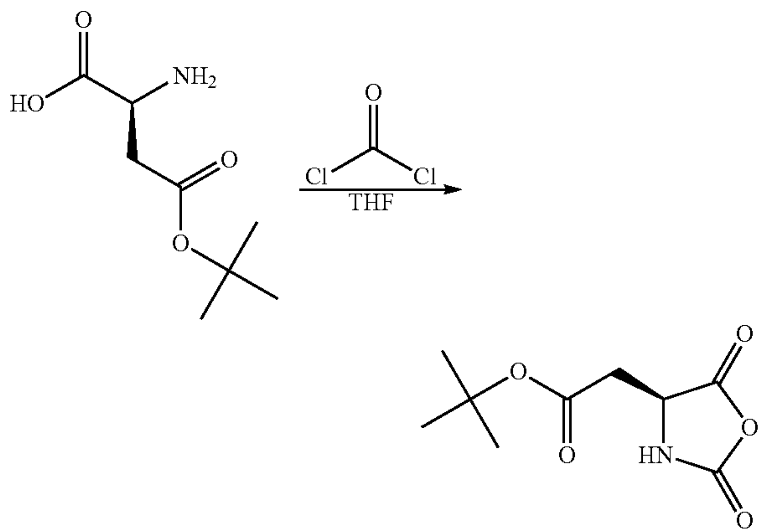
tert-Butyl Aspartate NCA
