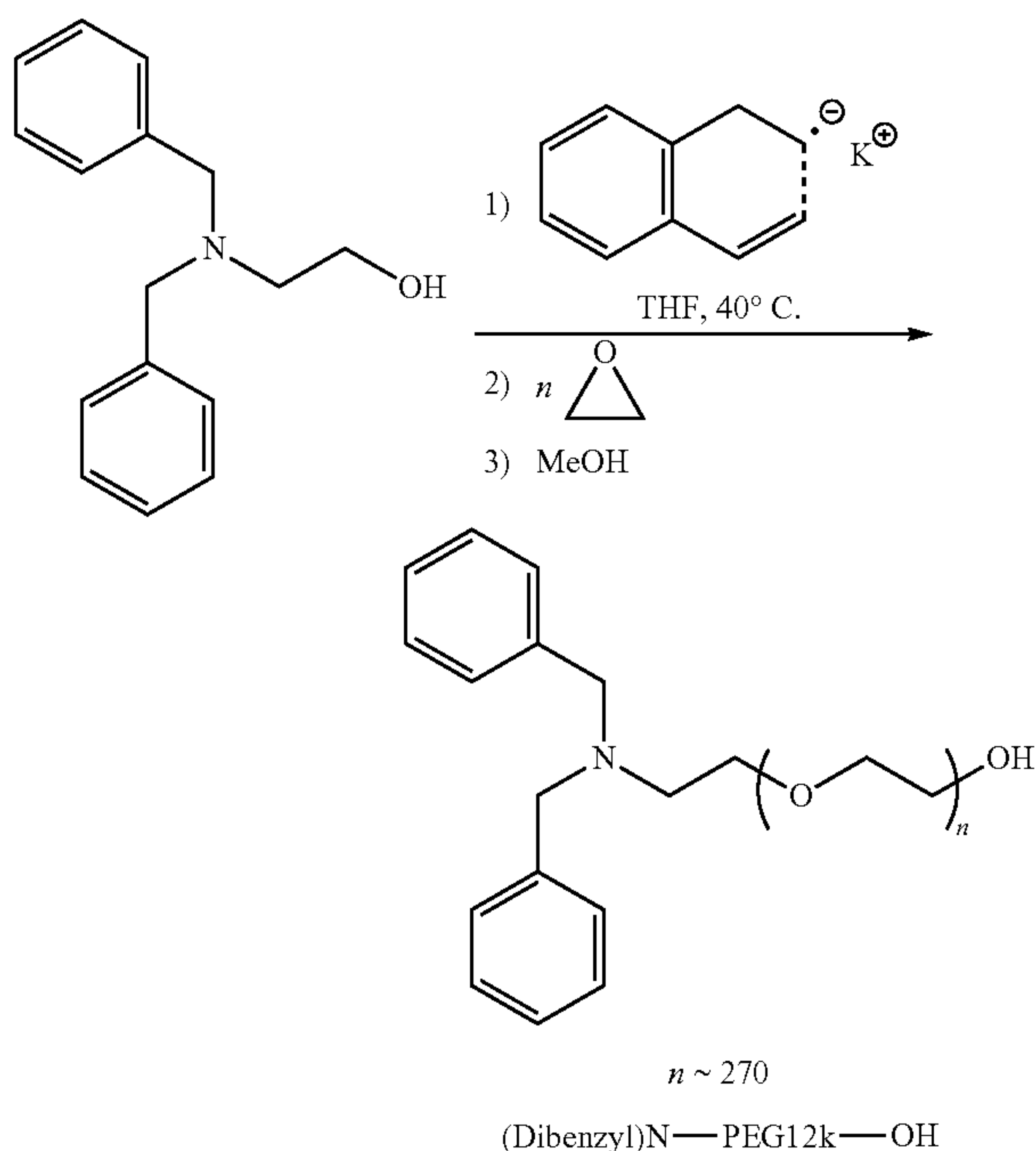
(Dibenzyl)-N-Poly(ethylene oxide) 270 -OH
