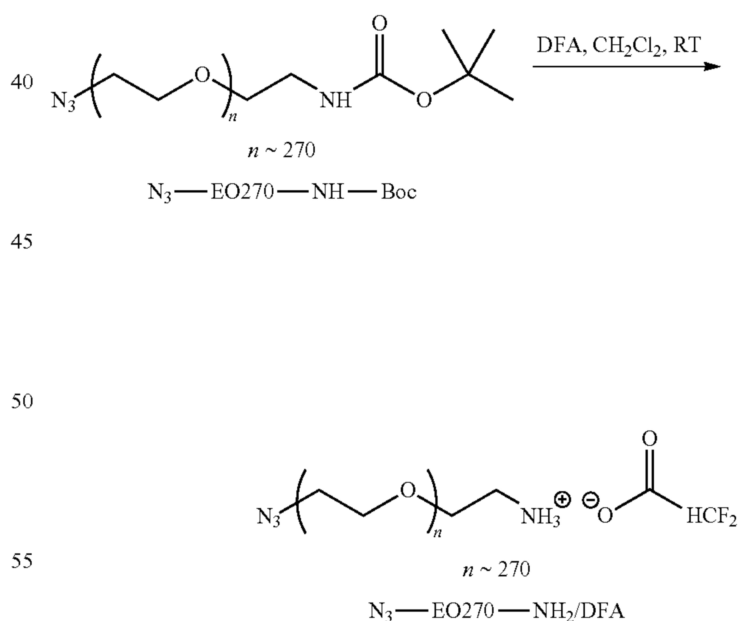
DFA + - NH 3 -Poly(ethylene oxide) 270 -N 3
