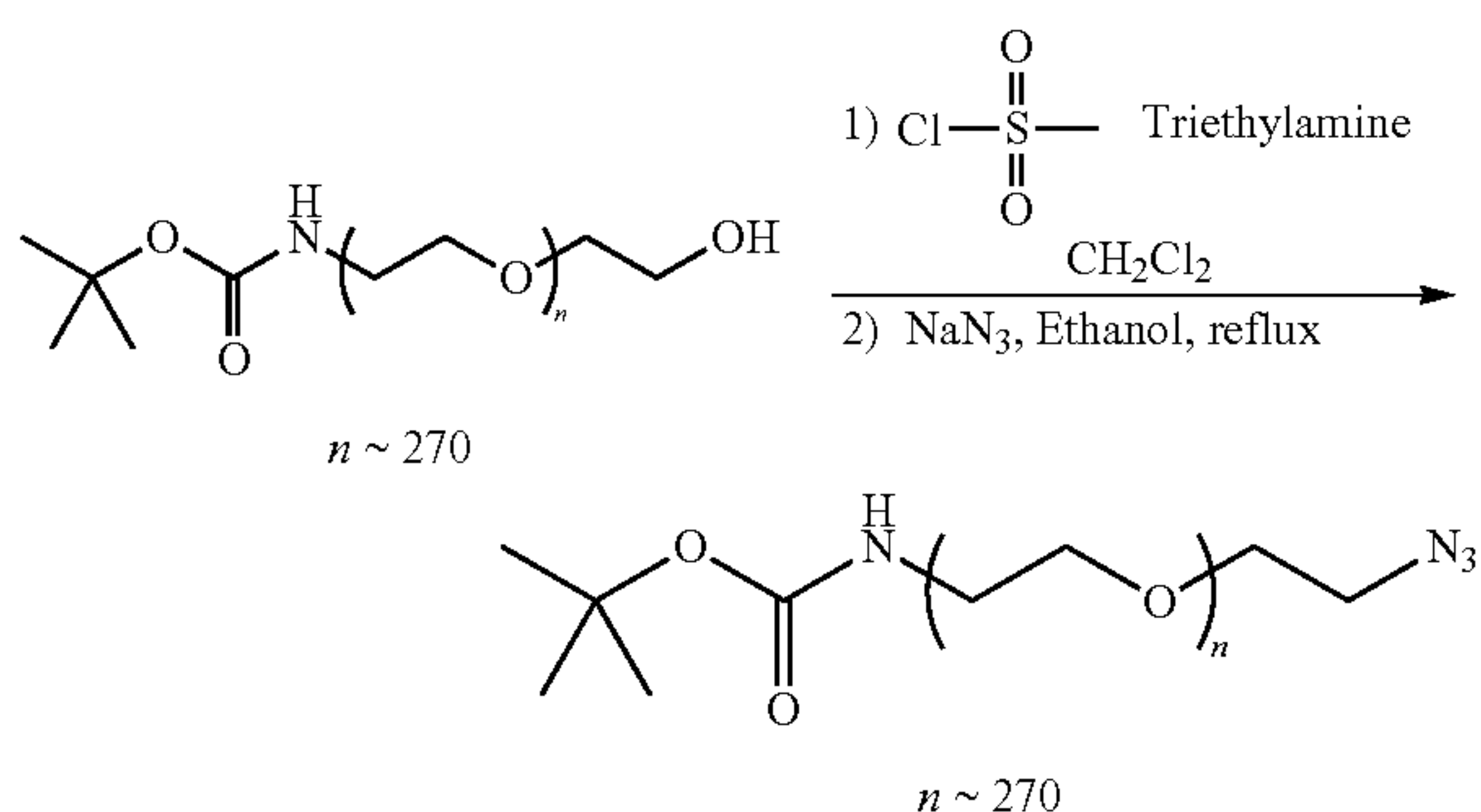
Boc-NH-Poly(ethylene oxide) 270 -N 3
