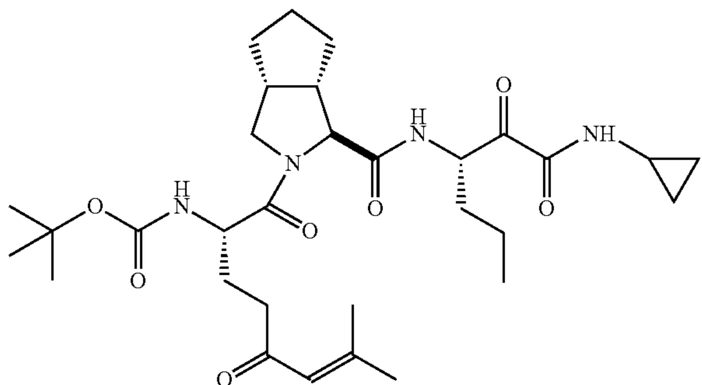
tert-butyl-(S)-1-((1S,3aR,6aS)-1-((S)-1-(cyclopropylamino)-1,2-dioxohexan-3-ylcarbamoyl)hexahydrocyclopenta[c]pyrrol-2(1H)-yl)-7-methyl-1,5-dioxooct-6-en-2-ylcarbamate
