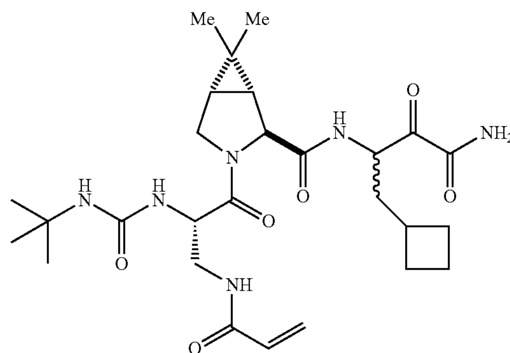
(1R,2S,5S)-3-((S)-3-acrylamido-2-(3-tert-butylureido)propanoyl)-N-(4-amino-1-cyclobutyl-3,4-dioxobutan-2-yl)-6,6-dimethyl-3-azabicyclo[3.1.0]hexane-2-carboxamide [I-1]
