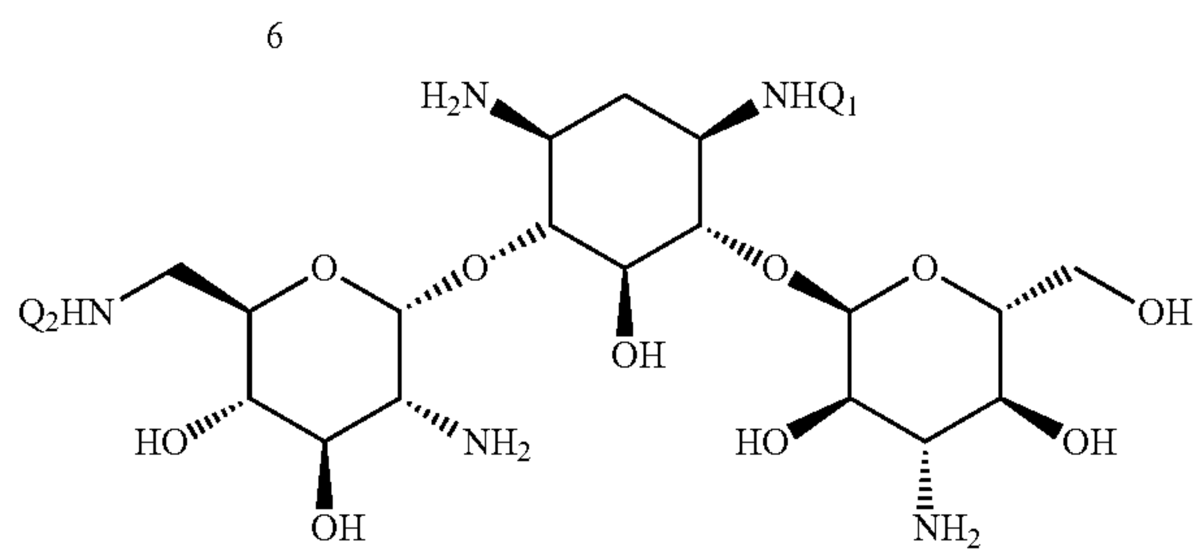
N-1, N-6'-bis-substituted kanamycin B
