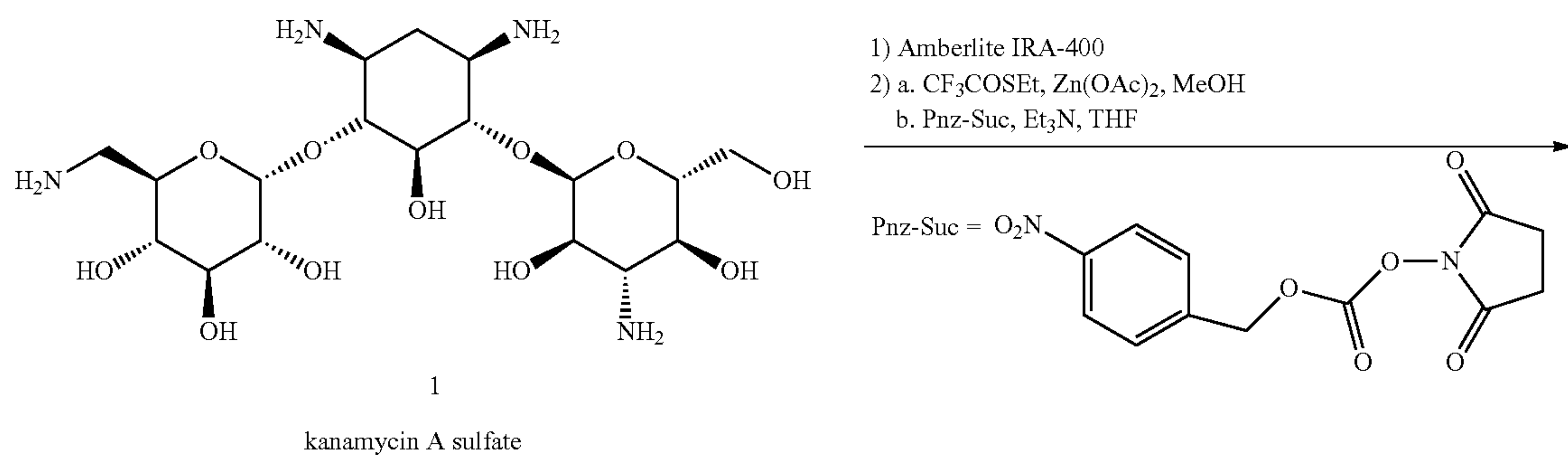
Scheme 1 N-6', N-1 Bis-substituted Kanamycin A Analogs
