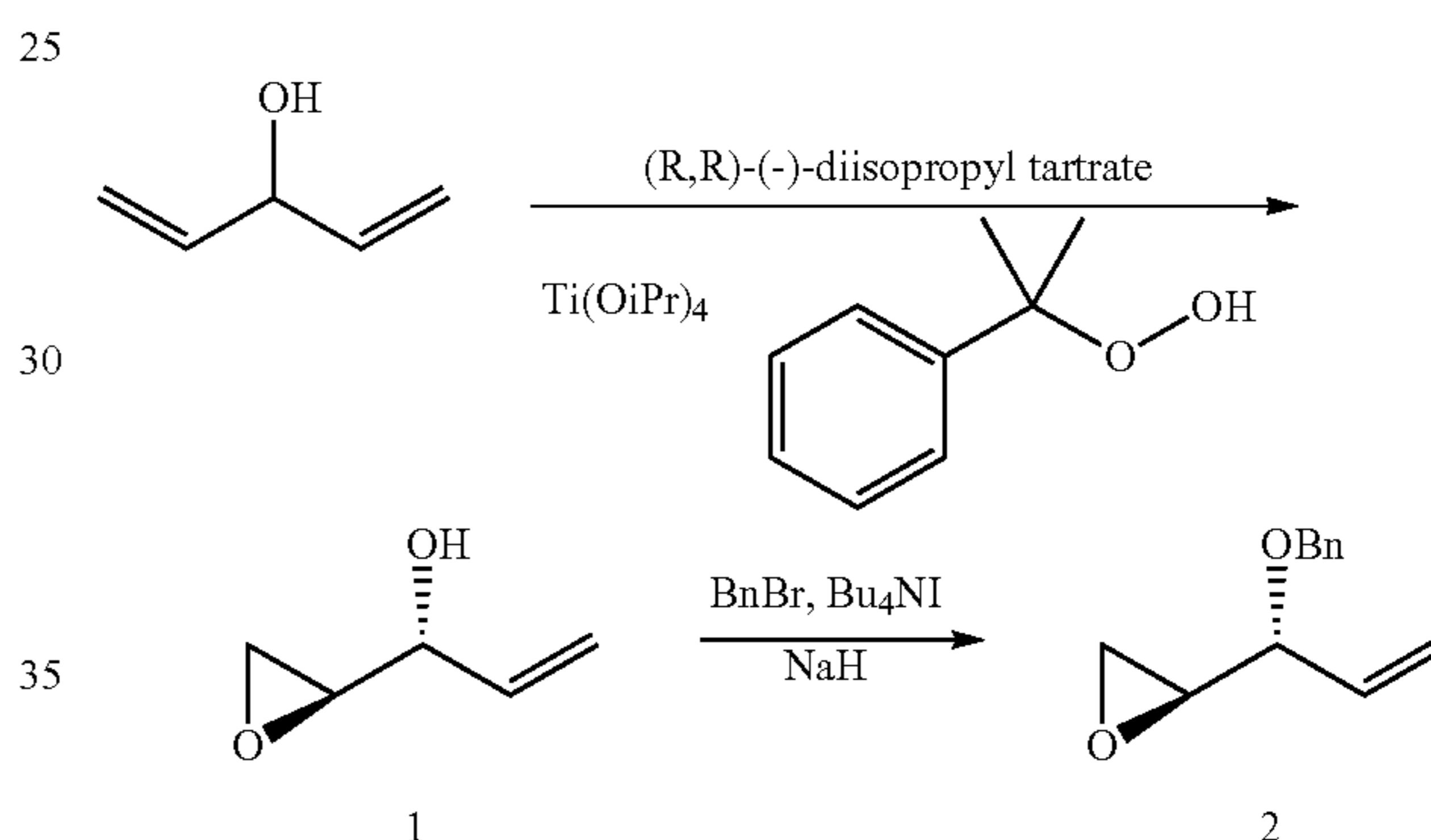
Synthesis of (2R,3R)-4-azido-2-benzyloxy-3-fluorobutanoic acid (5)
