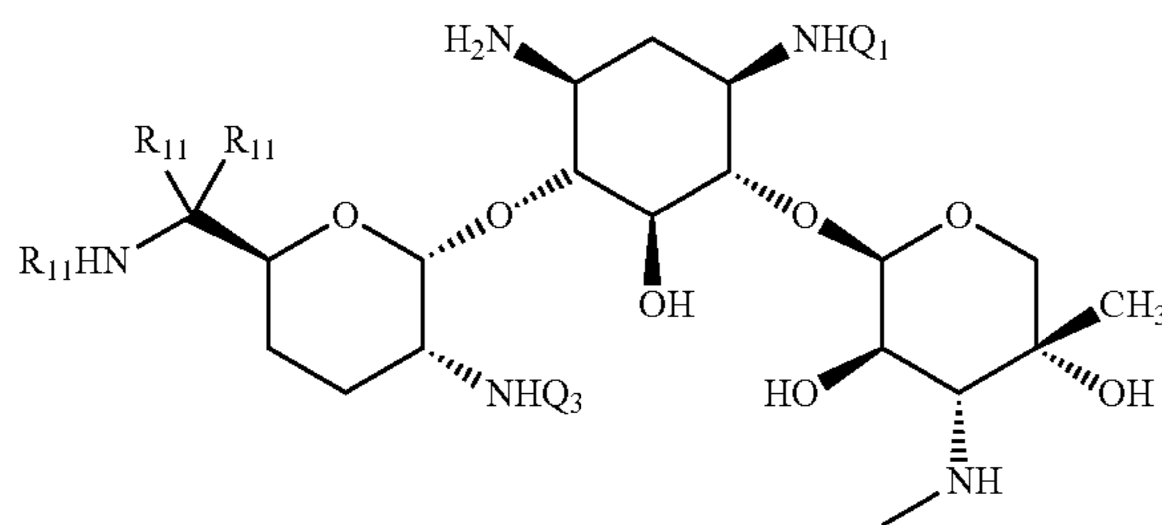
N-1, N-2'-bis-substituted gentamicin C1, C1a, C2 C2a, C2b
