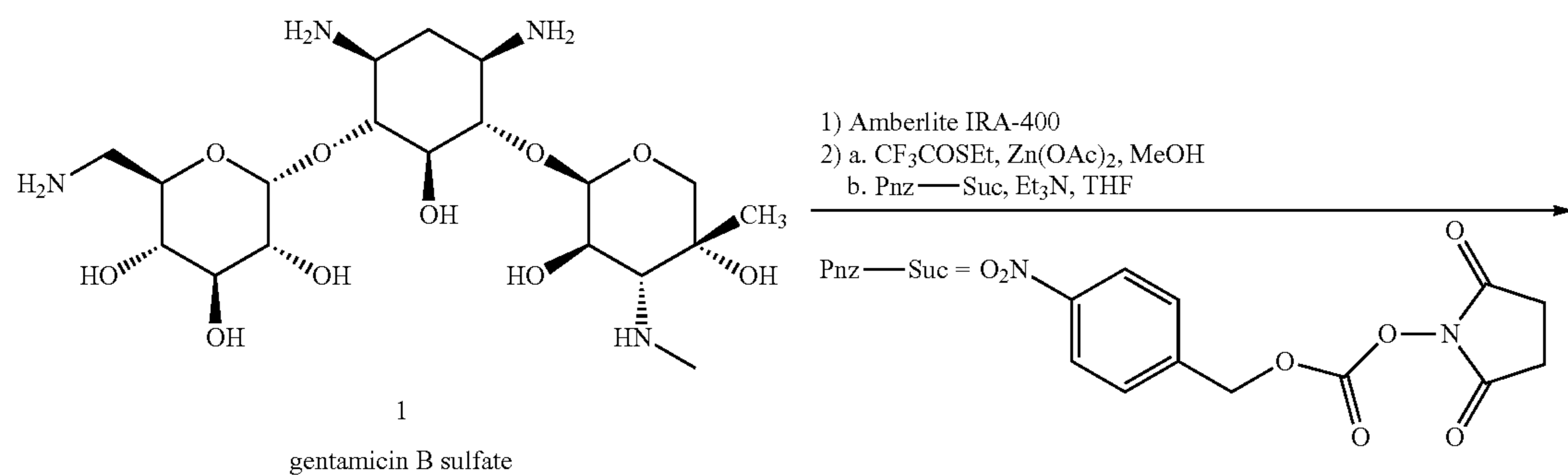
Scheme 1 N-6', N-1 Bis-substituted Gentamicin B Analogs
