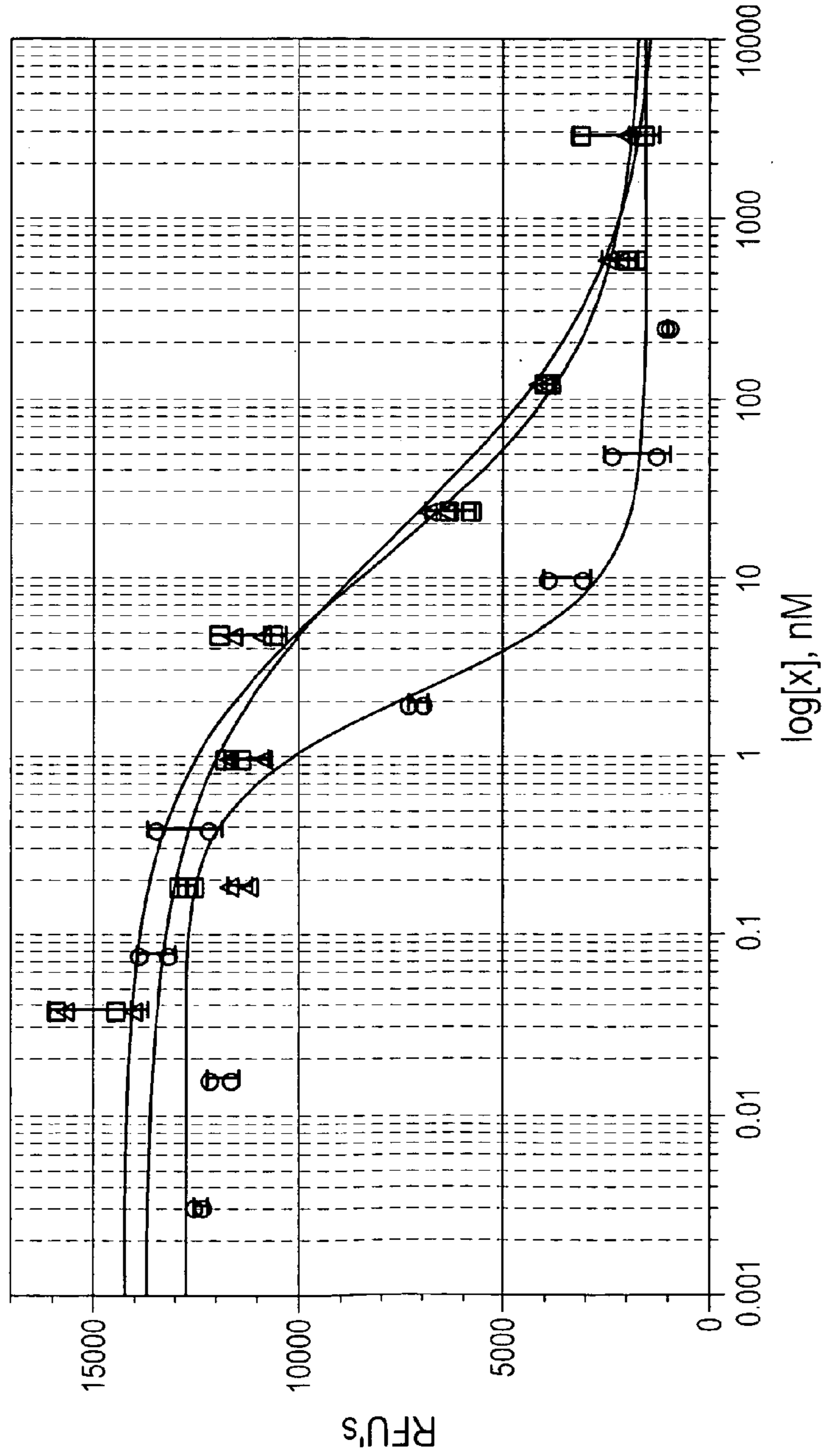
Eu-EGF Competitive Ligand Binding Assay LA-1, 679F09 Midscale, 679F09 HTPP
