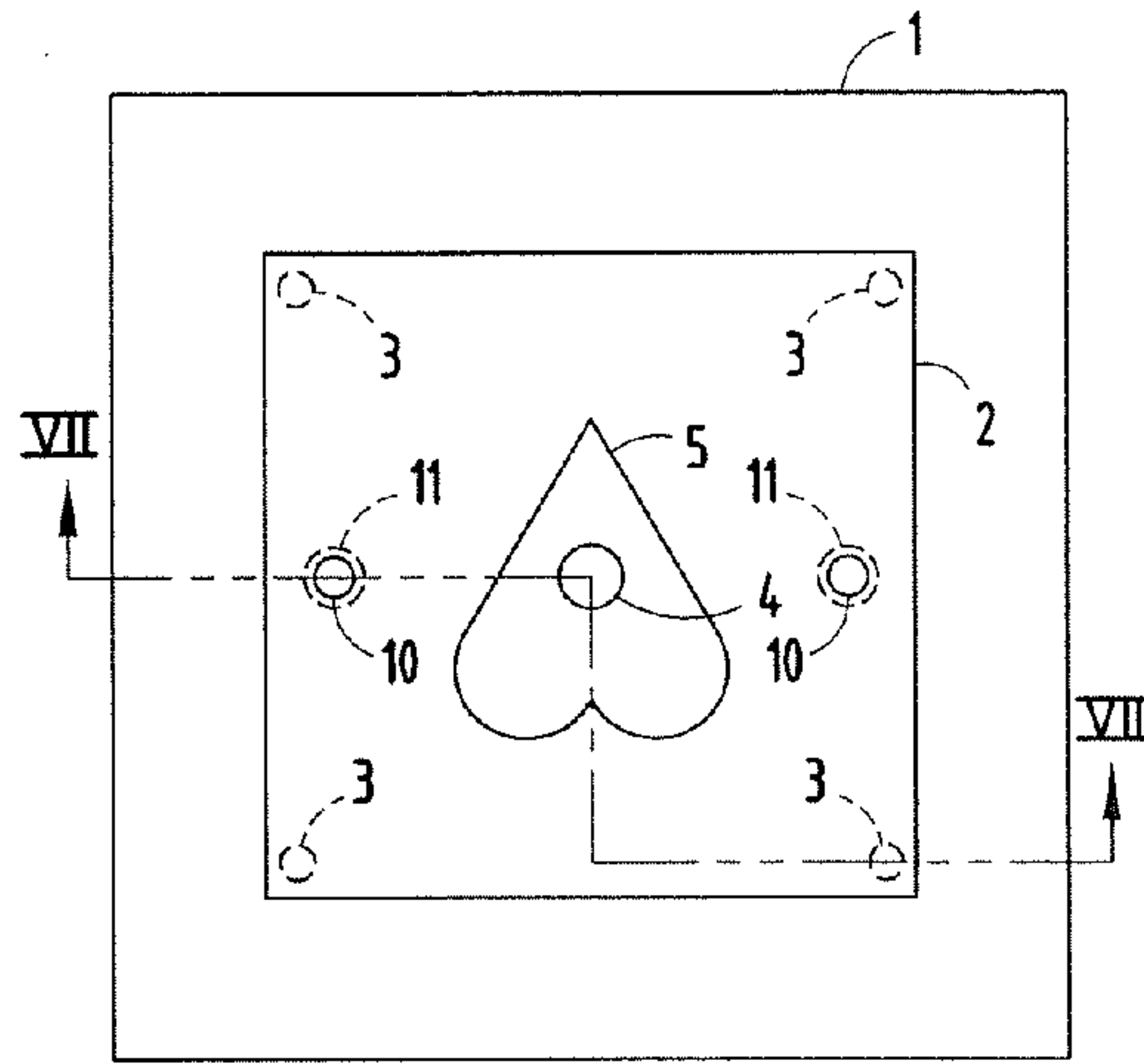
FIG. 6 PRIOR ART
