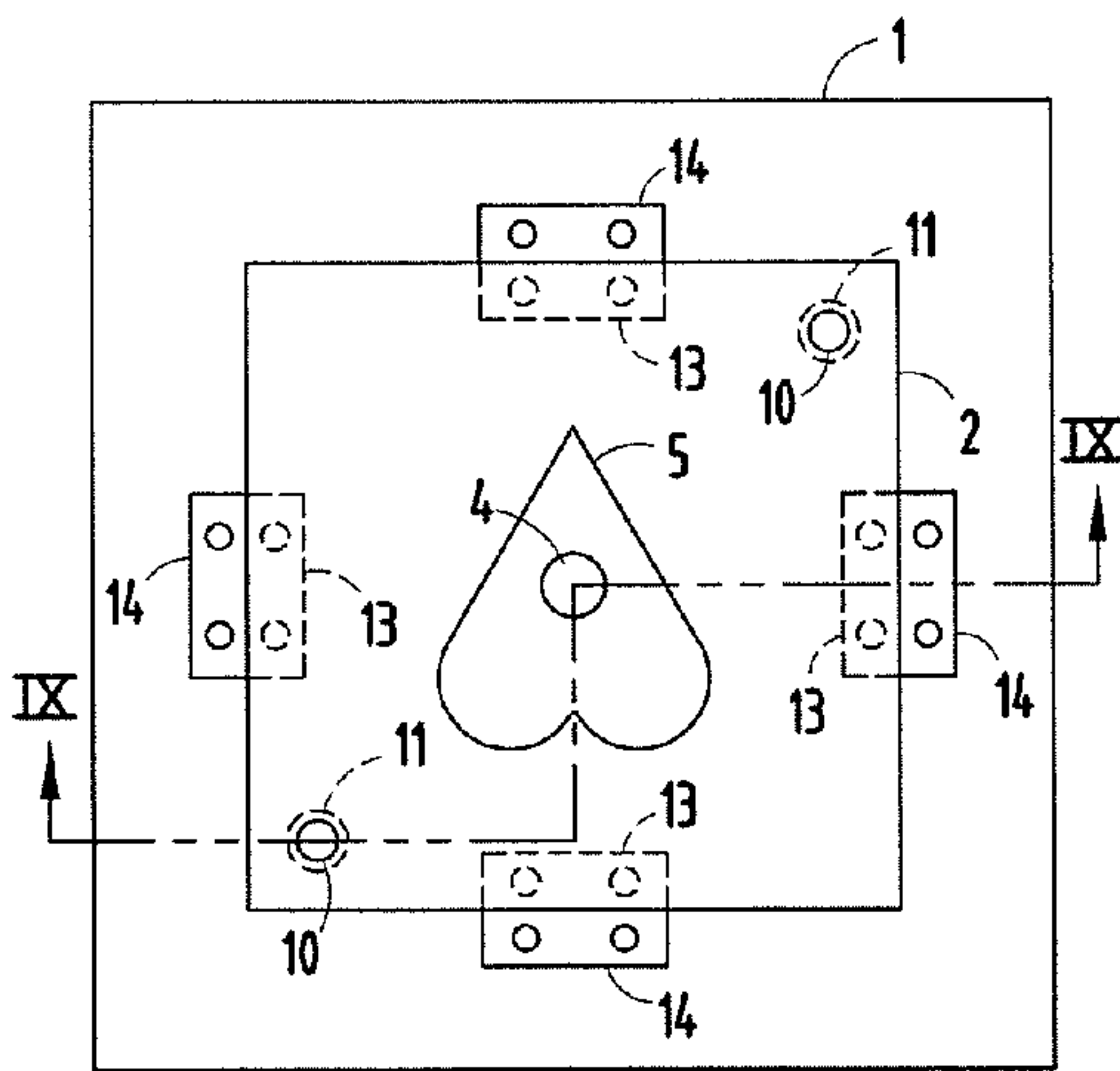
FIG. 8 PRIOR ART
