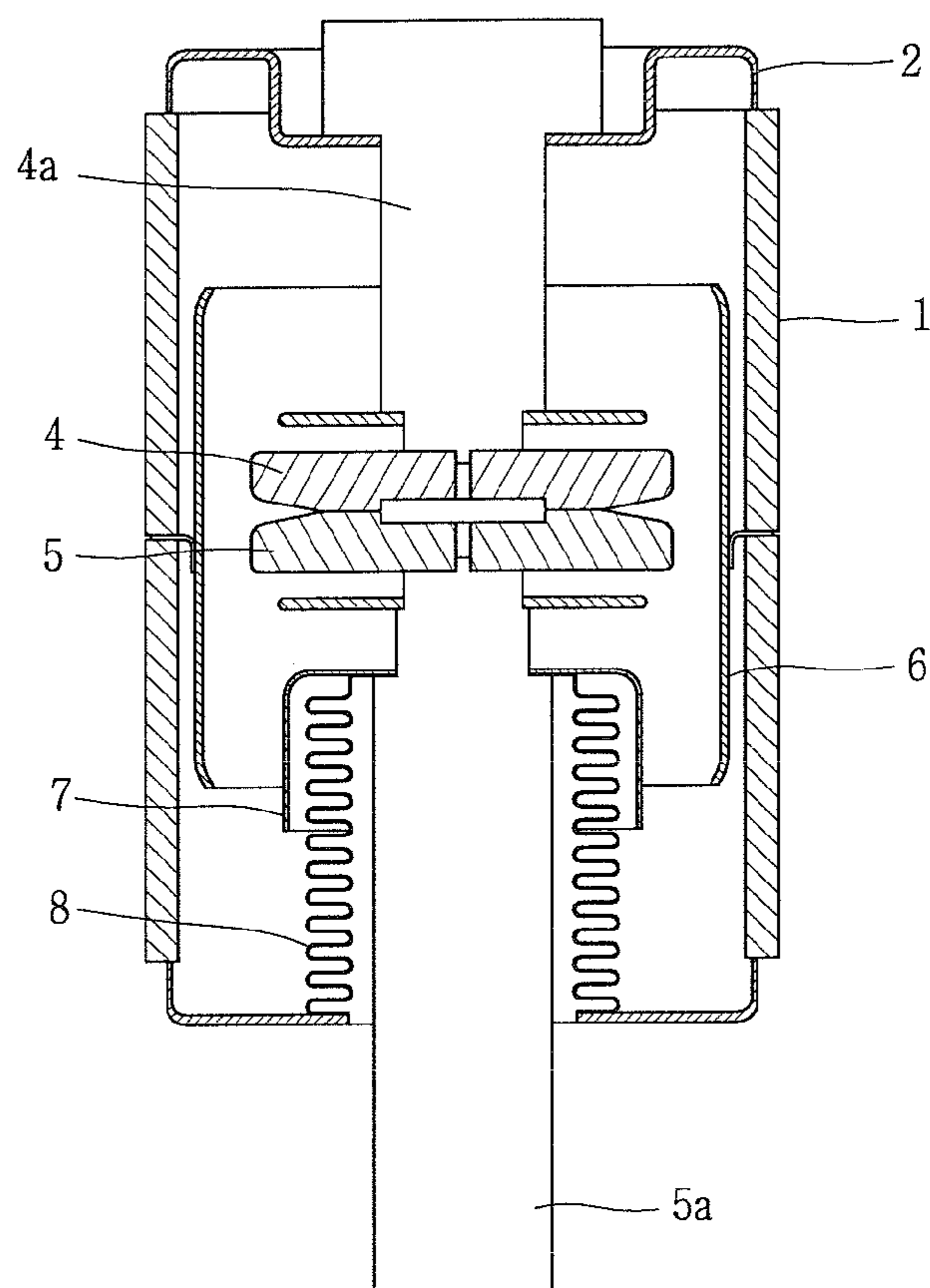
FIG. 1 PRIOR ART
