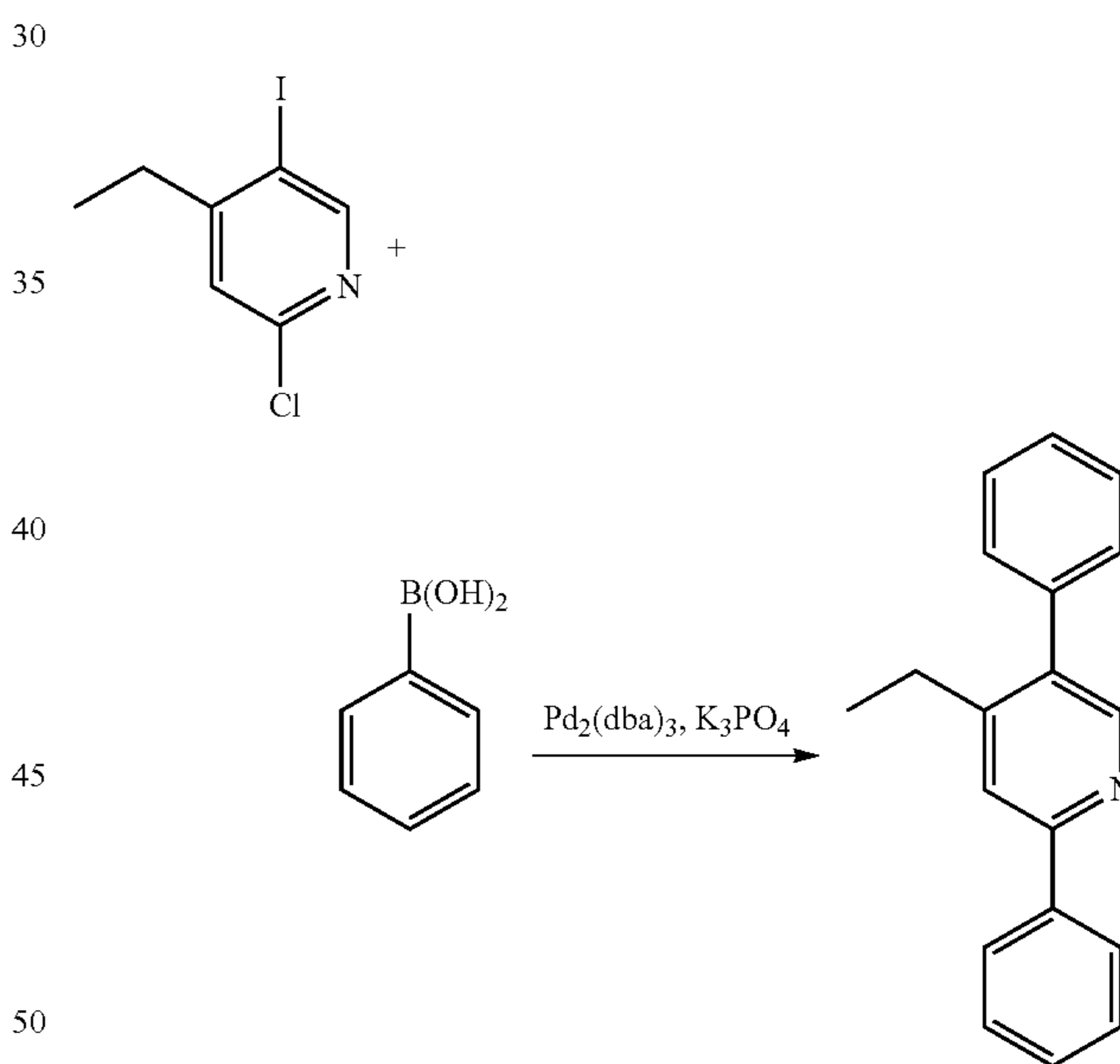
Synthesis of 2,5-diphenyl-4-ethylpyridine
