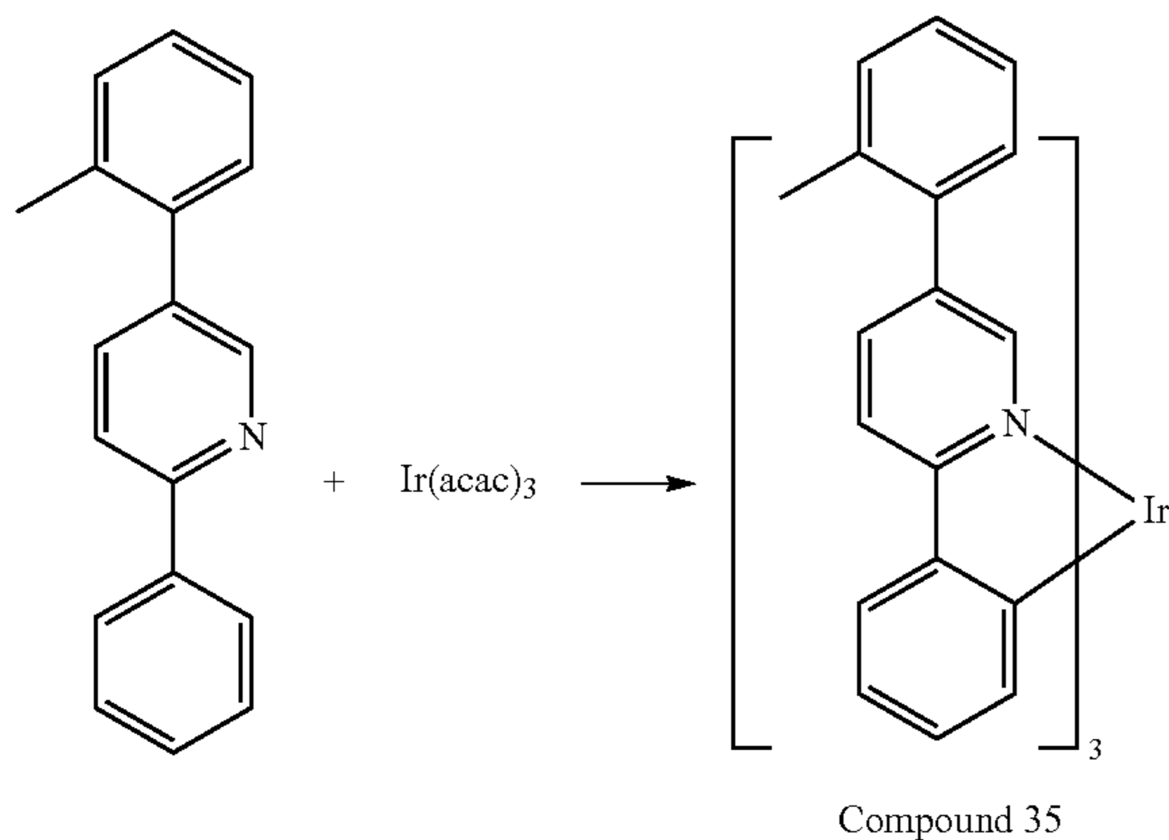
Synthesis of Compound 35
