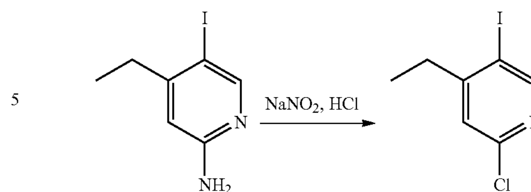
Synthesis of 2-chloro-4-ethyl-5-iodopyridine
