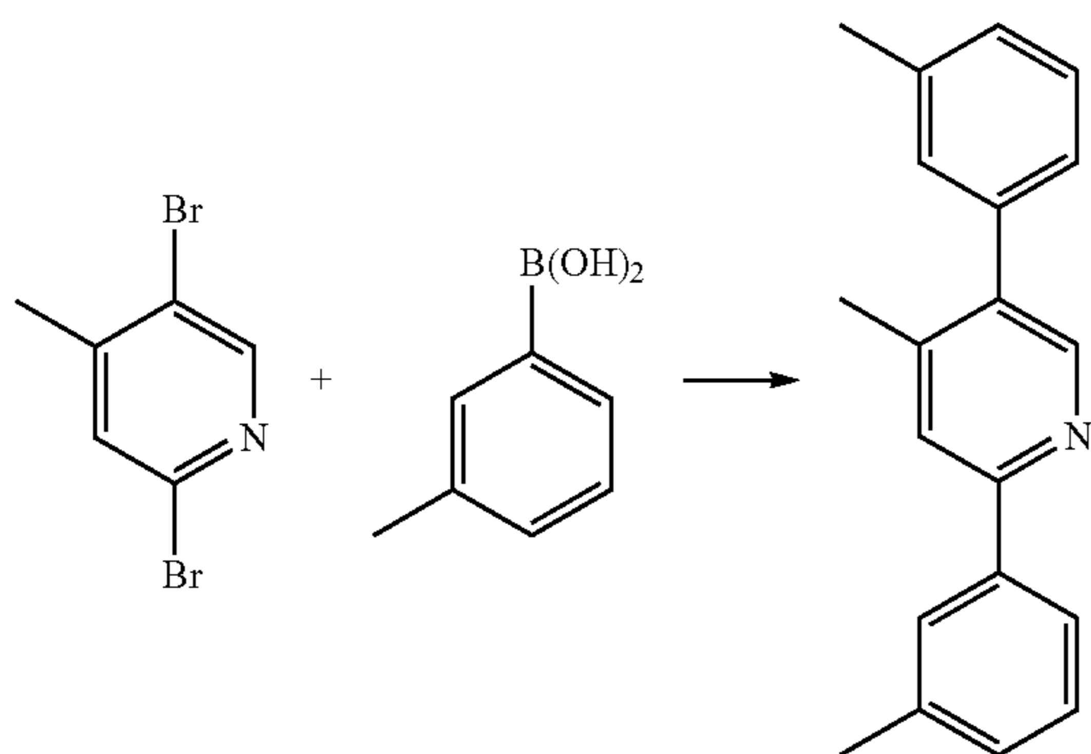
Synthesis of Compound 24
