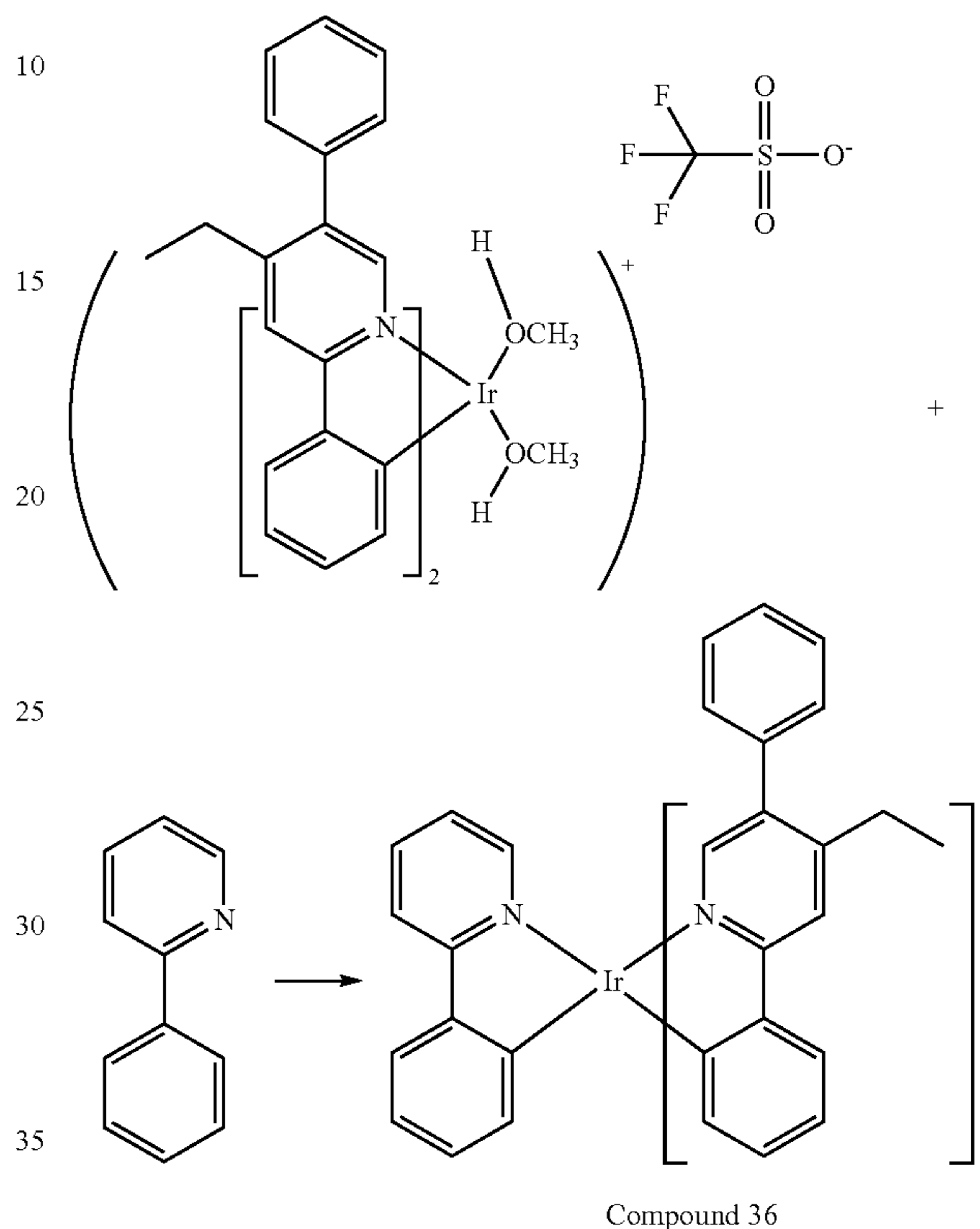
Synthesis of Compound 36
