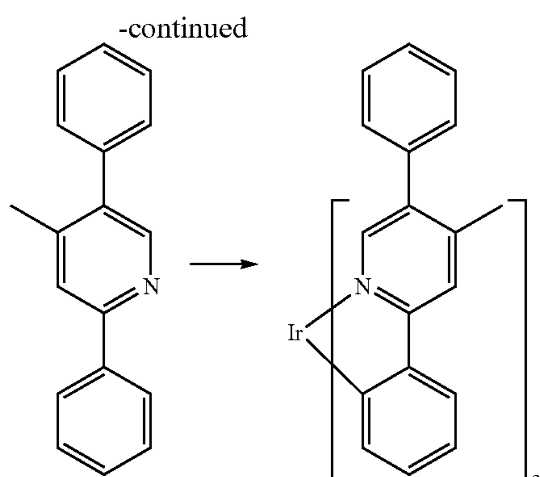
Synthesis of Compound 21
