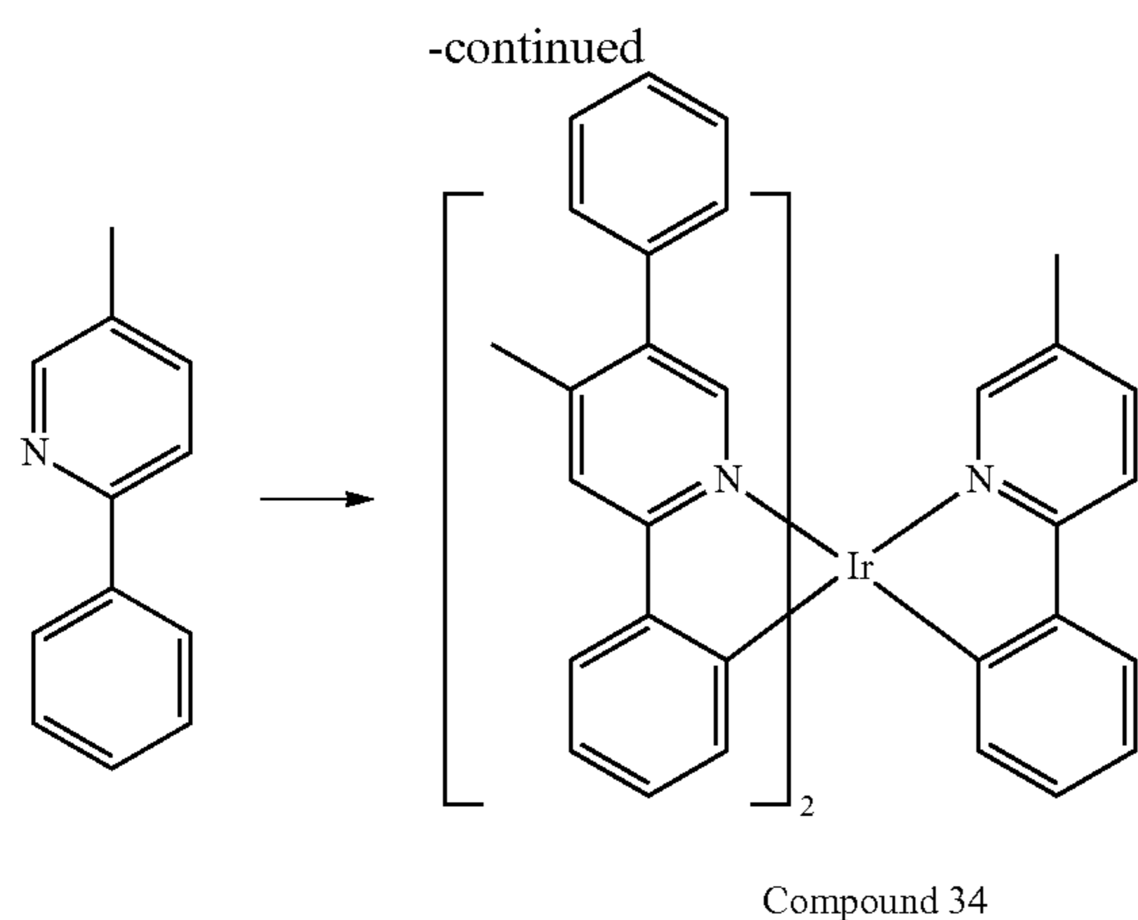
Synthesis of Compound 34
