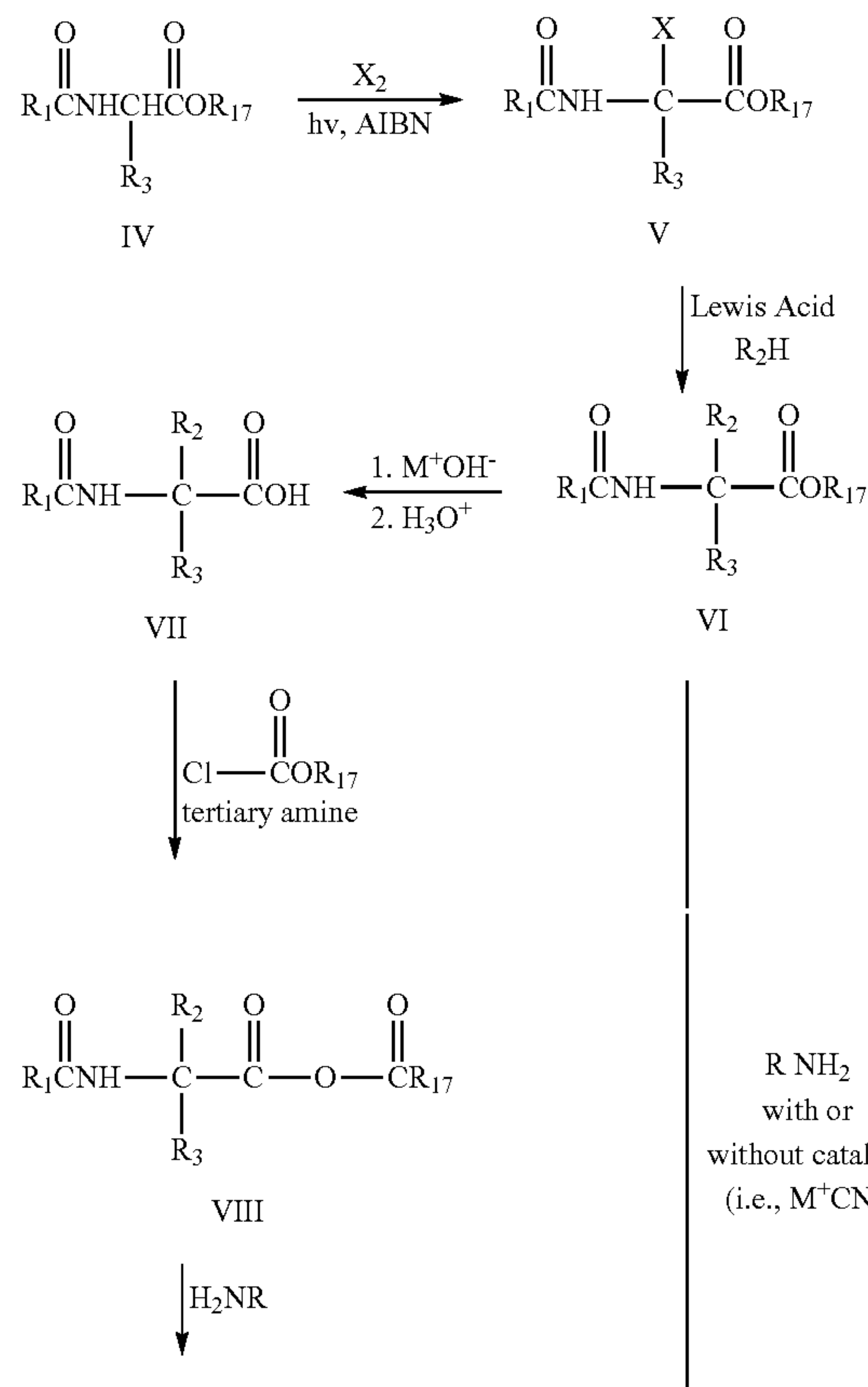
Scheme IV
