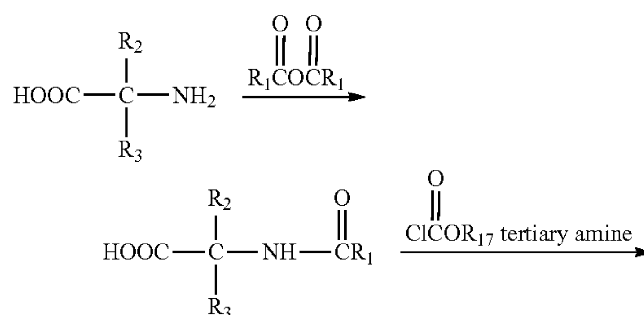
Scheme II
