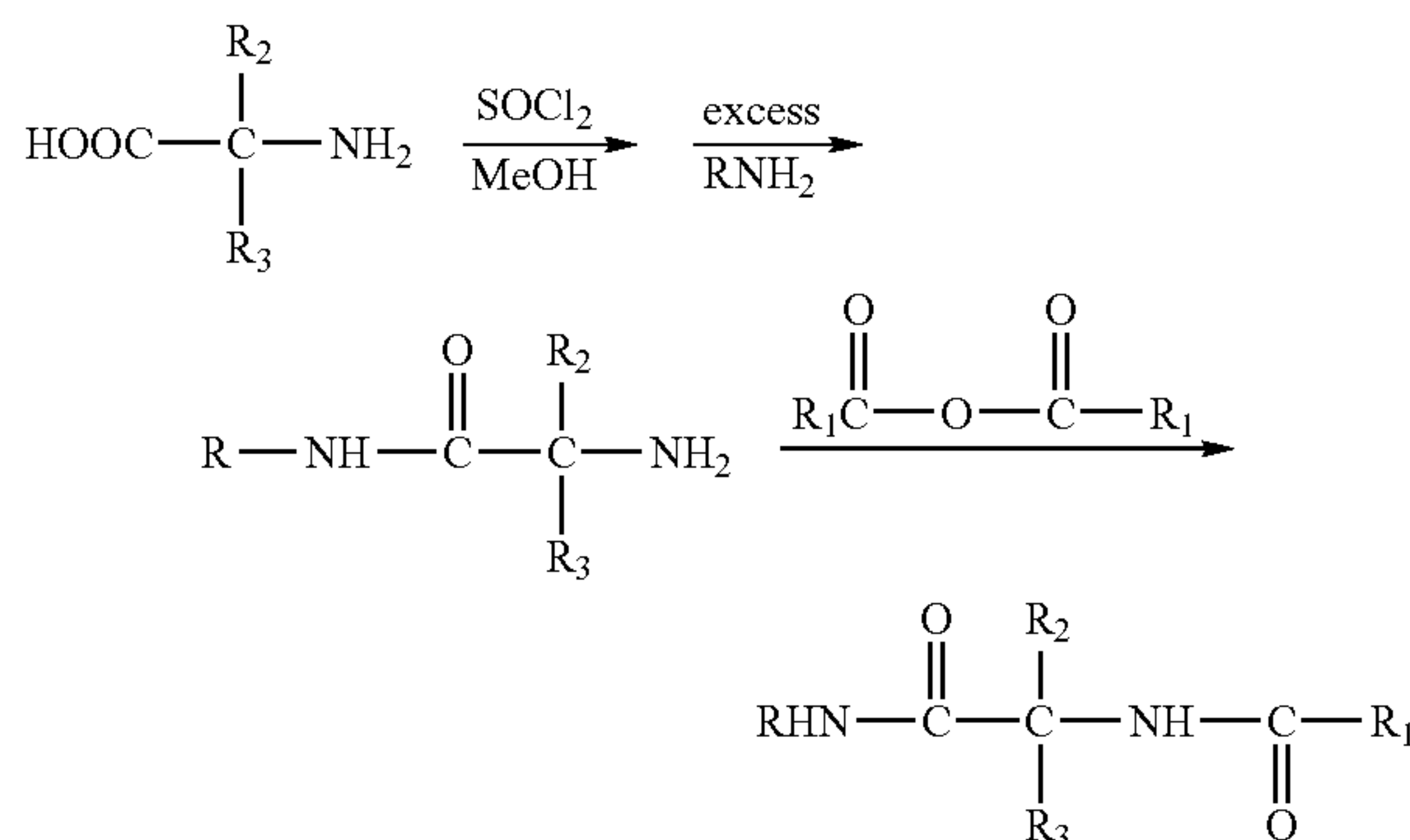
Scheme I
